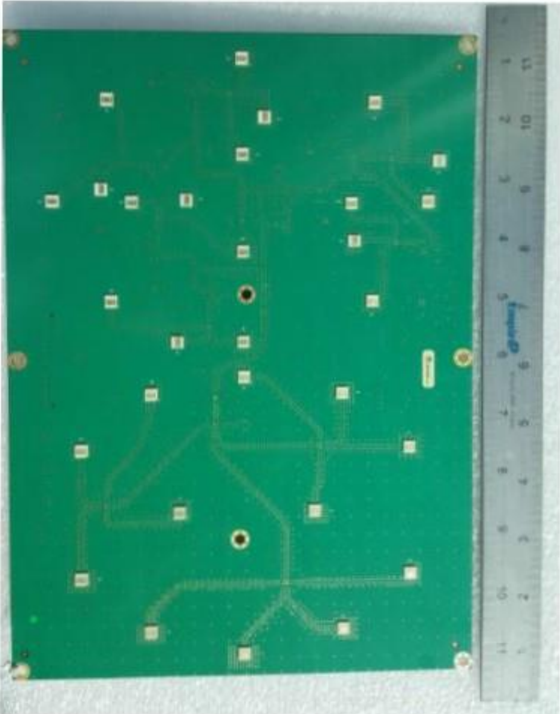
Figure 6 - PCBA,RF Panel,Back (Antenna side)
