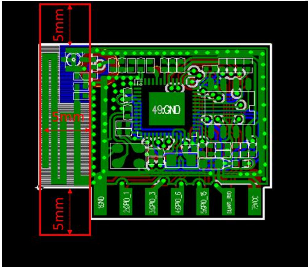
Figure 6 UA504 module antenna clearance diagram
