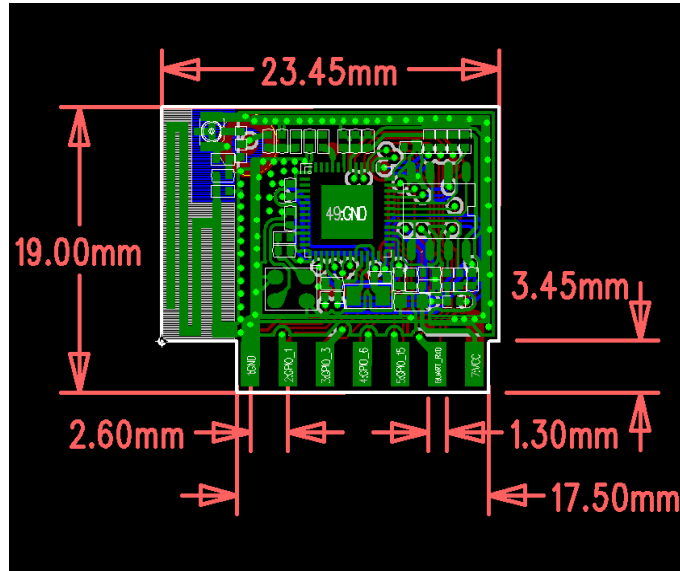
Figure 4 UA504 module dimensions
