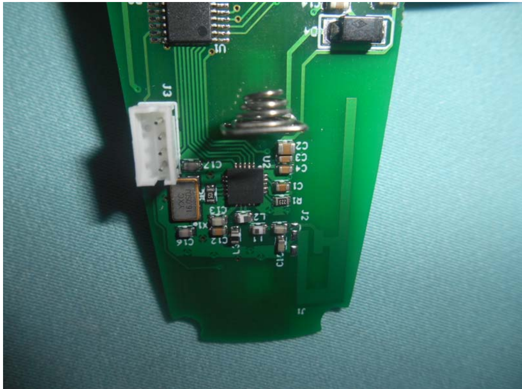
FIGURE 6 FEEDER/AREALIGHT (M/N: FEEDER1-REMOTE) CHIP AND CRYSTAL ON KEYBOARD
