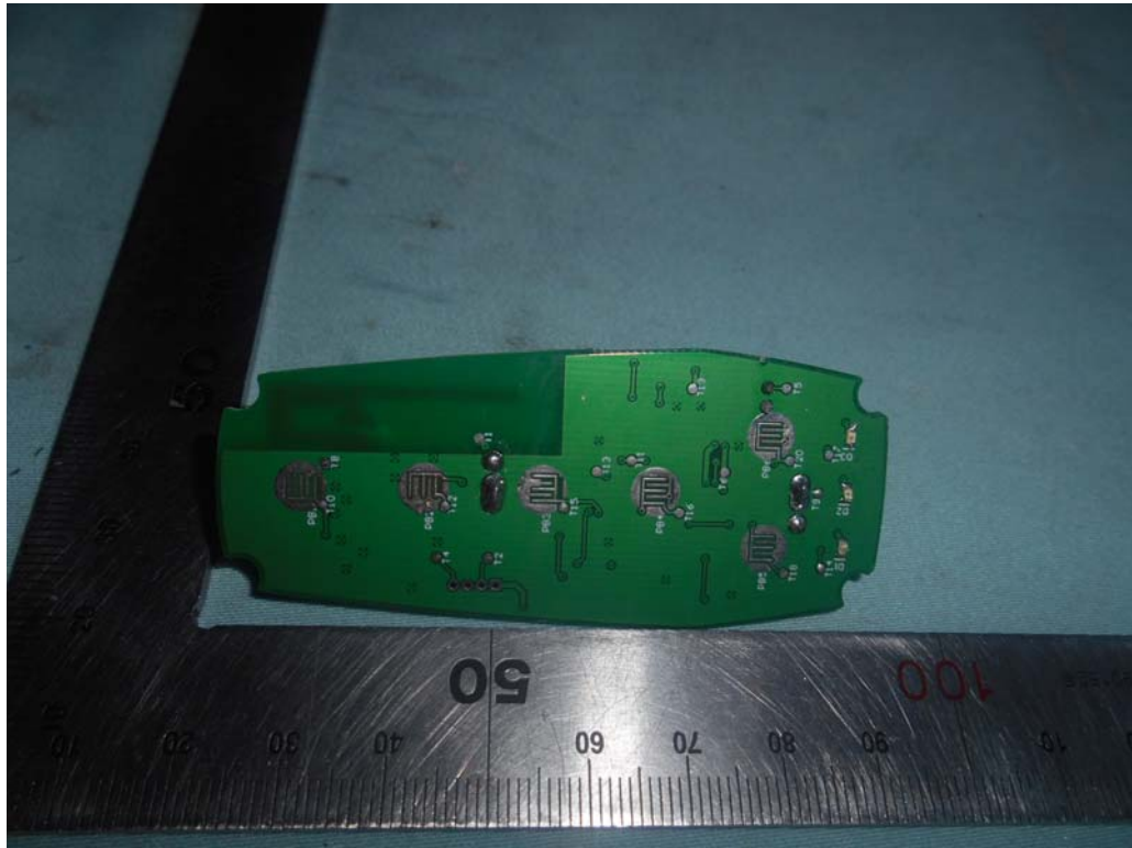
FIGURE 5 FEEDER/AREALIGHT (M/N: FEEDER1-REMOTE) KEYBOARD (BACK VIEW)
