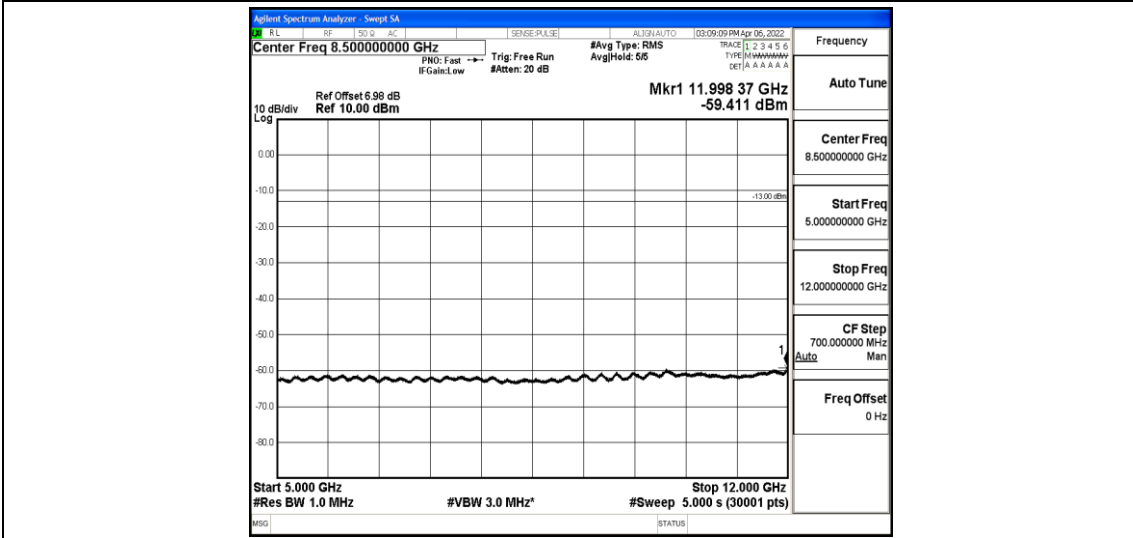
Band12-1.4MHz-QPSK-23173-1-0-High-5000-12000--59.41-PASS
