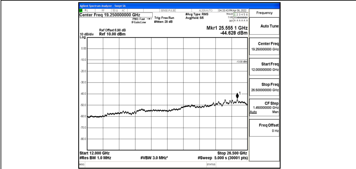
Band12-10MHz-16QAM-23095-1-0-Low-12000-26500--44.63-PASS
