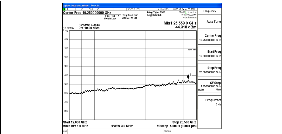
Band12-1.4MHz-16QAM-23095-1-0-Low-12000-26500--44.32-PASS
