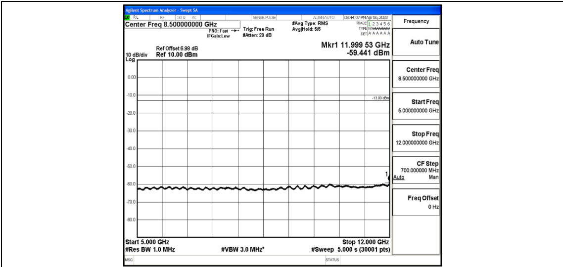
Band12-3MHz-16QAM-23165-1-0-High-5000-12000--59.44-PASS
