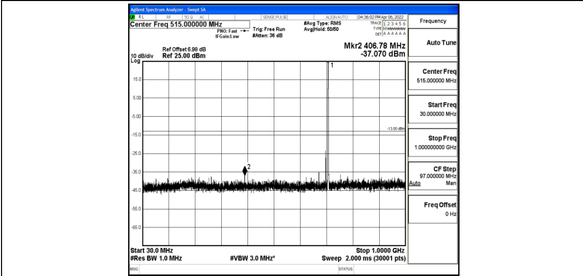
Band12-10MHz-16QAM-23130-1-0-High-30-1000--37.07-PASS
