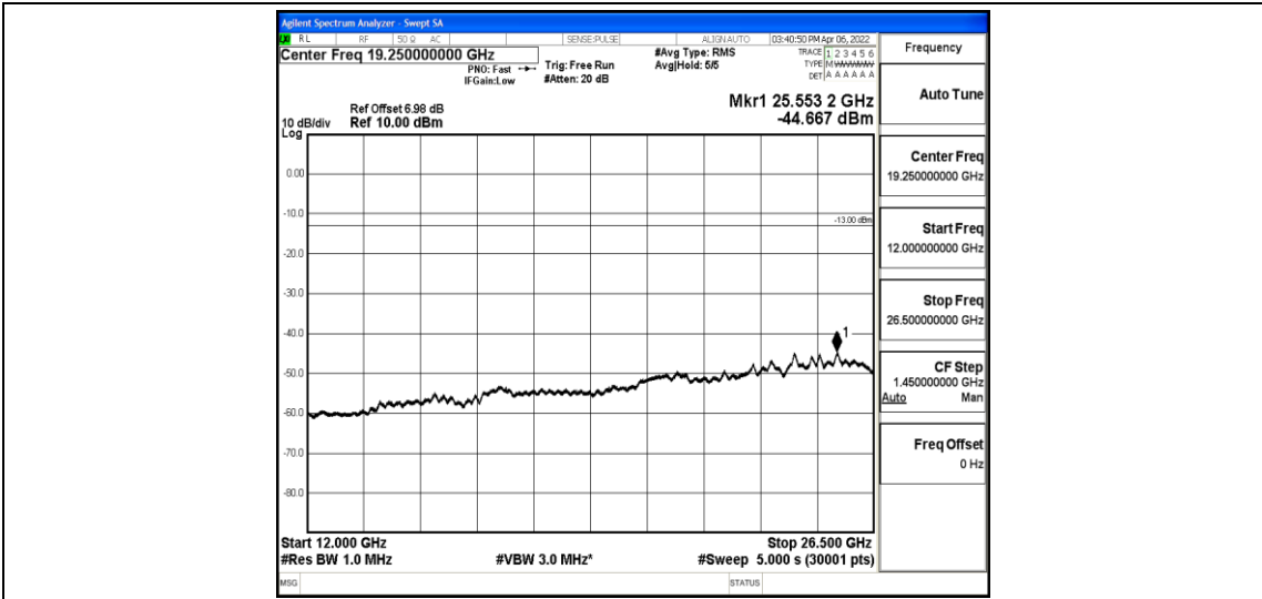
Band12-3MHz-16QAM-23095-1-0-Low-12000-26500--44.67-PASS
