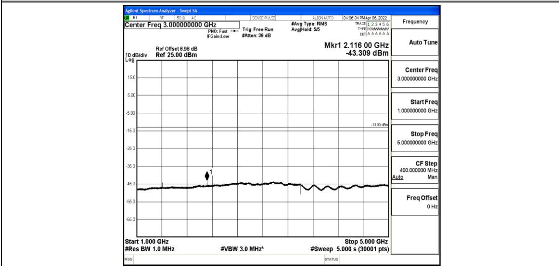
Band12-5MHz-QPSK-23095-1-0-Low-1000-5000--43.31-PASS
