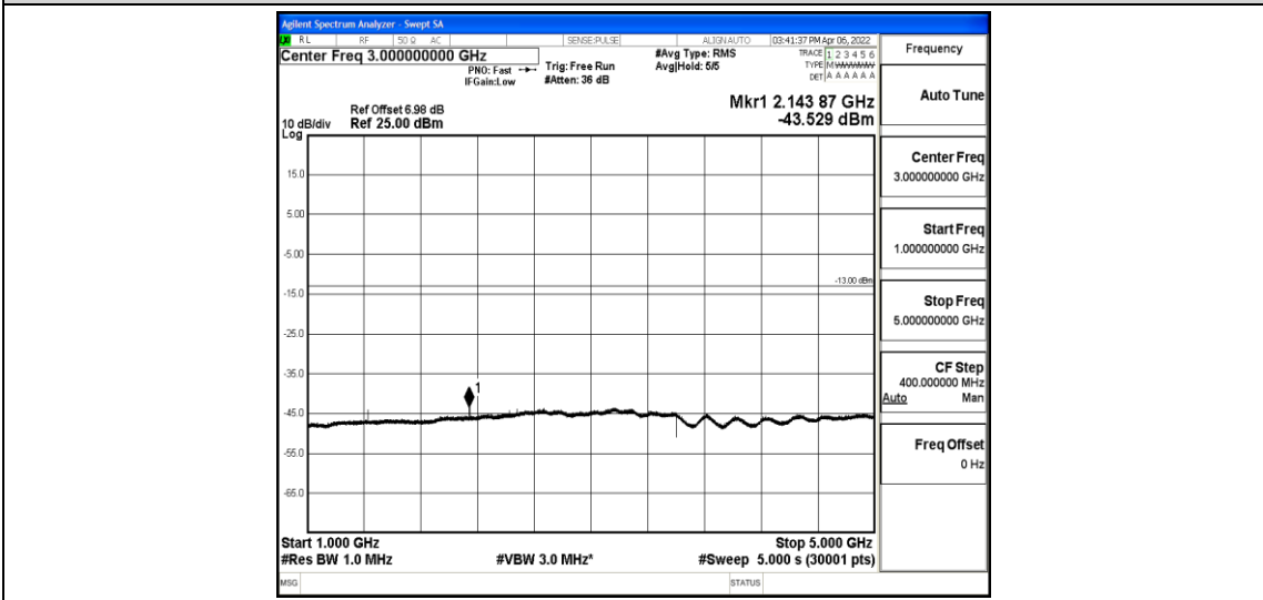
Band12-3MHz-QPSK-23165-1-0-High-1000-5000--43.53-PASS
