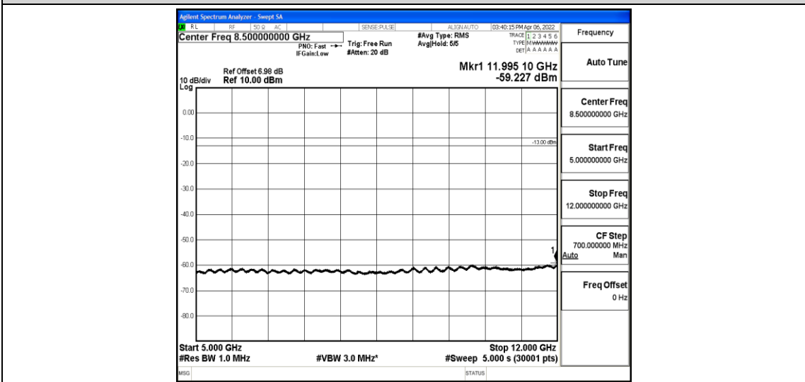
Band12-3MHz-16QAM-23095-1-0-Low-5000-12000--59.23-PASS
