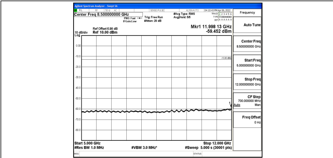
Band12-5MHz-QPSK-23155-1-0-High-5000-12000--59.45-PASS
