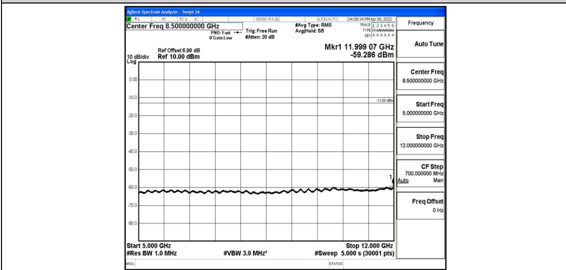
Band12-5MHz-16QAM-23095-1-0-Low-5000-12000--59.29-PASS
