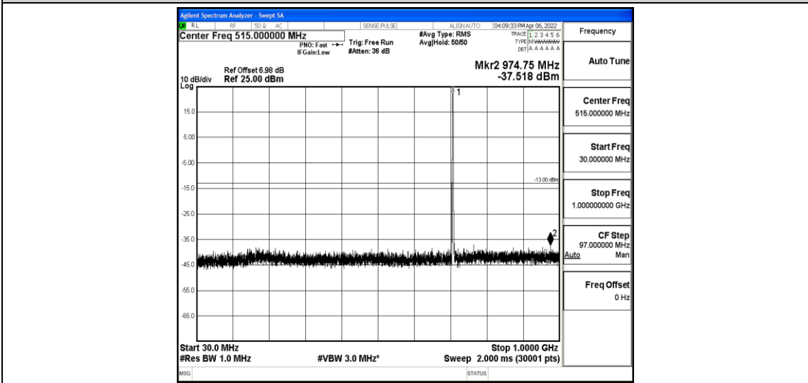
Band12-5MHz-QPSK-23155-1-0-High-30-1000--37.52-PASS
