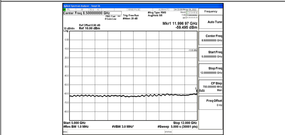
Band12-10MHz-16QAM-23095-1-0-Low-5000-12000--59.5-PASS
