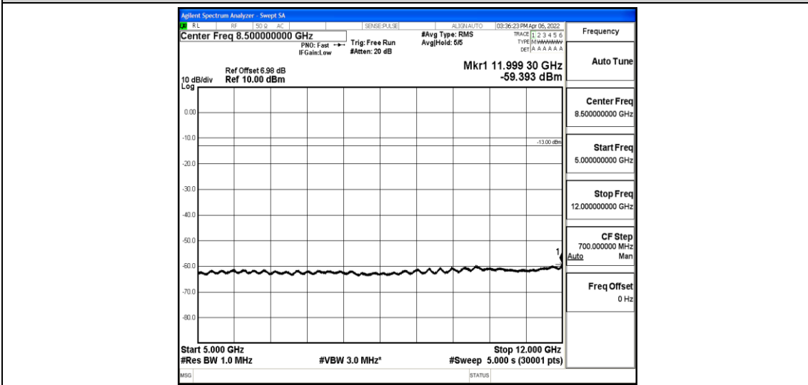
Band12-3MHz-16QAM-23025-1-0-Low-5000-12000--59.39-PASS
