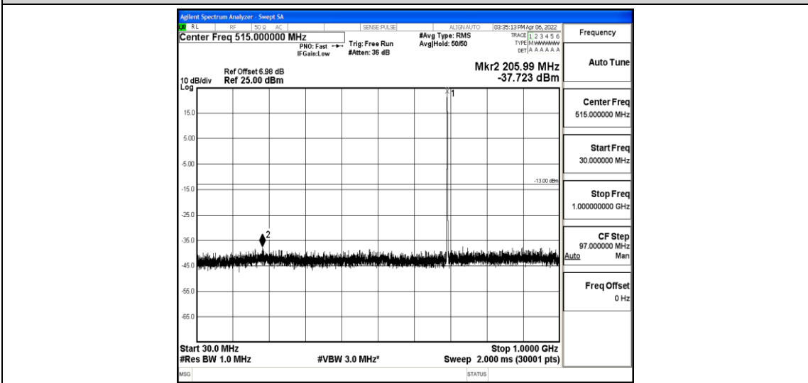
Band12-3MHz-16QAM-23025-1-0-Low-30-1000--37.72-PASS
