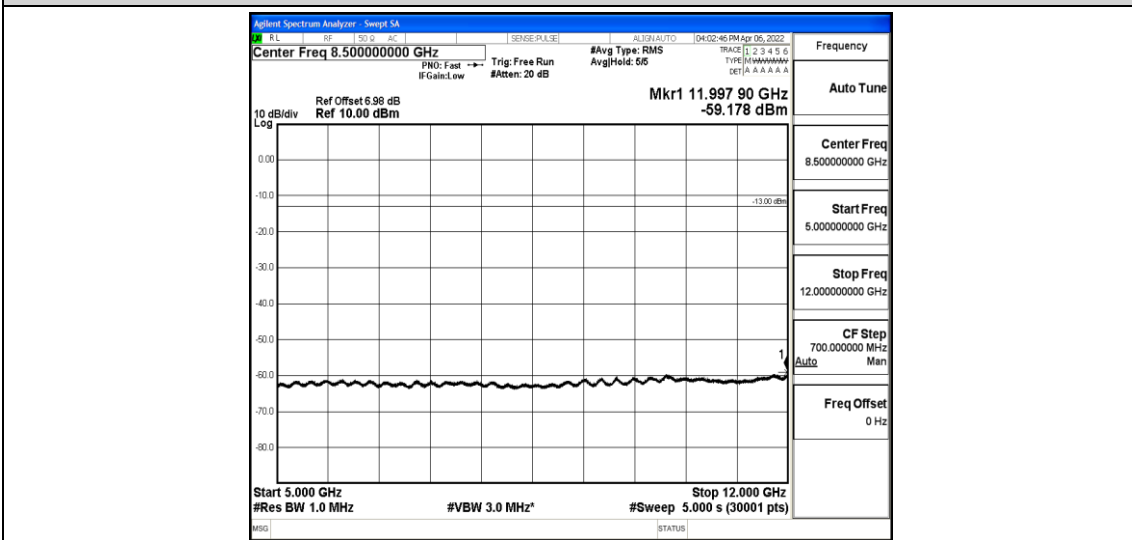
Band12-5MHz-QPSK-23035-1-0-Low-5000-12000--59.18-PASS
