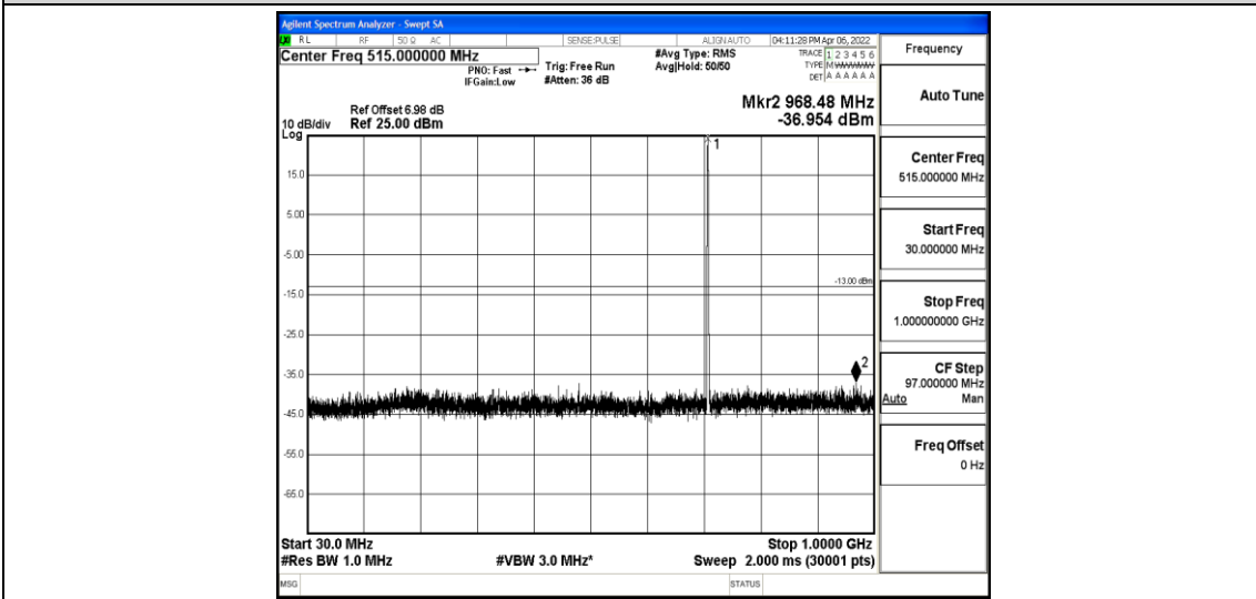
Band12-5MHz-16QAM-23155-1-0-High-30-1000--36.95-PASS
