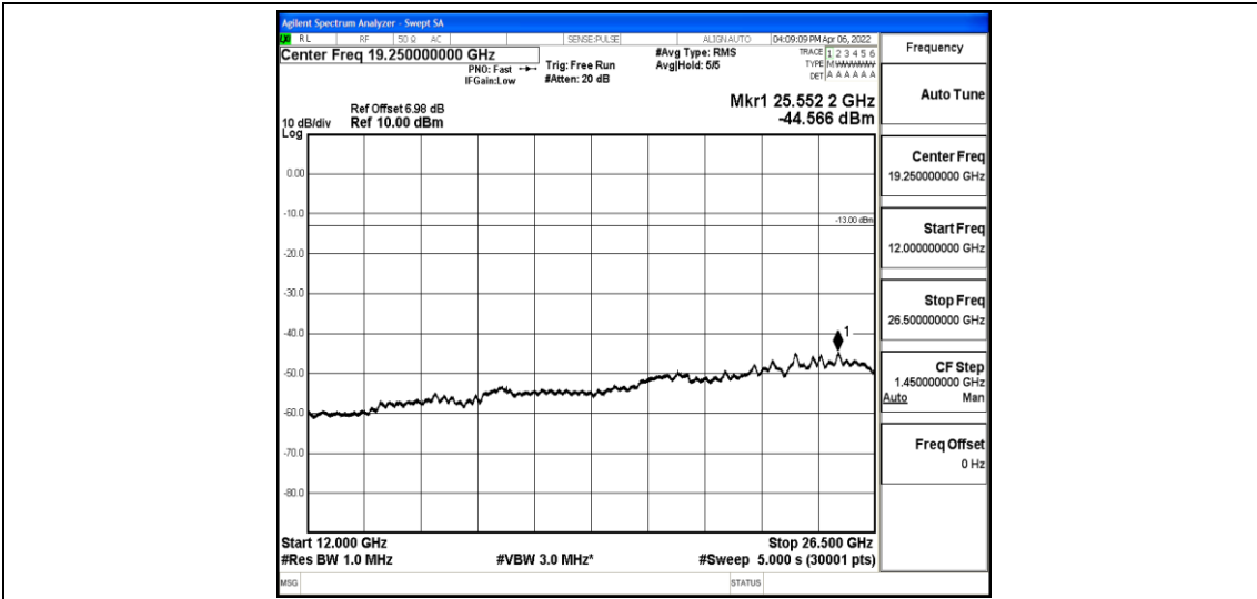
Band12-5MHz-16QAM-23095-1-0-Low-12000-26500--44.57-PASS
