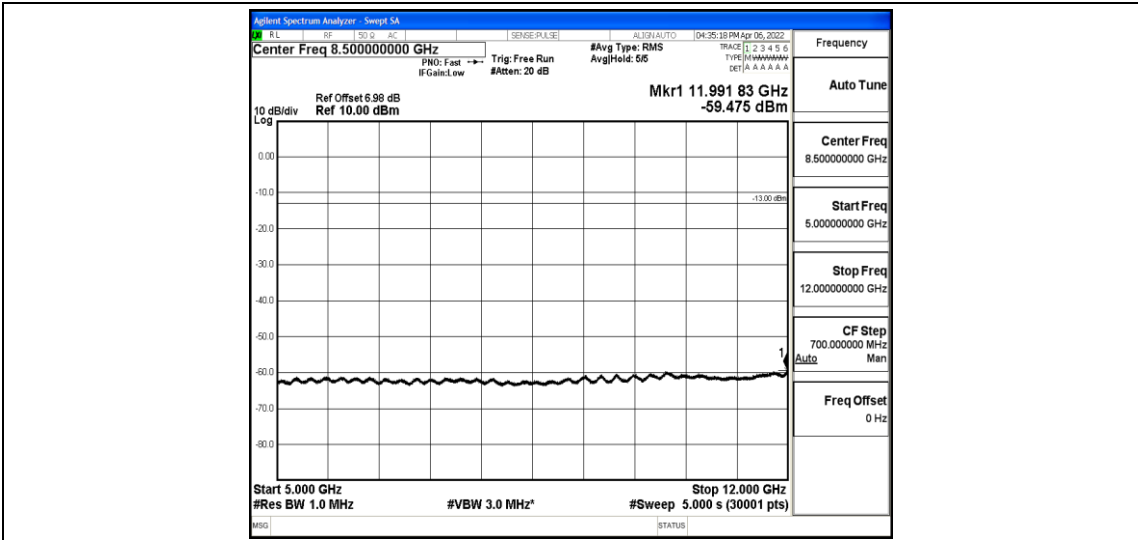
Band12-10MHz-QPSK-23130-1-0-High-5000-12000--59.48-PASS
