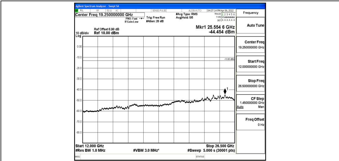
Band12-5MHz-QPSK-23095-1-0-Low-12000-26500--44.45-PASS
