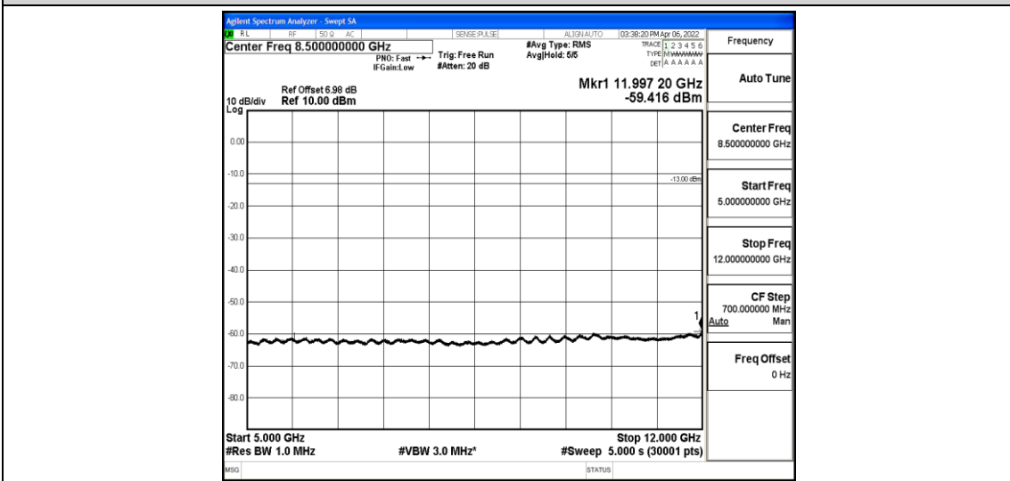
Band12-3MHz-QPSK-23095-1-0-Low-5000-12000--59.42-PASS
