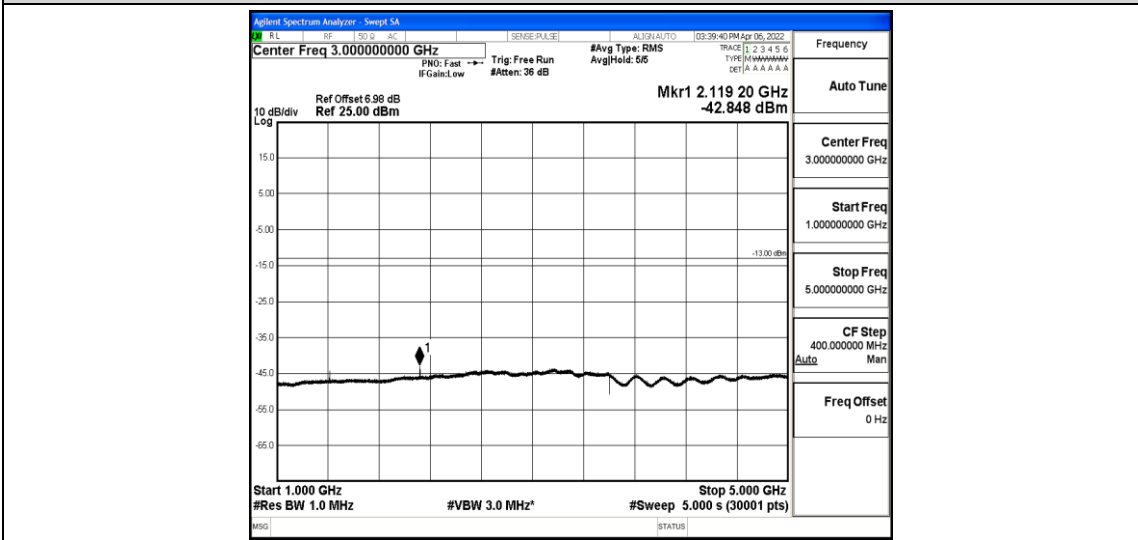
Band12-3MHz-16QAM-23095-1-0-Low-1000-5000--42.85-PASS
