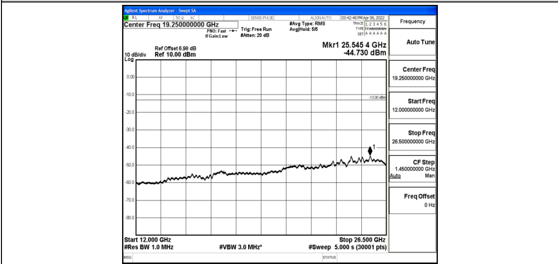
Band12-3MHz-QPSK-23165-1-0-High-12000-26500--44.73-PASS
