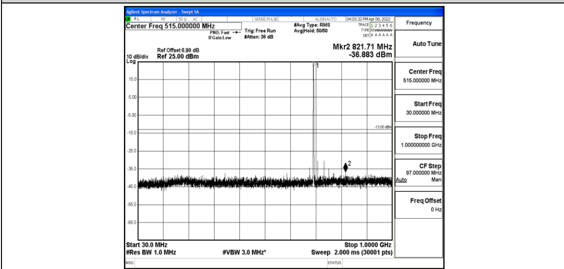
Band12-5MHz-16QAM-23035-1-0-Low-30-1000--36.88-PASS
