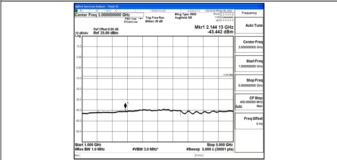
Band12-3MHz-16QAM-23165-1-0-High-1000-5000--43.44-PASS
