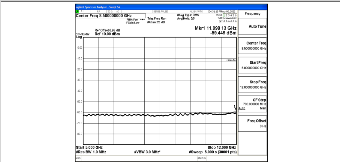
Band12-10MHz-QPSK-23095-1-0-Low-5000-12000--59.45-PASS
