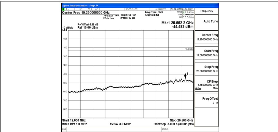
Band12-10MHz-QPSK-23095-1-0-Low-12000-26500--44.48-PASS
