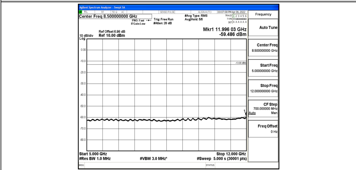
Band12-1.4MHz-16QAM-23095-1-0-Low-5000-12000--59.49-PASS
