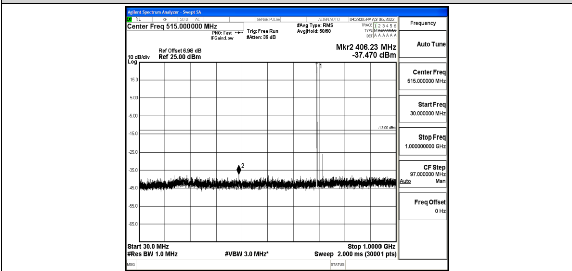
Band12-10MHz-16QAM-23060-1-0-Low-30-1000--37.47-PASS
