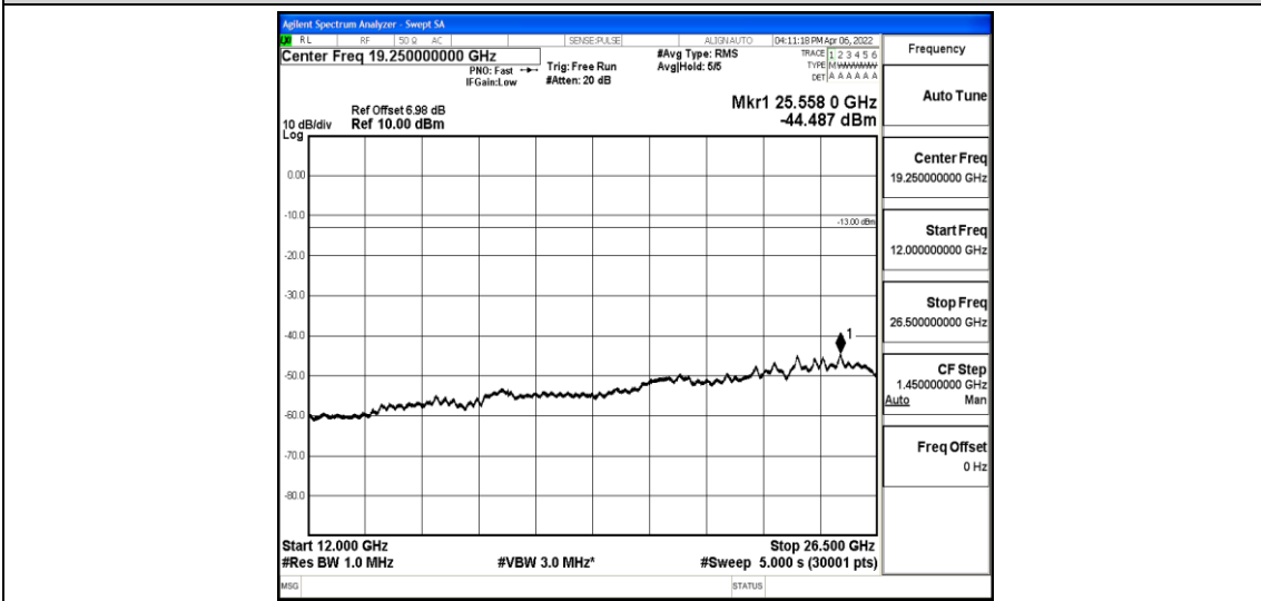
Band12-5MHz-QPSK-23155-1-0-High-12000-26500--44.49-PASS
