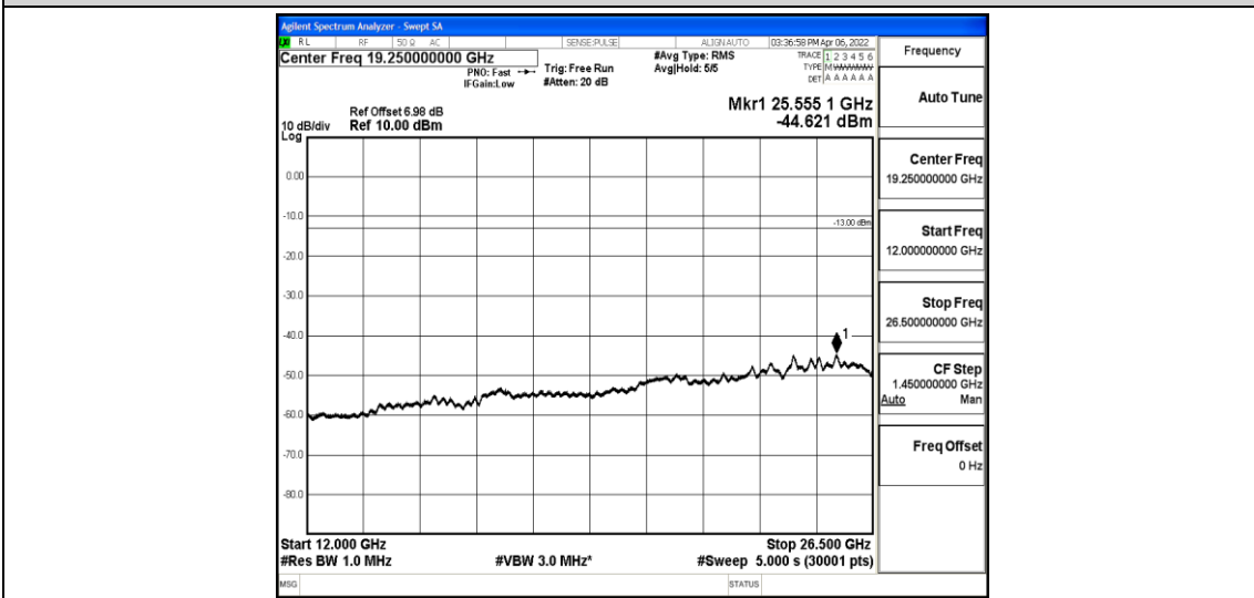
Band12-3MHz-16QAM-23025-1-0-Low-12000-26500--44.62-PASS
