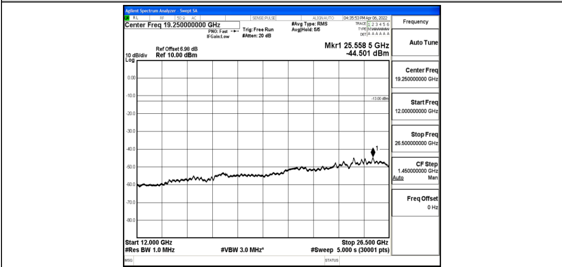
Band12-10MHz-QPSK-23130-1-0-High-12000-26500--44.5-PASS
