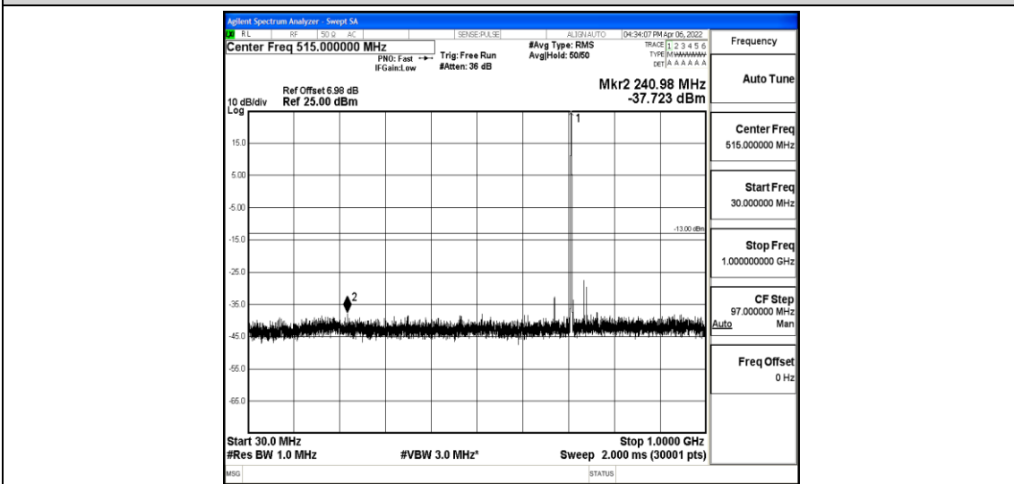
Band12-10MHz-QPSK-23130-1-0-High-30-1000--37.72-PASS
