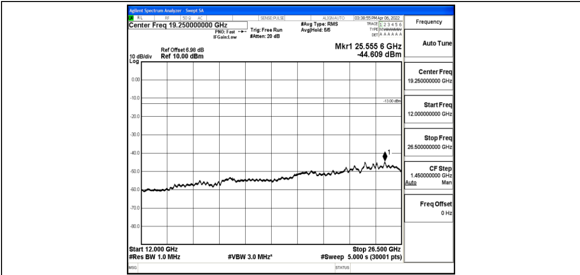
Band12-3MHz-QPSK-23095-1-0-Low-12000-26500--44.61-PASS
