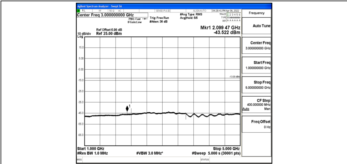
Band12-10MHz-16QAM-23060-1-0-Low-1000-5000--43.52-PASS
