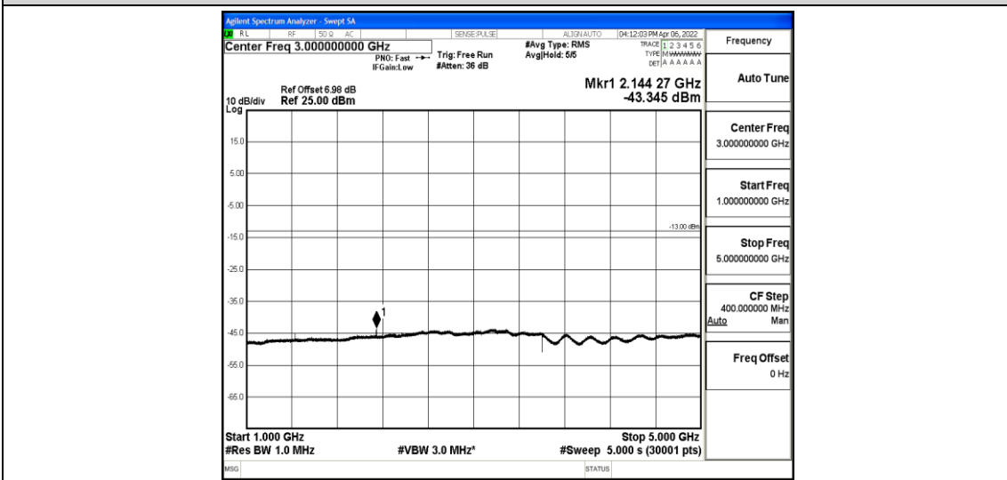
Band12-5MHz-16QAM-23155-1-0-High-1000-5000--43.35-PASS
