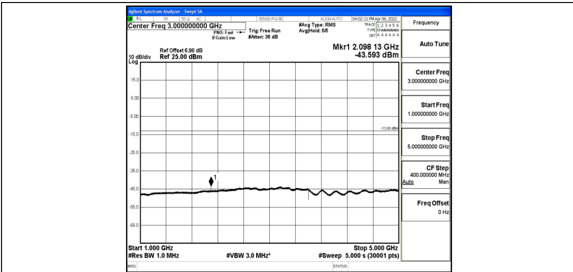
Band12-5MHz-QPSK-23035-1-0-Low-1000-5000--43.59-PASS
