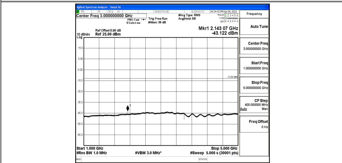
Band12-10MHz-QPSK-23130-1-0-High-1000-5000--43.12-PASS
