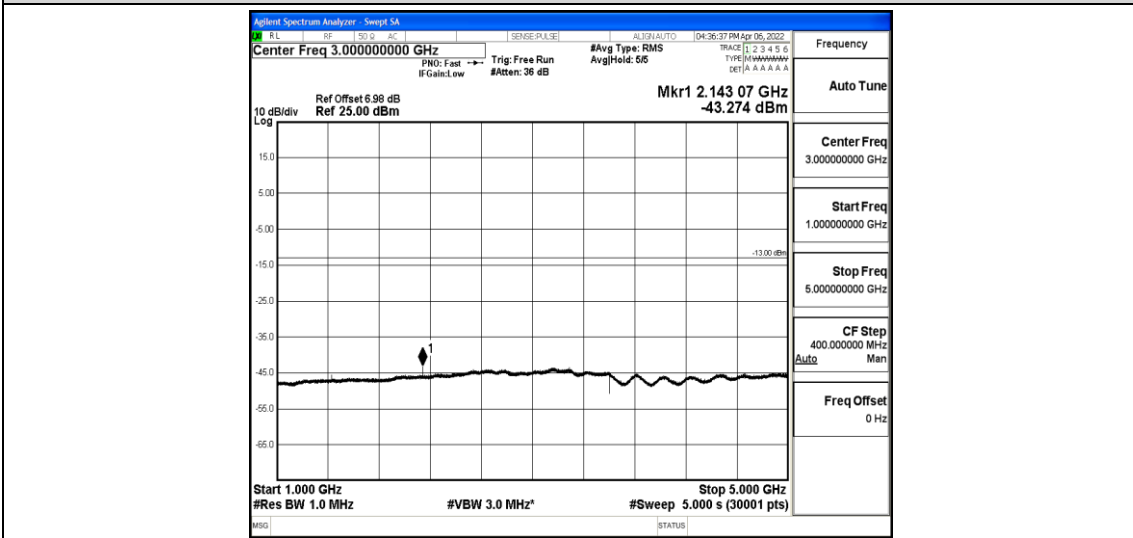
Band12-10MHz-16QAM-23130-1-0-High-1000-5000--43.27-PASS
