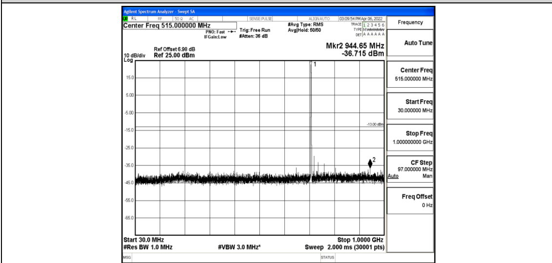
Band12-1.4MHz-16QAM-23173-1-0-High-30-1000--36.72-PASS
