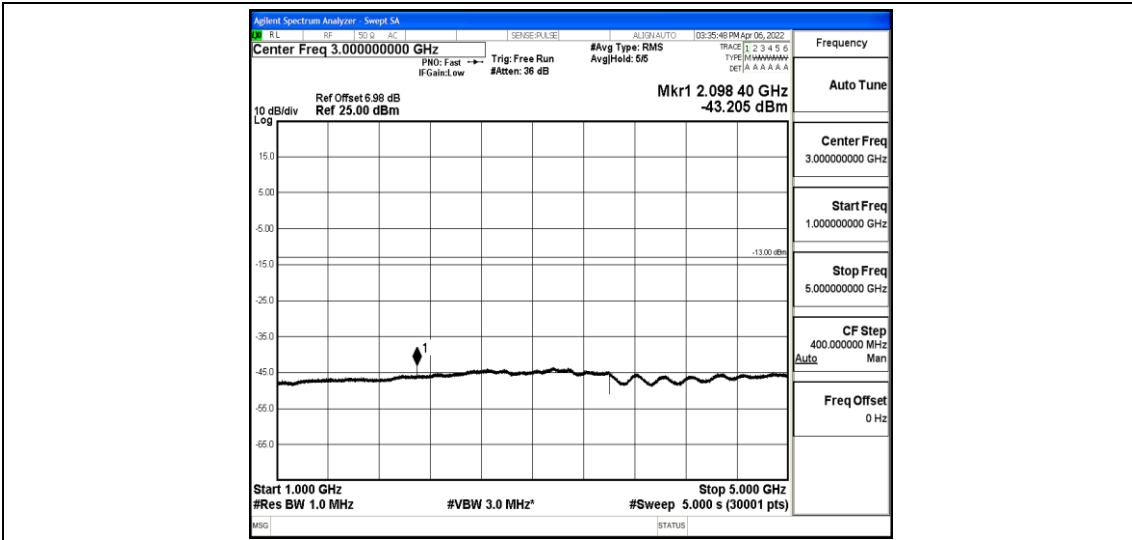
Band12-3MHz-16QAM-23025-1-0-Low-1000-5000--43.21-PASS
