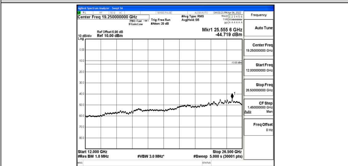
Band12-5MHz-QPSK-23035-1-0-Low-12000-26500--44.72-PASS
