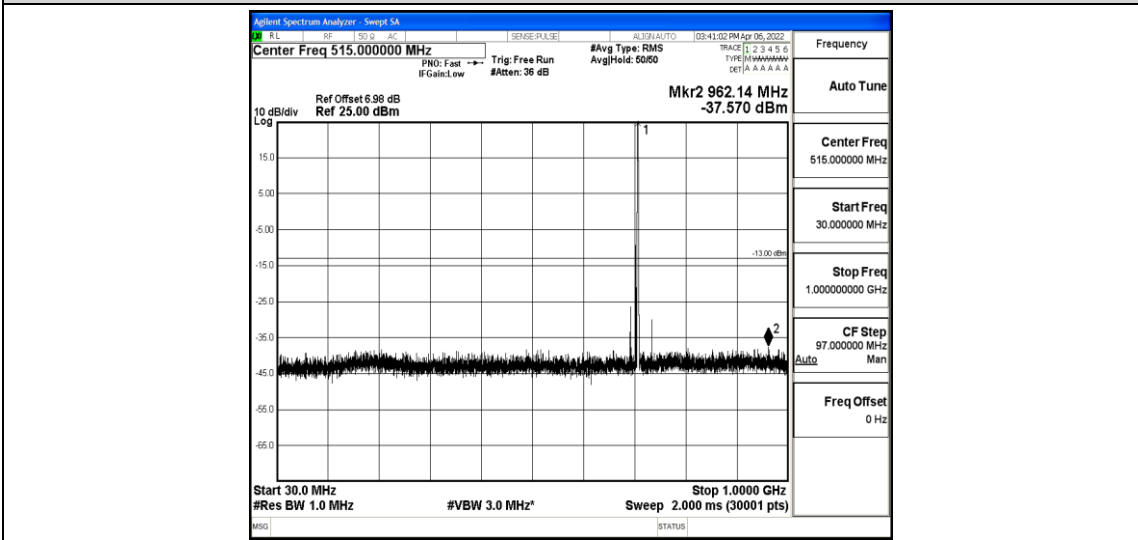
Band12-3MHz-QPSK-23165-1-0-High-30-1000--37.57-PASS
