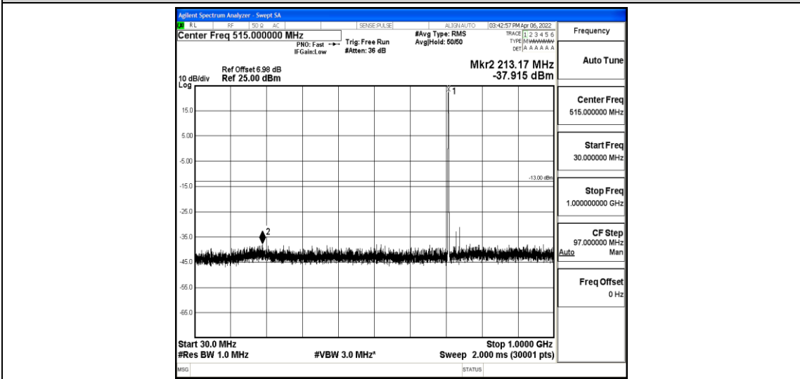
Band12-3MHz-16QAM-23165-1-0-High-30-1000--37.92-PASS
