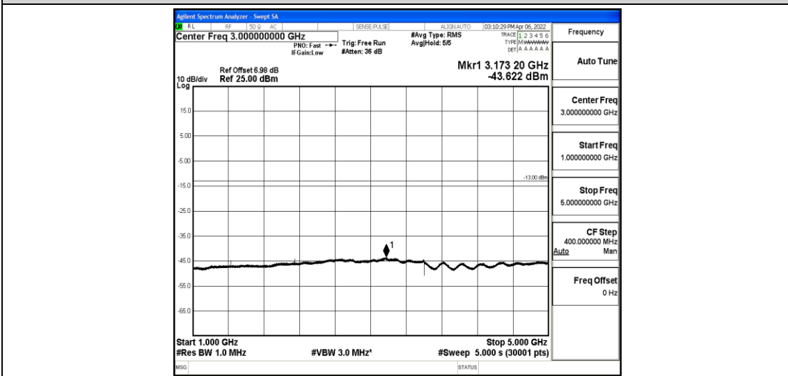
Band12-1.4MHz-16QAM-23173-1-0-High-1000-5000--43.62-PASS
