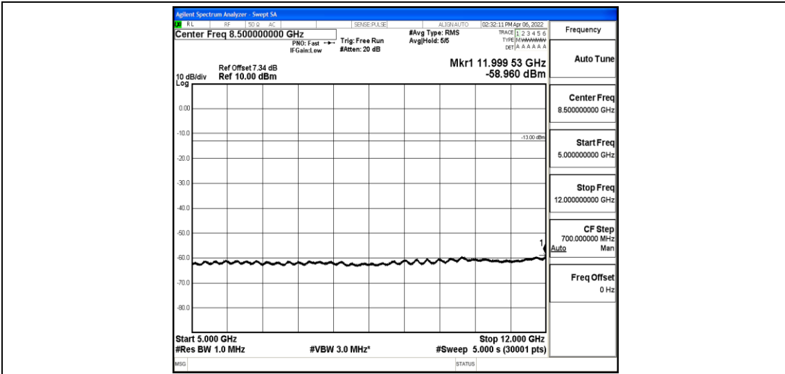
Band5-10MHz-QPSK-20600-1-0-High-5000-12000--58.96-PASS
