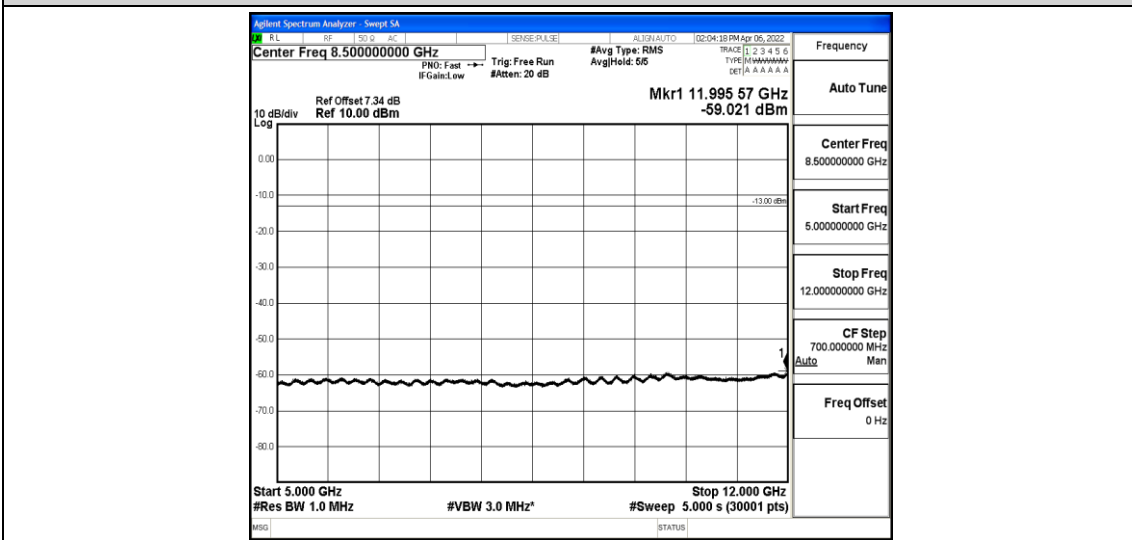
Band5-5MHz-16QAM-20525-1-0-Low-5000-12000--59.02-PASS
