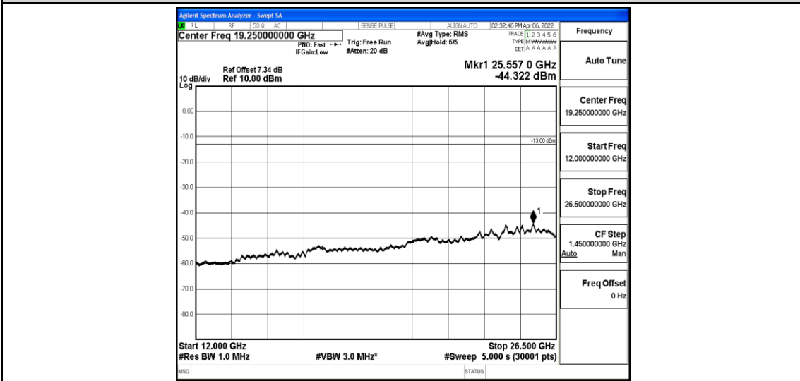
Band5-10MHz-QPSK-20600-1-0-High-12000-26500--44.32-PASS
