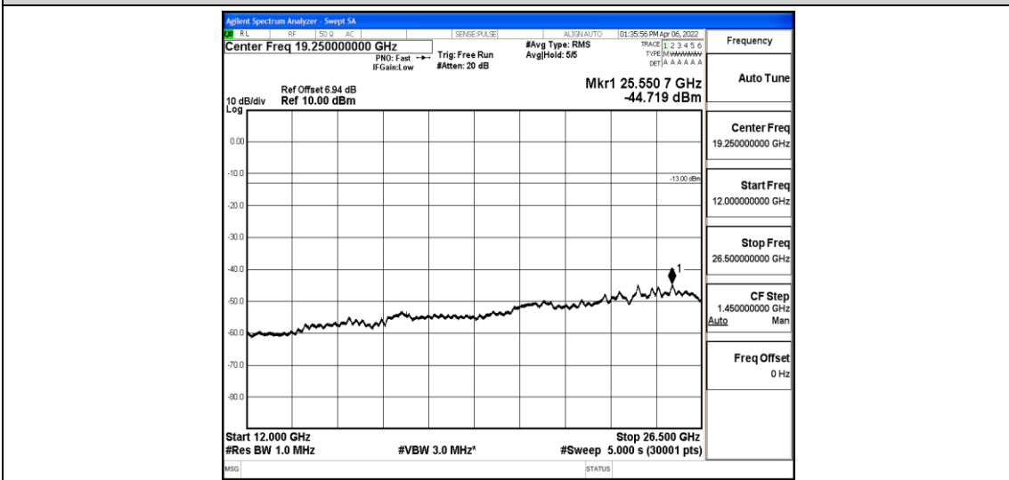
Band5-3MHz-16QAM-20415-1-0-Low-12000-26500--44.72-PASS
