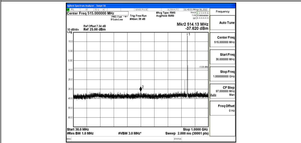
Band5-3MHz-QPSK-20635-1-0-High-30-1000--37.62-PASS
