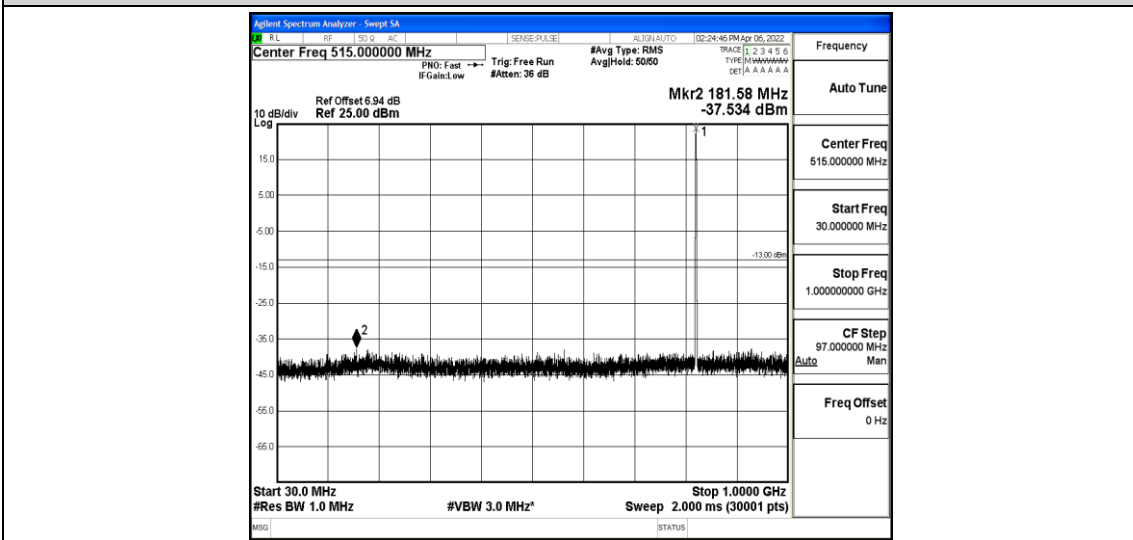
Band5-10MHz-16QAM-20450-1-0-Low-30-1000--37.53-PASS
