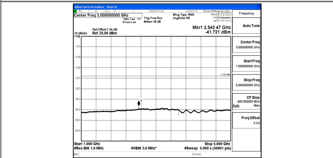
Band5-1.4MHz-16QAM-20643-1-0-High-1000-5000--41.72-PASS
