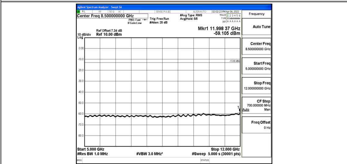
Band5-5MHz-QPSK-20525-1-0-Low-5000-12000--59.11-PASS
