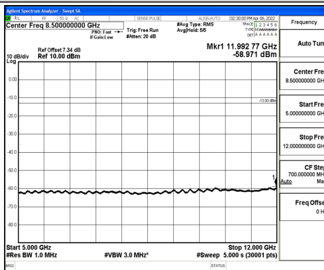
Band5-10MHz-16QAM-20525-1-0-Low-5000-12000--58.97-PASS
