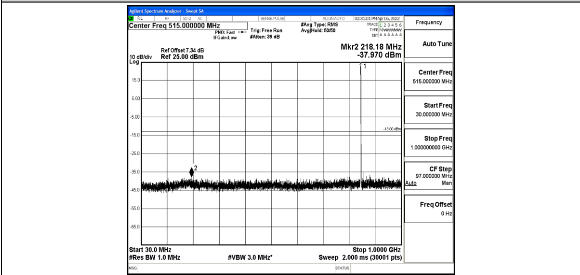
Band5-10MHz-QPSK-20600-1-0-High-30-1000--37.97-PASS
