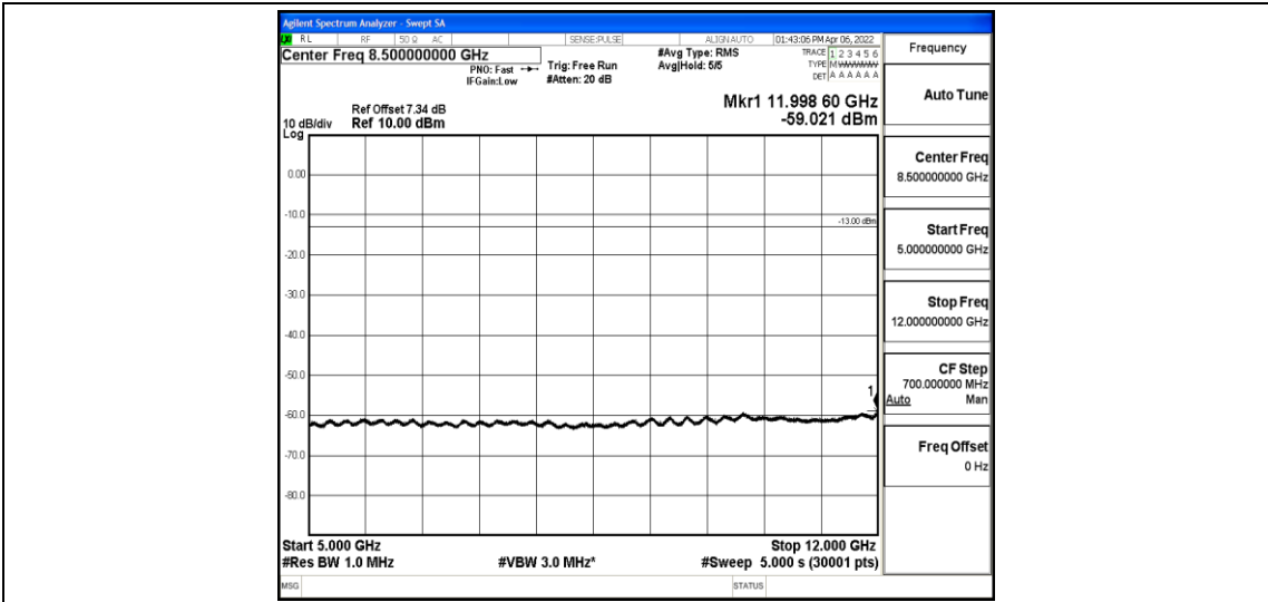
Band5-3MHz-16QAM-20635-1-0-High-5000-12000--59.02-PASS
