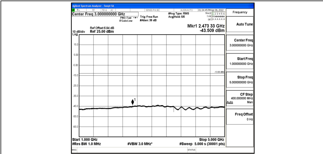
Band5-3MHz-16QAM-20415-1-0-Low-1000-5000--43.51-PASS
