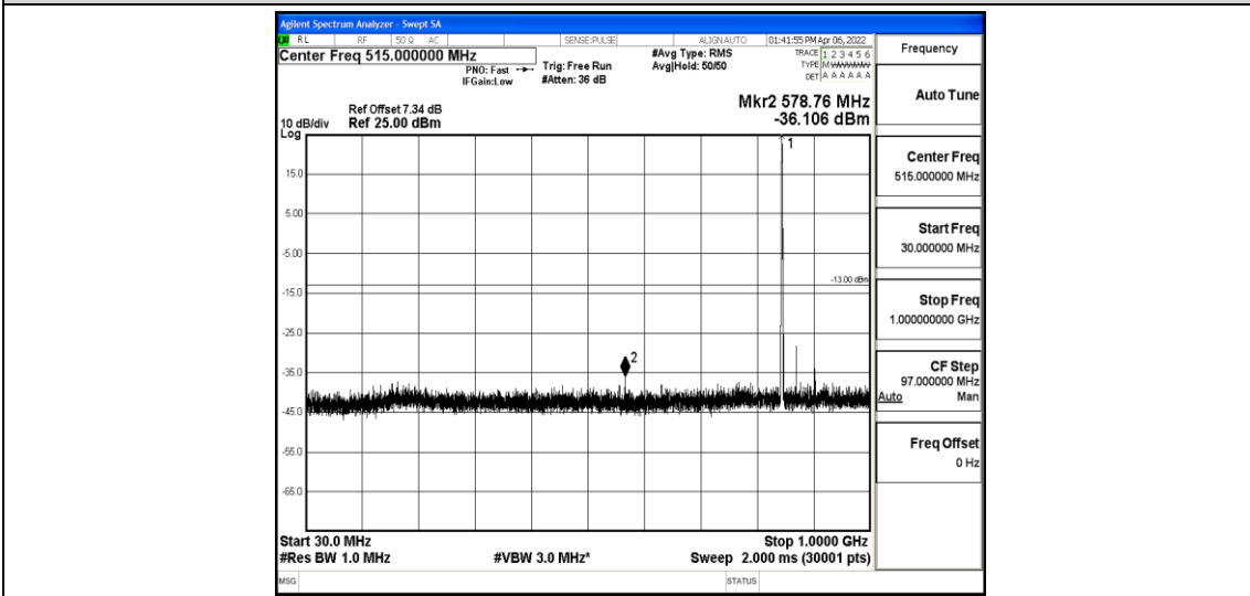
Band5-3MHz-16QAM-20635-1-0-High-30-1000--36.11-PASS
