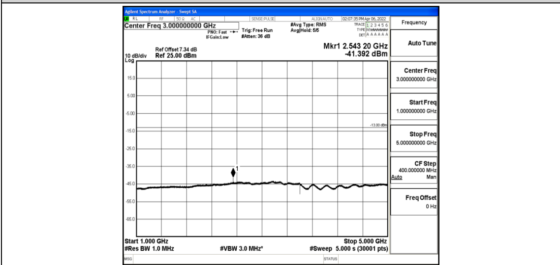
Band5-5MHz-16QAM-20625-1-0-High-1000-5000--41.39-PASS
