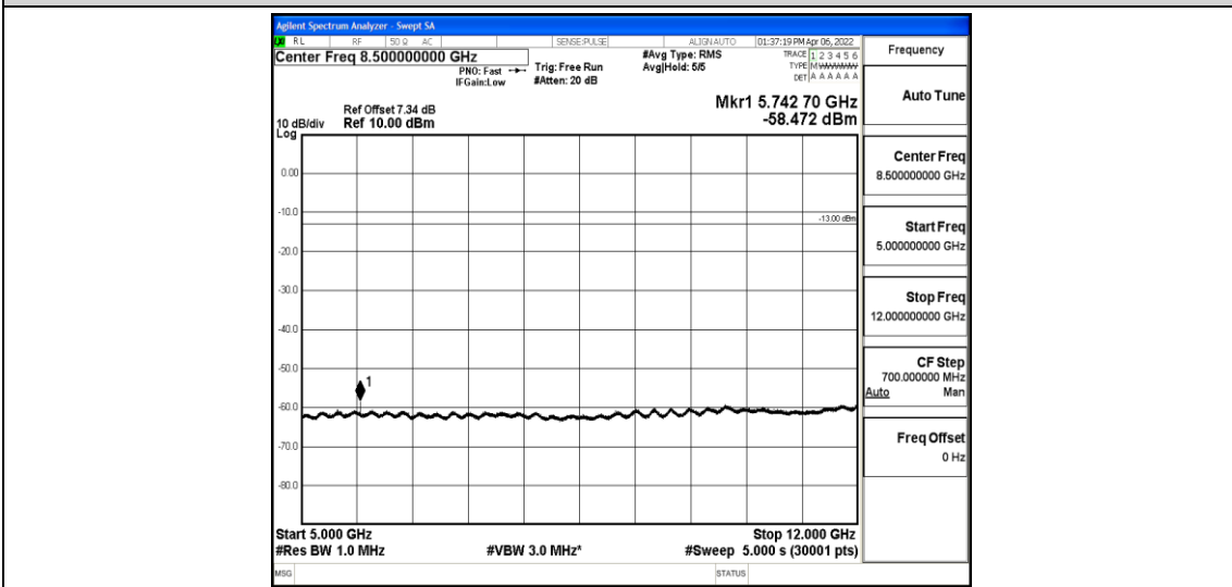
Band5-3MHz-QPSK-20525-1-0-Low-5000-12000--58.47-PASS
