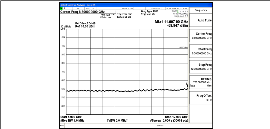
Band5-1.4MHz-QPSK-20643-1-0-High-5000-12000--58.95-PASS
