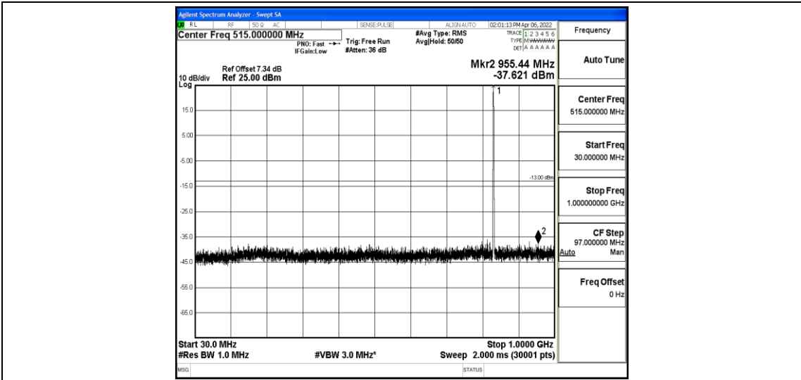
Band5-5MHz-QPSK-20525-1-0-Low-30-1000--37.62-PASS
