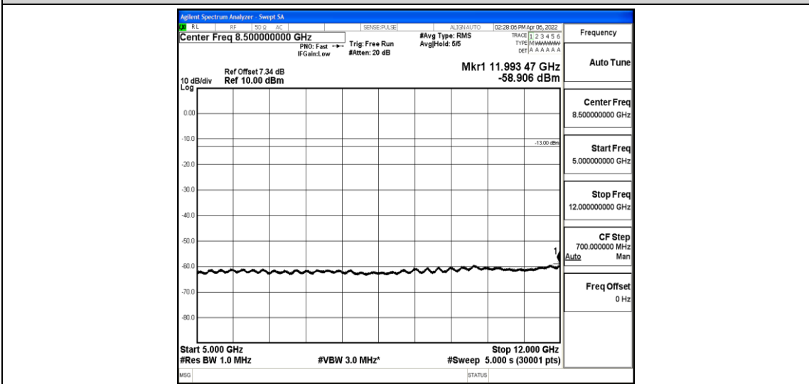
Band5-10MHz-QPSK-20525-1-0-Low-5000-12000--58.91-PASS
