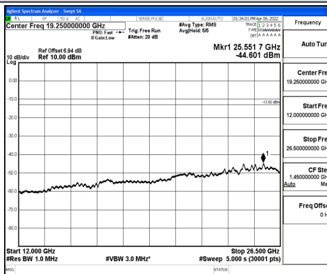
Band5-3MHz-QPSK-20415-1-0-Low-12000-26500--44.6-PASS
