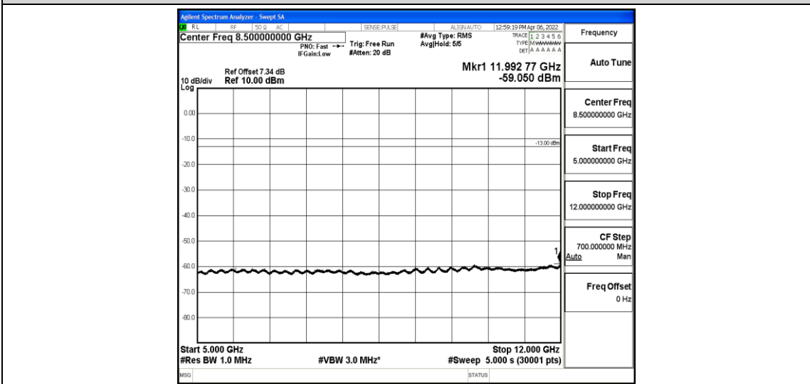
Band5-1.4MHz-16QAM-20525-1-0-Low-5000-12000--59.05-PASS
