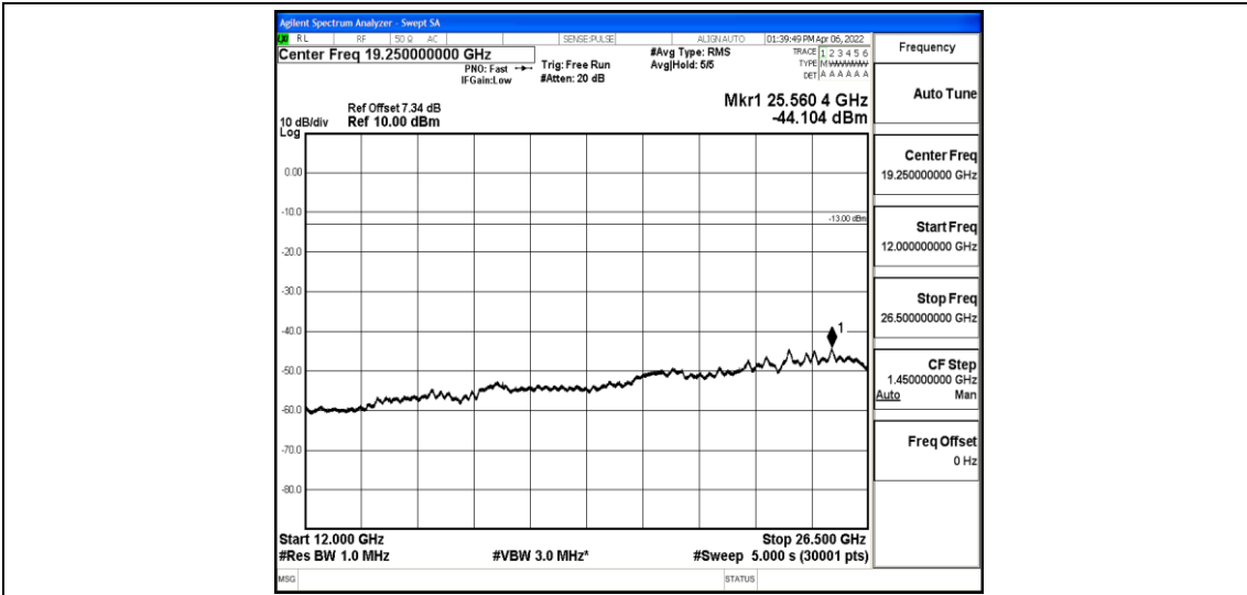
Band5-3MHz-16QAM-20525-1-0-Low-12000-26500--44.1-PASS
