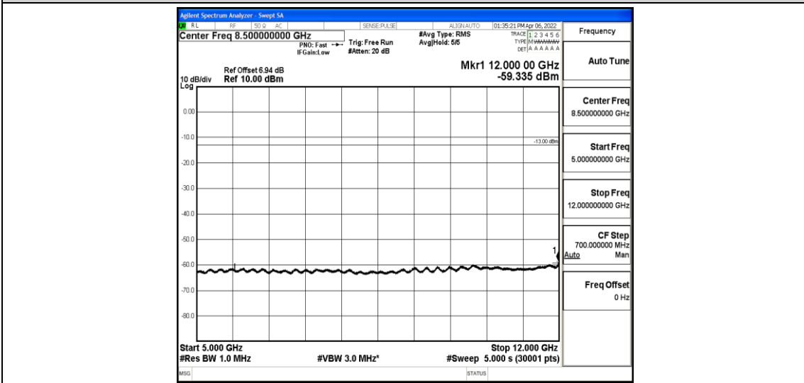
Band5-3MHz-16QAM-20415-1-0-Low-5000-12000--59.34-PASS
