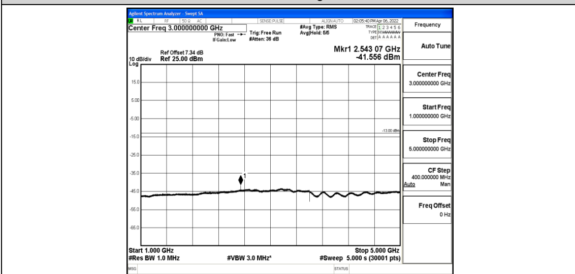
Band5-5MHz-QPSK-20625-1-0-High-1000-5000--41.56-PASS
