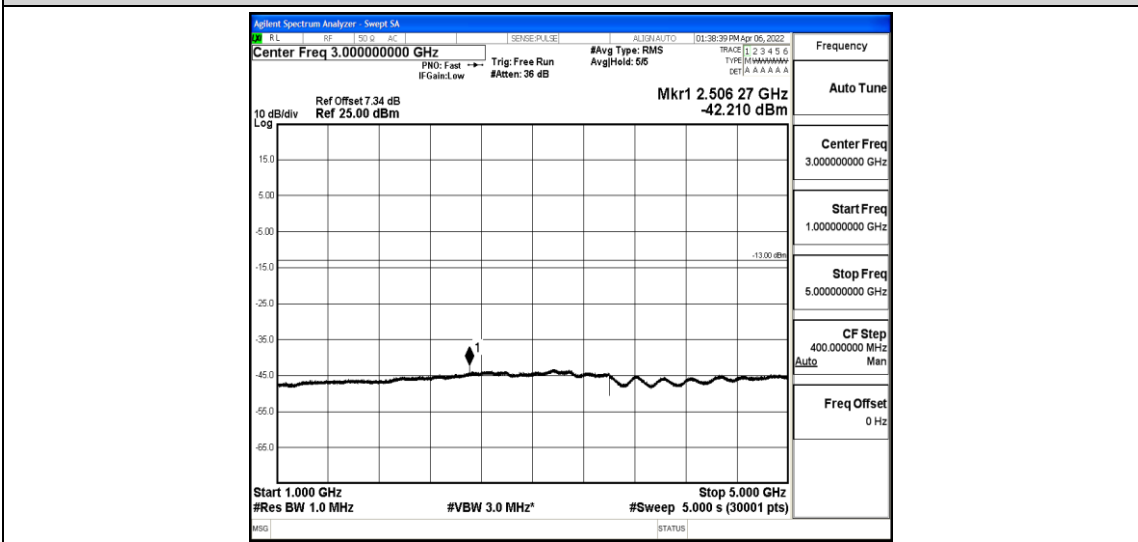
Band5-3MHz-16QAM-20525-1-0-Low-1000-5000--42.21-PASS
