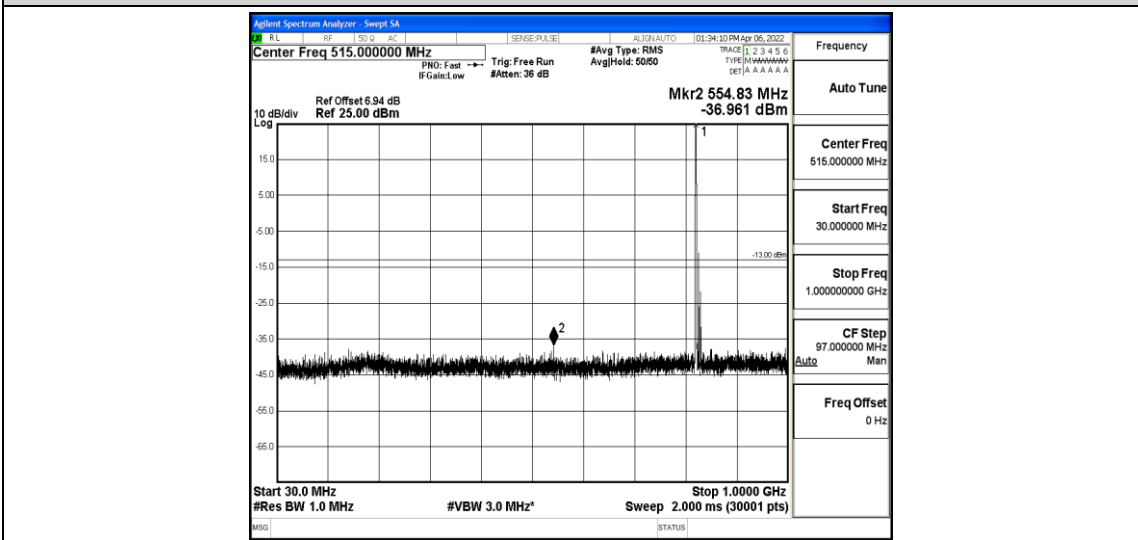
Band5-3MHz-16QAM-20415-1-0-Low-30-1000--36.96-PASS
