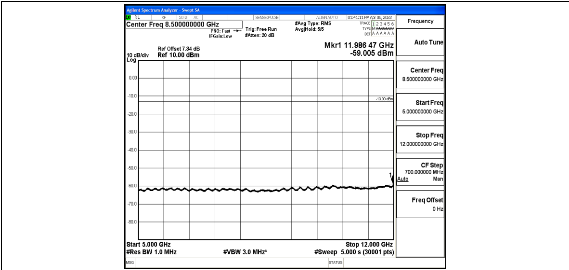
Band5-3MHz-QPSK-20635-1-0-High-5000-12000--59.01-PASS
