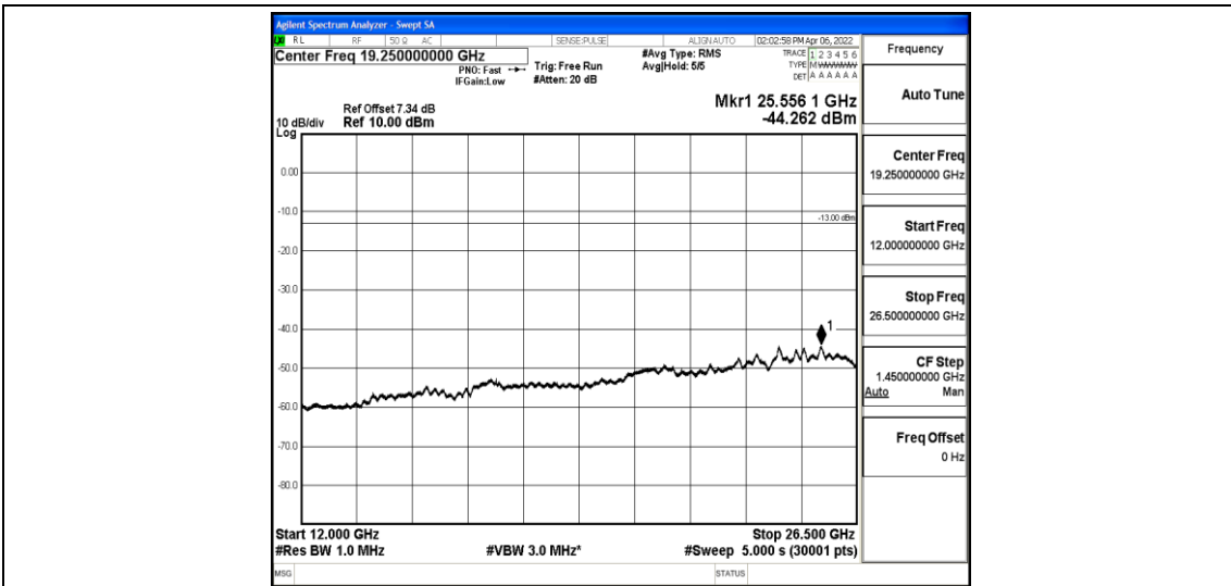
Band5-5MHz-QPSK-20525-1-0-Low-12000-26500--44.26-PASS
