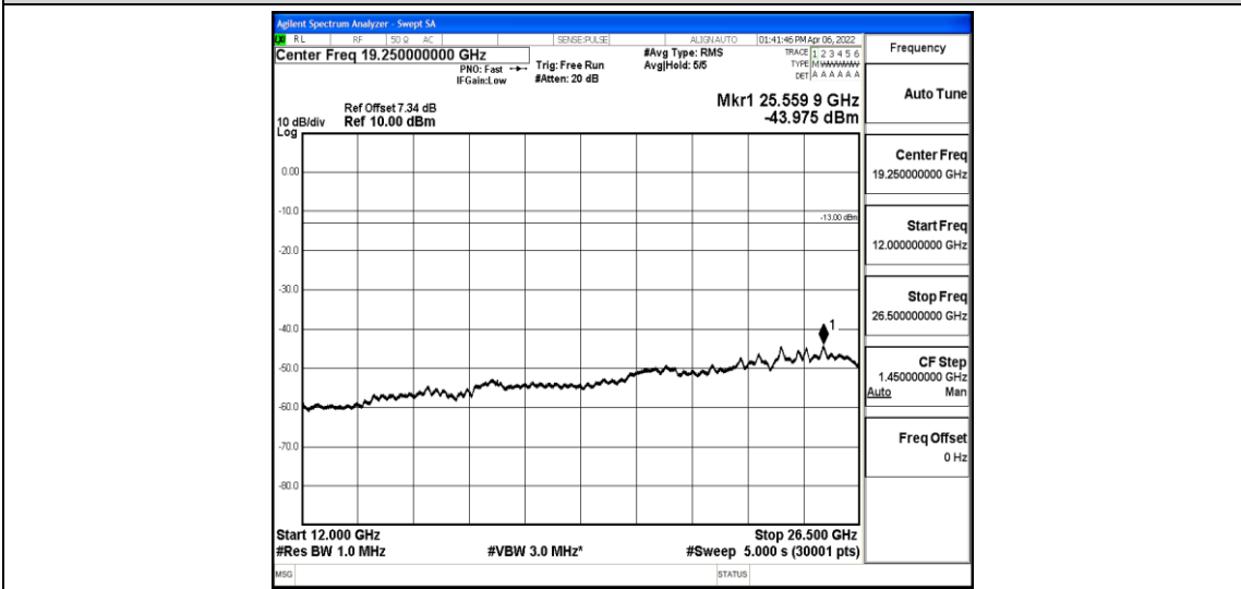
Band5-3MHz-QPSK-20635-1-0-High-12000-26500--43.98-PASS
