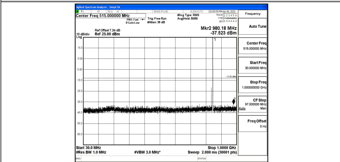
Band5-5MHz-QPSK-20625-1-0-High-30-1000--37.52-PASS
