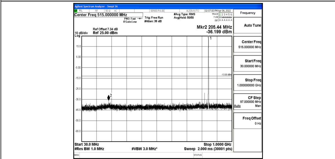
Band5-5MHz-16QAM-20625-1-0-High-30-1000--36.2-PASS
