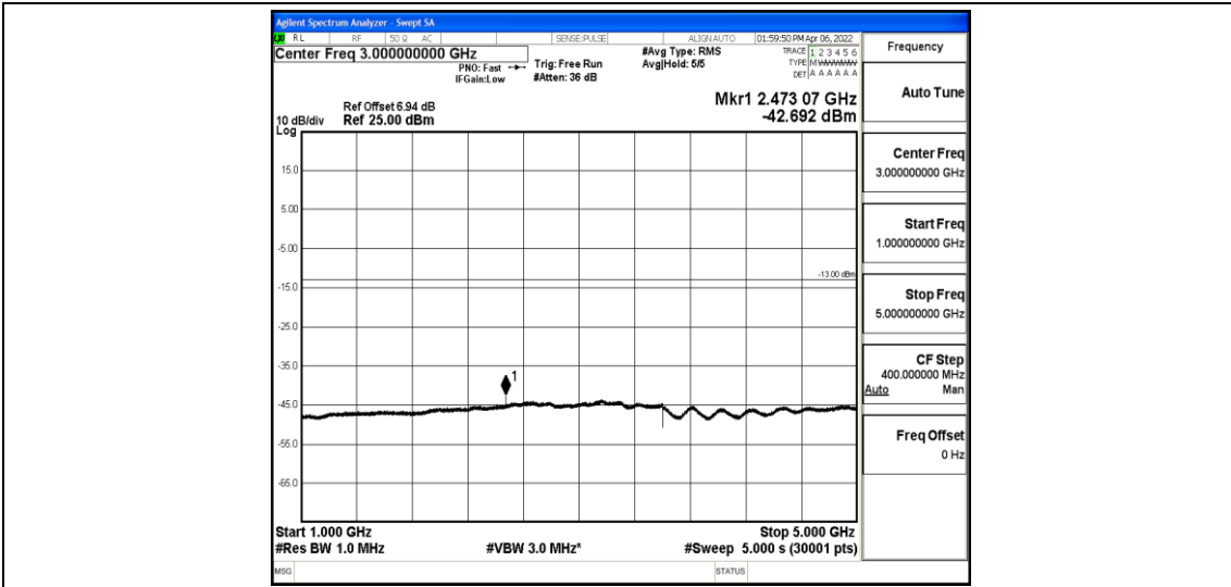
Band5-5MHz-16QAM-20425-1-0-Low-1000-5000--42.69-PASS
