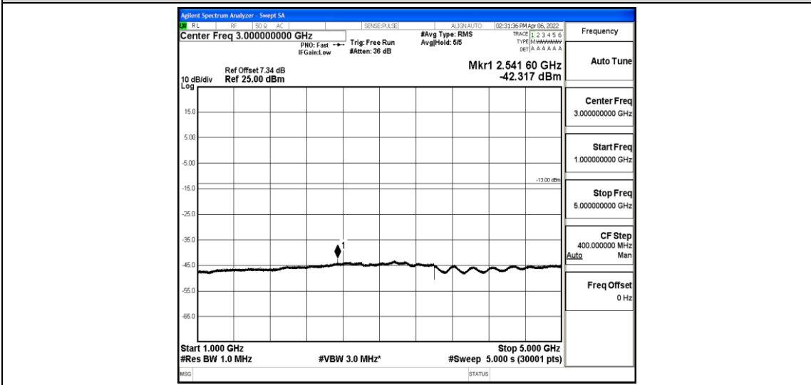
Band5-10MHz-QPSK-20600-1-0-High-1000-5000--42.32-PASS
