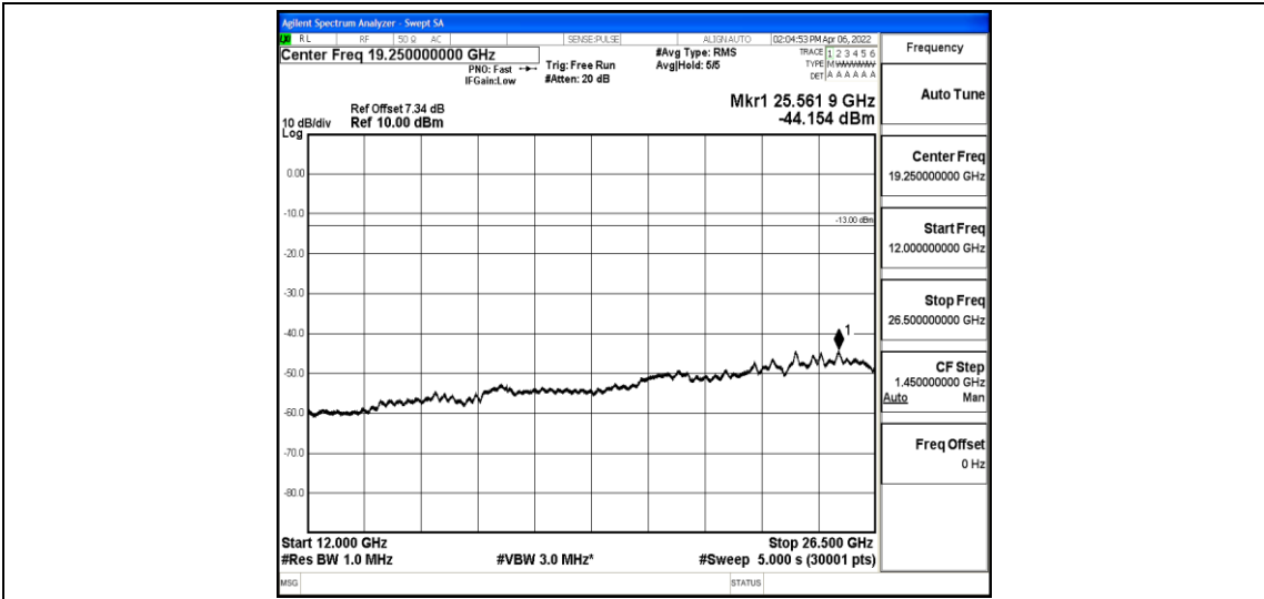
Band5-5MHz-16QAM-20525-1-0-Low-12000-26500--44.15-PASS
