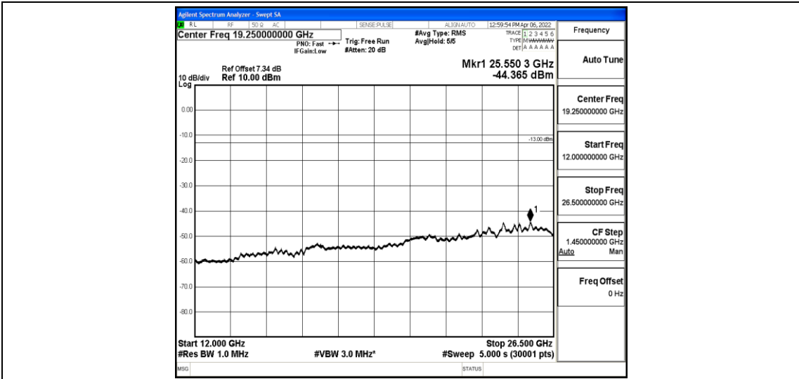
Band5-1.4MHz-16QAM-20525-1-0-Low-12000-26500--44.37-PASS
