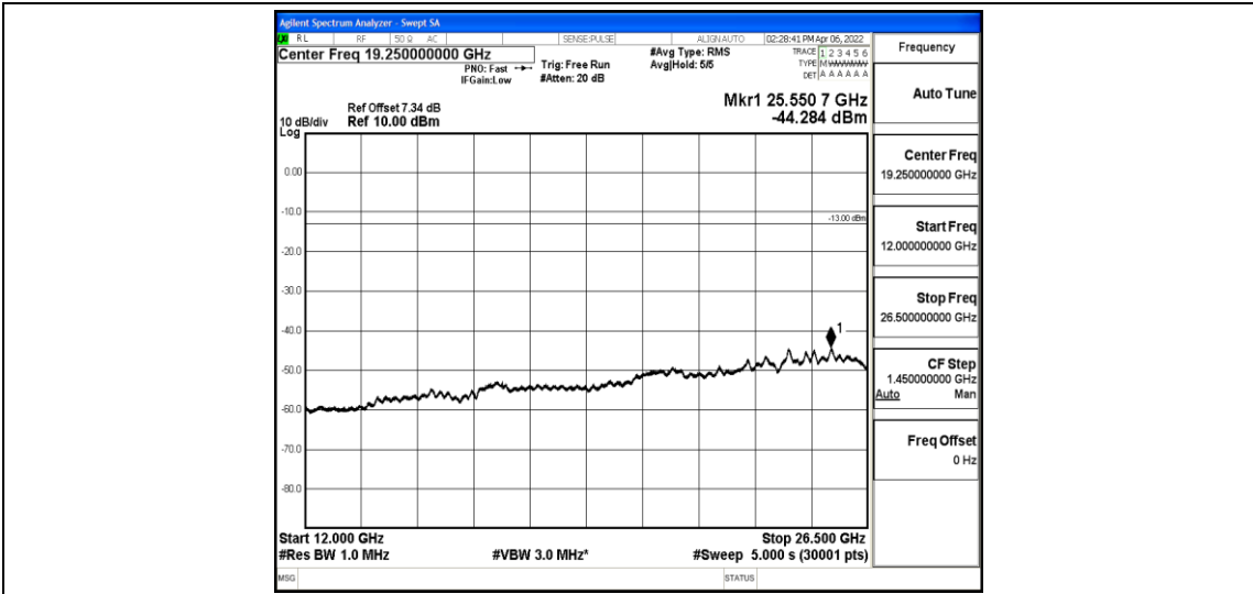
Band5-10MHz-QPSK-20525-1-0-Low-12000-26500--44.28-PASS
