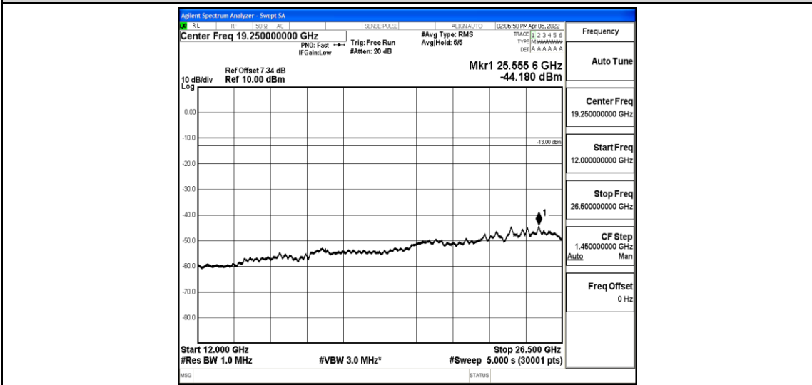
Band5-5MHz-QPSK-20625-1-0-High-12000-26500--44.18-PASS
