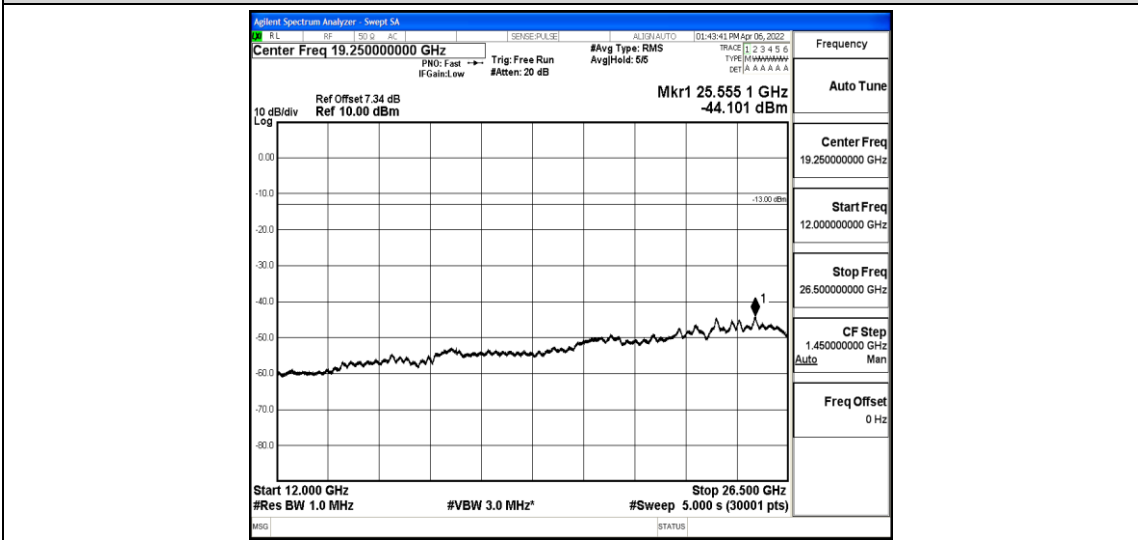
Band5-3MHz-16QAM-20635-1-0-High-12000-26500--44.1-PASS
