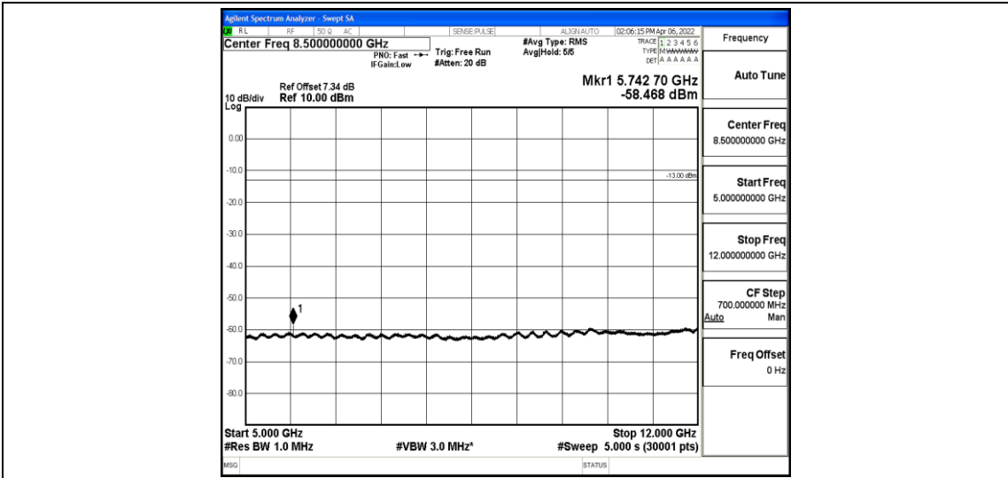
Band5-5MHz-QPSK-20625-1-0-High-5000-12000--58.47-PASS
