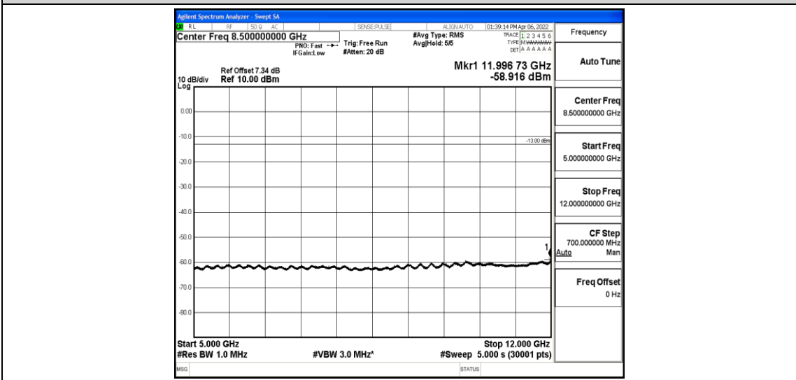
Band5-3MHz-16QAM-20525-1-0-Low-5000-12000--58.92-PASS
