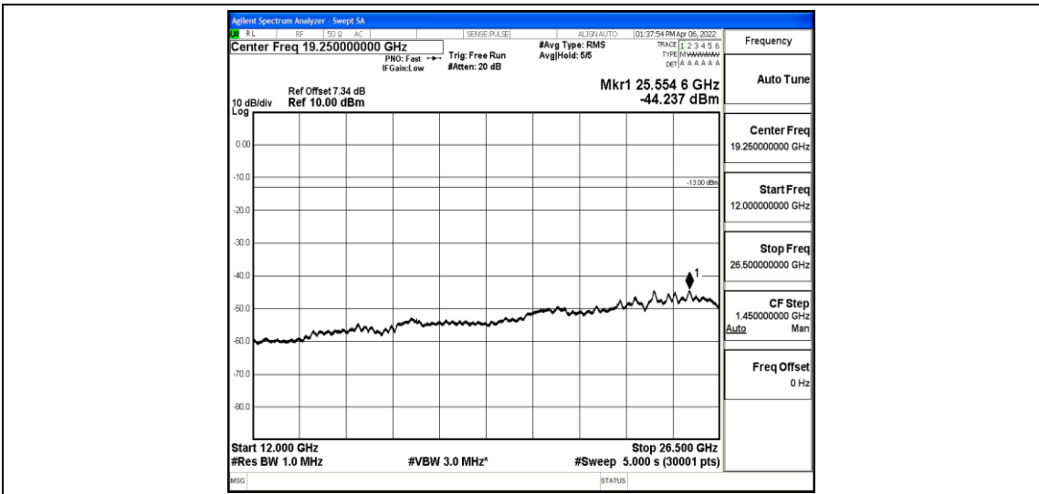
Band5-3MHz-QPSK-20525-1-0-Low-12000-26500--44.24-PASS
