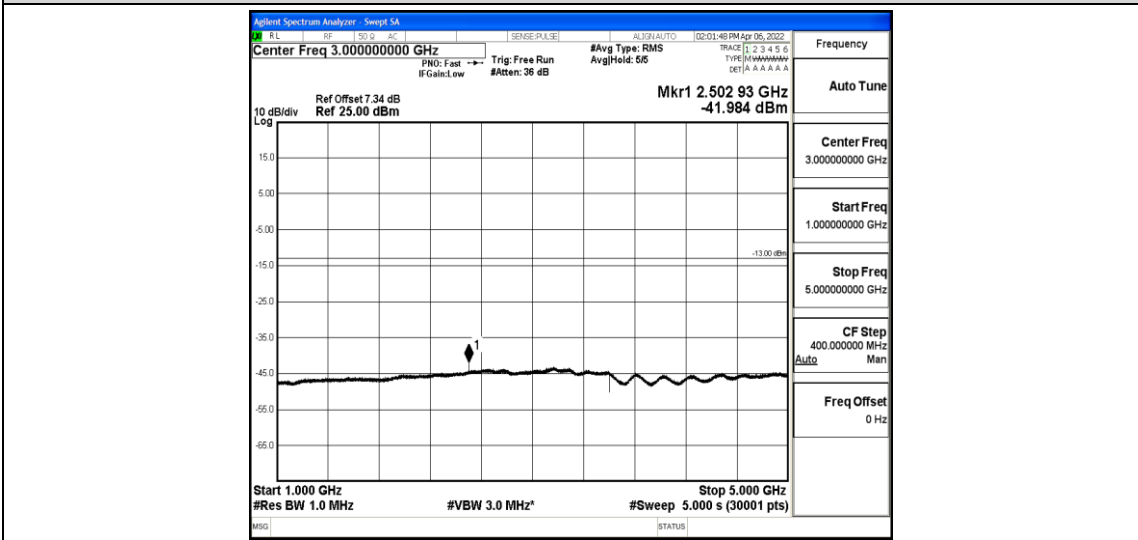
Band5-5MHz-QPSK-20525-1-0-Low-1000-5000--41.98-PASS
