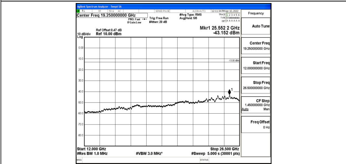
Band4-20MHz-QPSK-20300-1-0-High-12000-26500--43.15-PASS
