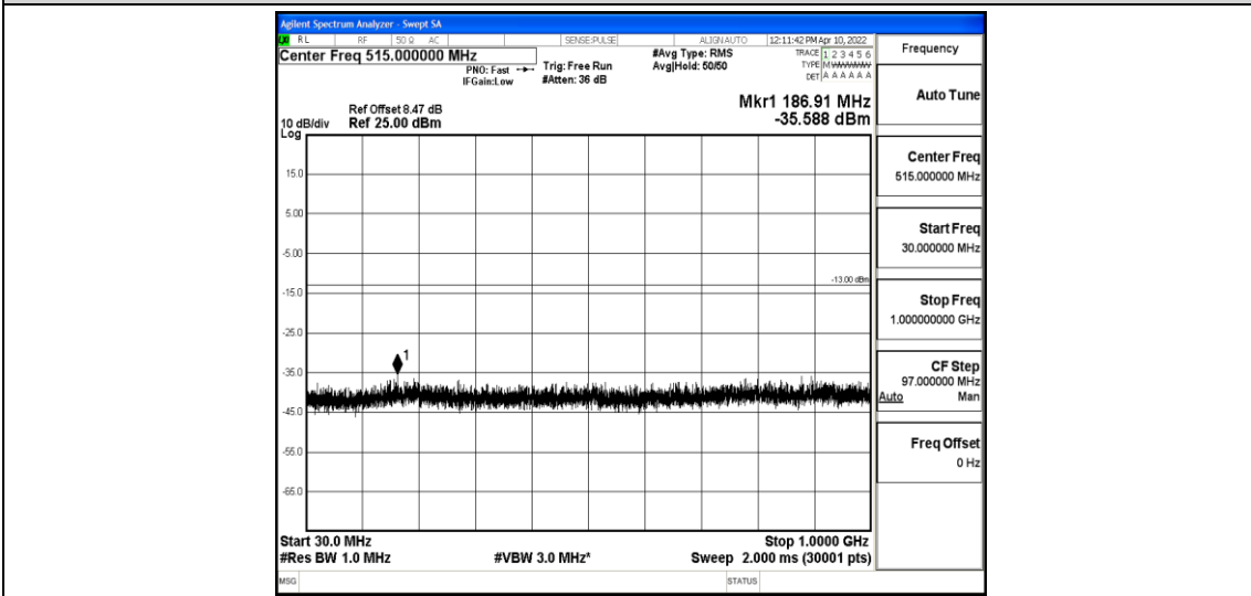
Band4-20MHz-16QAM-20300-1-0-High-30-1000--35.59-PASS
