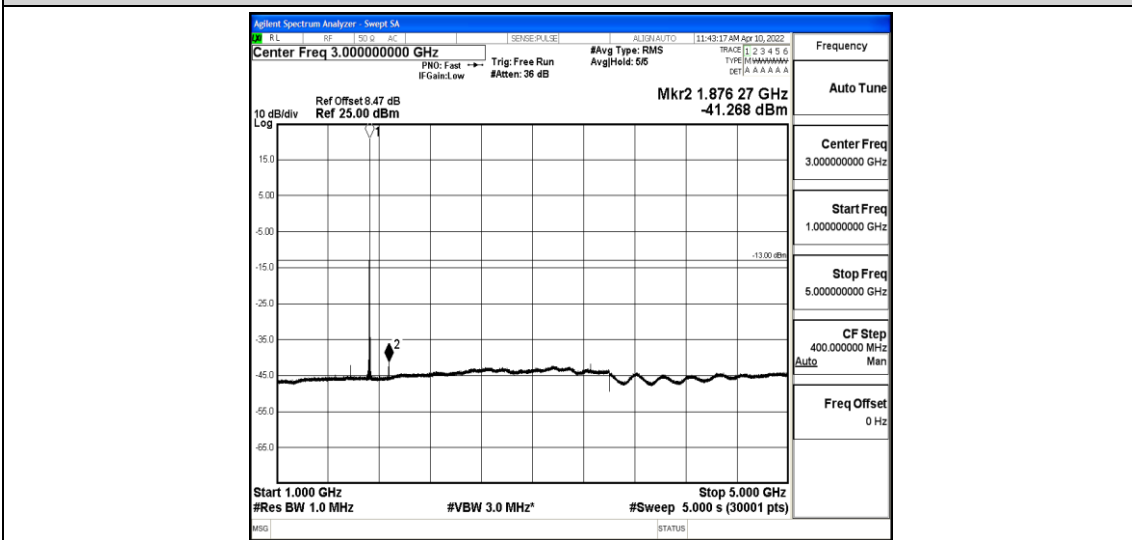
Band4-15MHz-QPSK-20175-1-0-Low-1000-5000--41.27-PASS
