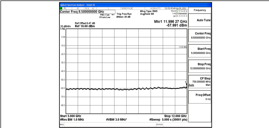
Band4-10MHz-QPSK-20350-1-0-High-5000-12000--57.99-PASS
