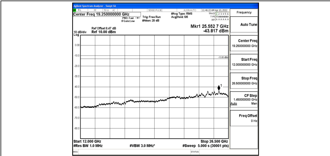
Band4-15MHz-16QAM-20175-1-0-Low-12000-26500--43.82-PASS
