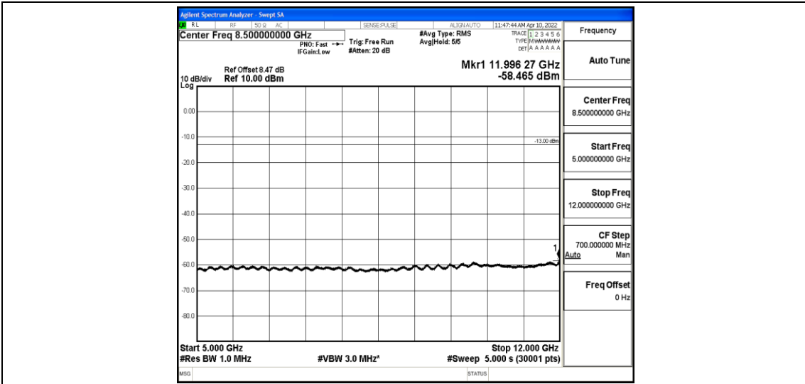
Band4-15MHz-QPSK-20325-1-0-High-5000-12000--58.47-PASS
