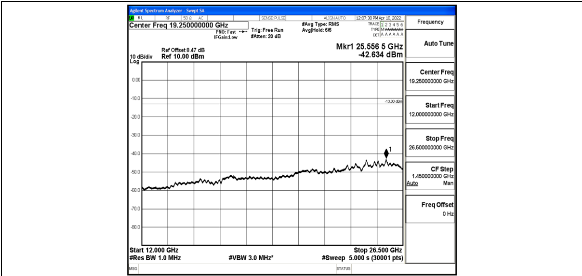
Band4-20MHz-QPSK-20175-1-0-Low-12000-26500--42.63-PASS
