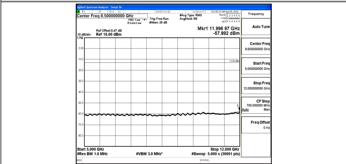
Band4-10MHz-16QAM-20175-1-0-Low-5000-12000--57.89-PASS
