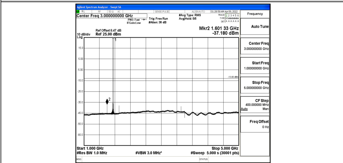
Band4-5MHz-QPSK-20375-1-0-High-1000-5000--37.18-PASS
