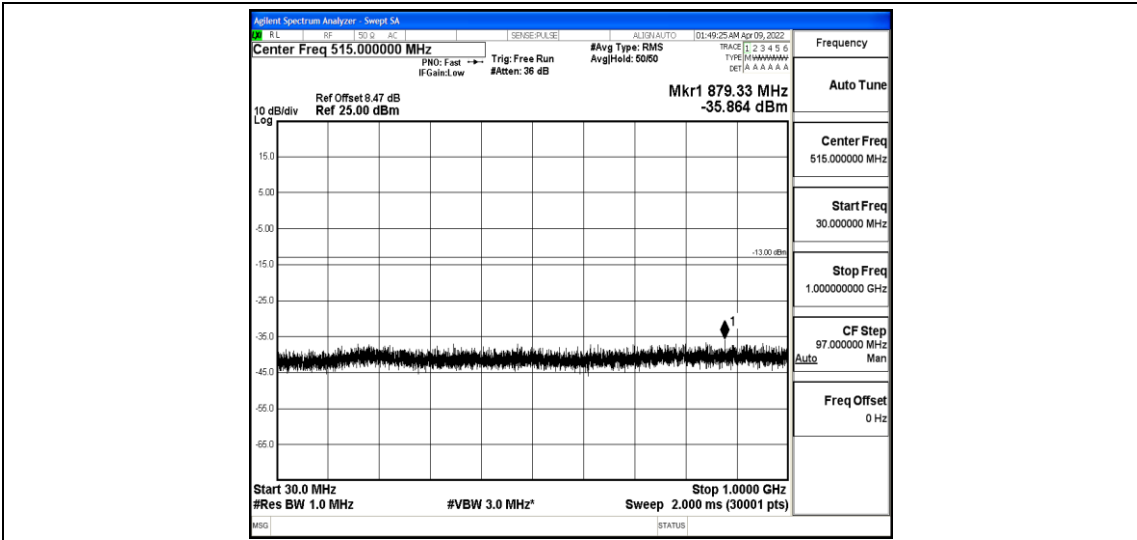
Band4-10MHz-16QAM-20175-1-0-Low-30-1000--35.86-PASS
