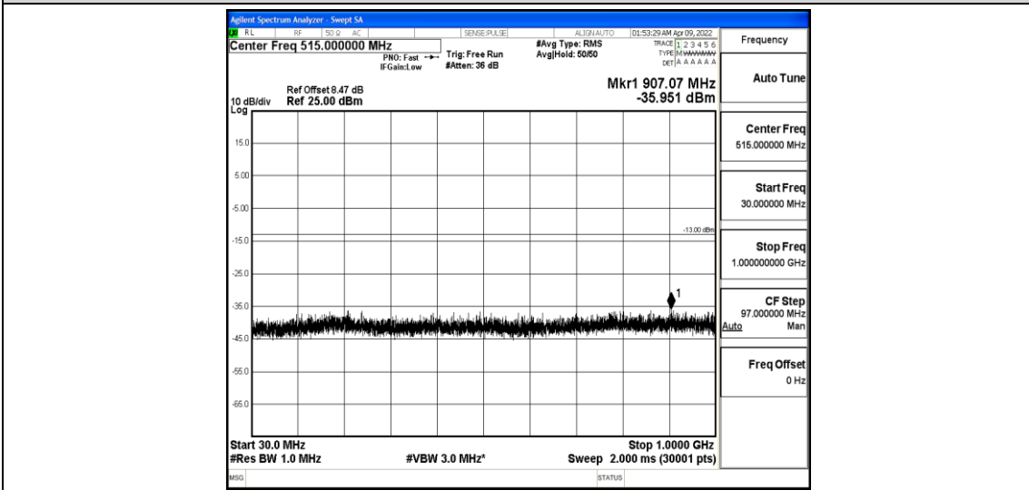
Band4-10MHz-16QAM-20350-1-0-High-30-1000--35.95-PASS
