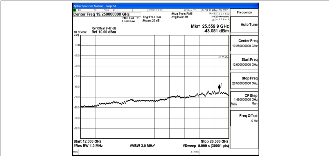
Band4-10MHz-16QAM-20175-1-0-Low-12000-26500--43.08-PASS
