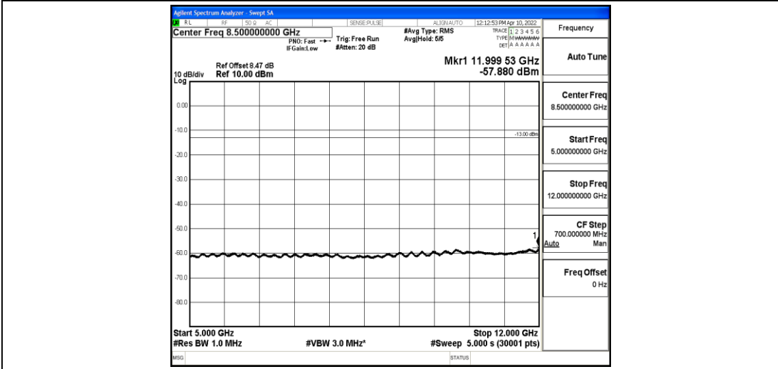
Band4-20MHz-16QAM-20300-1-0-High-5000-12000--57.88-PASS
