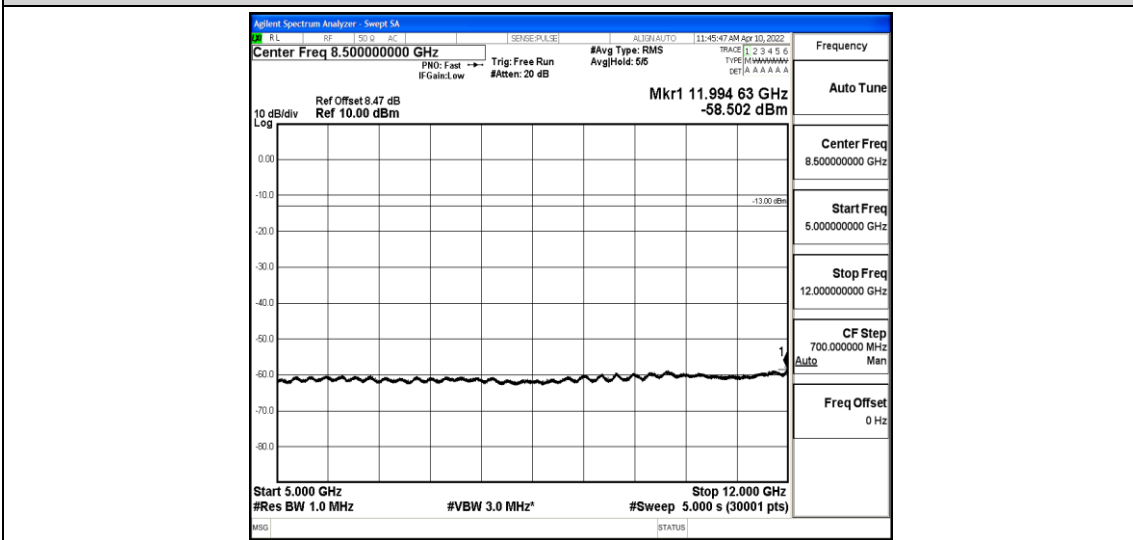
Band4-15MHz-16QAM-20175-1-0-Low-5000-12000--58.5-PASS
