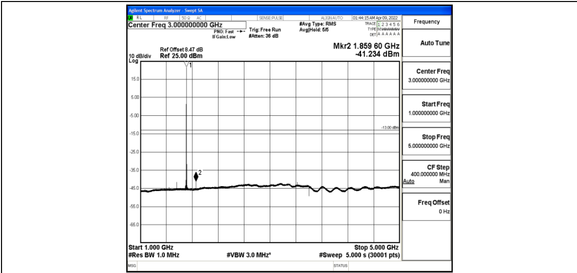
Band4-10MHz-QPSK-20000-1-0-Low-1000-5000--41.23-PASS
