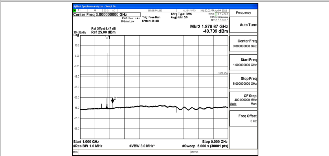
Band4-10MHz-16QAM-20175-1-0-Low-1000-5000--40.71-PASS
