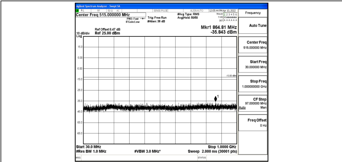
Band4-20MHz-QPSK-20175-1-0-Low-30-1000--35.84-PASS
