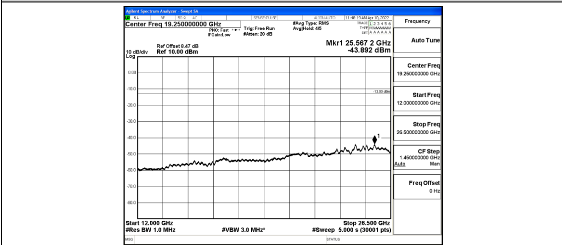
Band4-15MHz-QPSK-20325-1-0-High-12000-26500--43.89-PASS
