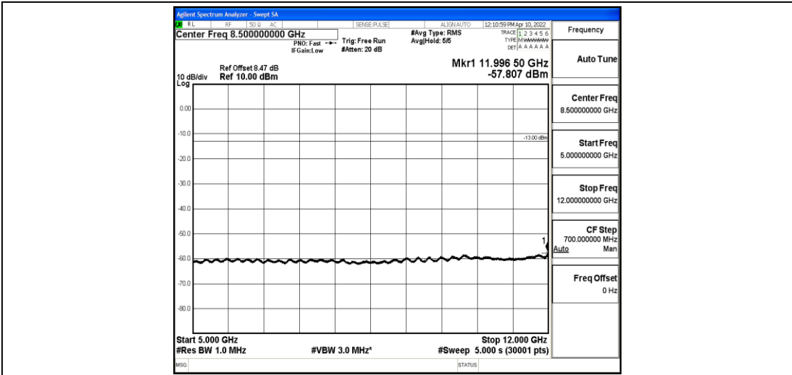
Band4-20MHz-QPSK-20300-1-0-High-5000-12000--57.81-PASS
