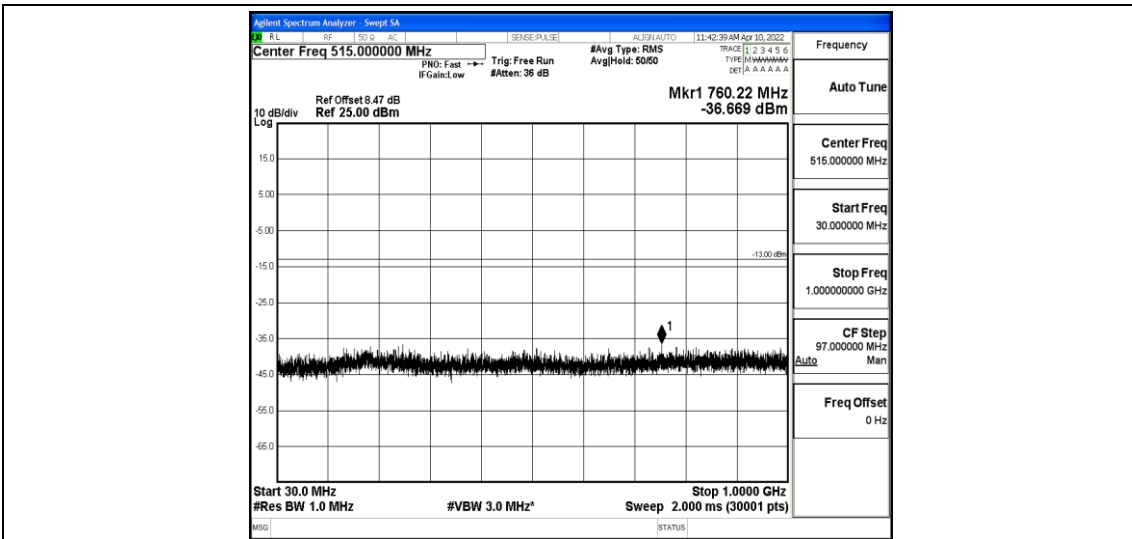
Band4-15MHz-QPSK-20175-1-0-Low-30-1000--36.67-PASS
