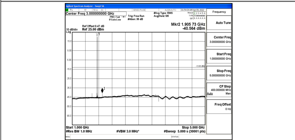
Band4-10MHz-16QAM-20350-1-0-High-1000-5000--40.56-PASS
