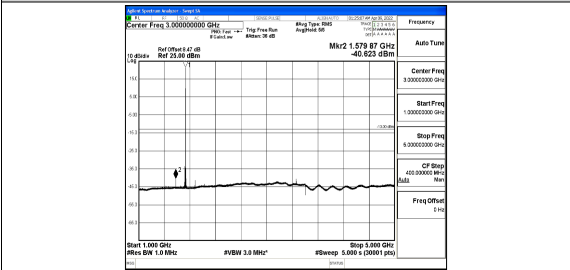
Band4-5MHz-QPSK-20175-1-0-Low-1000-5000--40.62-PASS
