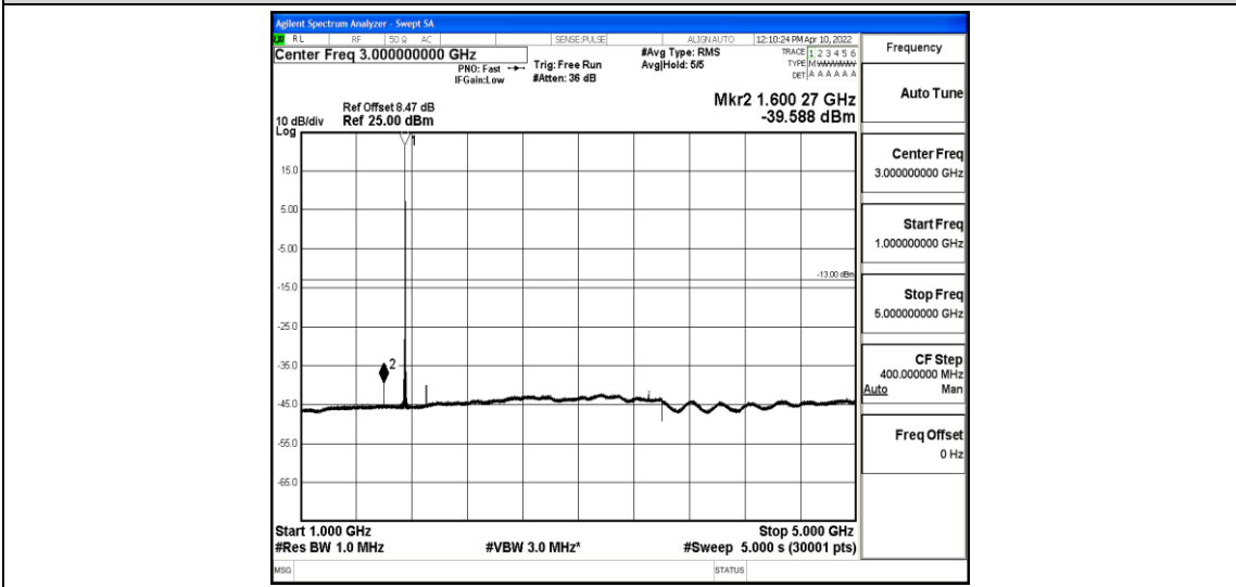
Band4-20MHz-QPSK-20300-1-0-High-1000-5000--39.59-PASS
