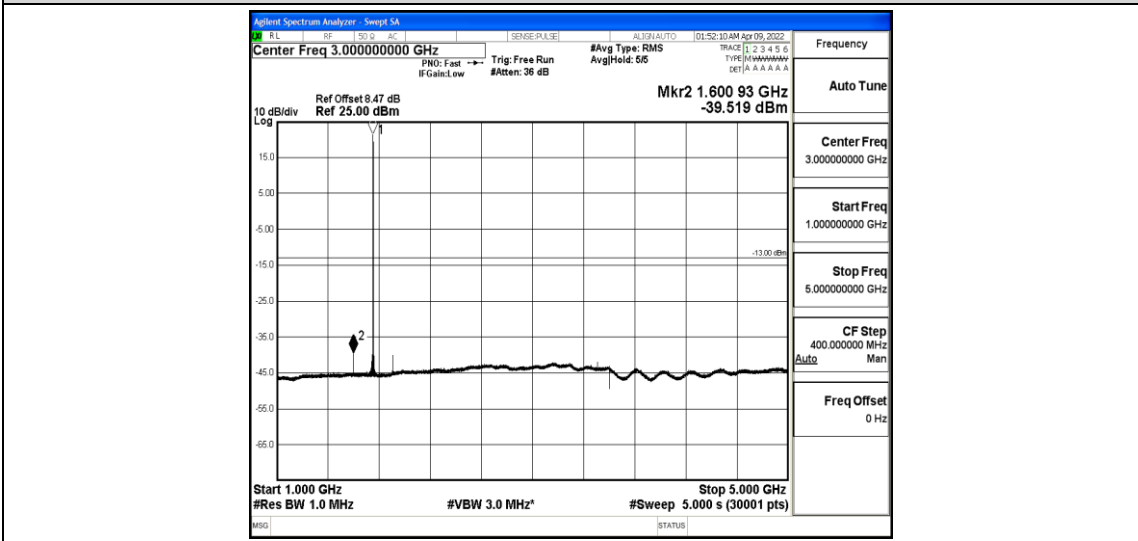
Band4-10MHz-QPSK-20350-1-0-High-1000-5000--39.52-PASS
