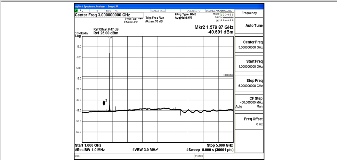
Band4-5MHz-16QAM-20175-1-0-Low-1000-5000--40.59-PASS
