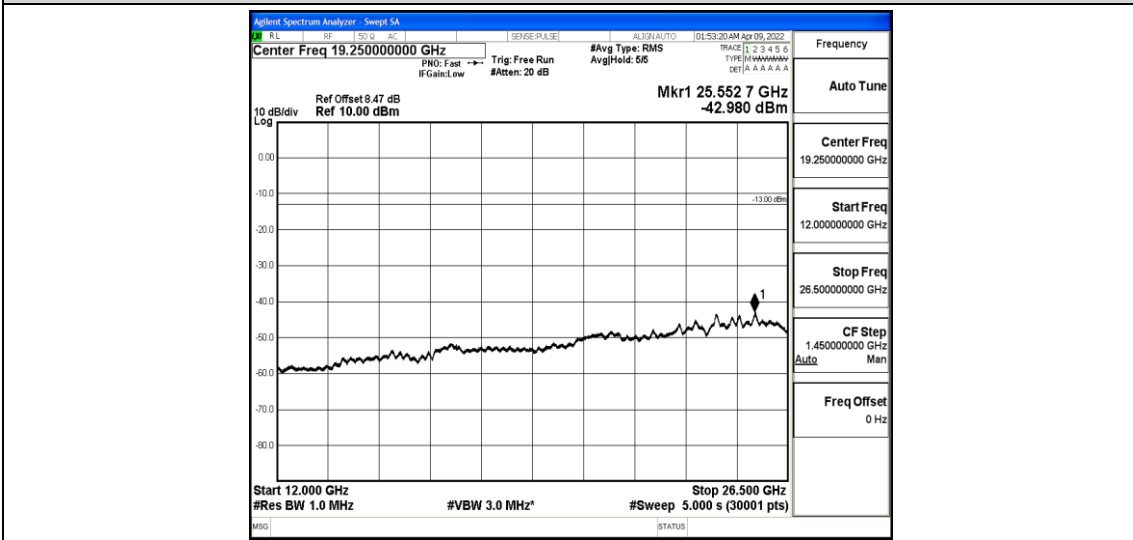
Band4-10MHz-QPSK-20350-1-0-High-12000-26500--42.98-PASS
