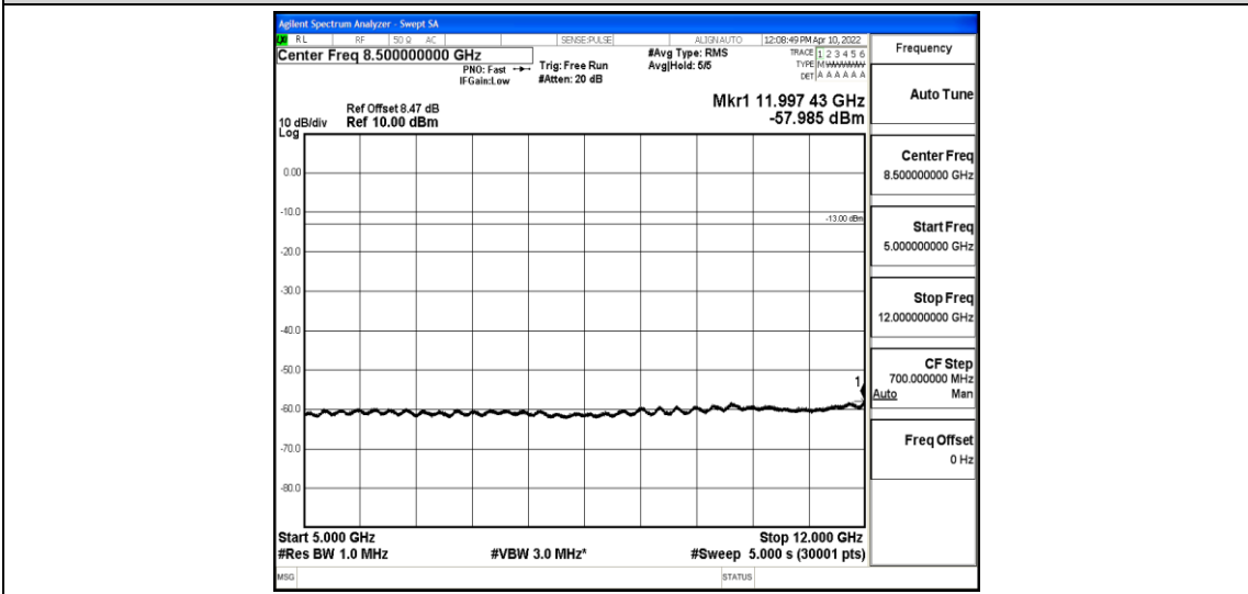
Band4-20MHz-16QAM-20175-1-0-Low-5000-12000--57.99-PASS
