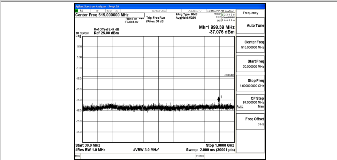
Band4-15MHz-QPSK-20325-1-0-High-30-1000--37.08-PASS
