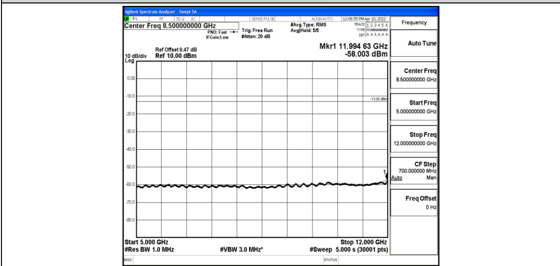
Band4-20MHz-QPSK-20175-1-0-Low-5000-12000--58-PASS
