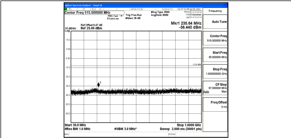
Band4-10MHz-QPSK-20175-1-0-Low-30-1000--36.44-PASS
