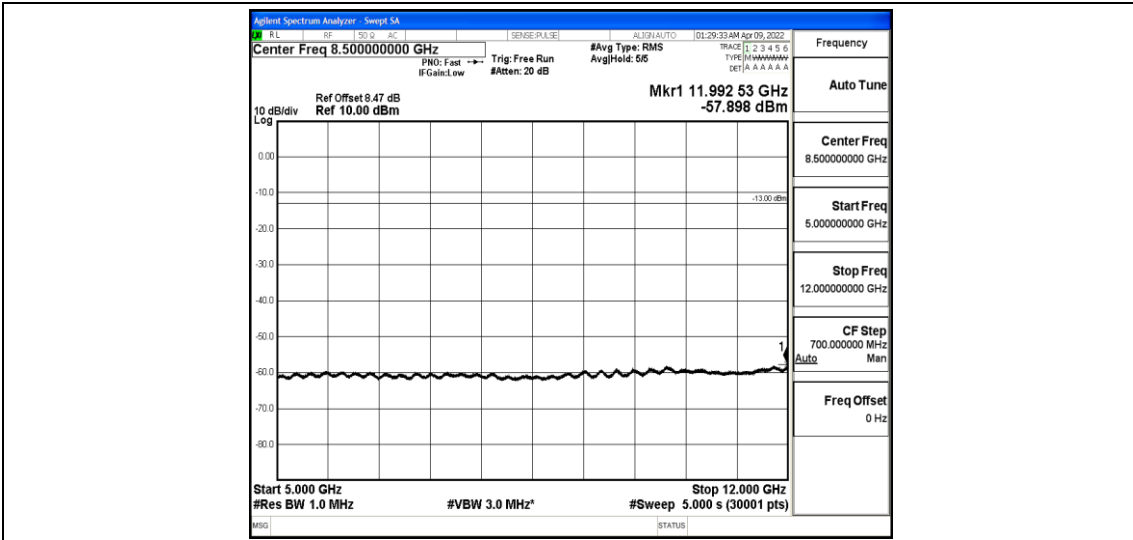
Band4-5MHz-QPSK-20375-1-0-High-5000-12000--57.9-PASS
