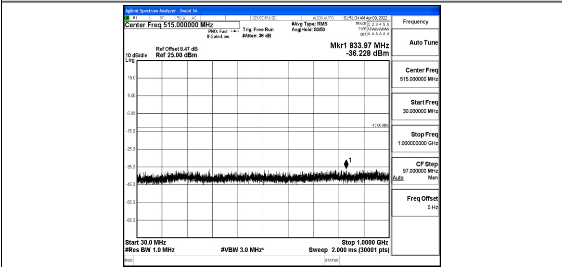
Band4-10MHz-QPSK-20350-1-0-High-30-1000--36.23-PASS
