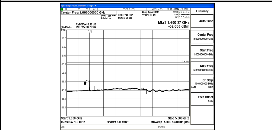
Band4-20MHz-16QAM-20300-1-0-High-1000-5000--39.64-PASS
