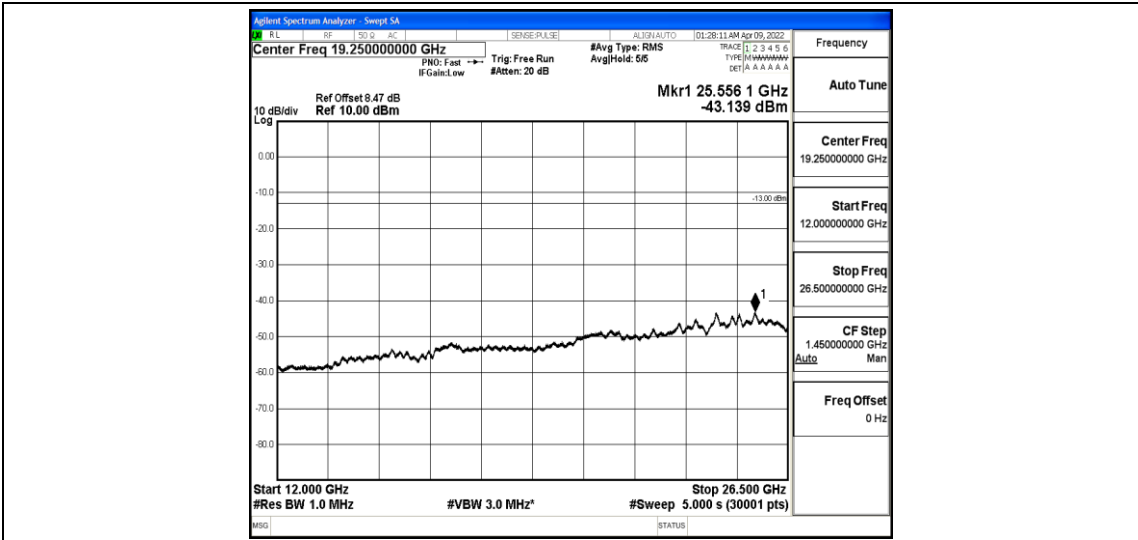
Band4-5MHz-16QAM-20175-1-0-Low-12000-26500--43.14-PASS
