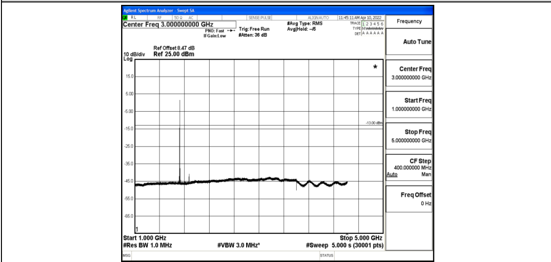
Band4-15MHz-16QAM-20175-1-0-Low-1000-5000--41.27-PASS
