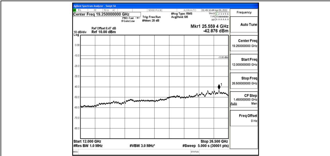
Band4-10MHz-QPSK-20175-1-0-Low-12000-26500--42.88-PASS
