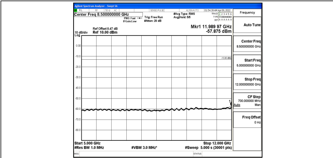
Band4-10MHz-16QAM-20350-1-0-High-5000-12000--57.88-PASS
