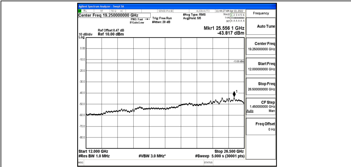
Band4-15MHz-QPSK-20175-1-0-Low-12000-26500--43.82-PASS
