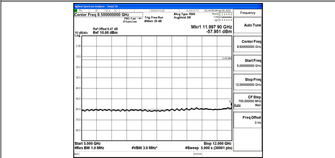
Band4-10MHz-QPSK-20000-1-0-Low-5000-12000--57.95-PASS
