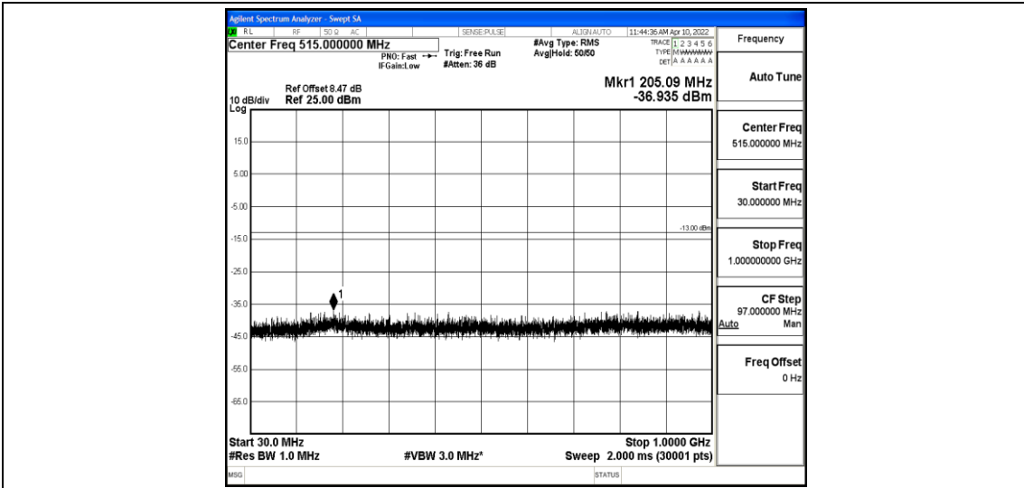
Band4-15MHz-16QAM-20175-1-0-Low-30-1000--36.94-PASS
