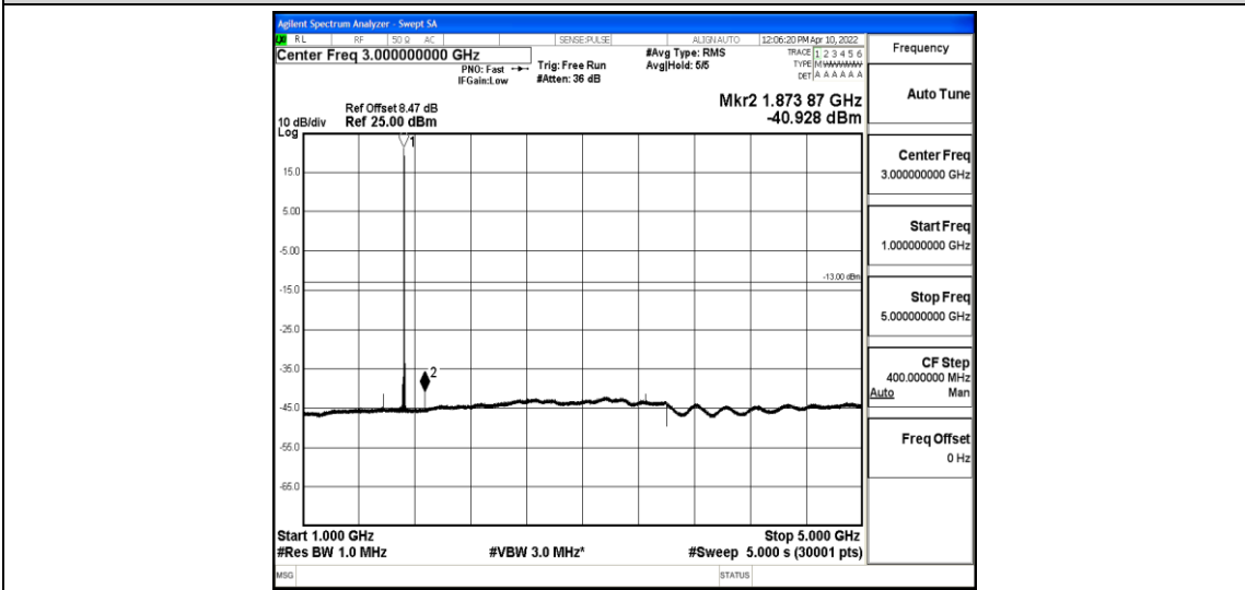
Band4-20MHz-QPSK-20175-1-0-Low-1000-5000--40.93-PASS
