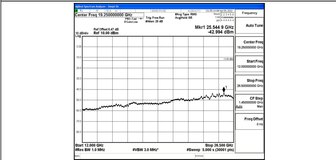
Band4-10MHz-16QAM-20350-1-0-High-12000-26500--42.99-PASS
