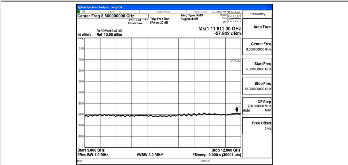
Band4-5MHz-QPSK-20175-1-0-Low-5000-12000--57.94-PASS
