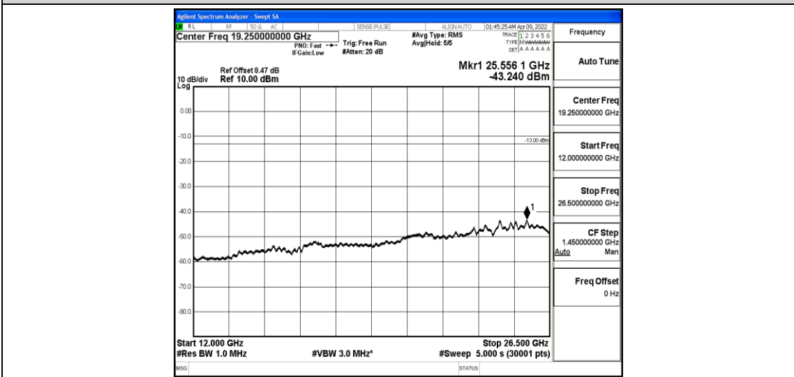
Band4-10MHz-QPSK-20000-1-0-Low-12000-26500--43.24-PASS
