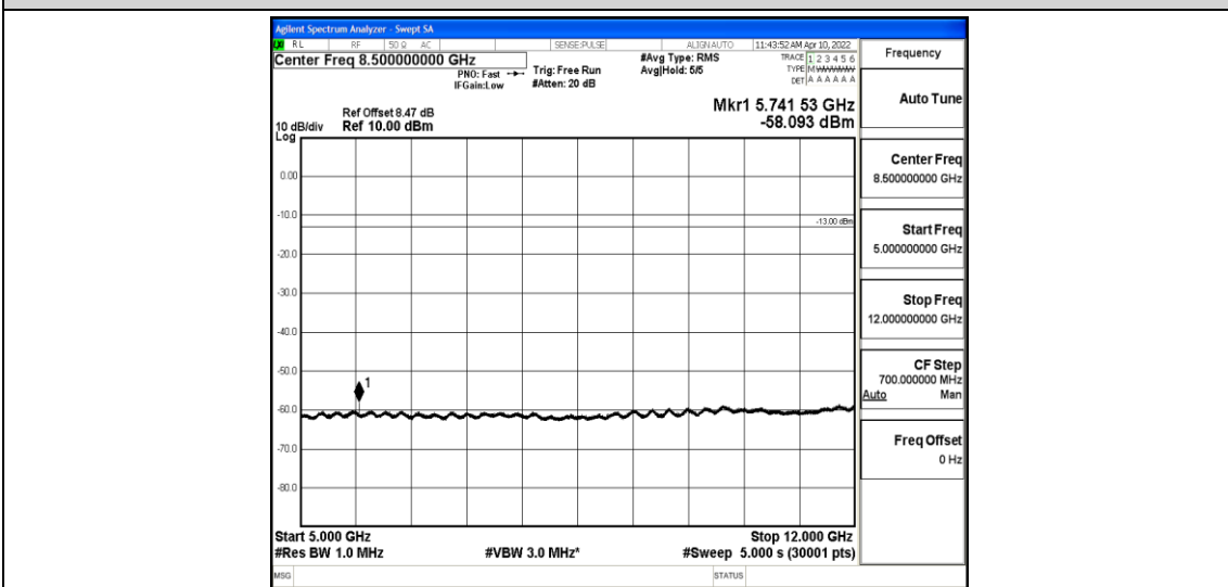
Band4-15MHz-QPSK-20175-1-0-Low-5000-12000--58.09-PASS
