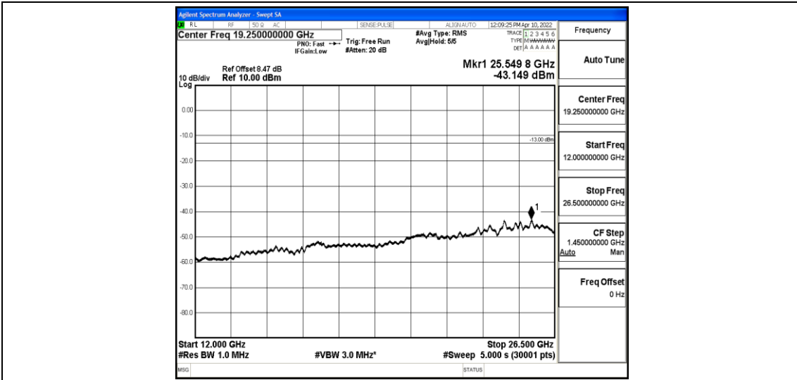
Band4-20MHz-16QAM-20175-1-0-Low-12000-26500--43.15-PASS
