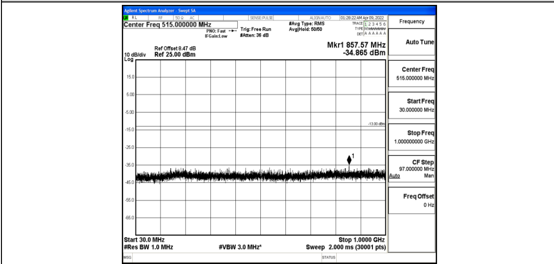
Band4-5MHz-QPSK-20375-1-0-High-30-1000--34.87-PASS
