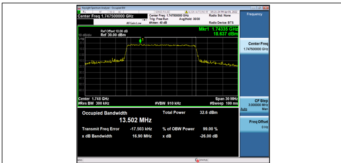
Band4-15MHz-16QAM-20325-75RB#0-13.502
