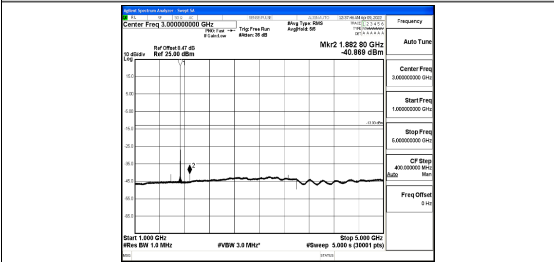
Band4-1.4MHz-QPSK-20175-1-0-Low-1000-5000--40.87-PASS
