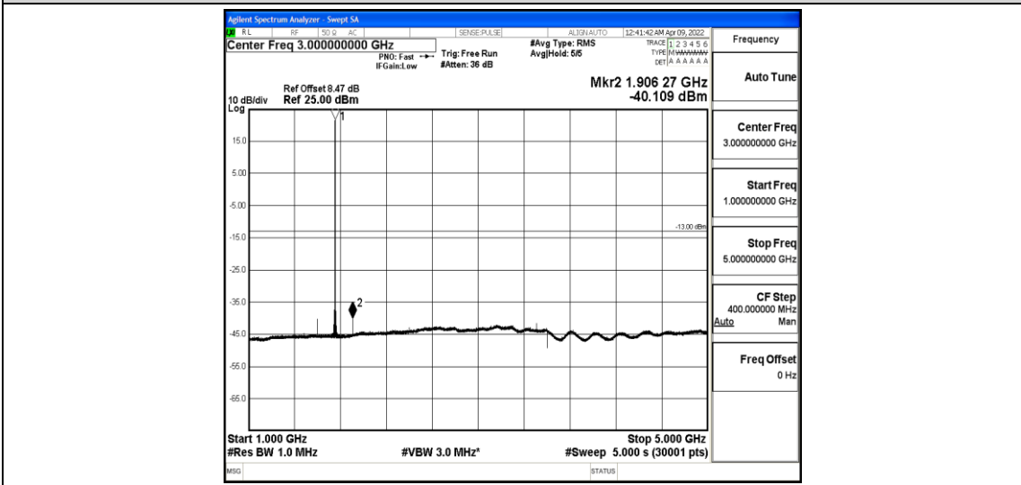
Band4-1.4MHz-QPSK-20393-1-0-High-1000-5000--40.11-PASS
