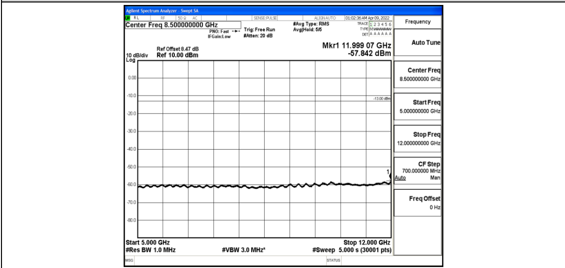
Band4-3MHz-QPSK-20175-1-0-Low-5000-12000--57.84-PASS
