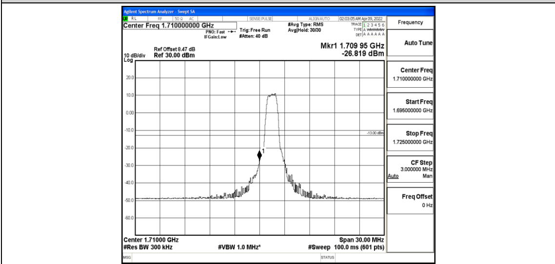
Band4-15MHz-QPSK-20025-6-0-Low--26.82-PASS
