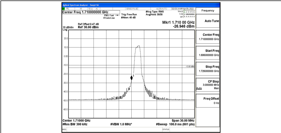
Band4-15MHz-16QAM-20025-6-0-Low--26.95-PASS
