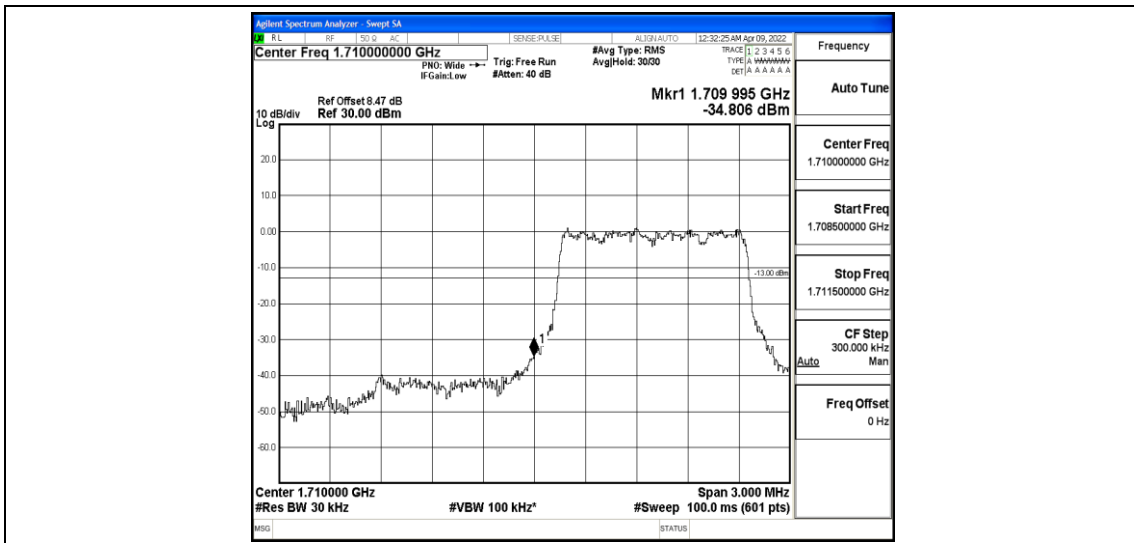
Band4-1.4MHz-QPSK-19957-6-0-Low--34.81-PASS
