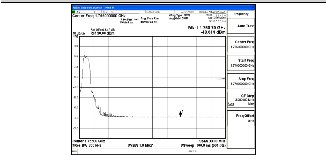
Band4-15MHz-QPSK-20325-6-0-Low--48.61-PASS
