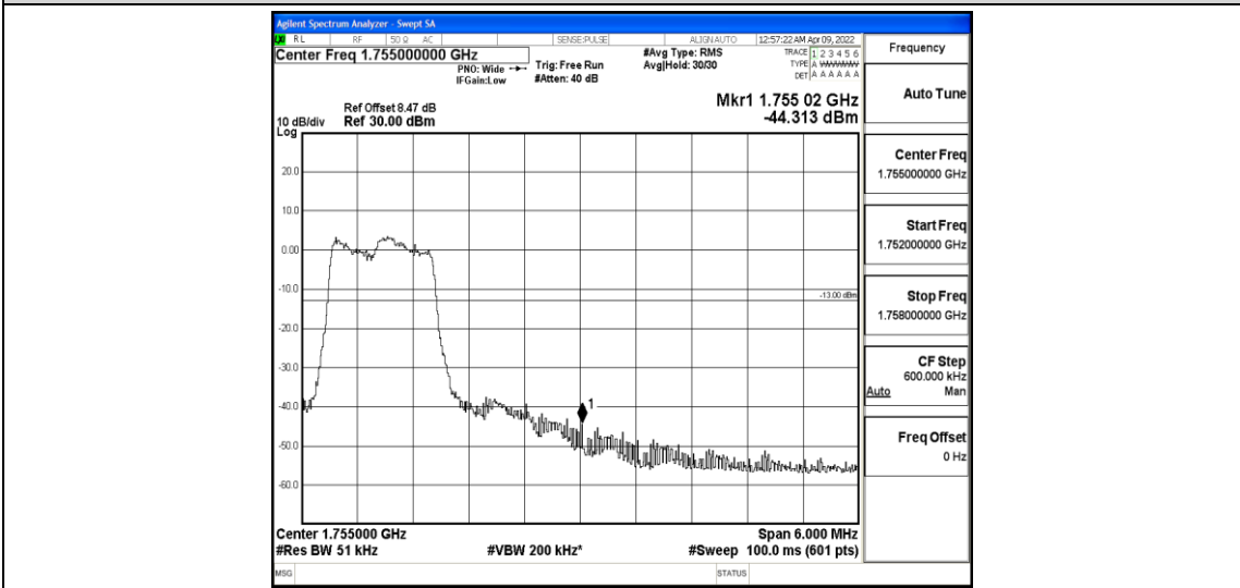
Band4-3MHz-16QAM-20385-6-0-Low--44.31-PASS
