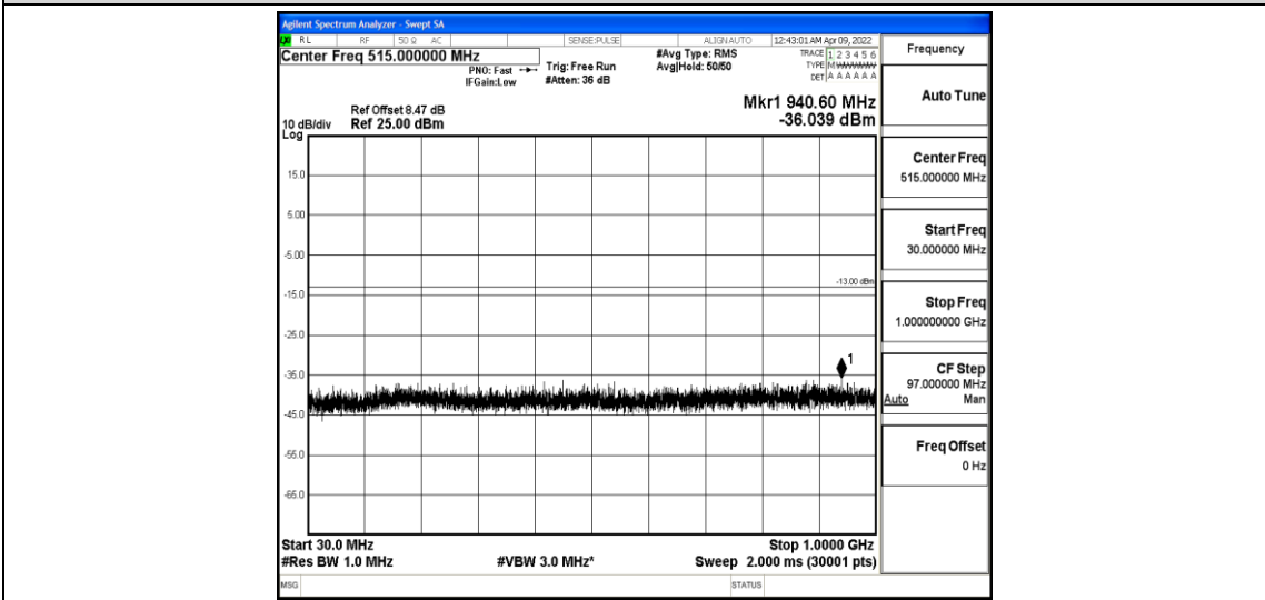
Band4-1.4MHz-16QAM-20393-1-0-High-30-1000--36.04-PASS
