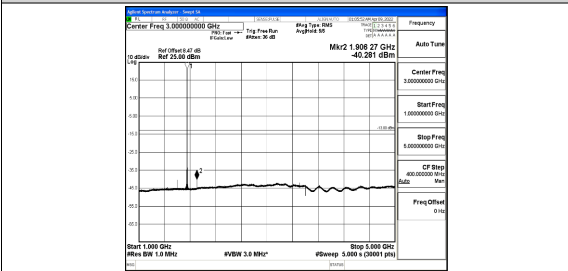
Band4-3MHz-QPSK-20385-1-0-High-1000-5000--40.28-PASS
