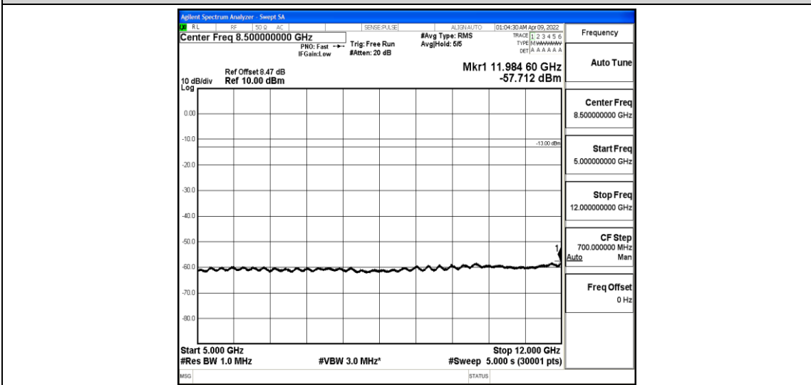
Band4-3MHz-16QAM-20175-1-0-Low-5000-12000--57.71-PASS
