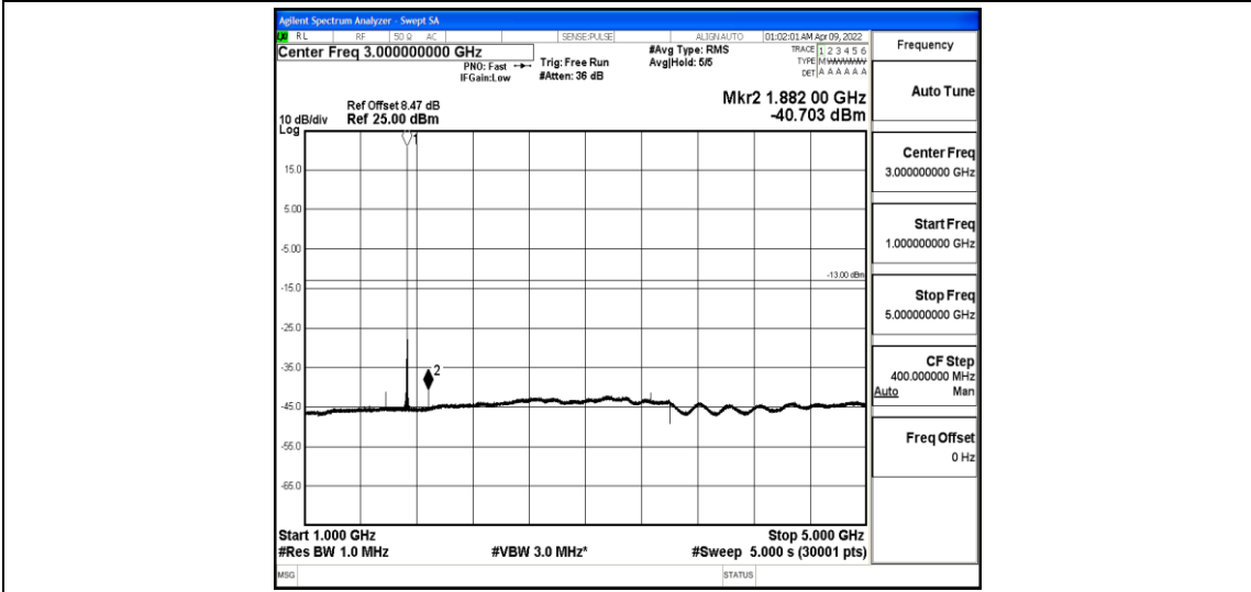
Band4-3MHz-QPSK-20175-1-0-Low-1000-5000--40.7-PASS
