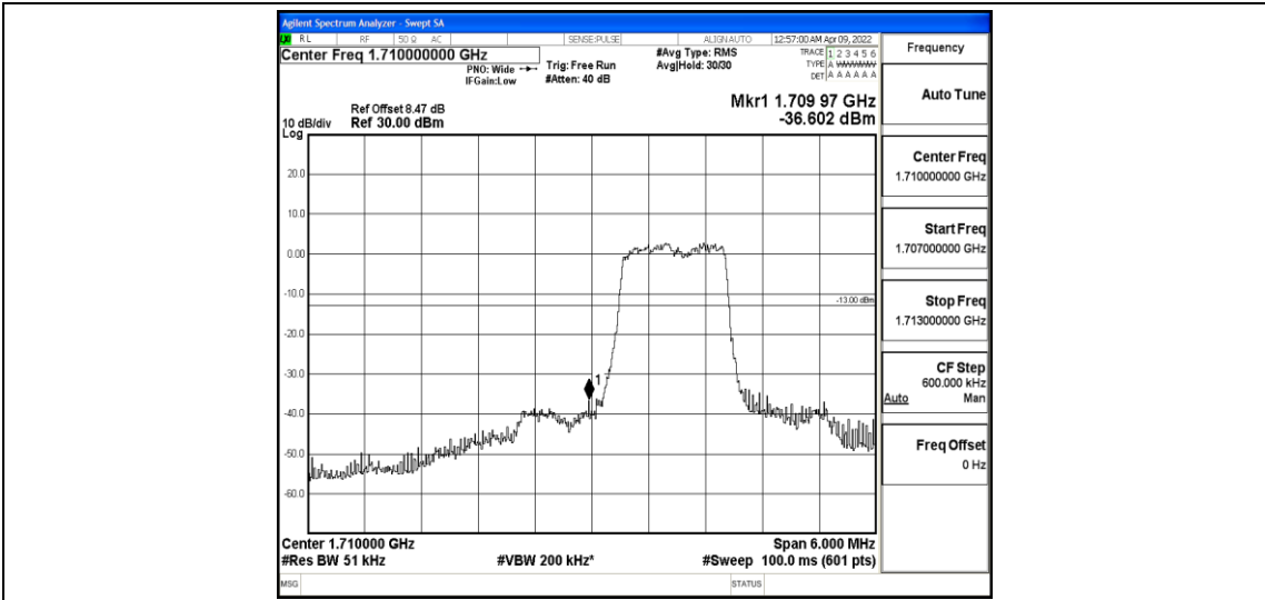
Band4-3MHz-16QAM-19965-6-0-Low--36.60-PASS
