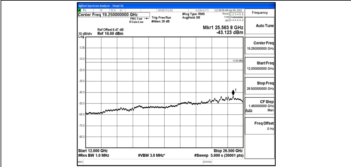
Band4-1.4MHz-QPSK-20175-1-0-Low-12000-26500--43.12-PASS
