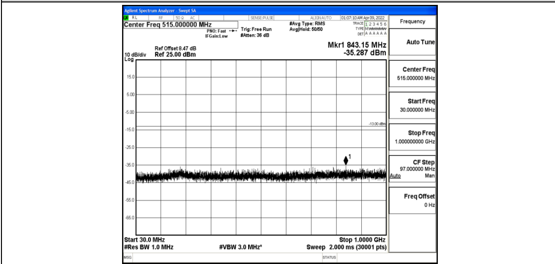
Band4-3MHz-16QAM-20385-1-0-High-30-1000--35.29-PASS
