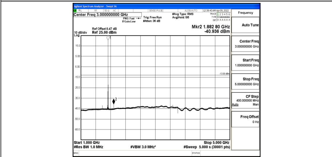
Band4-1.4MHz-16QAM-20175-1-0-Low-1000-5000--40.94-PASS
