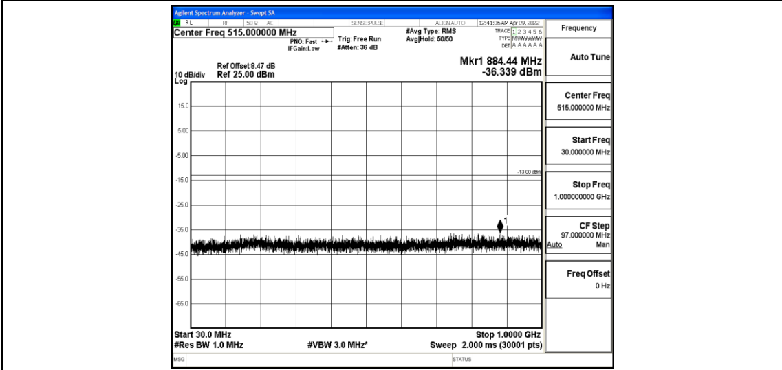
Band4-1.4MHz-QPSK-20393-1-0-High-30-1000--36.34-PASS
