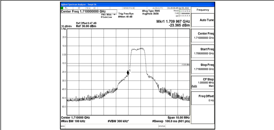
Band4-5MHz-16QAM-19975-6-0-Low--23.36-PASS
