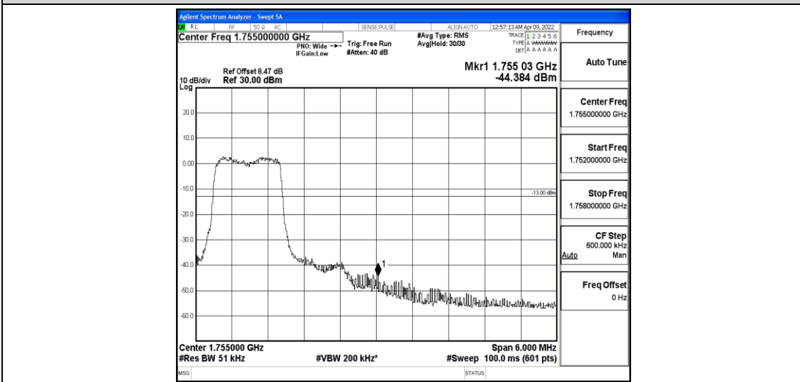
Band4-3MHz-QPSK-20385-6-0-Low--44.38-PASS
