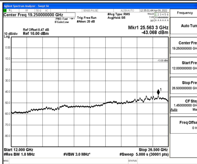
Band4-1.4MHz-QPSK-19957-1-0-Low-12000-26500--43.07-PASS
