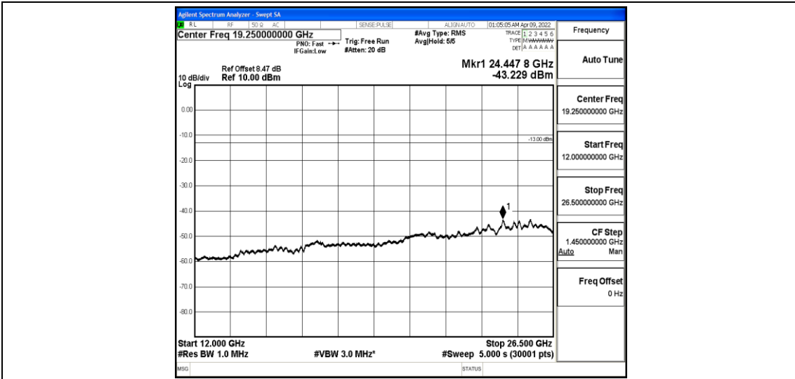
Band4-3MHz-16QAM-20175-1-0-Low-12000-26500--43.23-PASS
