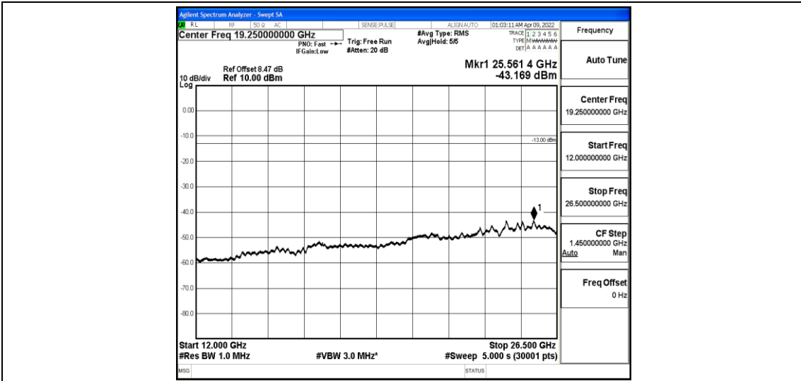
Band4-3MHz-QPSK-20175-1-0-Low-12000-26500--43.17-PASS
