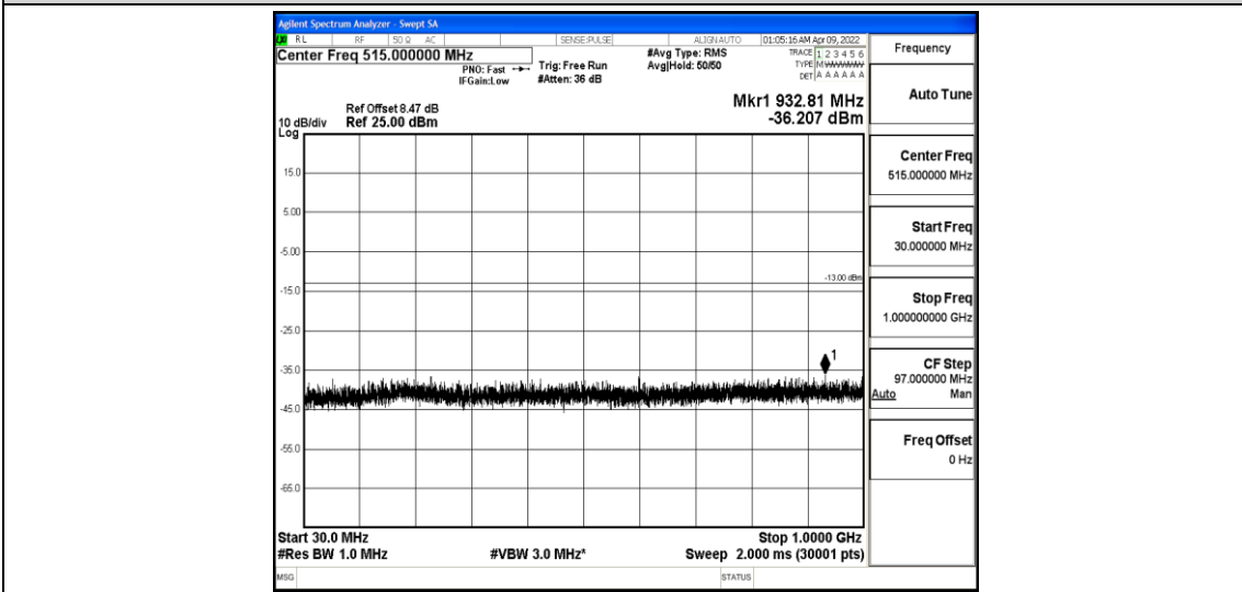
Band4-3MHz-QPSK-20385-1-0-High-30-1000--36.21-PASS
