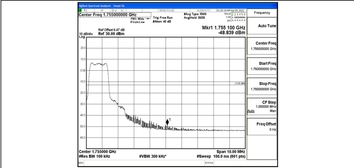
Band4-5MHz-QPSK-20375-6-0-Low--48.84-PASS
