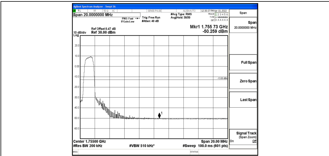
Band4-10MHz-16QAM-20350-6-0-Low--50.26-PASS
