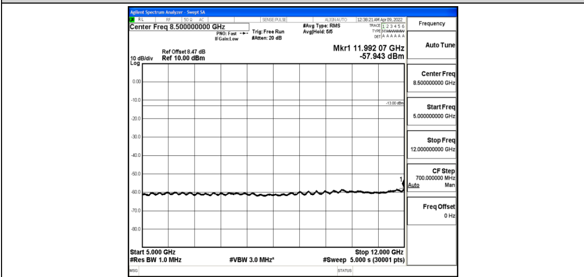
Band4-1.4MHz-QPSK-20175-1-0-Low-5000-12000--57.94-PASS
