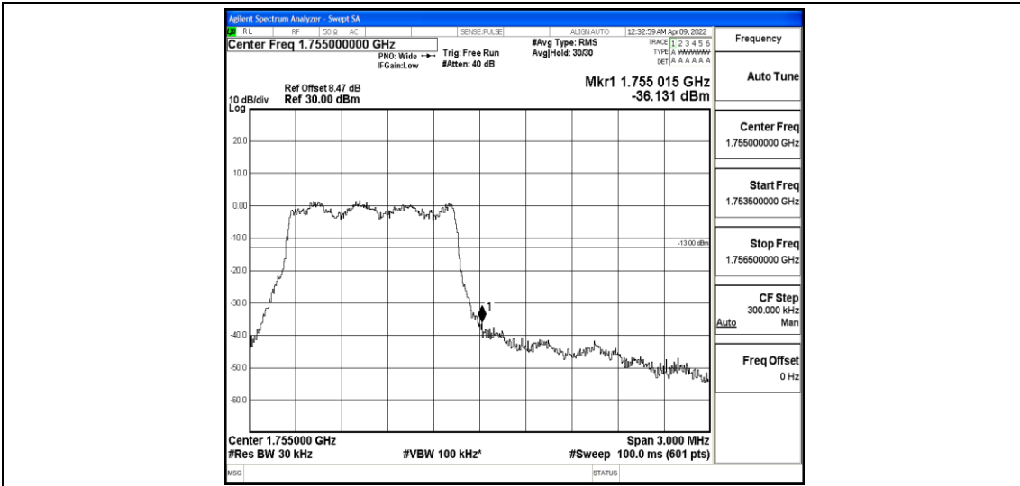
Band4-1.4MHz-16QAM-20393-6-0-Low--36.13-PASS
