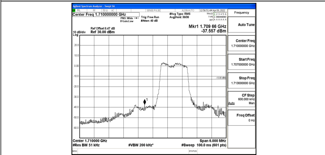
Band4-3MHz-QPSK-19965-6-0-Low--37.56-PASS
