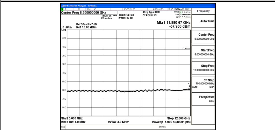
Band4-1.4MHz-16QAM-20175-1-0-Low-5000-12000--57.95-PASS
