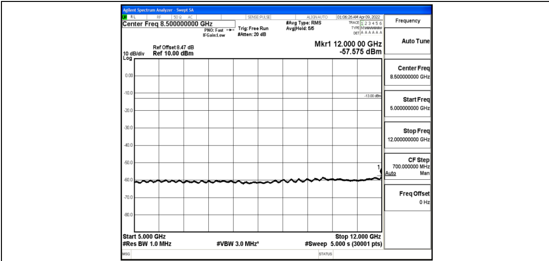
Band4-3MHz-QPSK-20385-1-0-High-5000-12000--57.58-PASS
