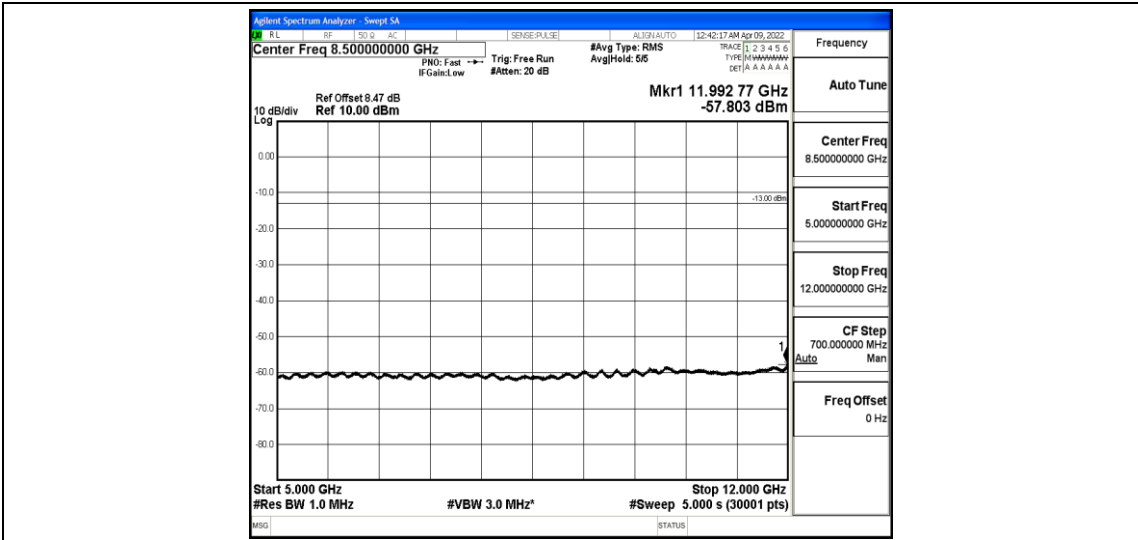
Band4-1.4MHz-QPSK-20393-1-0-High-5000-12000--57.8-PASS
