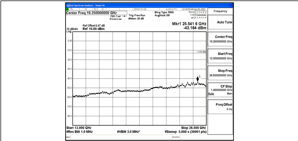
Band4-1.4MHz-16QAM-20175-1-0-Low-12000-26500--43.18-PASS
