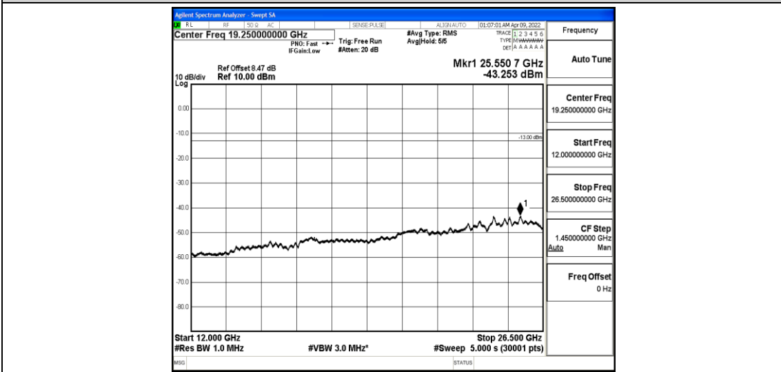
Band4-3MHz-QPSK-20385-1-0-High-12000-26500--43.25-PASS
