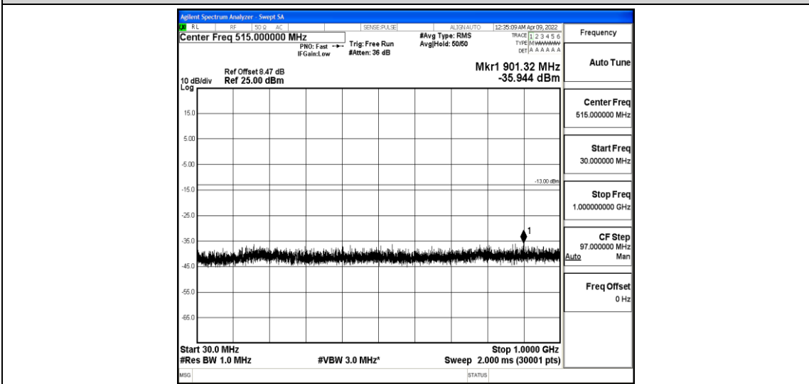
Band4-1.4MHz-16QAM-19957-1-0-Low-30-1000--35.94-PASS
