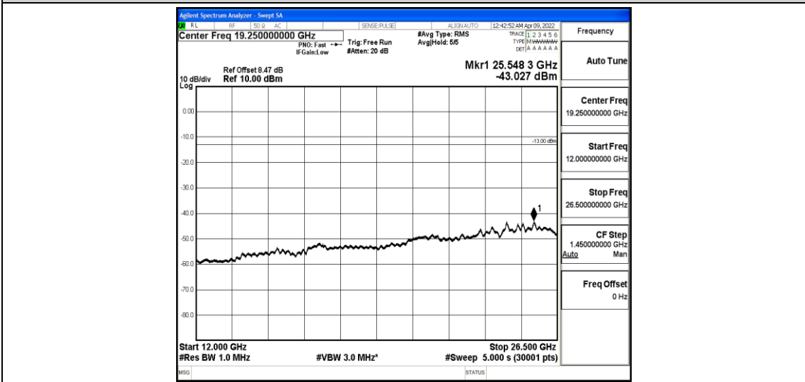
Band4-1.4MHz-QPSK-20393-1-0-High-12000-26500--43.03-PASS
