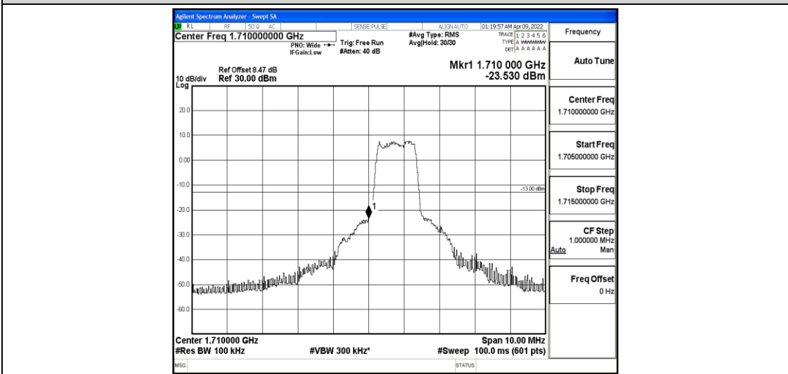
Band4-5MHz-QPSK-19975-6-0-Low--23.53-PASS
