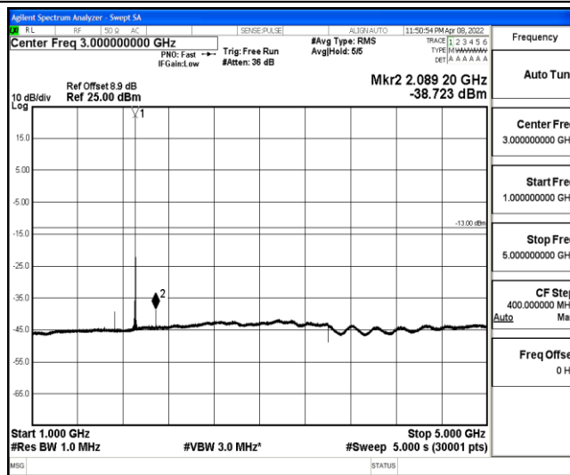
Band2-20MHz-16QAM-19100-1-0-High-1000-5000--38.72-PASS
