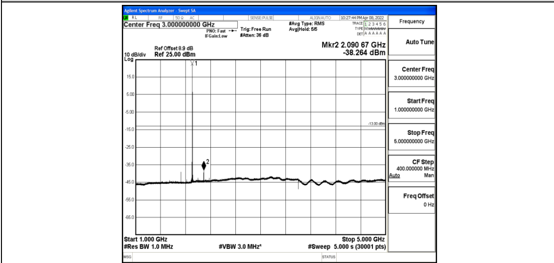
Band2-5MHz-16QAM-19175-1-0-High-1000-5000--38.26-PASS
