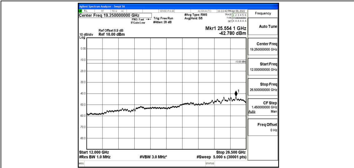
Band2-15MHz-QPSK-18900-1-0-Low-12000-26500--42.78-PASS
