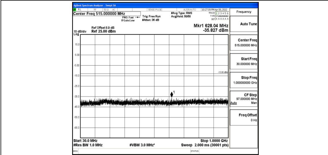
Band2-5MHz-16QAM-19175-1-0-High-30-1000--35.83-PASS
