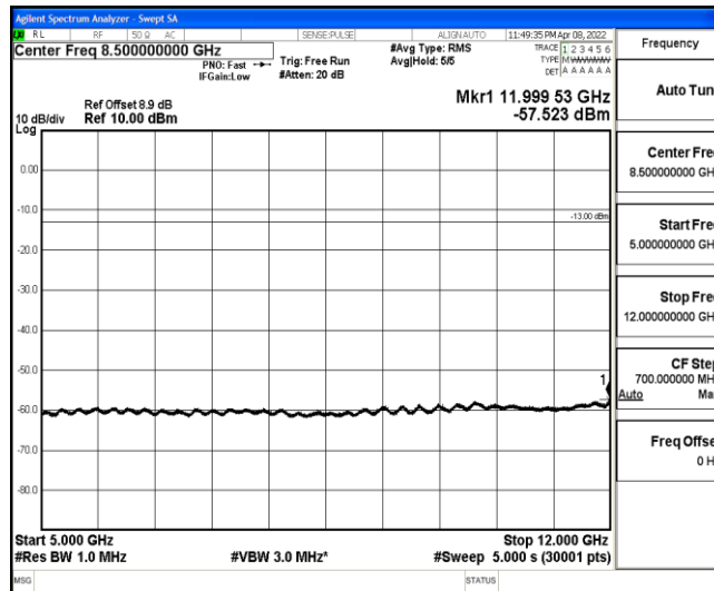
Band2-20MHz-QPSK-19100-1-0-High-5000-12000--57.52-PASS
