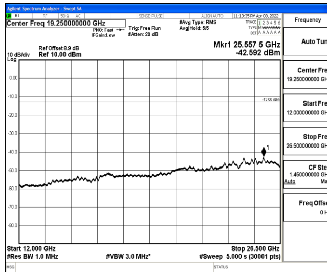
Band2-15MHz-16QAM-18900-1-0-Low-12000-26500--42.59-PASS
