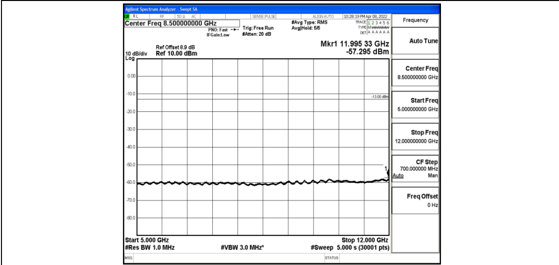
Band2-5MHz-16QAM-19175-1-0-High-5000-12000--57.3-PASS
