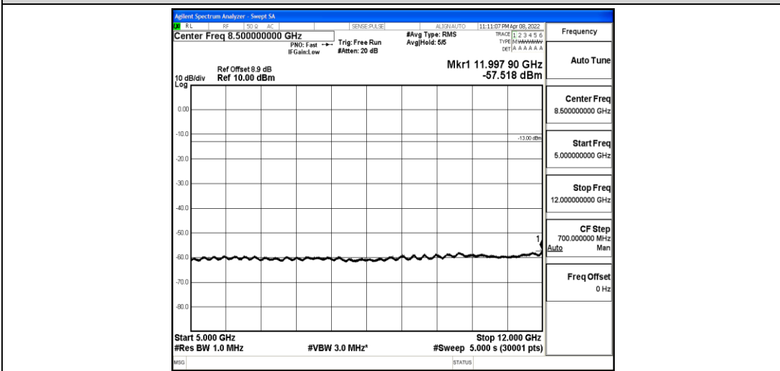
Band2-15MHz-QPSK-18900-1-0-Low-5000-12000--57.52-PASS
