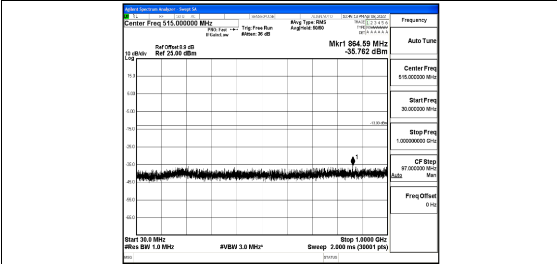
Band2-10MHz-QPSK-19150-1-0-High-30-1000--35.76-PASS
