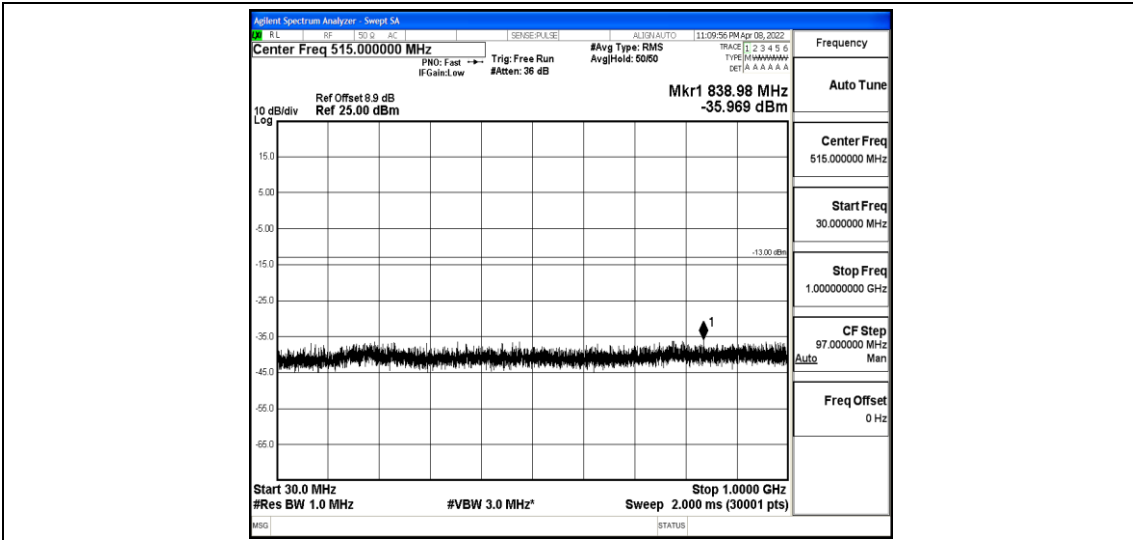
Band2-15MHz-QPSK-18900-1-0-Low-30-1000--35.97-PASS
