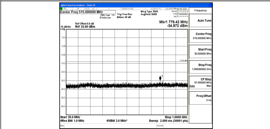
Band2-15MHz-QPSK-19125-1-0-High-30-1000--34.87-PASS
