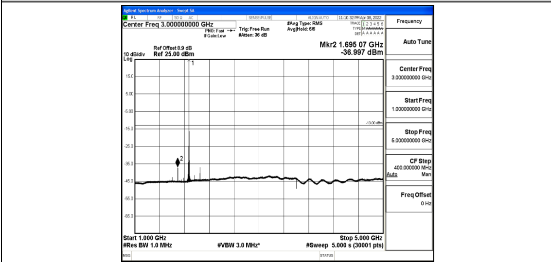
Band2-15MHz-QPSK-18900-1-0-Low-1000-5000--37-PASS
