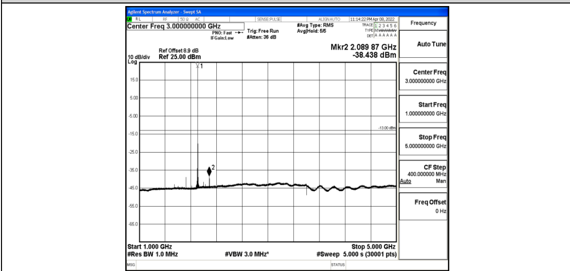
Band2-15MHz-QPSK-19125-1-0-High-1000-5000--38.44-PASS
