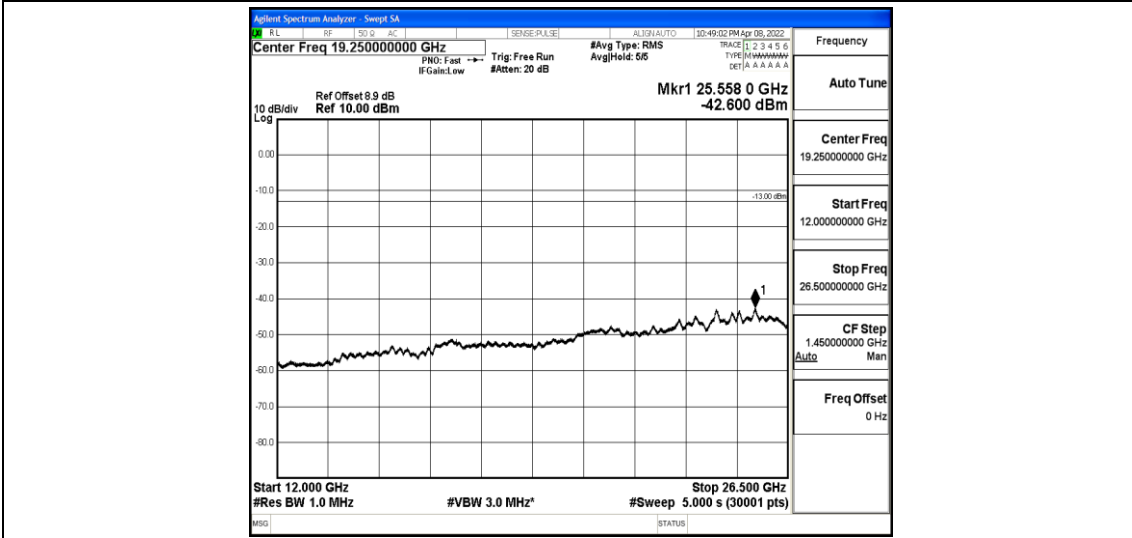
Band2-10MHz-16QAM-18900-1-0-Low-12000-26500--42.6-PASS
