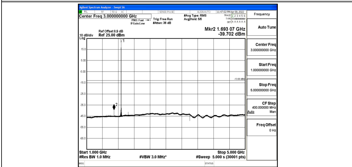
Band2-20MHz-16QAM-18900-1-0-Low-1000-5000--39.7-PASS
