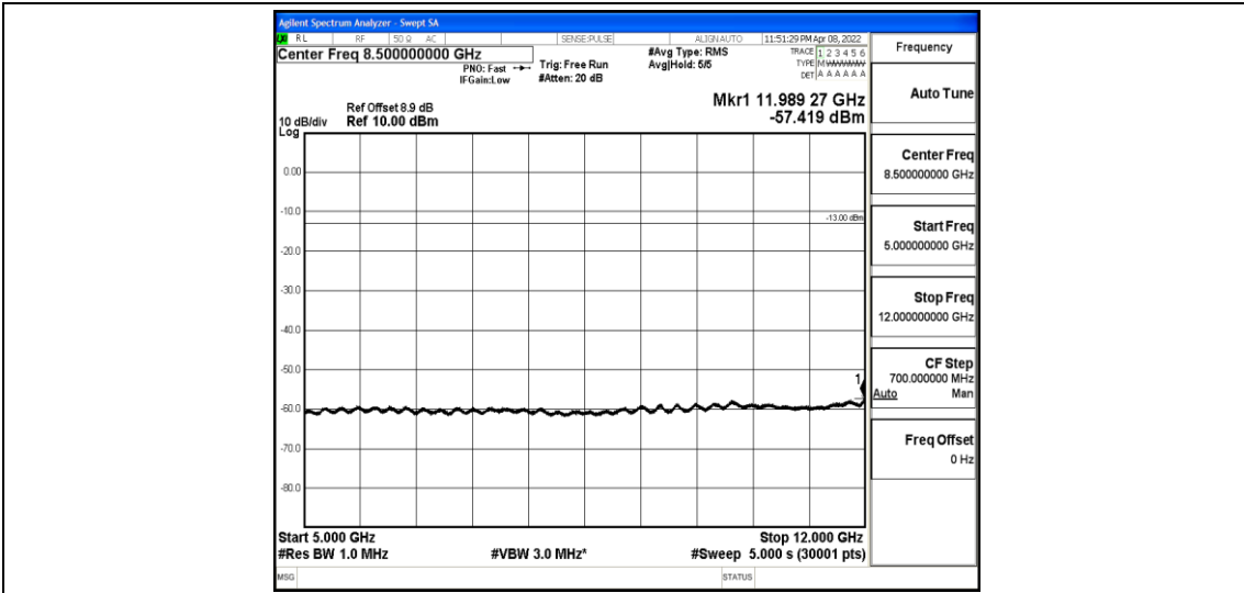
Band2-20MHz-16QAM-19100-1-0-High-5000-12000--57.42-PASS
