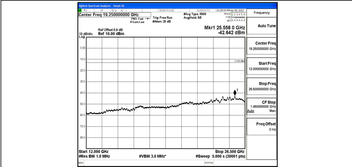
Band2-5MHz-16QAM-19175-1-0-High-12000-26500--42.64-PASS
