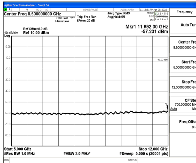
Band2-15MHz-16QAM-19125-1-0-High-5000-12000--57.23-PASS
