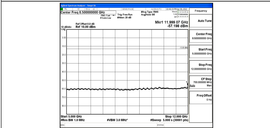
Band2-10MHz-QPSK-18900-1-0-Low-5000-12000--57.2-PASS
