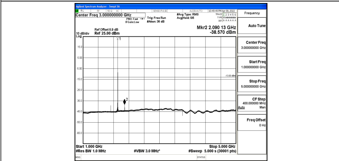
Band2-10MHz-QPSK-19150-1-0-High-1000-5000--38.57-PASS
