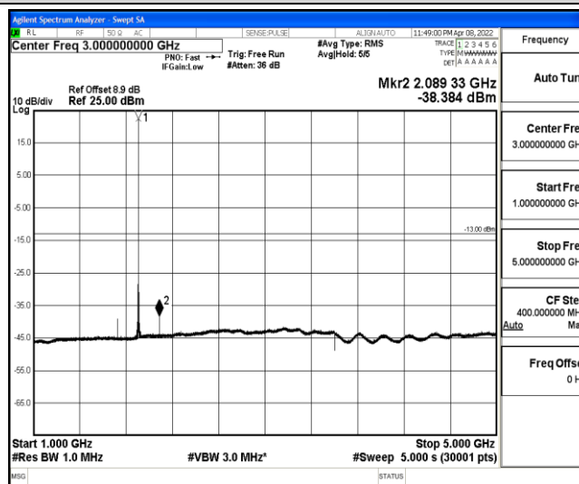
Band2-20MHz-QPSK-19100-1-0-High-1000-5000--38.38-PASS
