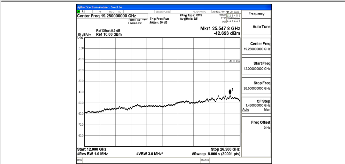
Band2-10MHz-QPSK-18650-1-0-Low-12000-26500--42.69-PASS
