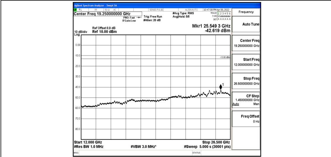
Band2-10MHz-QPSK-18900-1-0-Low-12000-26500--42.62-PASS
