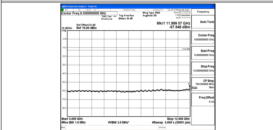
Band2-20MHz-16QAM-18900-1-0-Low-5000-12000--57.55-PASS
