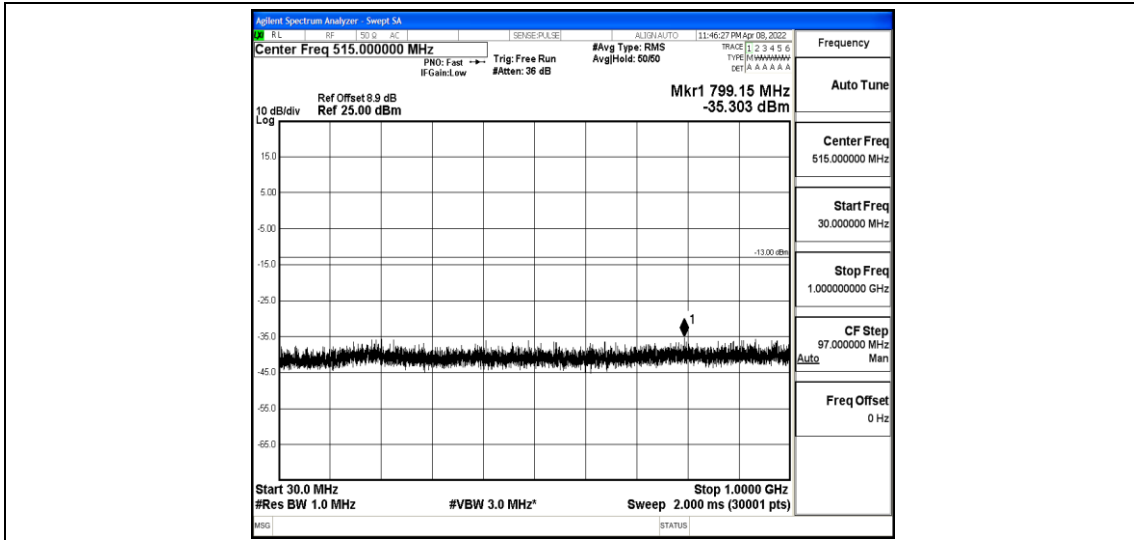
Band2-20MHz-16QAM-18900-1-0-Low-30-1000--35.3-PASS
