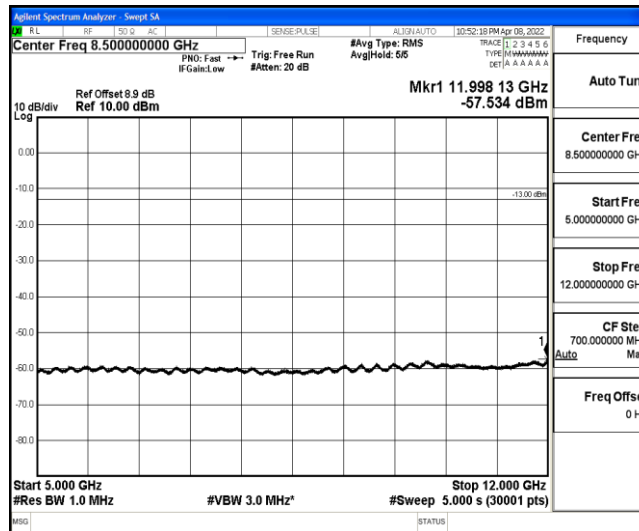
Band2-10MHz-16QAM-19150-1-0-High-5000-12000--57.53-PASS
