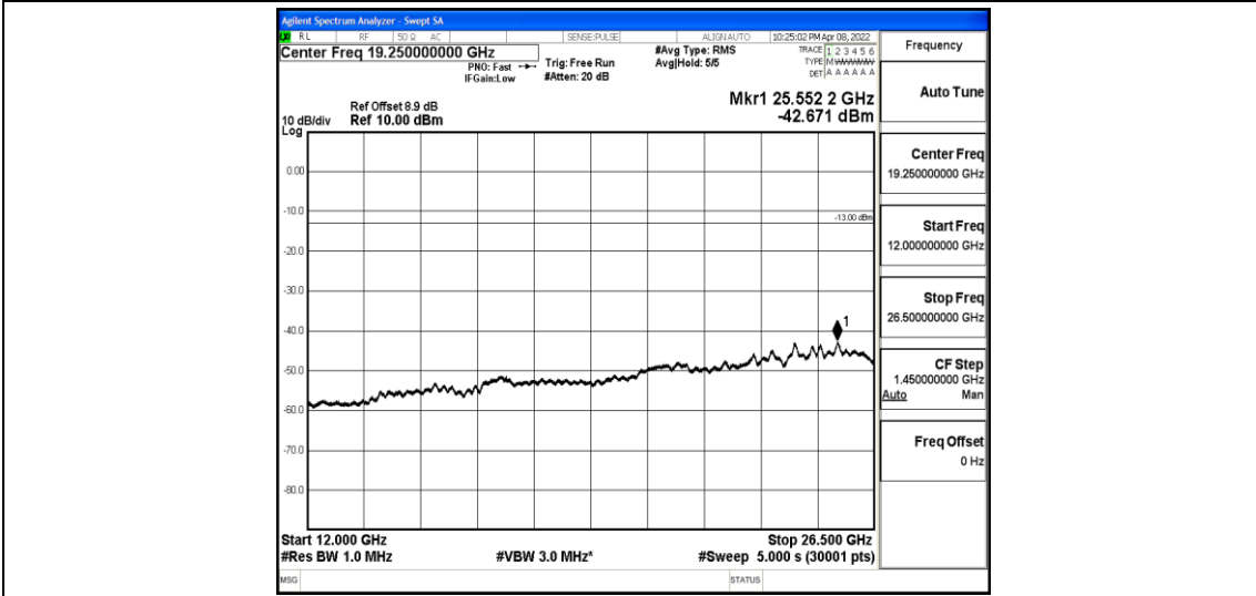
Band2-5MHz-16QAM-18900-1-0-Low-12000-26500--42.67-PASS
