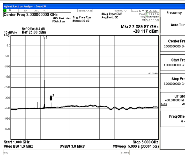
Band2-15MHz-16QAM-19125-1-0-High-1000-5000--38.12-PASS
