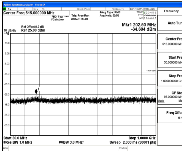
Band2-10MHz-16QAM-18900-1-0-Low-30-1000--34.69-PASS
