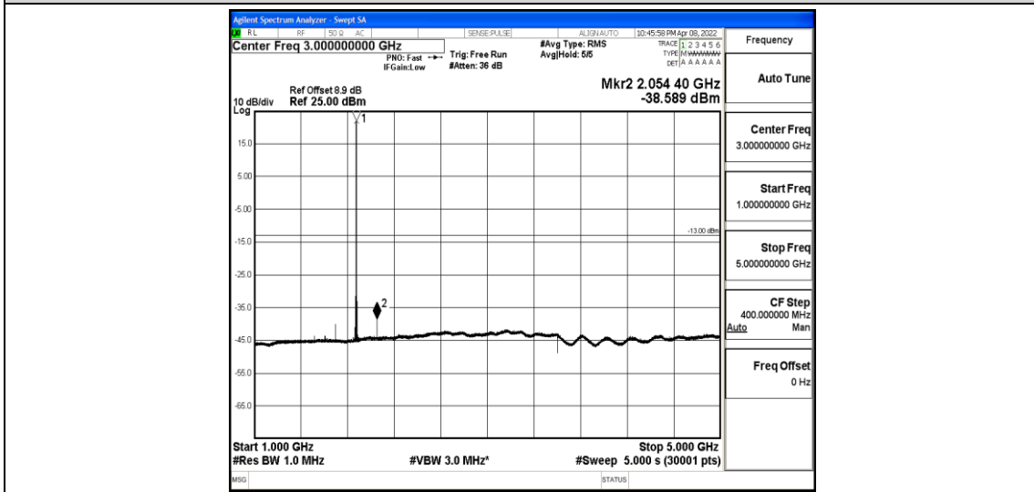
Band2-10MHz-QPSK-18900-1-0-Low-1000-5000--38.59-PASS
