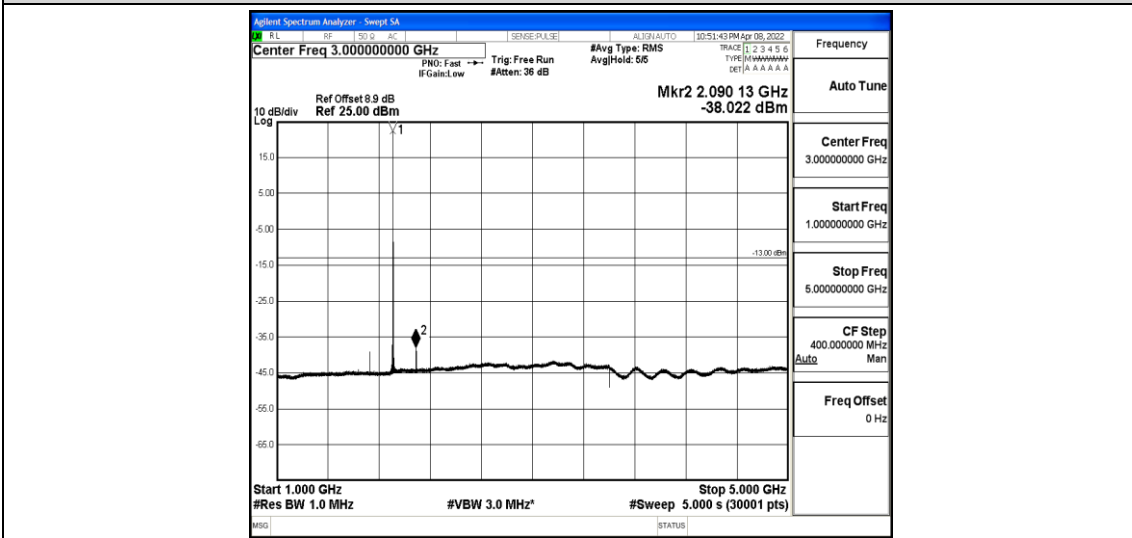
Band2-10MHz-16QAM-19150-1-0-High-1000-5000--38.02-PASS
