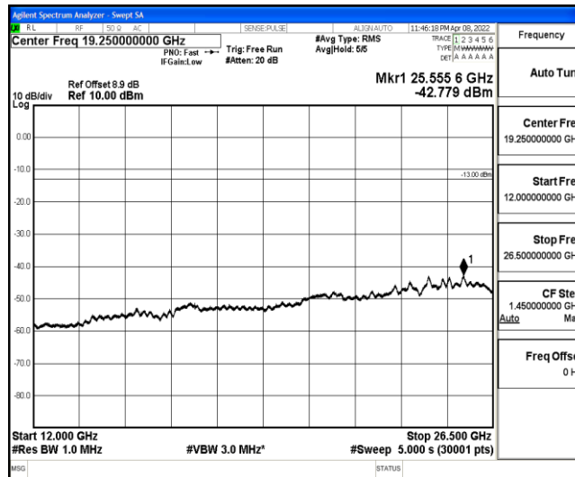
Band2-20MHz-QPSK-18900-1-0-Low-12000-26500--42.78-PASS
