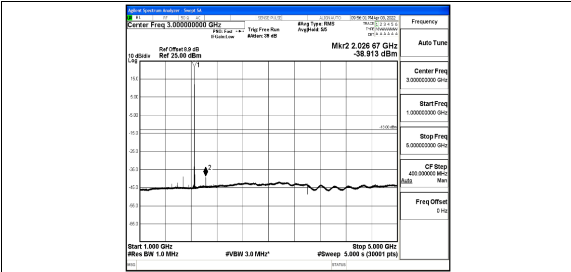
Band2-3MHz-16QAM-18615-1-0-Low-1000-5000--38.91-PASS
