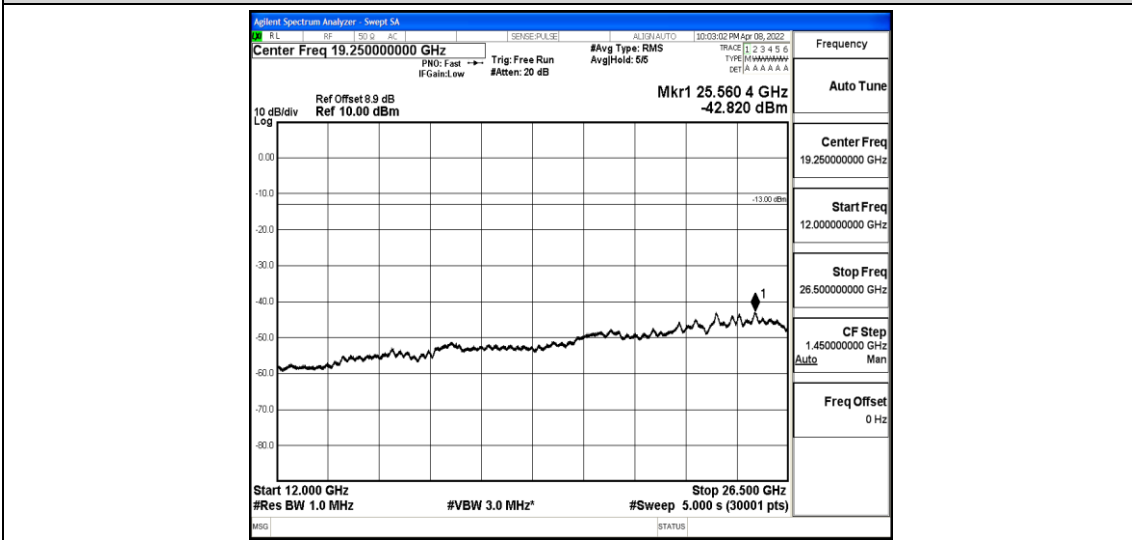
Band2-3MHz-QPSK-19185-1-0-High-12000-26500--42.82-PASS
