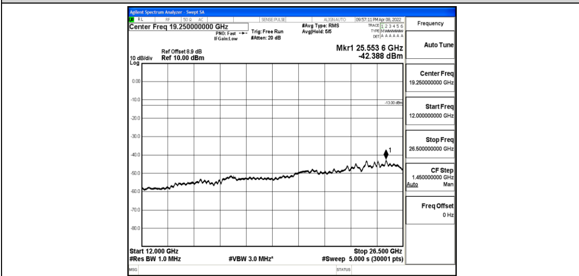
Band2-3MHz-16QAM-18615-1-0-Low-12000-26500--42.39-PASS
