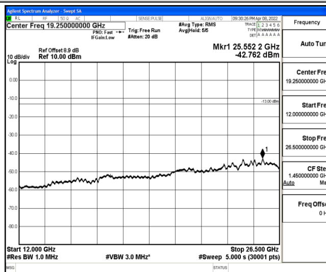
Band2-1.4MHz-QPSK-18607-1-0-Low-12000-26500--42.76-PASS
