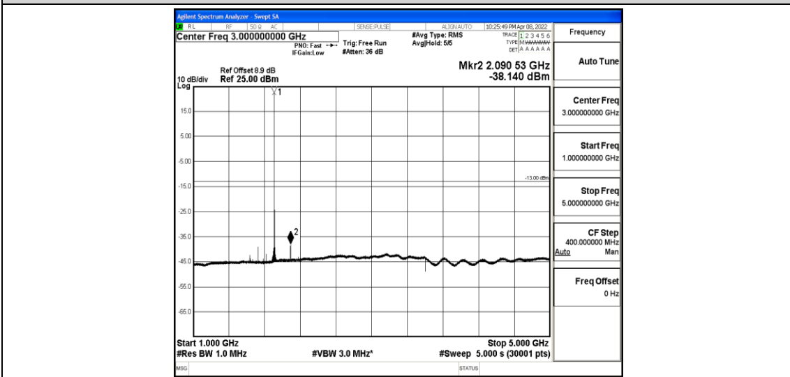
Band2-5MHz-QPSK-19175-1-0-High-1000-5000--38.14-PASS
