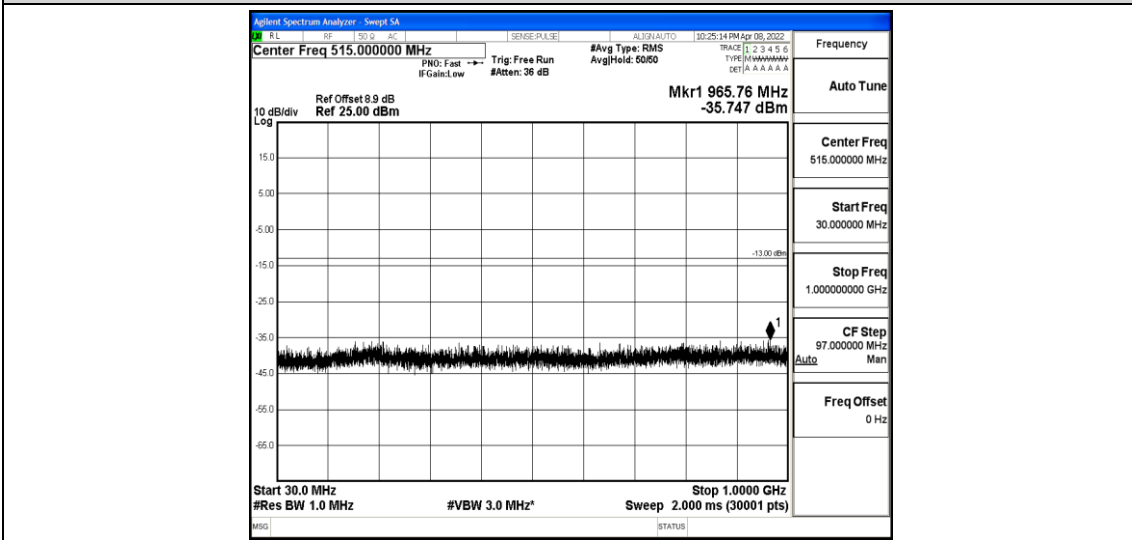
Band2-5MHz-QPSK-19175-1-0-High-30-1000--35.75-PASS
