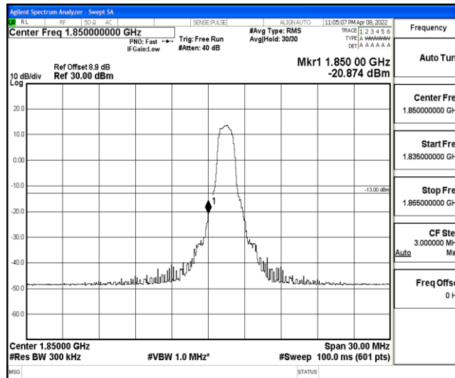
Band2-15MHz-QPSK-18675-6-0-Low--20.87-PASS
