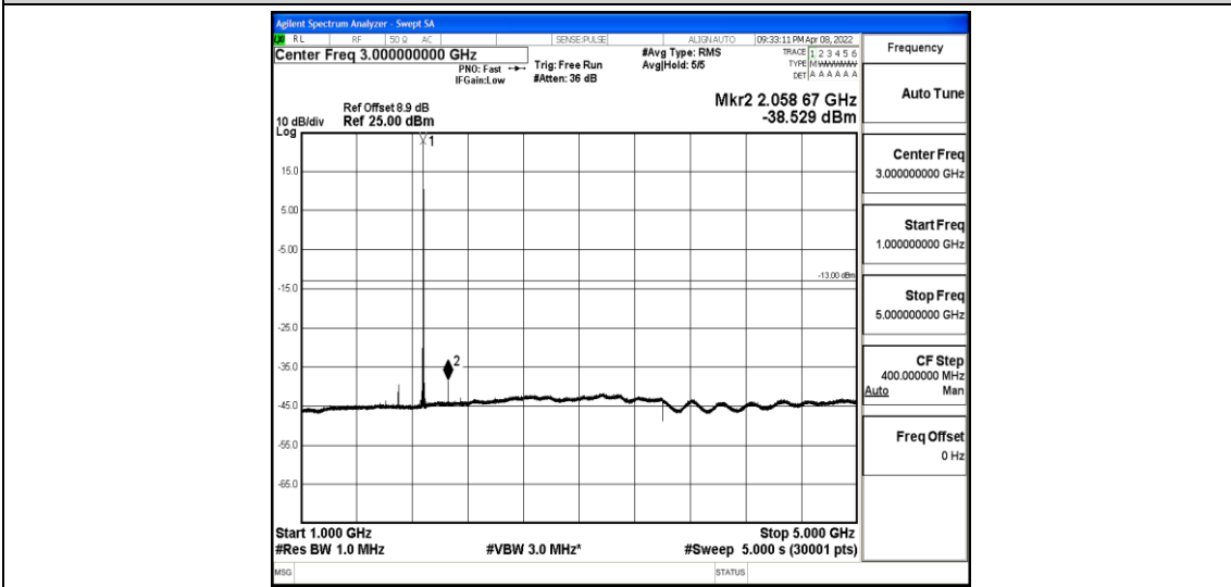
Band2-1.4MHz-QPSK-18900-1-0-Low-1000-5000--38.53-PASS
