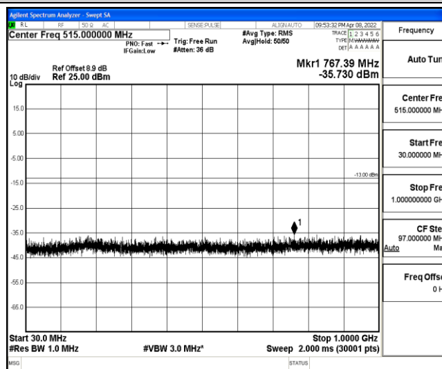
Band2-3MHz-QPSK-18615-1-0-Low-30-1000--35.73-PASS
