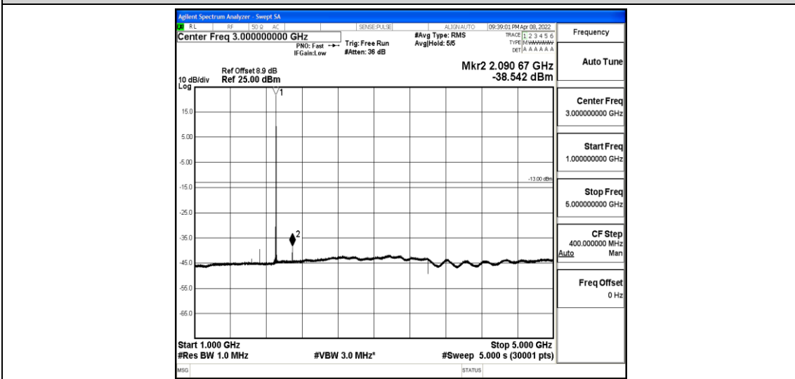
Band2-1.4MHz-16QAM-19193-1-0-High-1000-5000--38.54-PASS
