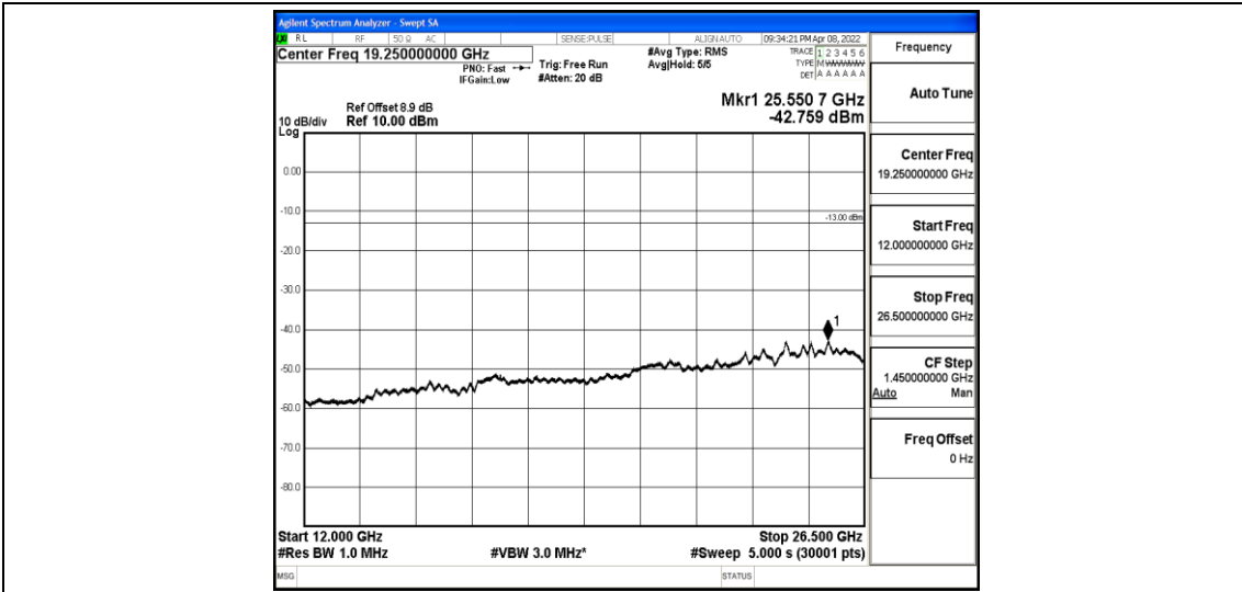
Band2-1.4MHz-QPSK-18900-1-0-Low-12000-26500--42.76-PASS
