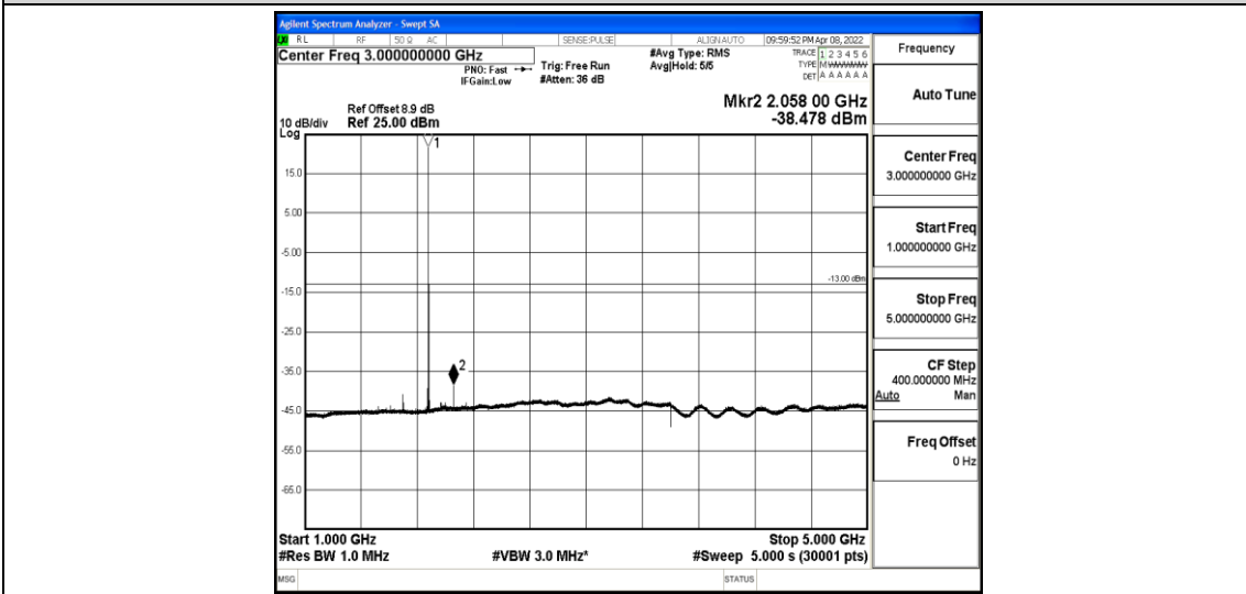
Band2-3MHz-16QAM-18900-1-0-Low-1000-5000--38.48-PASS
