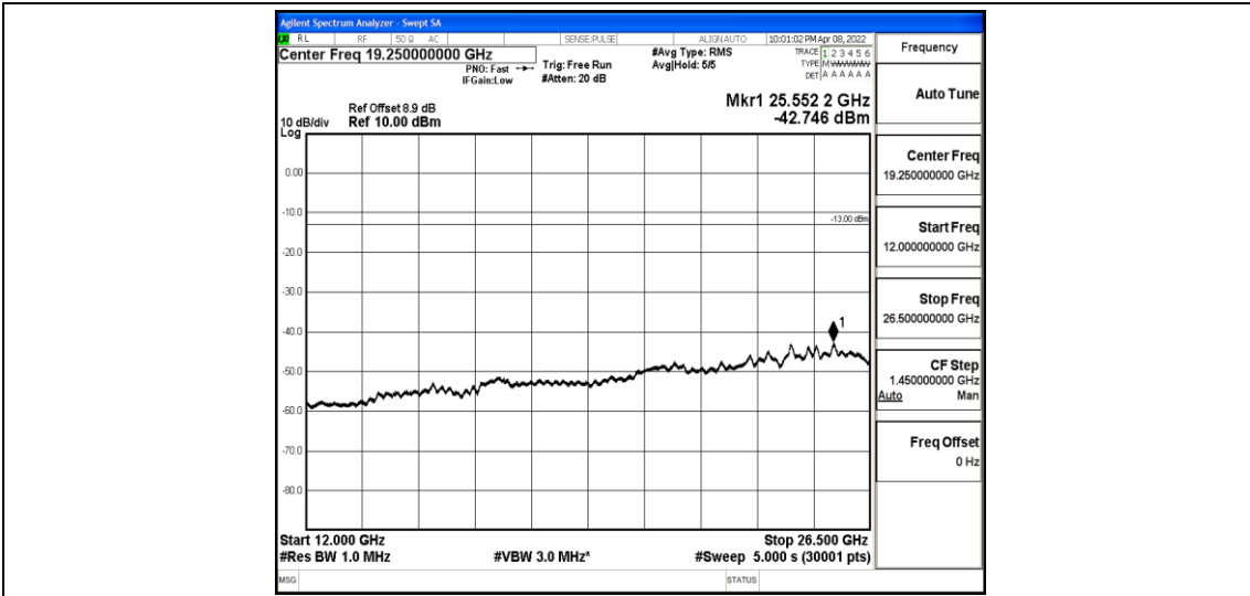
Band2-3MHz-16QAM-18900-1-0-Low-12000-26500--42.75-PASS
