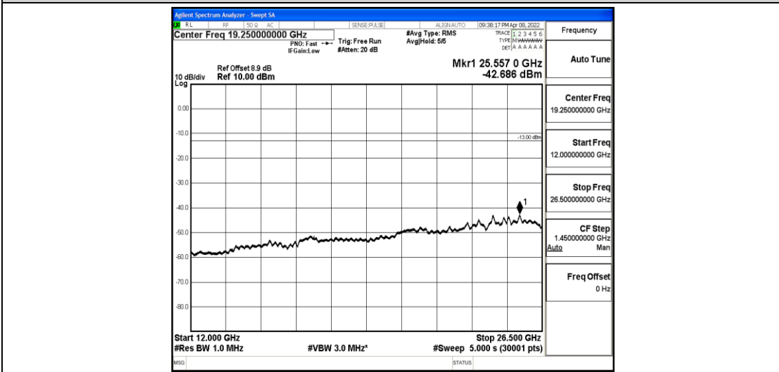
Band2-1.4MHz-QPSK-19193-1-0-High-12000-26500--42.69-PASS
