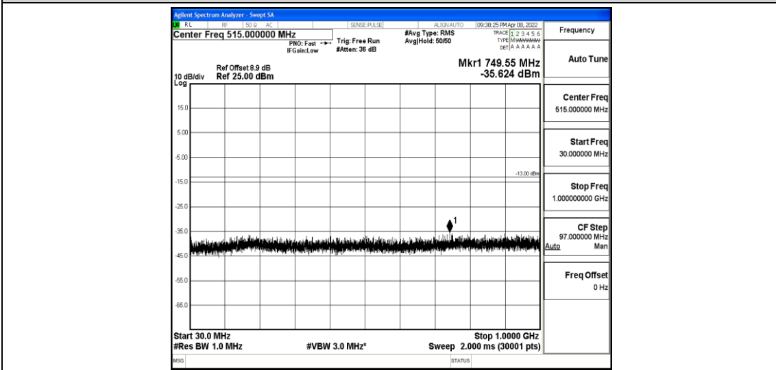
Band2-1.4MHz-16QAM-19193-1-0-High-30-1000--35.62-PASS
