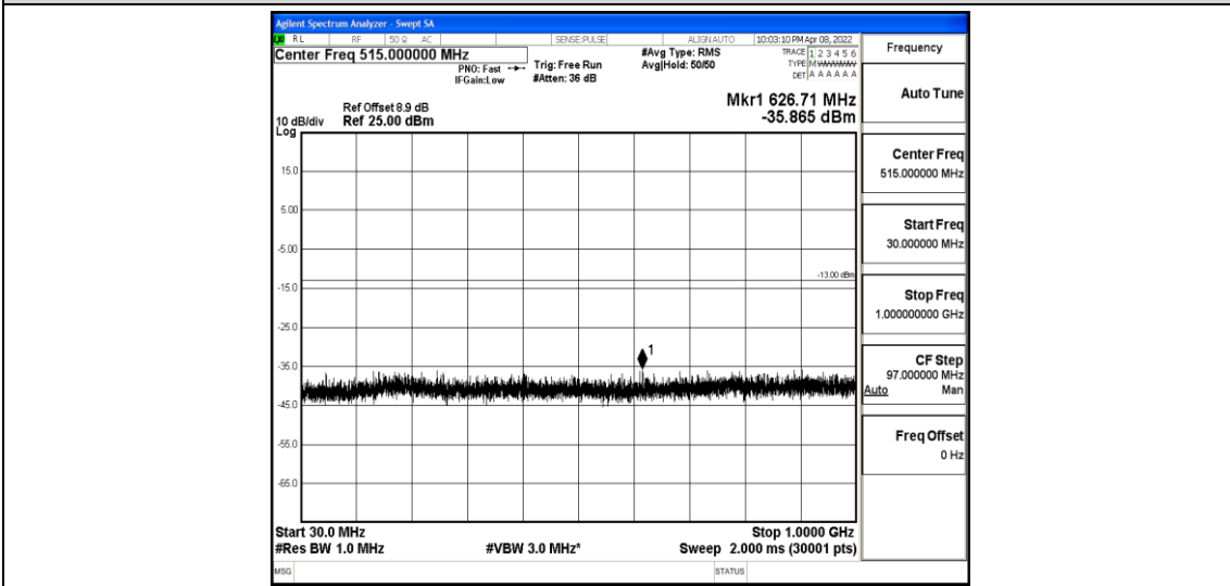
Band2-3MHz-16QAM-19185-1-0-High-30-1000--35.87-PASS
