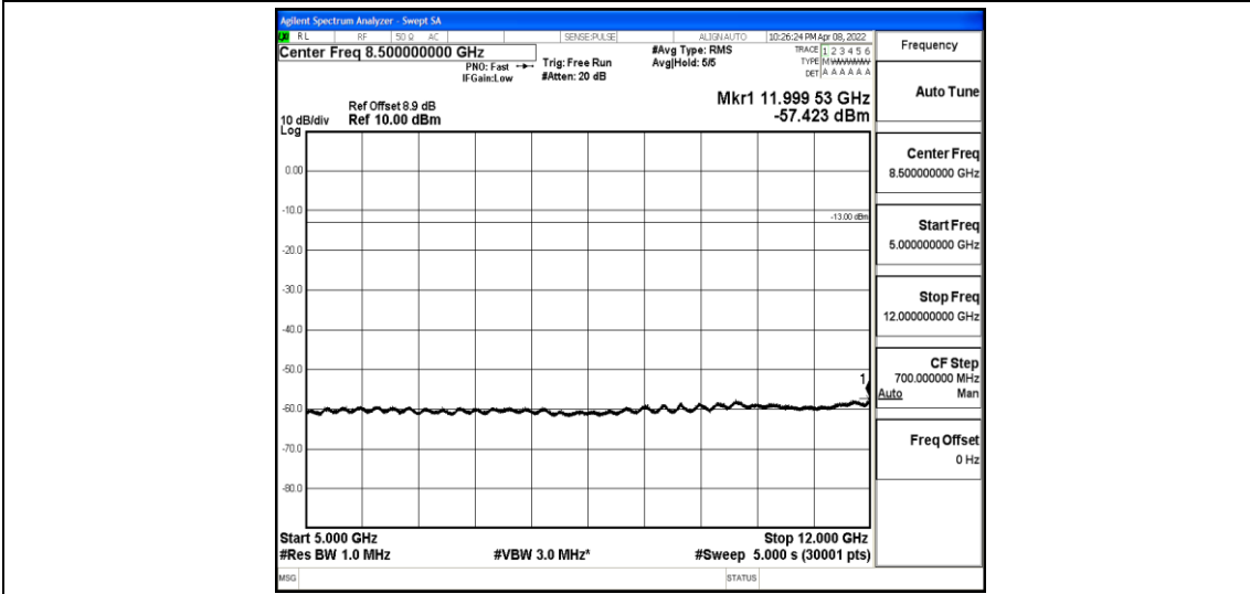
Band2-5MHz-QPSK-19175-1-0-High-5000-12000--57.42-PASS
