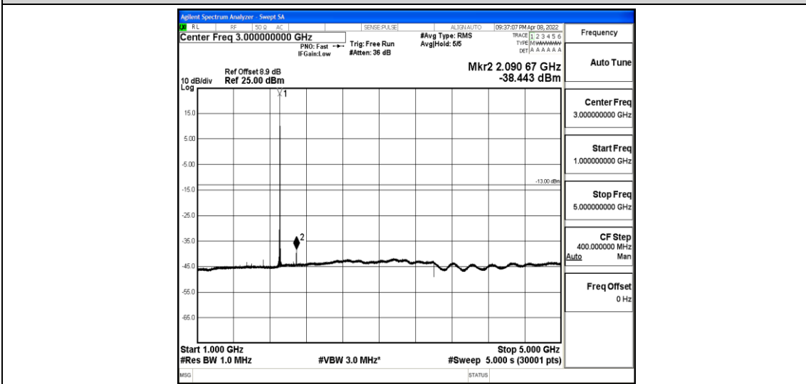
Band2-1.4MHz-QPSK-19193-1-0-High-1000-5000--38.44-PASS
