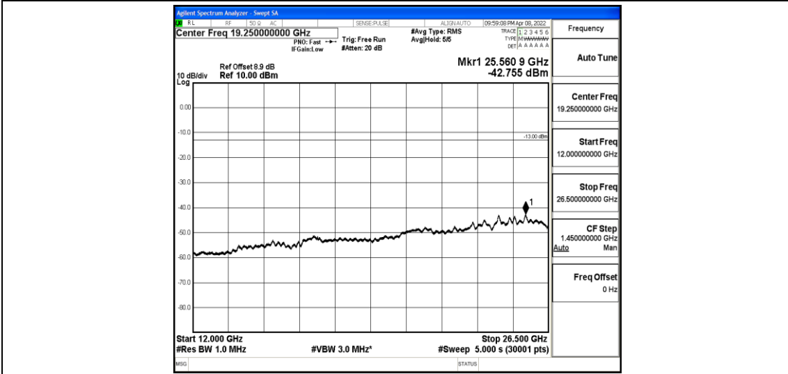
Band2-3MHz-QPSK-18900-1-0-Low-12000-26500--42.76-PASS
