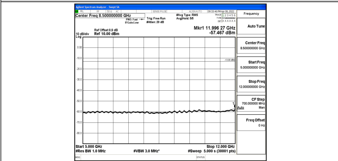
Band2-1.4MHz-QPSK-18900-1-0-Low-5000-12000--57.47-PASS
