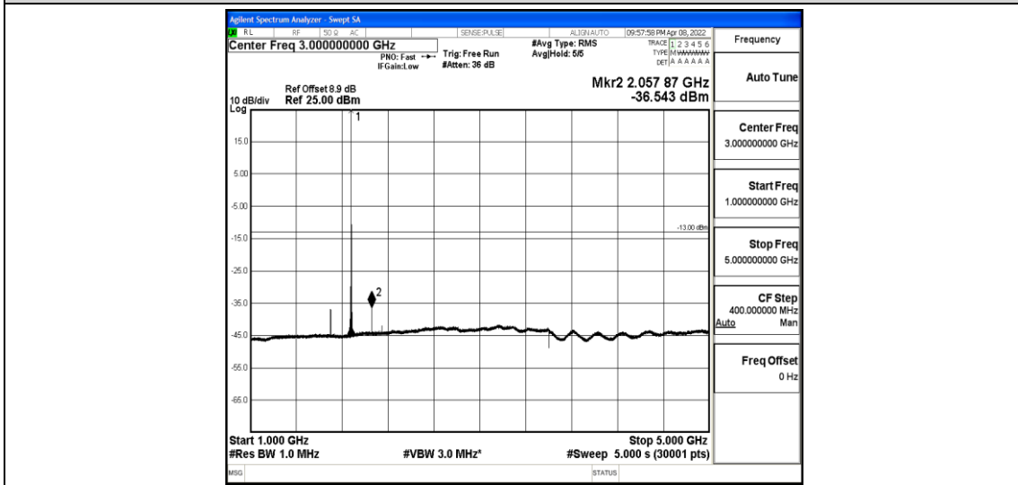
Band2-3MHz-QPSK-18900-1-0-Low-1000-5000--36.54-PASS
