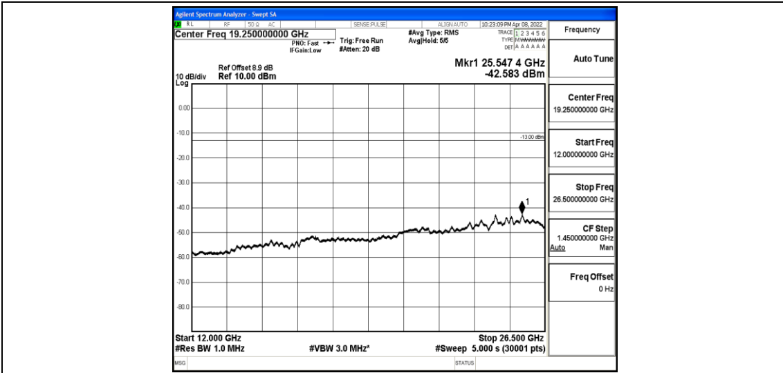
Band2-5MHz-QPSK-18900-1-0-Low-12000-26500--42.58-PASS
