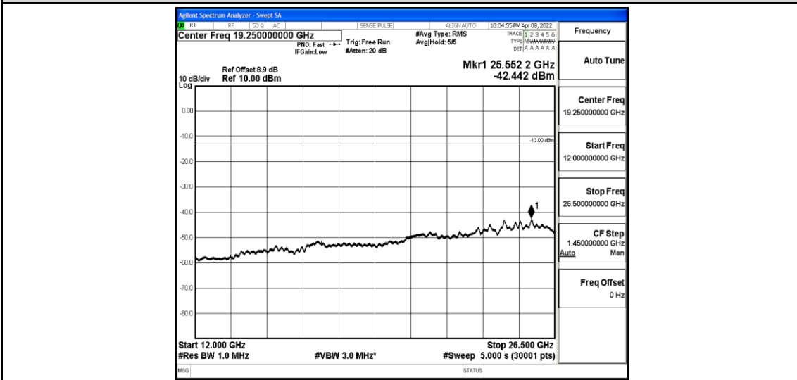
Band2-3MHz-16QAM-19185-1-0-High-12000-26500--42.44-PASS
