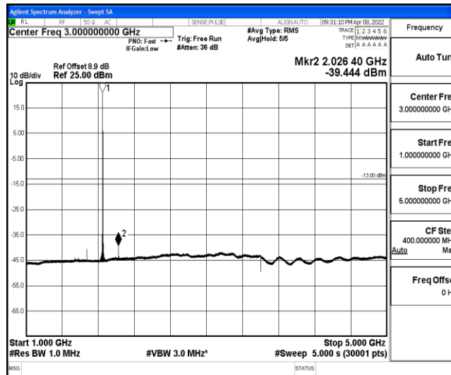
Band2-1.4MHz-16QAM-18607-1-0-Low-1000-5000--39.44-PASS
