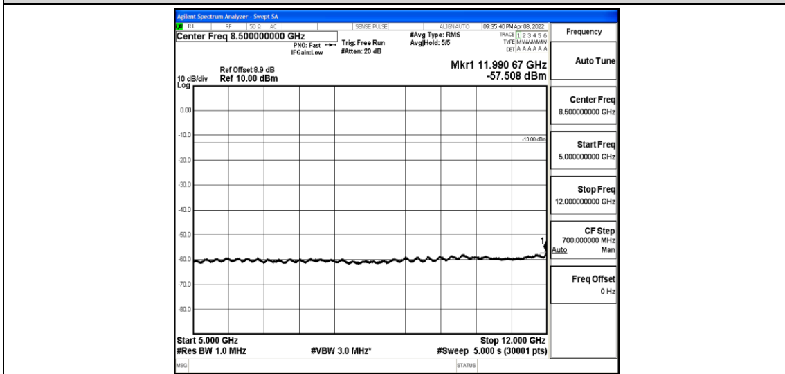
Band2-1.4MHz-16QAM-18900-1-0-Low-5000-12000--57.51-PASS
