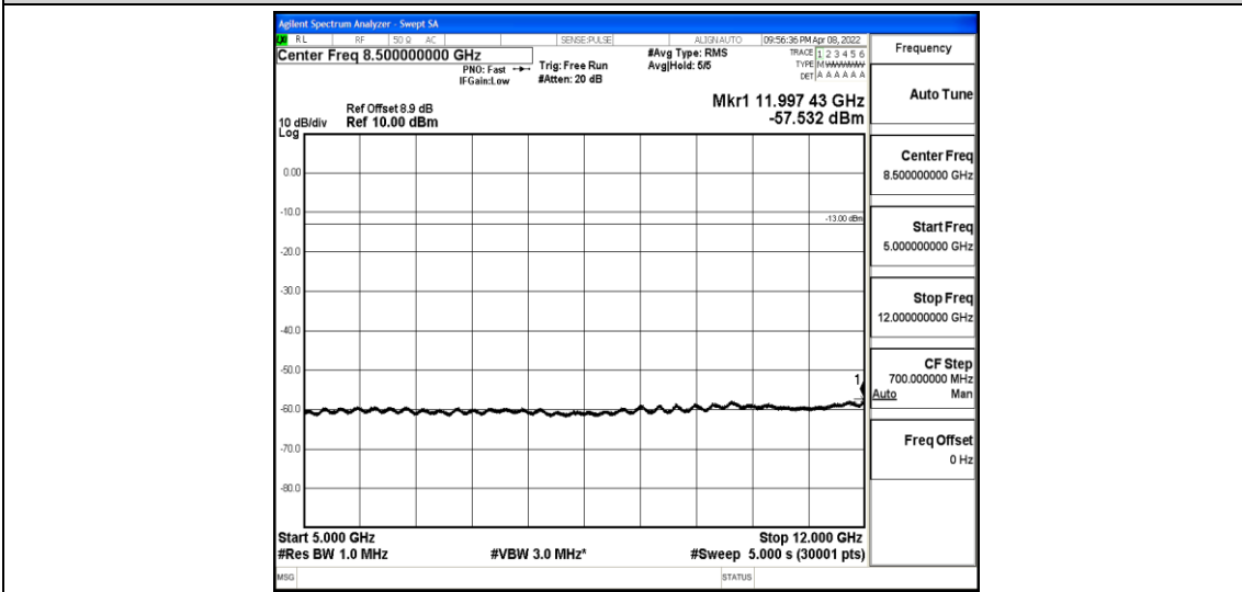
Band2-3MHz-16QAM-18615-1-0-Low-5000-12000--57.53-PASS
