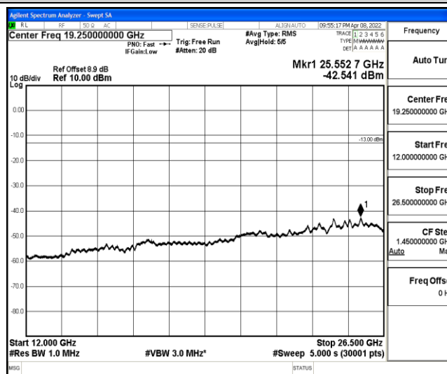
Band2-3MHz-QPSK-18615-1-0-Low-12000-26500--42.54-PASS
