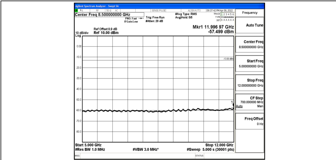
Band2-1.4MHz-QPSK-19193-1-0-High-5000-12000--57.5-PASS
