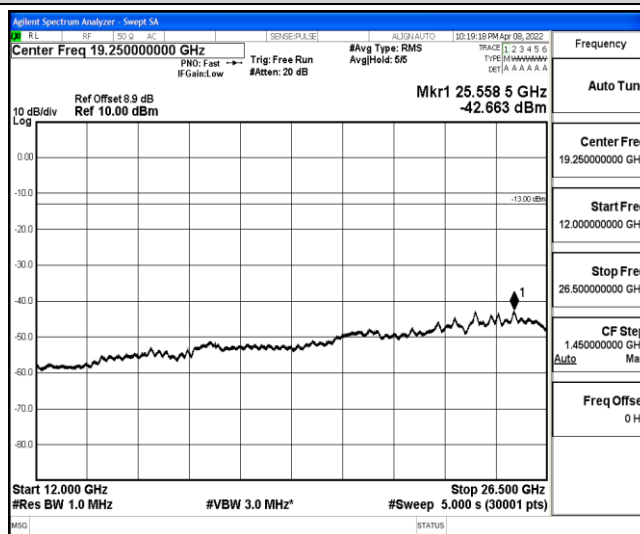
Band2-5MHz-QPSK-18625-1-0-Low-12000-26500--42.66-PASS
