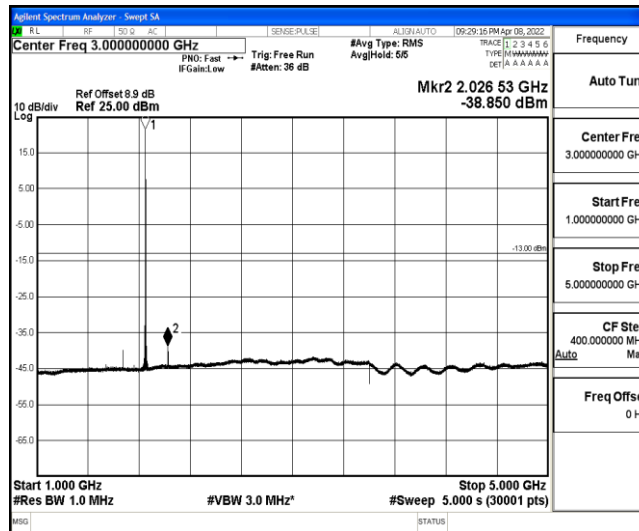
Band2-1.4MHz-QPSK-18607-1-0-Low-1000-5000--38.85-PASS
