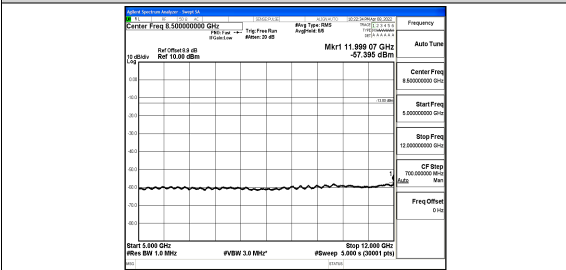
Band2-5MHz-QPSK-18900-1-0-Low-5000-12000--57.4-PASS
