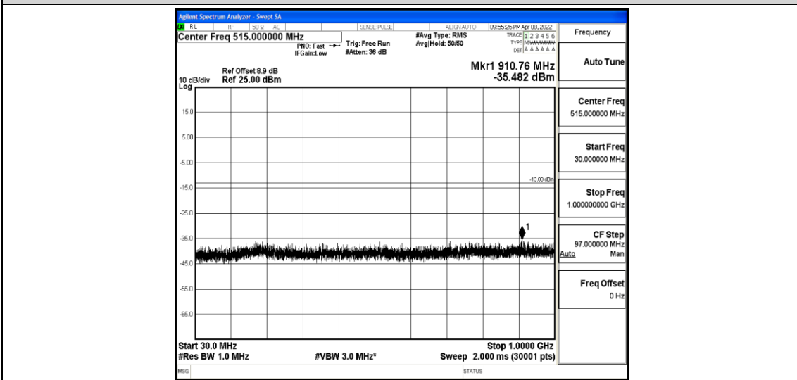
Band2-3MHz-16QAM-18615-1-0-Low-30-1000--35.48-PASS
