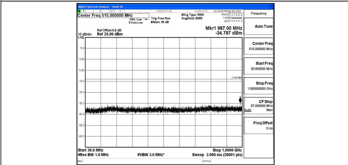
Band2-5MHz-16QAM-18625-1-0-Low-30-1000--34.8-PASS
