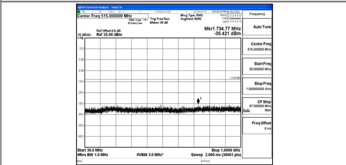
Band2-1.4MHz-16QAM-18607-1-0-Low-30-1000--35.42-PASS
