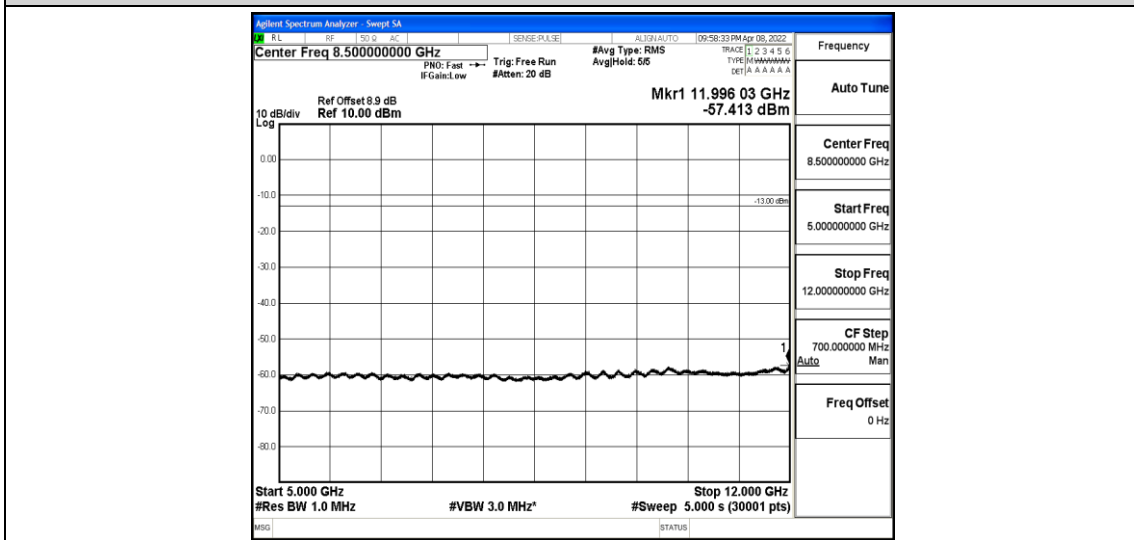
Band2-3MHz-QPSK-18900-1-0-Low-5000-12000--57.41-PASS
