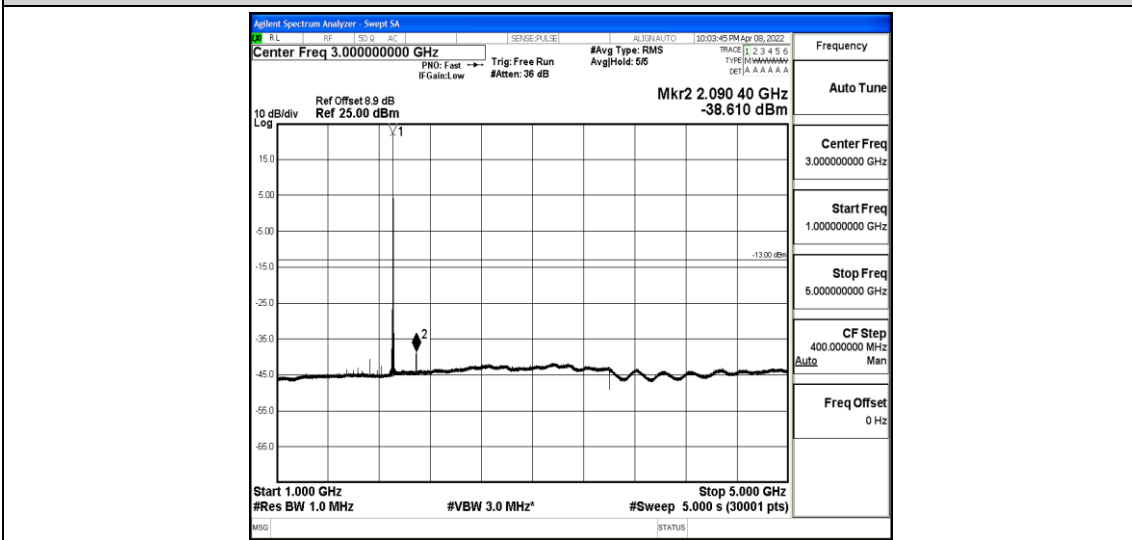
Band2-3MHz-16QAM-19185-1-0-High-1000-5000--38.61-PASS
