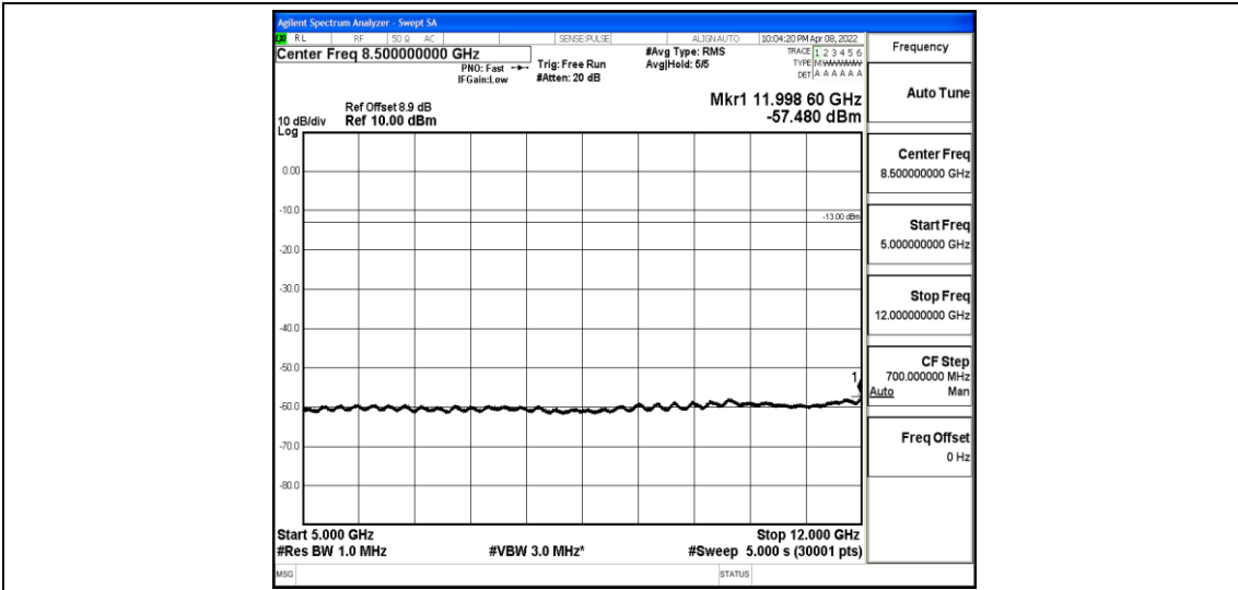
Band2-3MHz-16QAM-19185-1-0-High-5000-12000--57.48-PASS
