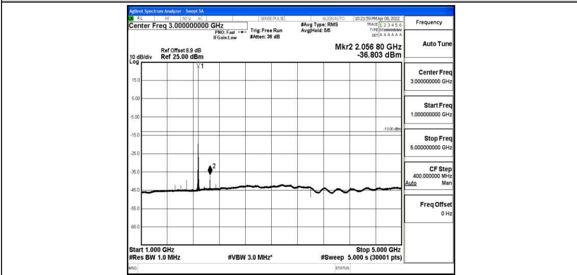
Band2-5MHz-QPSK-18900-1-0-Low-1000-5000--36.8-PASS
