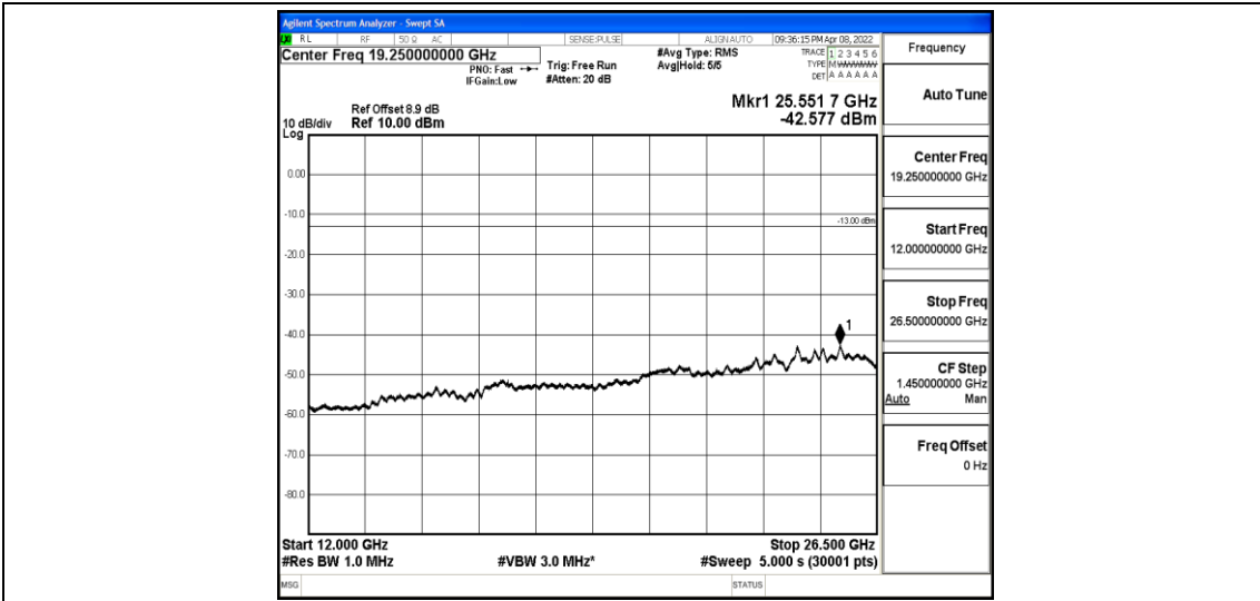
Band2-1.4MHz-16QAM-18900-1-0-Low-12000-26500--42.58-PASS
