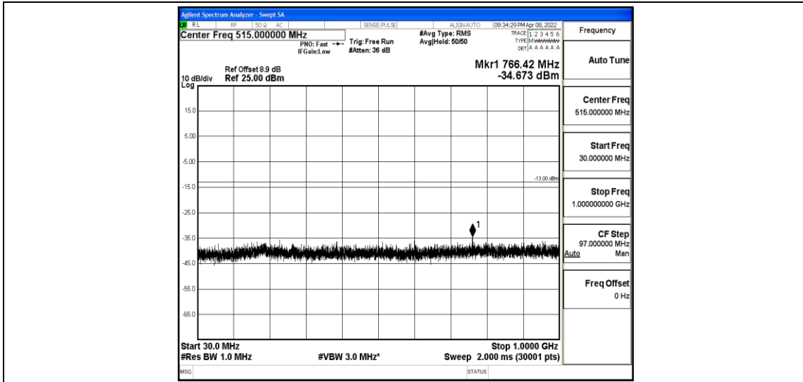
Band2-1.4MHz-16QAM-18900-1-0-Low-30-1000--34.67-PASS
