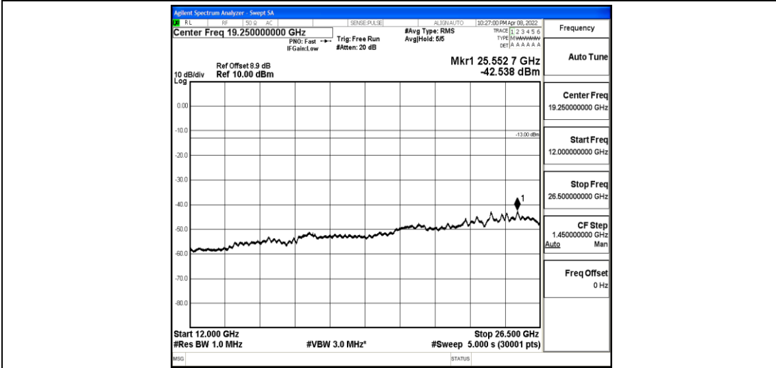
Band2-5MHz-QPSK-19175-1-0-High-12000-26500--42.54-PASS
