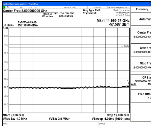
Band2-1.4MHz-16QAM-19193-1-0-High-5000-12000--57.59-PASS
