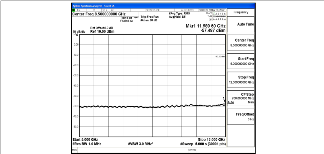
Band2-3MHz-QPSK-19185-1-0-High-5000-12000--57.49-PASS
