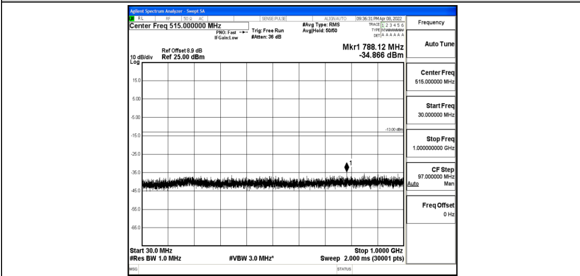
Band2-1.4MHz-QPSK-19193-1-0-High-30-1000--34.87-PASS
