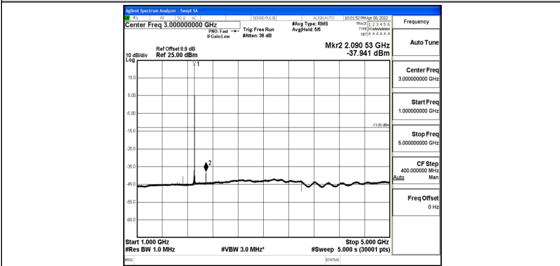
Band2-3MHz-QPSK-19185-1-0-High-1000-5000--37.94-PASS
