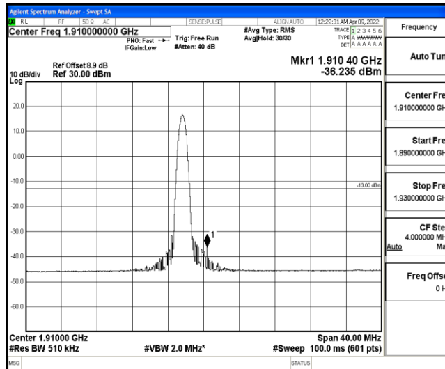
Band2-20MHz-QPSK-19100-1-0-High--36.24-PASS
