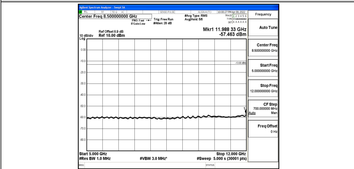
Band2-3MHz-16QAM-18900-1-0-Low-5000-12000--57.46-PASS
