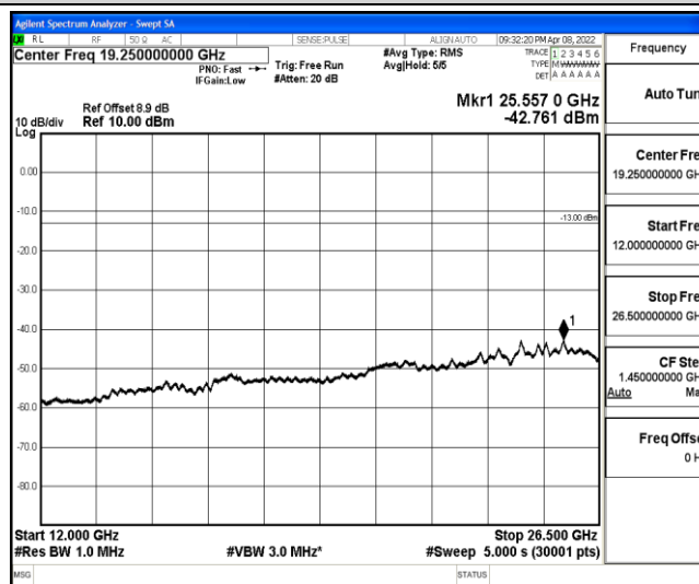
Band2-1.4MHz-16QAM-18607-1-0-Low-12000-26500--42.76-PASS
