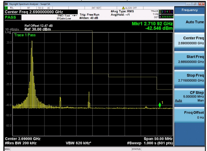
Subtest:83, Channel:41490, Bandwidth:20, Modulation:QPSK, RB Number: 1, RB Position:LOW
