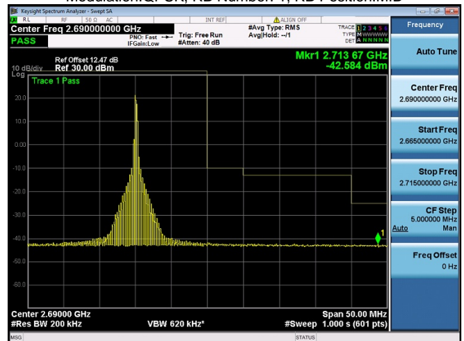
Subtest:84, Channel:41490, Bandwidth:20, Modulation:QPSK, RB Number: 1, RB Position:MID
