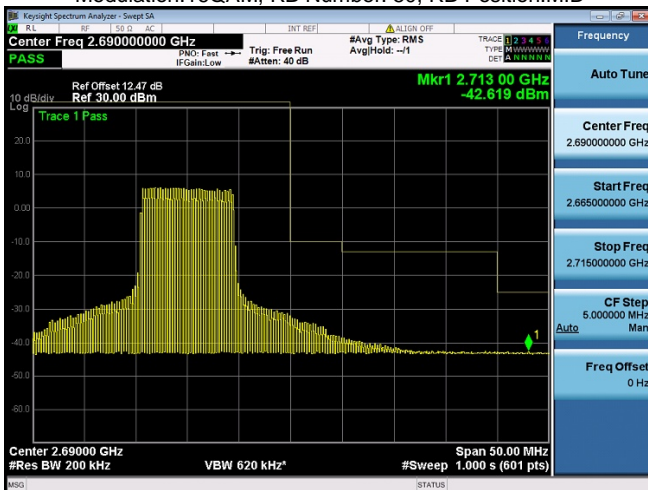
Subtest:93, Channel:41490, Bandwidth:20, Modulation:16QAM, RB Number: 50, RB Position:MID
