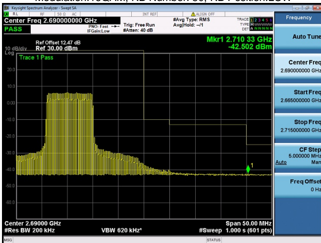
Subtest:92, Channel:41490, Bandwidth:20, Modulation:16QAM, RB Number: 50, RB Position:LOW
