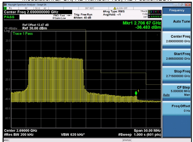
Subtest:95, Channel:41490, Bandwidth:20, Modulation:QPSK, RB Number: 100, RB Position:LOW
