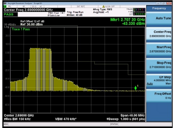
Subtest:64, Channel:41515, Bandwidth:15, Modulation:16QAM, RB Number: 36, RB Position:LOW
