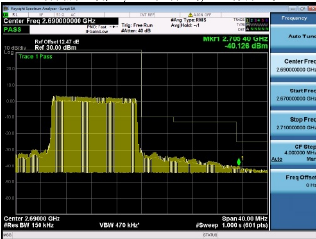
Subtest:68, Channel:41515, Bandwidth:15, Modulation:16QAM, RB Number: 75, RB Position:LOW
