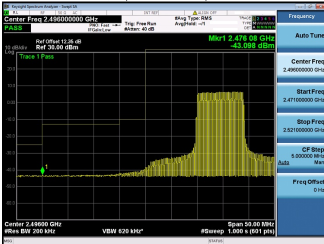
Subtest:80, Channel:39750, Bandwidth:20, Modulation:16QAM, RB Number: 50, RB Position:HIGH
