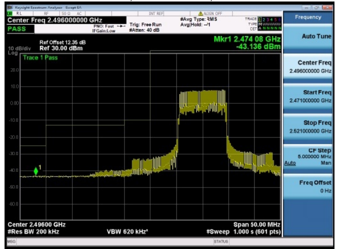
Subtest:76, Channel:39750, Bandwidth:20, Modulation:QPSK, RB Number: 50, RB Position:MID
