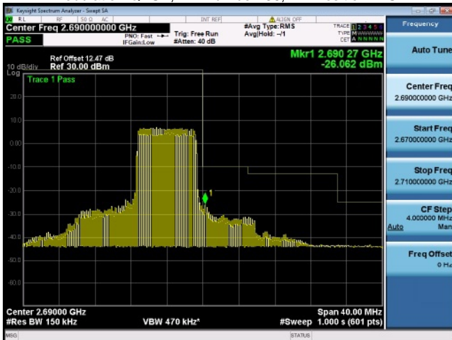
Subtest:63, Channel:41515, Bandwidth:15, Modulation:QPSK, RB Number: 36, RB Position:HIGH
