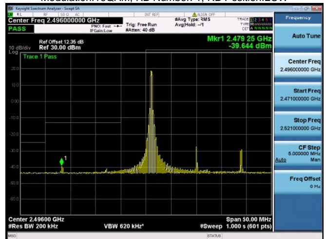
Subtest:72, Channel:39750, Bandwidth:20, Modulation:16QAM, RB Number: 1, RB Position:LOW
