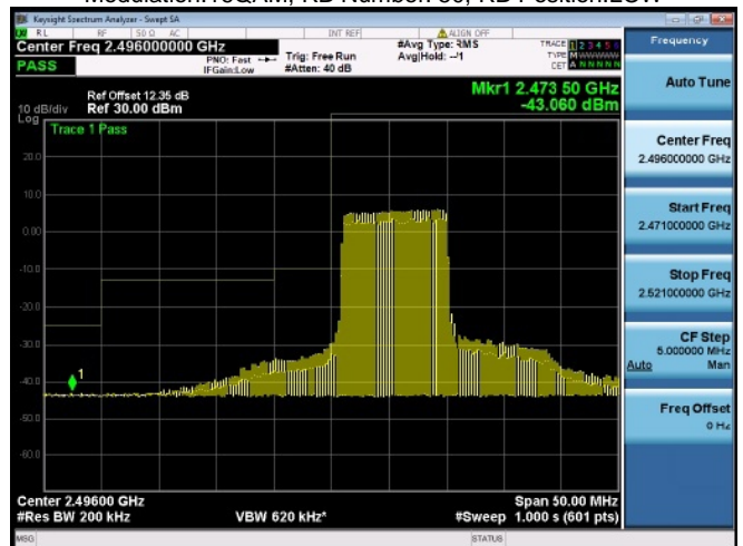
Subtest:78, Channel:39750, Bandwidth:20, Modulation:16QAM, RB Number: 50, RB Position:LOW
