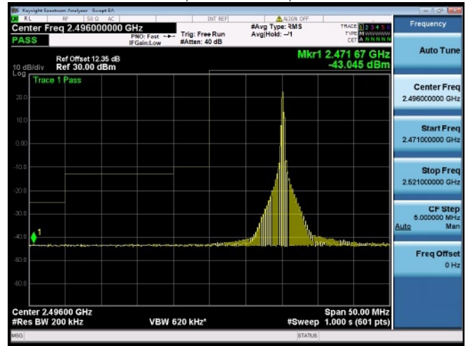
Subtest:70, Channel:39750, Bandwidth:20, Modulation:QPSK, RB Number: 1, RB Position:MID
