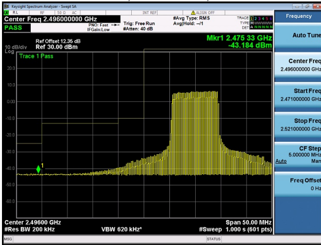
Subtest:79, Channel:39750, Bandwidth:20, Modulation:16QAM, RB Number: 50, RB Position:MID
