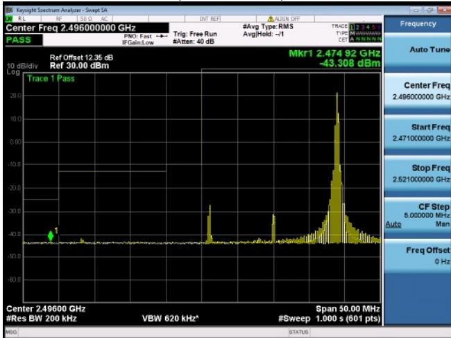
Subtest:74, Channel:39750, Bandwidth:20, Modulation:16QAM, RB Number: 1, RB Position:HIGH
