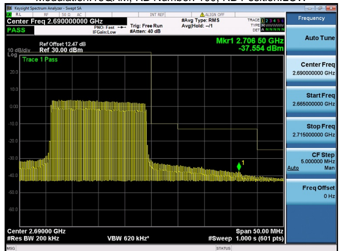
Subtest:96, Channel:41490, Bandwidth:20, Modulation:16QAM, RB Number: 100, RB Position:LOW
