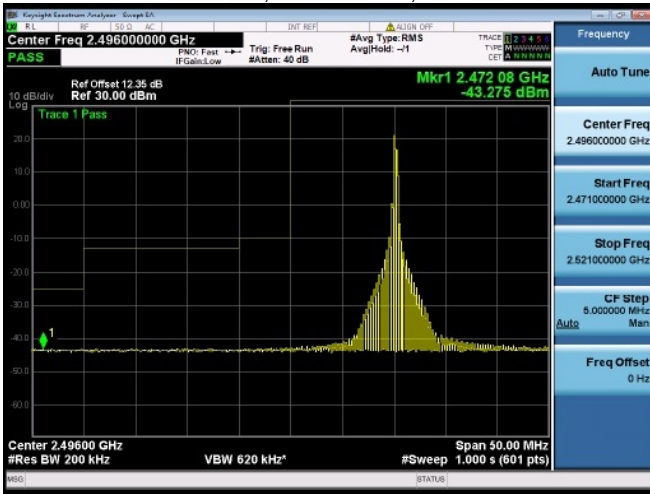
Subtest:73, Channel:39750, Bandwidth:20, Modulation:16QAM, RB Number: 1, RB Position:MID
