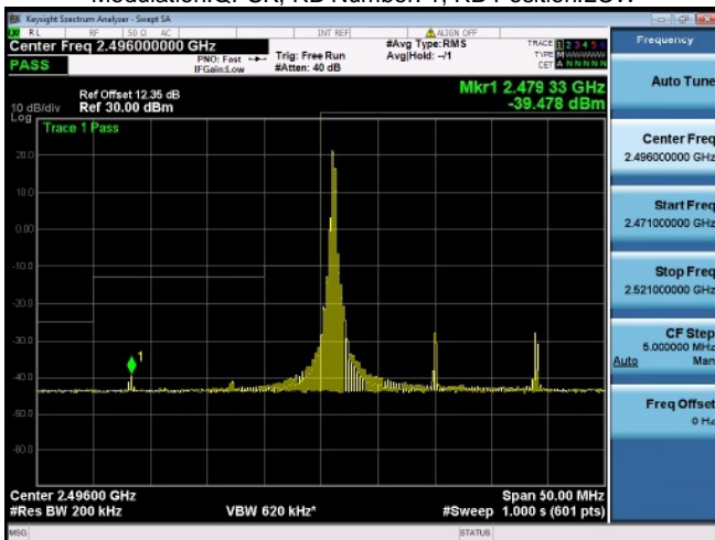
Subtest:69, Channel:39750, Bandwidth:20, Modulation:QPSK, RB Number: 1, RB Position:LOW
