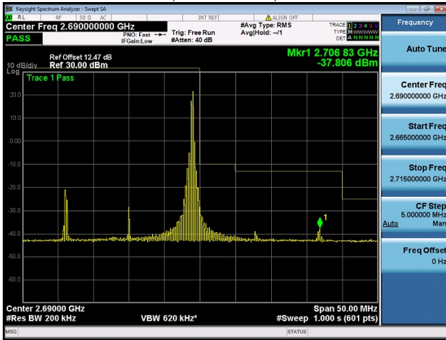
Subtest:85, Channel:41490, Bandwidth:20, Modulation:QPSK, RB Number: 1, RB Position:HIGH
