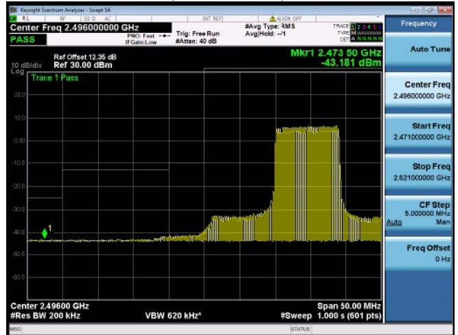
Subtest:77, Channel:39750, Bandwidth:20, Modulation:QPSK, RB Number: 50, RB Position:HIGH
