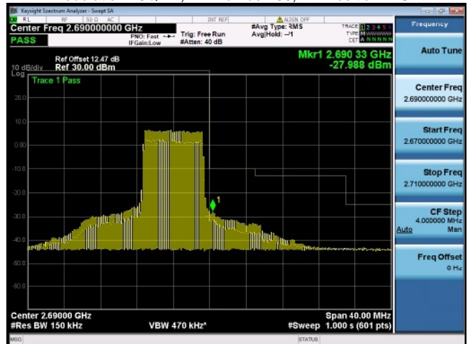
Subtest:66, Channel:41515, Bandwidth:15, Modulation:16QAM, RB Number: 36, RB Position:HIGH
