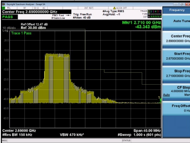
Subtest:62, Channel:41515, Bandwidth:15, Modulation:QPSK, RB Number: 36, RB Position:MID
