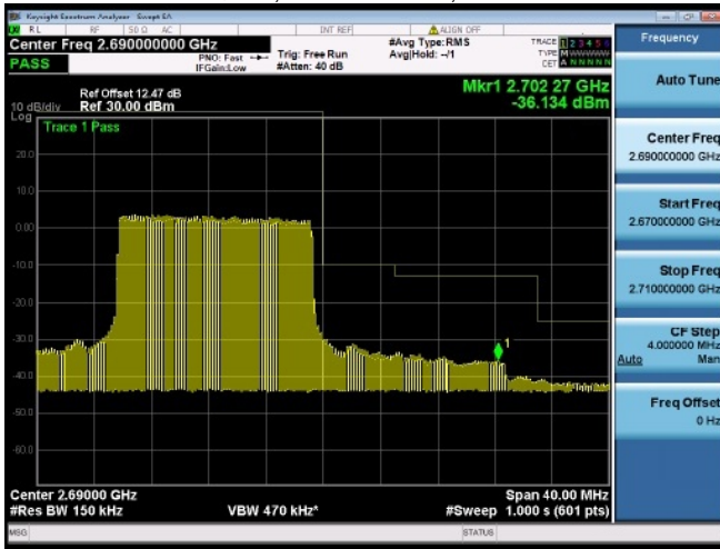
Subtest:67, Channel:41515, Bandwidth:15, Modulation:QPSK, RB Number: 75, RB Position:LOW
