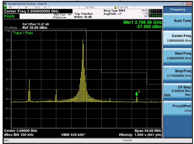
Subtest:88, Channel:41490, Bandwidth:20, Modulation:16QAM, RB Number: 1, RB Position:HIGH
