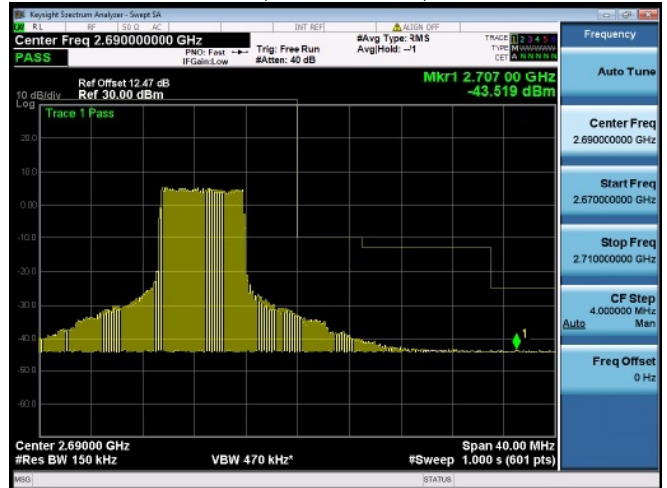
Subtest:65, Channel:41515, Bandwidth:15, Modulation:16QAM, RB Number: 36, RB Position:MID
