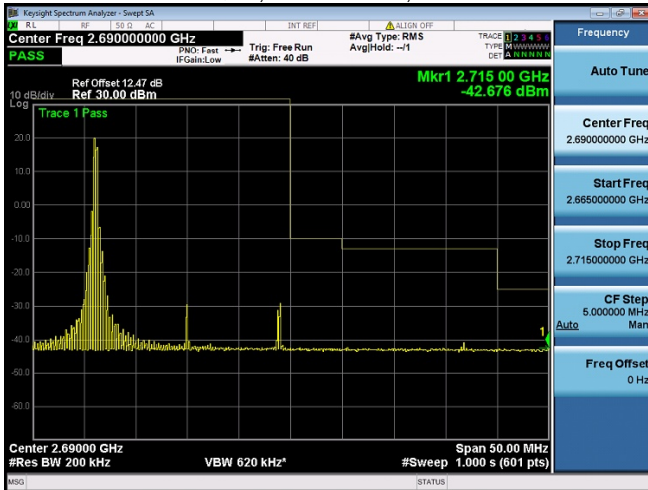
Subtest:86, Channel:41490, Bandwidth:20, Modulation:16QAM, RB Number: 1, RB Position:LOW
