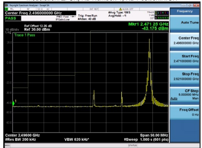
Subtest:71, Channel:39750, Bandwidth:20, Modulation:QPSK, RB Number: 1, RB Position:HIGH
