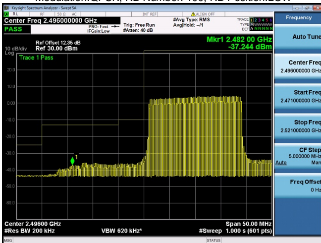
Subtest:81, Channel:39750, Bandwidth:20, Modulation:QPSK, RB Number: 100, RB Position:LOW
