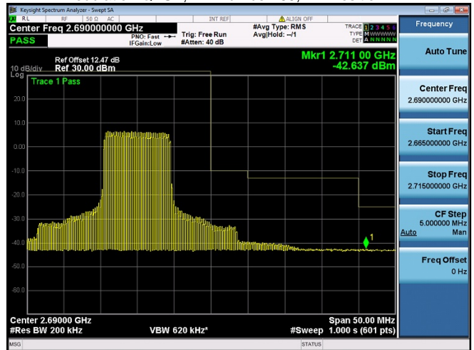
Subtest:90, Channel:41490, Bandwidth:20, Modulation:QPSK, RB Number: 50, RB Position:MID
