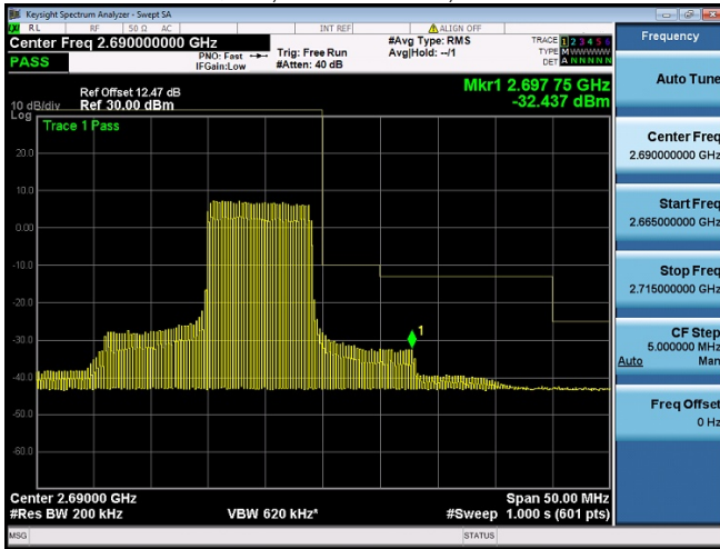
Subtest:91, Channel:41490, Bandwidth:20, Modulation:QPSK, RB Number: 50, RB Position:HIGH
