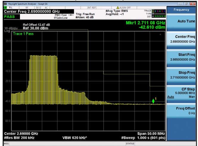
Subtest:89, Channel:41490, Bandwidth:20, Modulation:QPSK, RB Number: 50, RB Position:LOW
