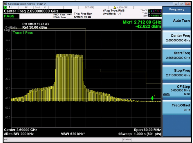
Subtest:94, Channel:41490, Bandwidth:20, Modulation:16QAM, RB Number: 50, RB Position:HIGH
