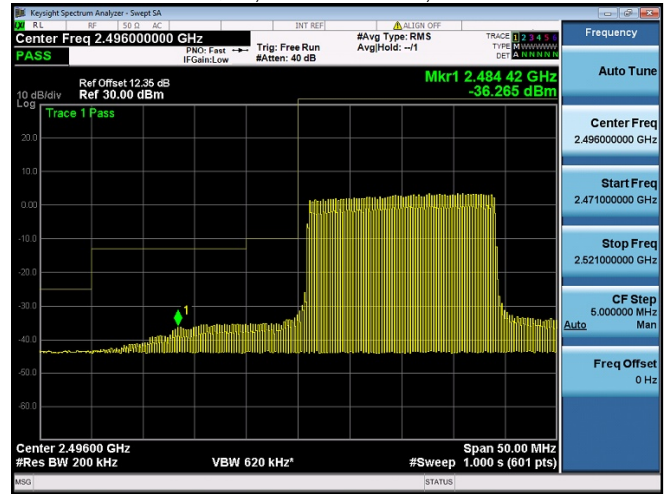
Subtest:82, Channel:39750, Bandwidth:20, Modulation:16QAM, RB Number: 100, RB Position:LOW
