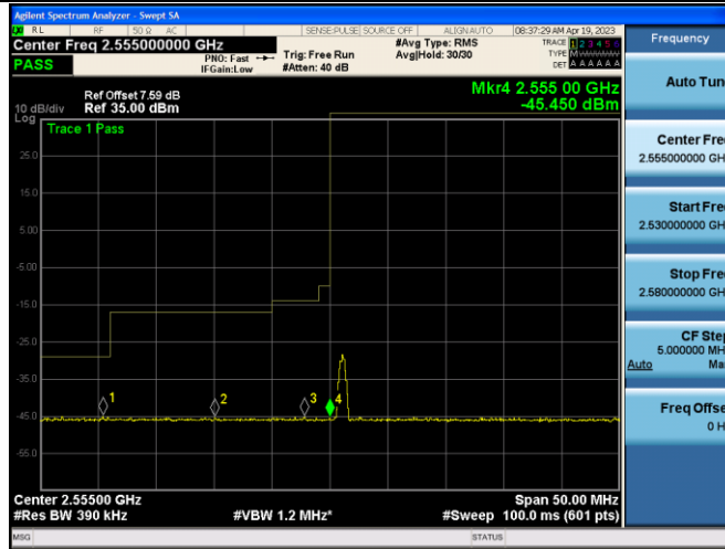
Band41-20MHz-16QAM-40340-1RB#99
