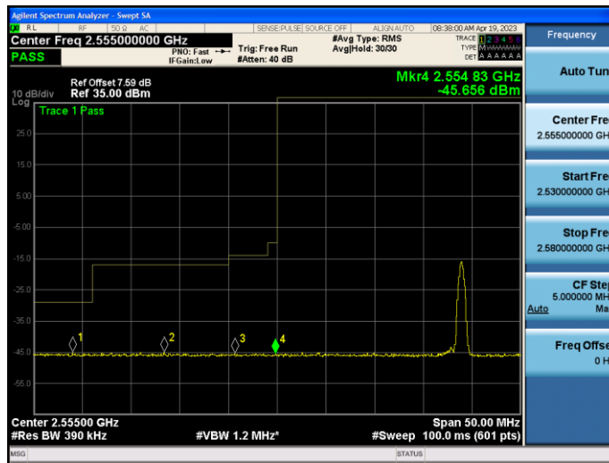
Band41-20MHz-16QAM-40340-100RB#0
