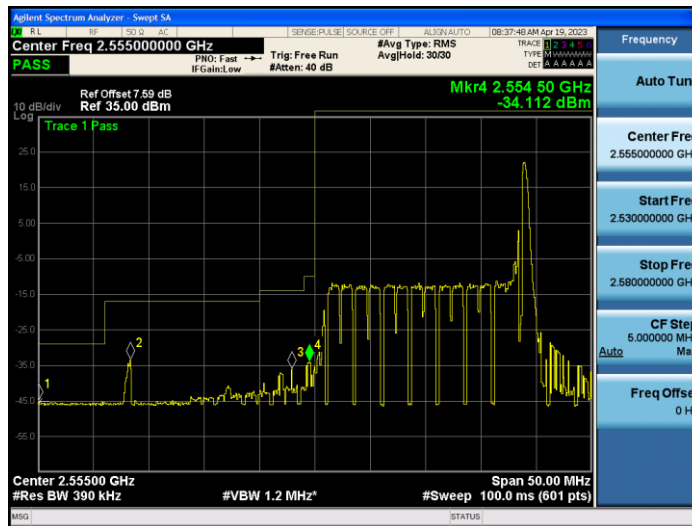
Band41-20MHz-QPSK-40340-100RB#0
