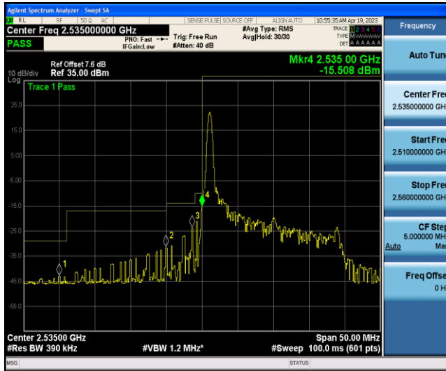
Band41-20MHz-16QAM-40140-1RB#99
