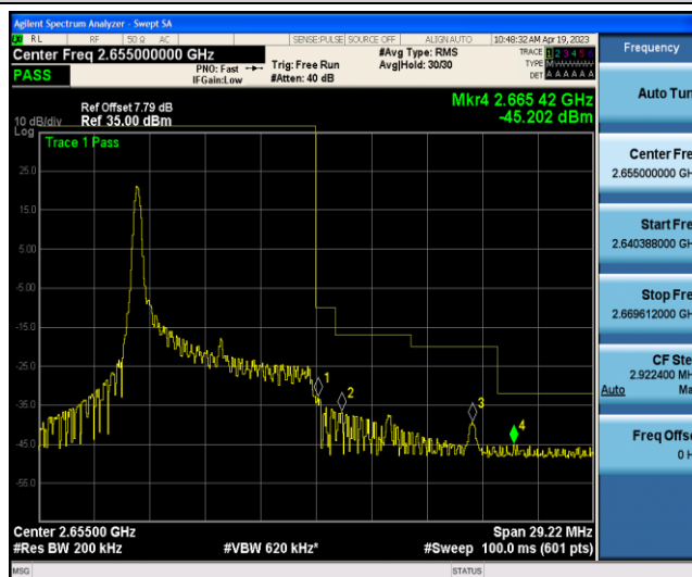
Band41-10MHz-16QAM-41190-1RB#49
