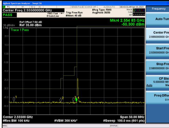
Band41-5MHz-16QAM-40265-1RB#24
