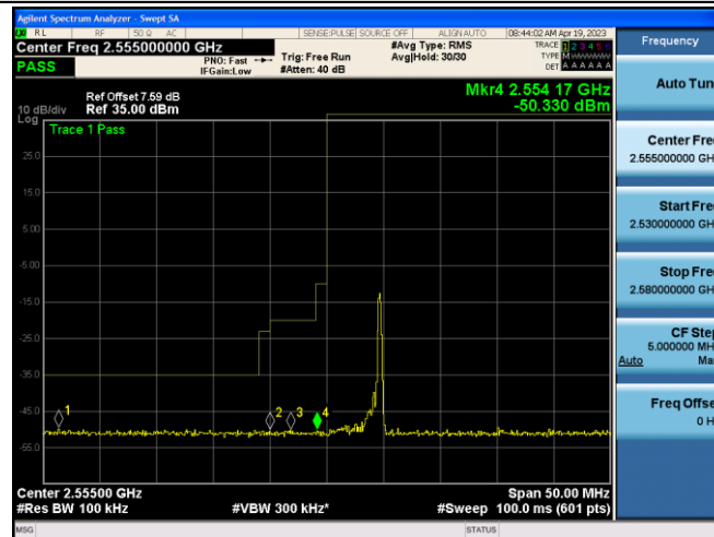
Band41-5MHz-16QAM-40265-25RB#0
