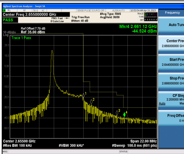
Band41-5MHz-QPSK-41215-1RB#24
