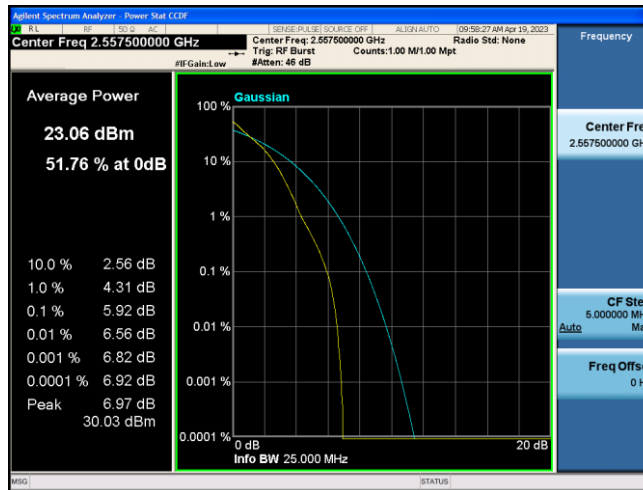
Band41-5MHz-16QAM-40265-25RB#0
