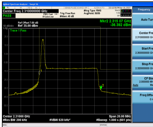
Band40-10MHz-QPSK-38750-1RB#49
