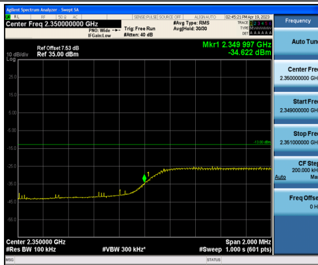
Band40-5MHz-QPSK-39175-25RB#0
