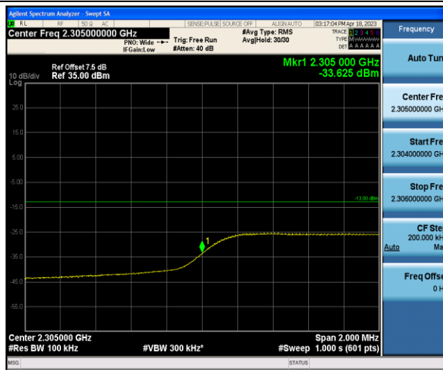
Band40-5MHz-16QAM-38725-25RB#0
