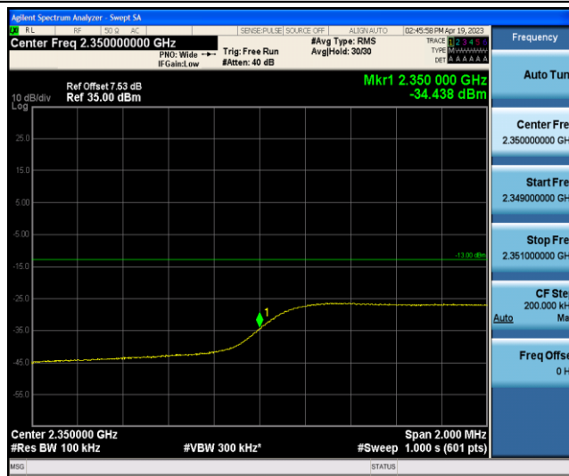
Band40-5MHz-16QAM-39175-25RB#0
