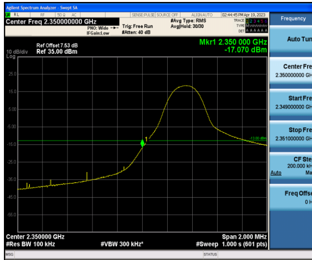
Band40-5MHz-16QAM-39175-1RB#24
