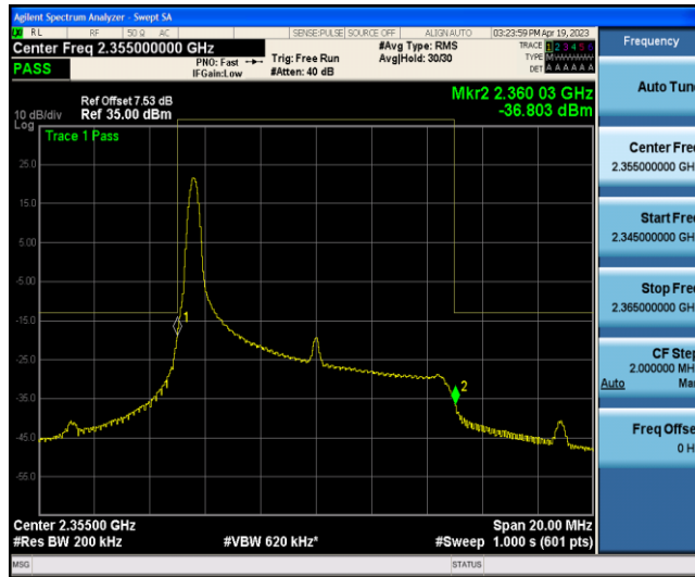
Band40-10MHz-QPSK-39200-1RB#49
