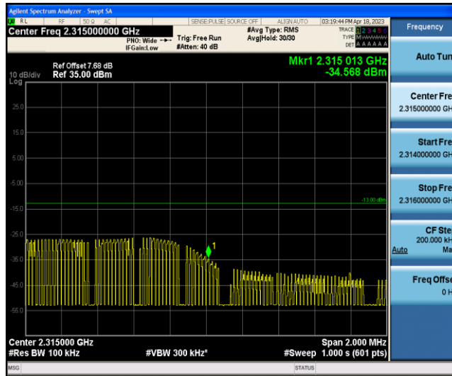
Band40-5MHz-16QAM-38775-1RB#24
