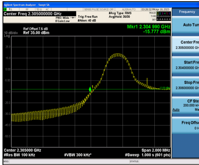
Band40-5MHz-16QAM-38725-1RB#24
