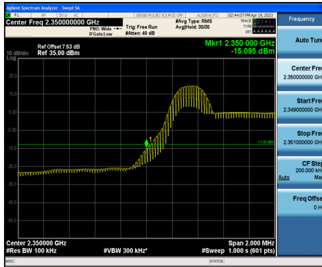
Band40-5MHz-QPSK-39175-1RB#24
