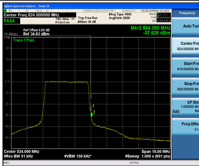
Band26-3MHz-16QAM-26805-1RB#0
