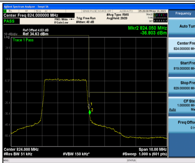
Band26-3MHz-QPSK-26805-1RB#0
