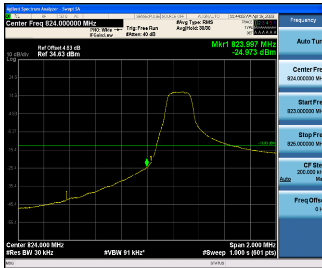
Band26-1.4MHz-QPSK-26797-1RB#5
