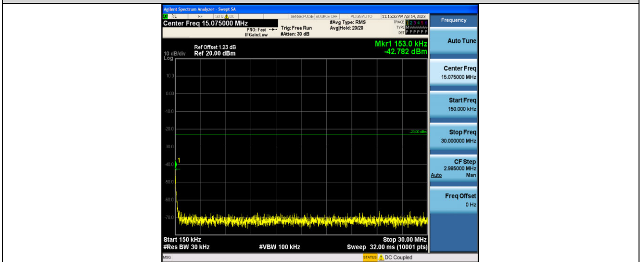
GPRS1900-512-0.15~30MHz
