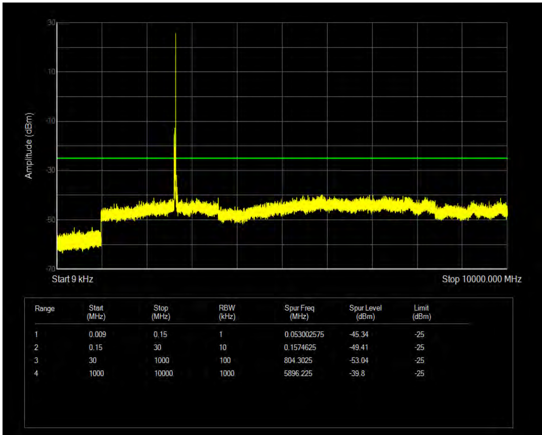
Band41(2555-2655) QAM16 BW=20MHz Channel=41140 RB Size=50 Position=#0
