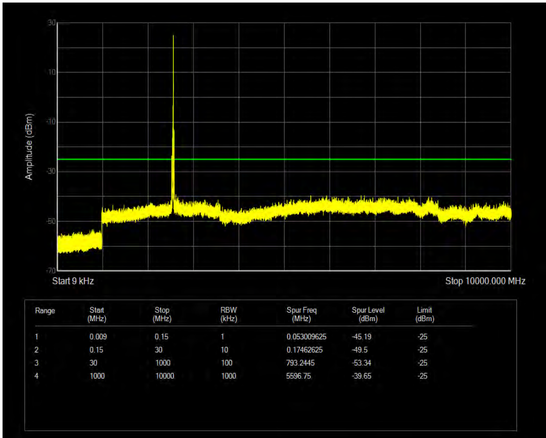
Band41(2555-2655) QAM16 BW=20MHz Channel=40340 RB Size=50 Position=#0
