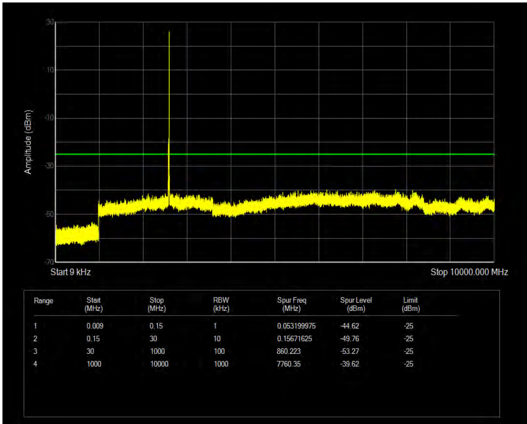
Band41(2555-2655) QAM16 BW=10MHz Channel=40740 RB Size=25 Position=#Max
