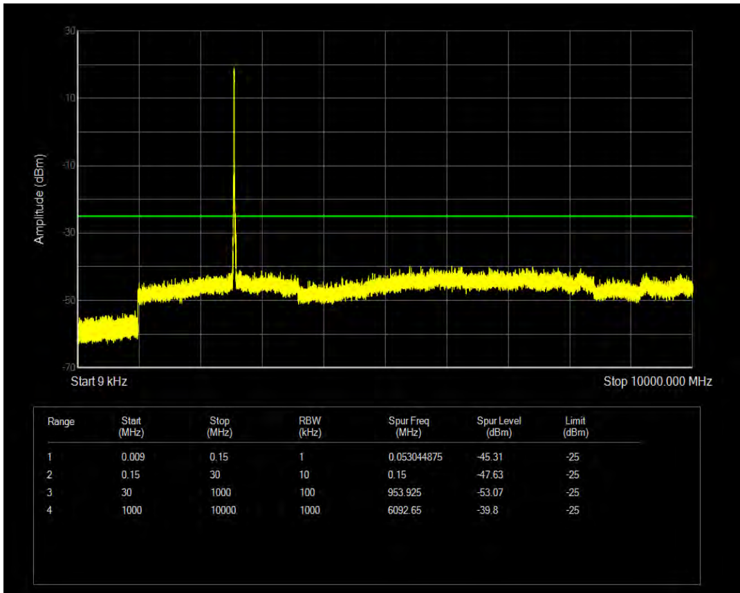
Band41(2555-2655) QAM16 BW=20MHz Channel=40340 RB Size=50 Position=#0
