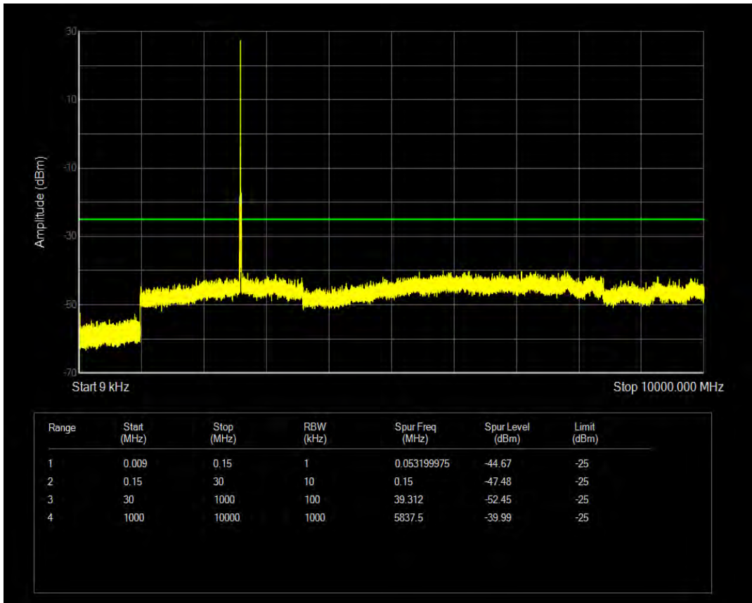
Band41(2555-2655) QPSK BW=10MHz Channel=40740 RB Size=1 Position=#Max
