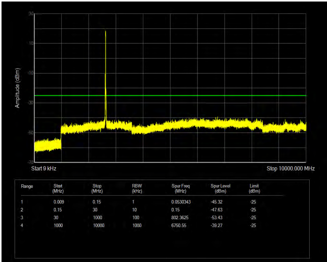
Band41(2555-2655) QAM16 BW=20MHz Channel=41140 RB Size=50 Position=#0
