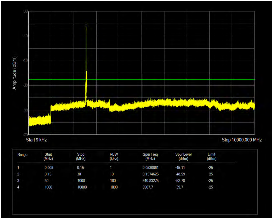
Band41(2555-2655) QPSK BW=20MHz Channel=40340 RB Size=50 Position=#Max
