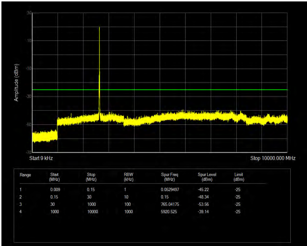
Band41(2555-2655) QAM16 BW=15MHz Channel=41165 RB Size=36 Position=#Max
