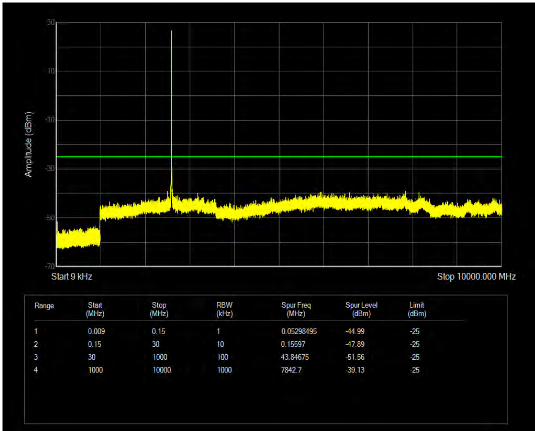
Band41(2555-2655) QPSK BW=20MHz Channel=40740 RB Size=1 Position=#Max
