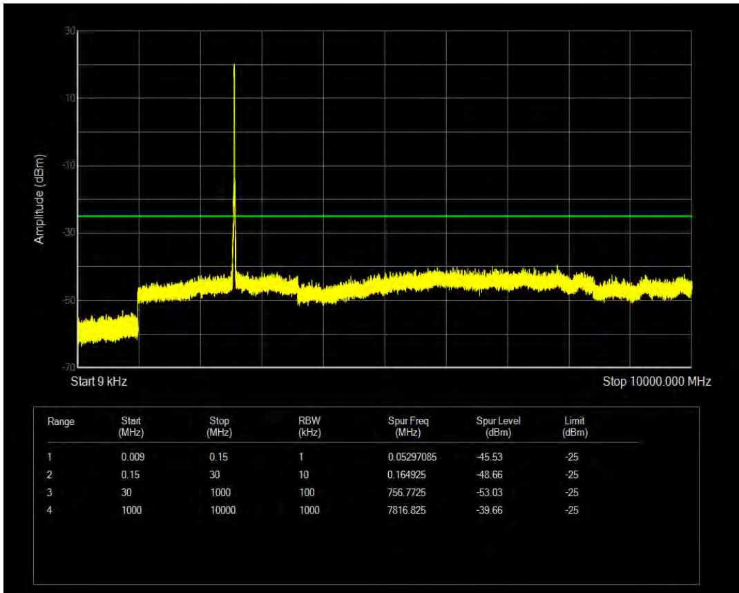
Band41(2555-2655) QPSK BW=20MHz Channel=40340 RB Size=50 Position=#Max
