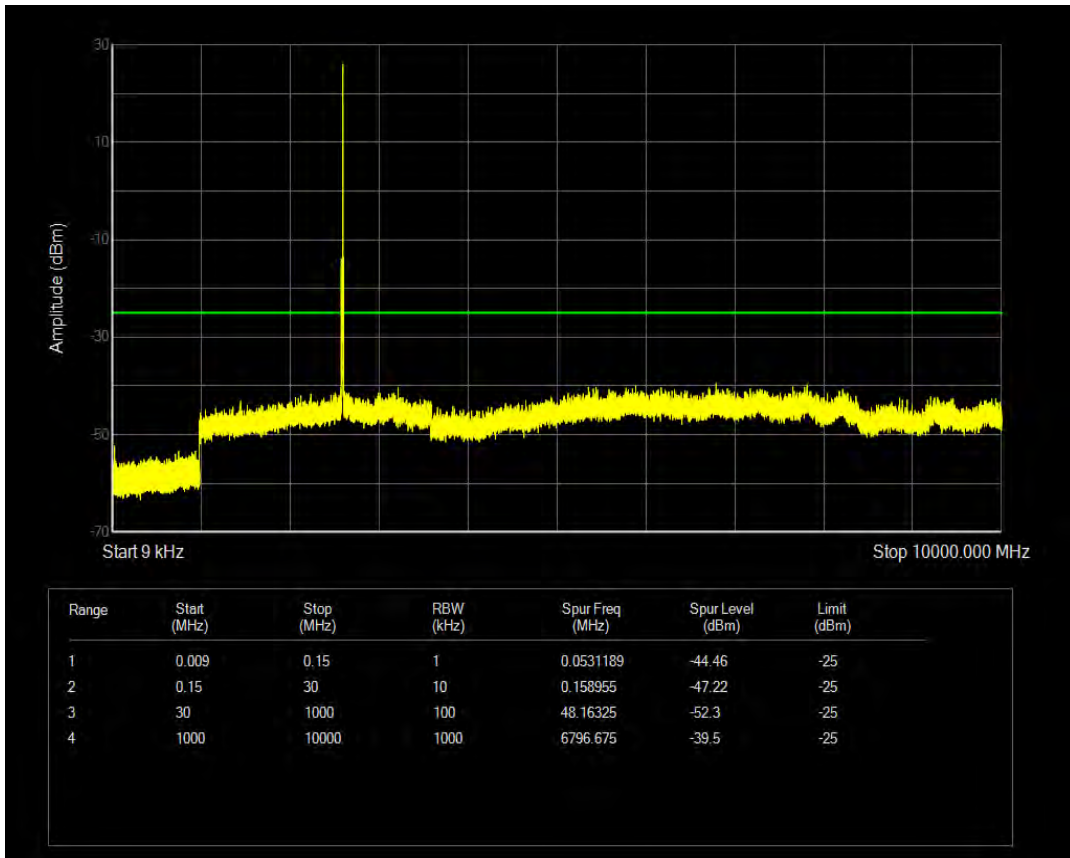
Band41(2555-2655) QPSK BW=10MHz Channel=40740 RB Size=1 Position=#Max
