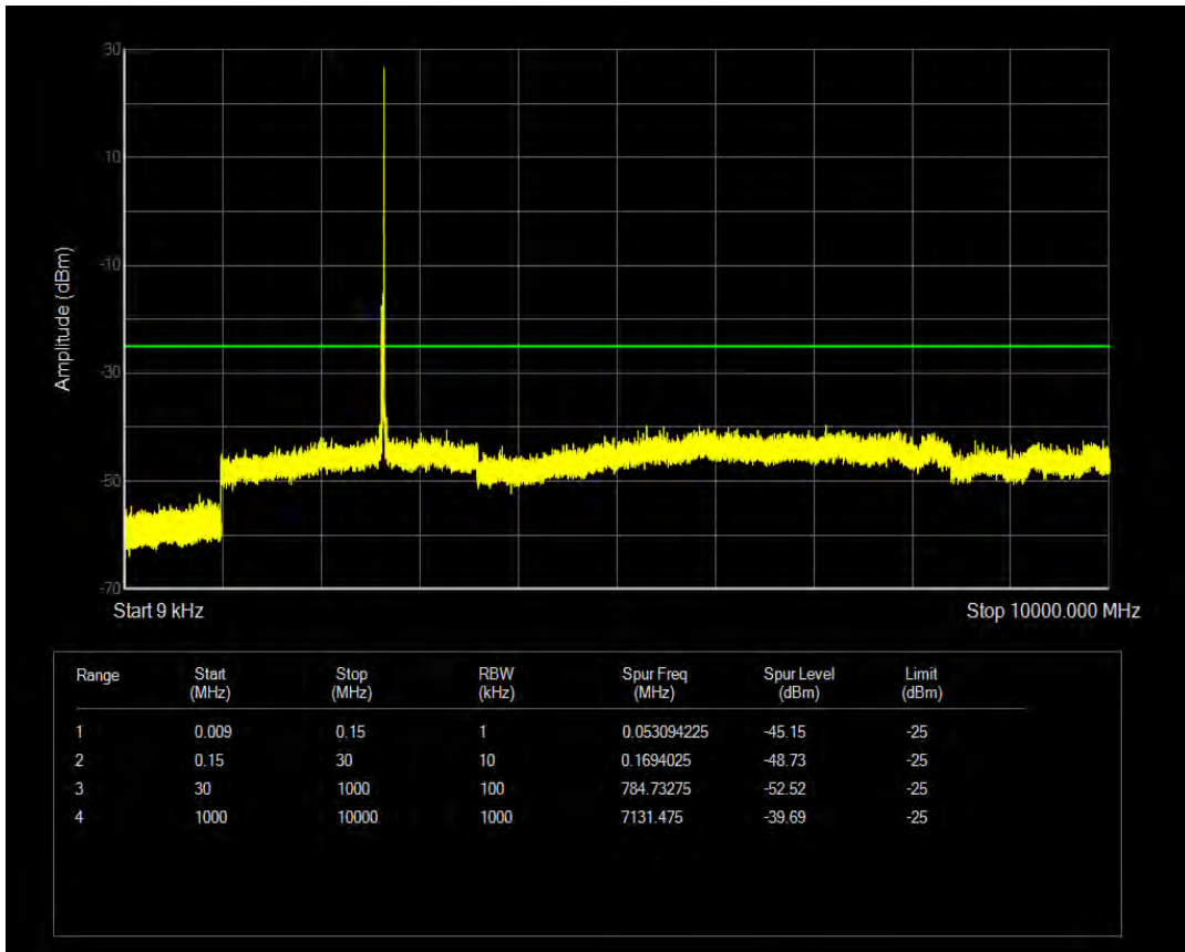
Band41(2555-2655) QAM16 BW=15MHz Channel=41165 RB Size=36 Position=#Max
