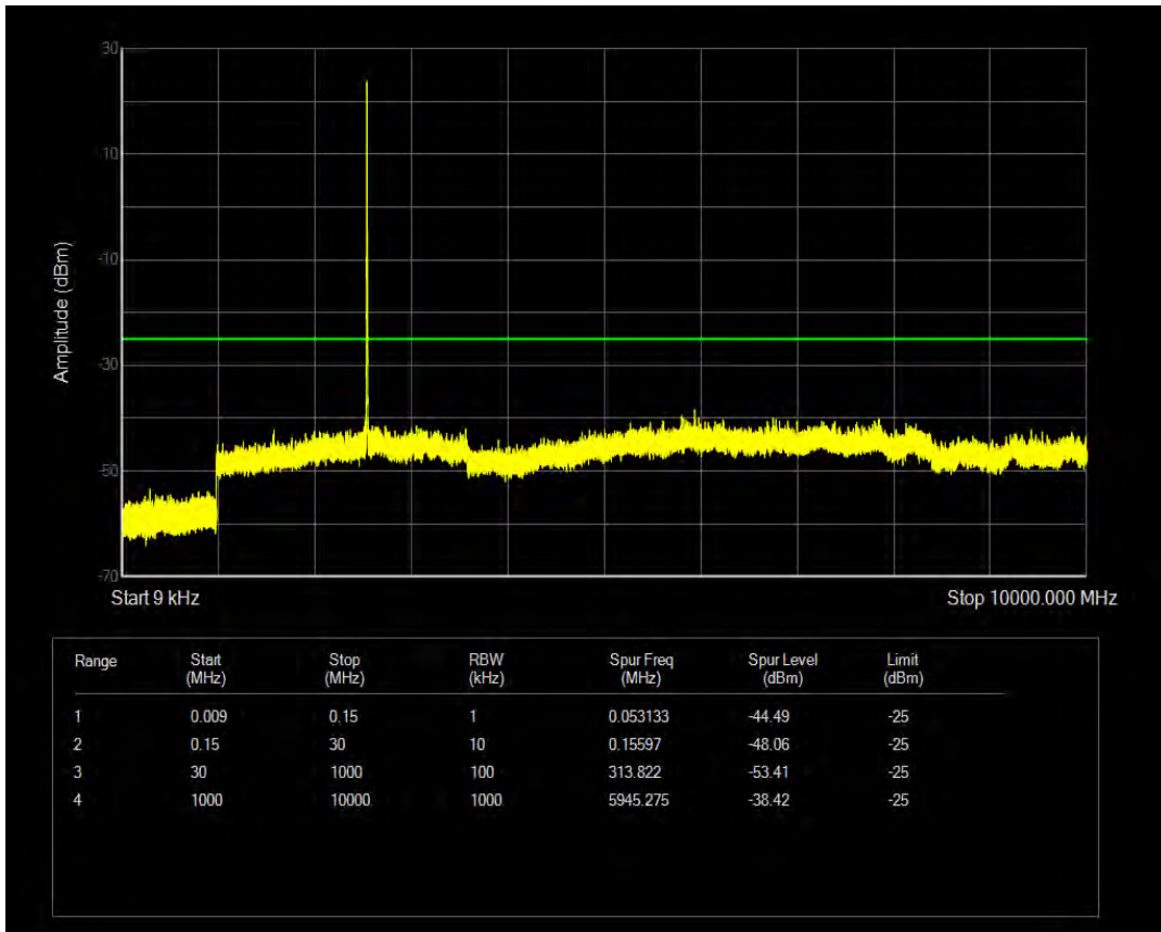
Band41(2555-2655) QPSK BW=5MHz Channel=40265 RB Size=12 Position=#Max
