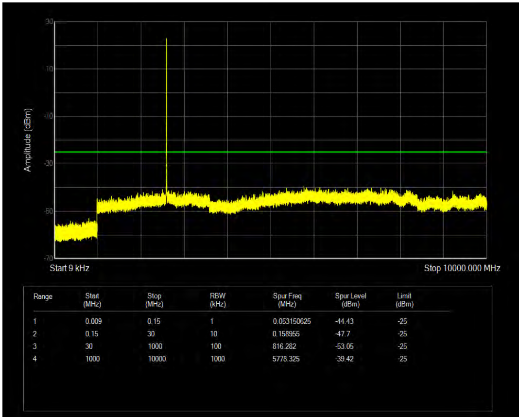
Band41(2555-2655) QPSK BW=5MHz Channel=40740 RB Size=12 Position=#Max
