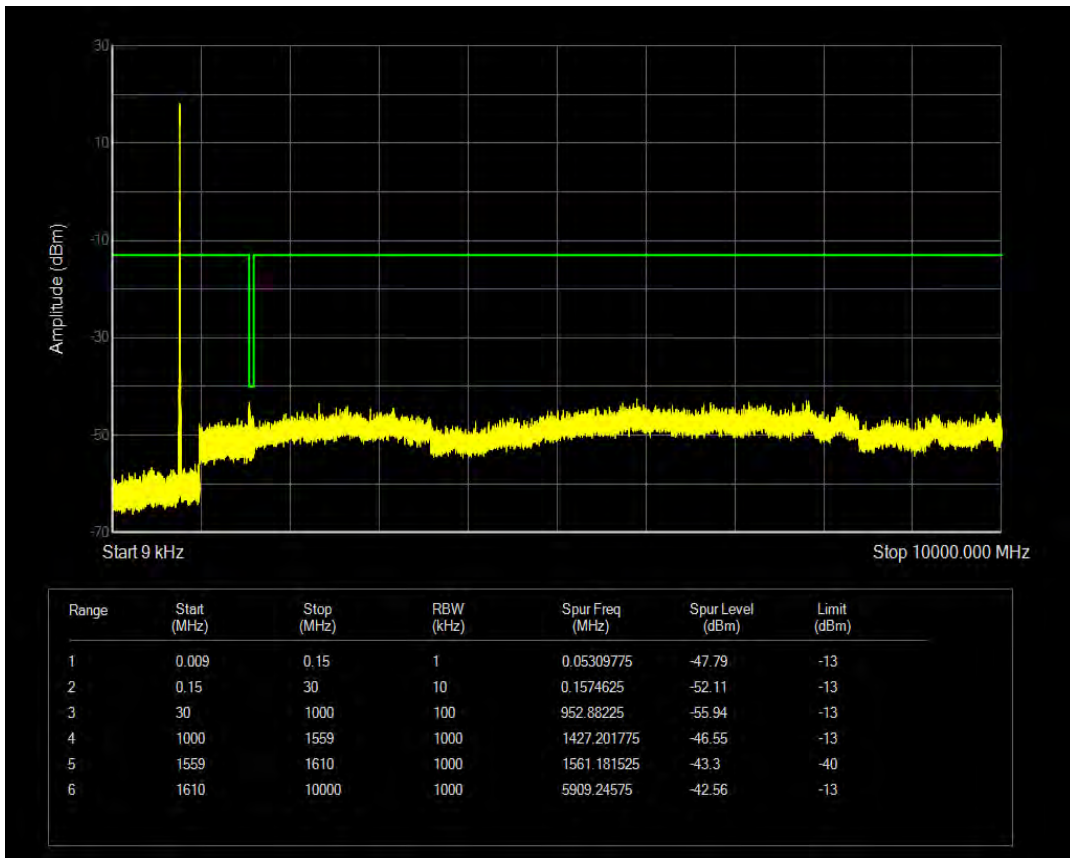
Band13 QPSK BW=5MHz Channel=23230 RB Size=12 Position=#Max
