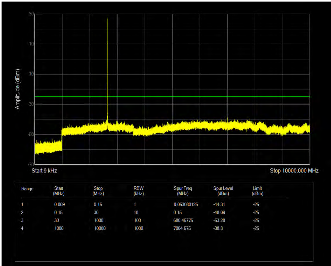
Band41(2555-2655) QAM16 BW=5MHz Channel=41215 RB Size=12 Position=#0
