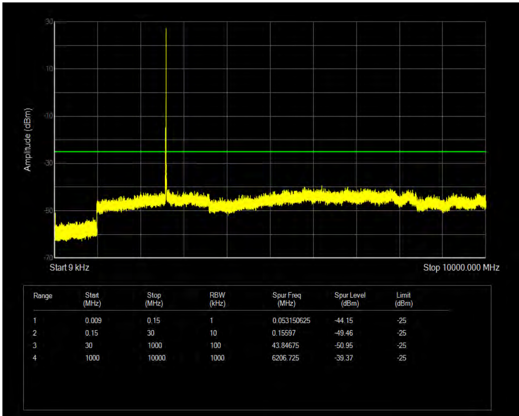
Band41(2555-2655) QPSK BW=10MHz Channel=40740 RB Size=1 Position=#Mid
