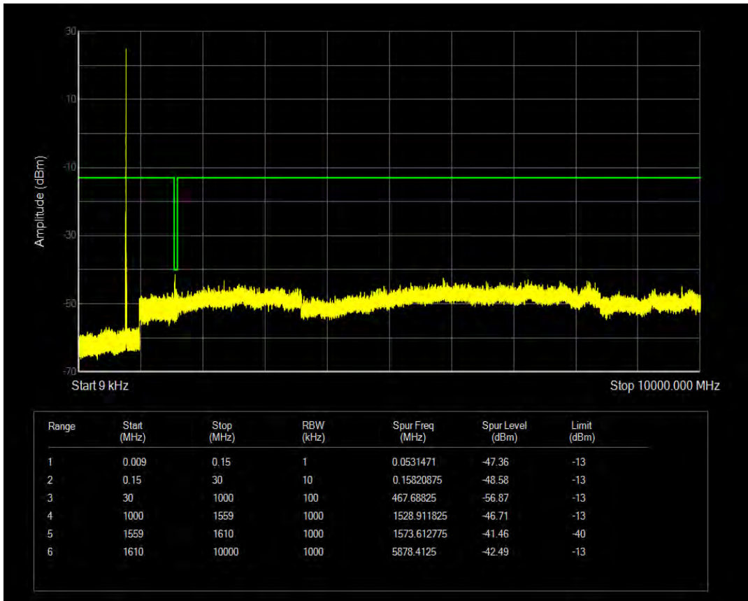
Band13 QAM16 BW=5MHz Channel=23255 RB Size=12 Position=#0
