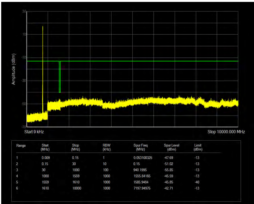
Band13 QAM16 BW=5MHz Channel=23205 RB Size=12 Position=#Max
