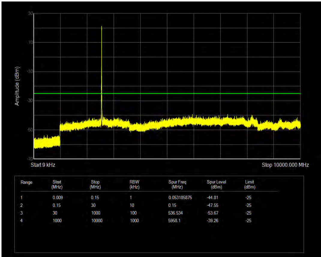
Band41(2555-2655) QPSK BW=10MHz Channel=40740 RB Size=1 Position=#Mid
