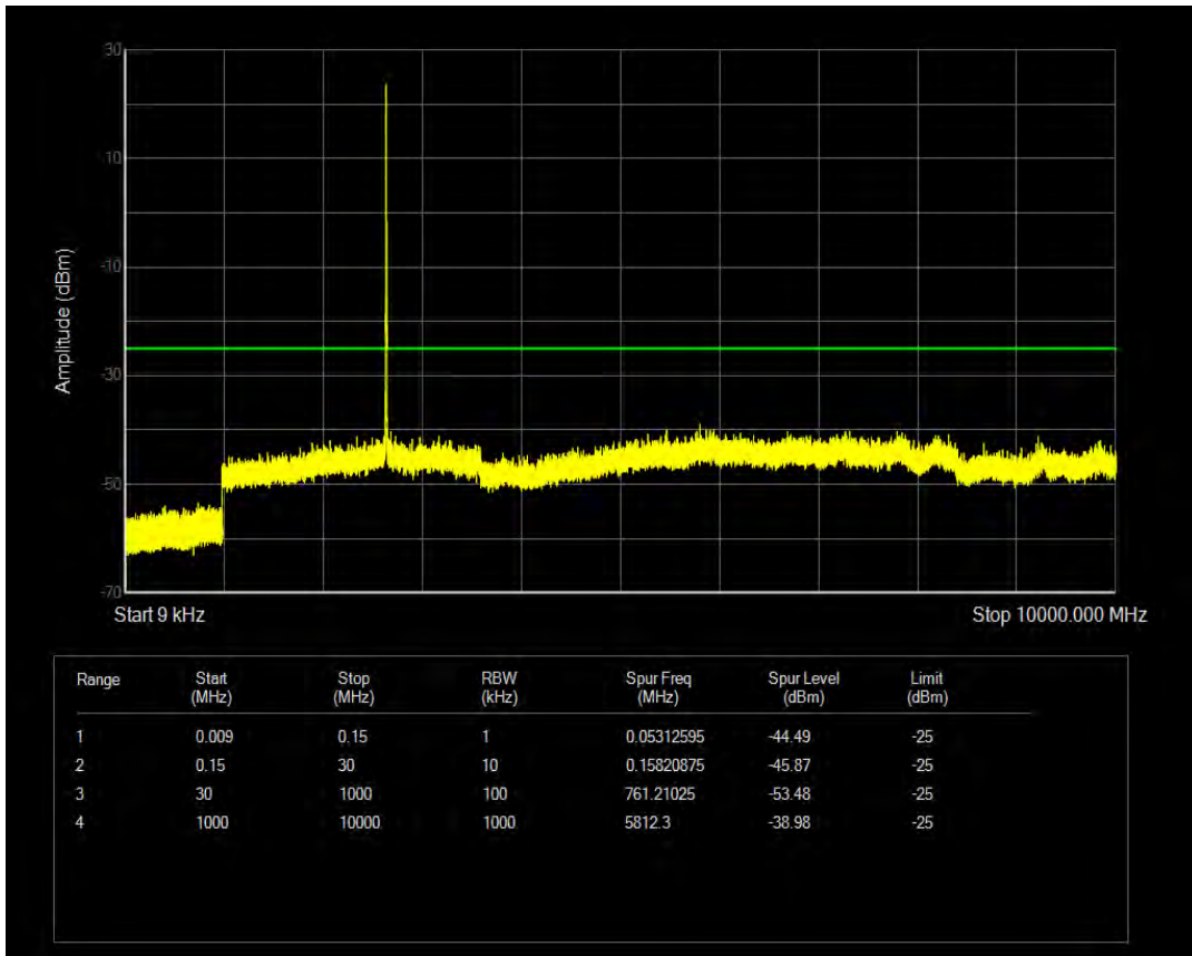
Band41(2555-2655) QAM16 BW=5MHz Channel=41215 RB Size=12 Position=#0
