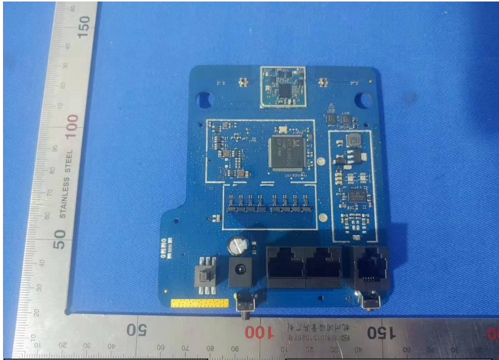
WIFI antenne 2 TX 2.4&5G
