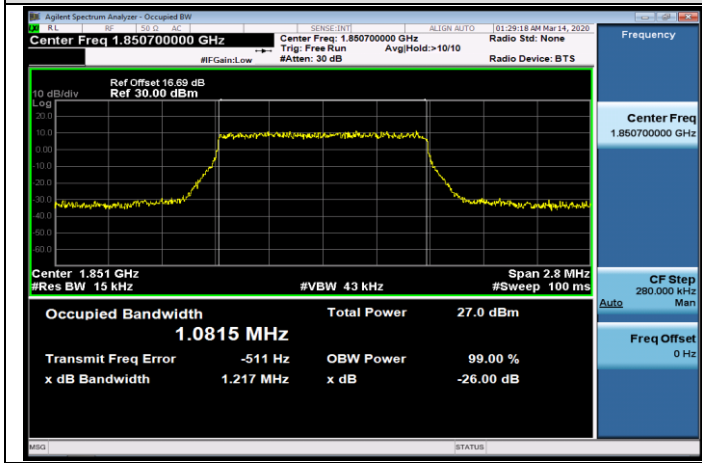
LCH_QPSK_6RB#0
