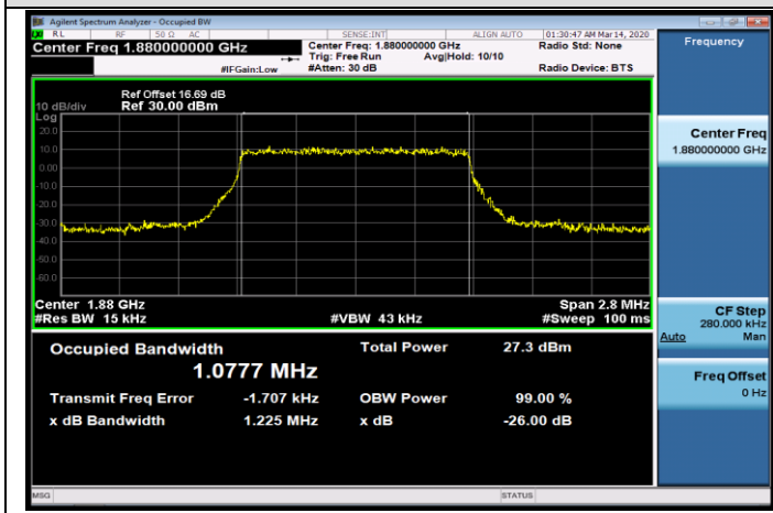
MCH_QPSK_6RB#0
