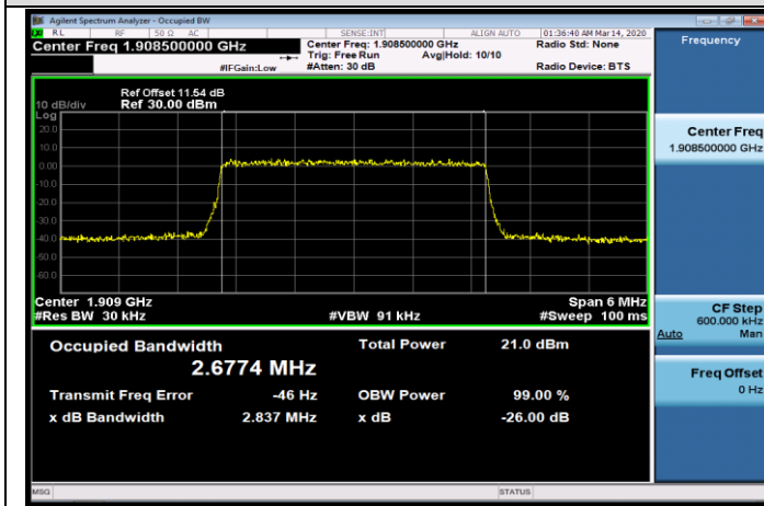
HCH_QPSK_15RB#0
