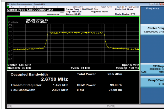
MCH_QPSK_15RB#0
