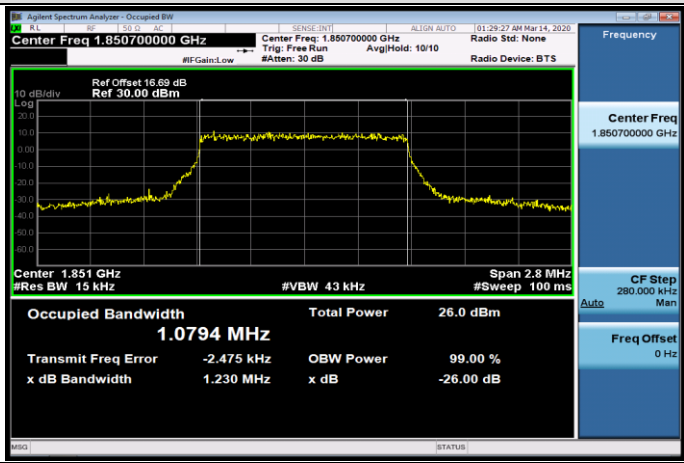
LCH_16QAM_6RB#0
