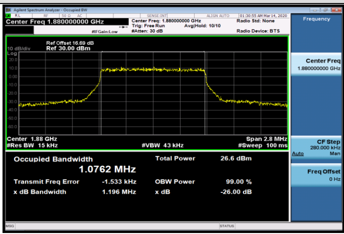
MCH_16QAM_6RB#0
