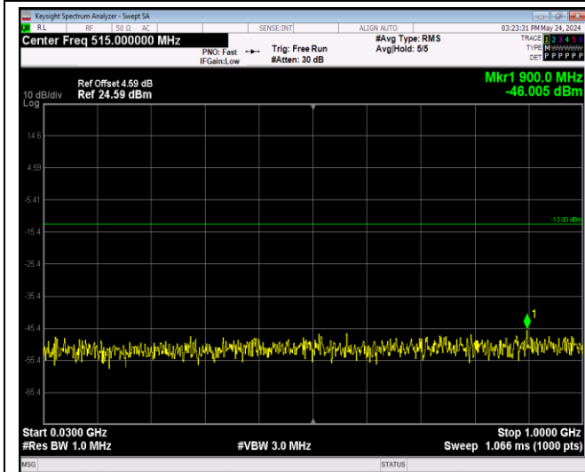
Band66-20MHz-64QAM-132572-1RB#0-Range1:30~1000MHz
