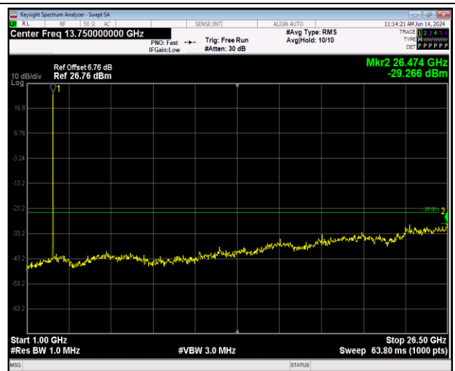
Band41-20MHz-16QAM-41490-1RB#0-Range2:1000~26500MHz
