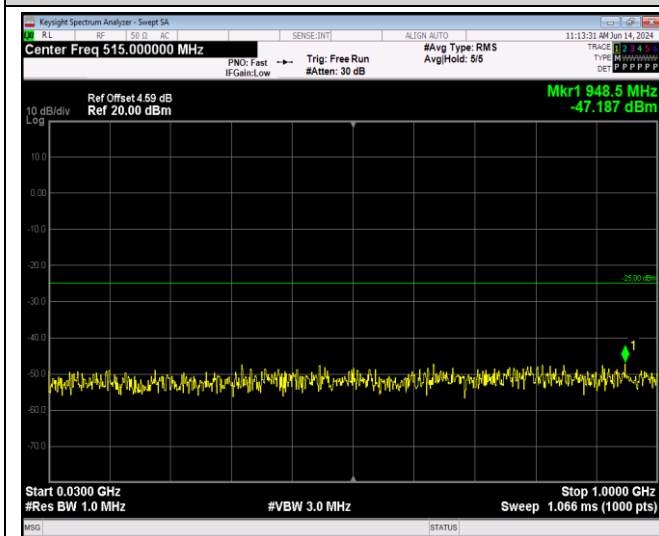
Band41-20MHz-64QAM-39750-1RB#0-Range1:30~1000MHz
