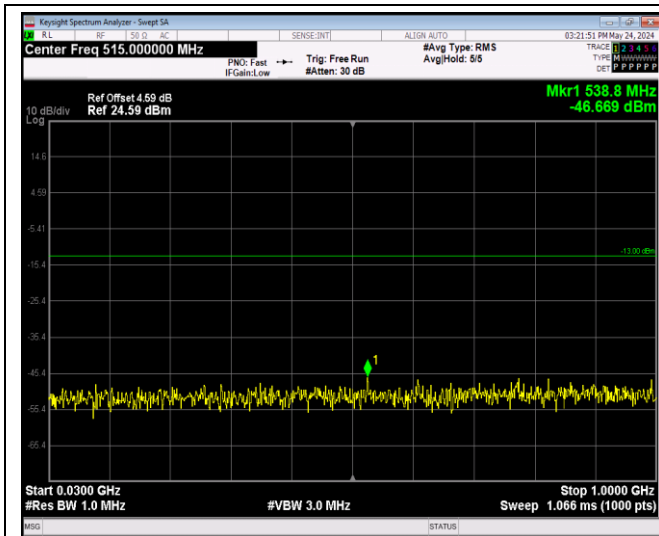
Band66-20MHz-64QAM-132322-1RB#0-Range1:30~1000MHz
