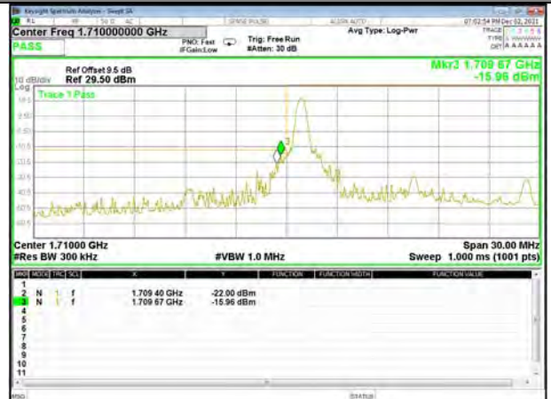
Band 66_15M_QPSK_Low_1-RB
