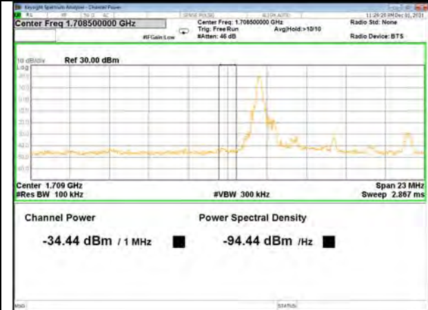
Band 4_5M_QPSK_Low_Full-RB
