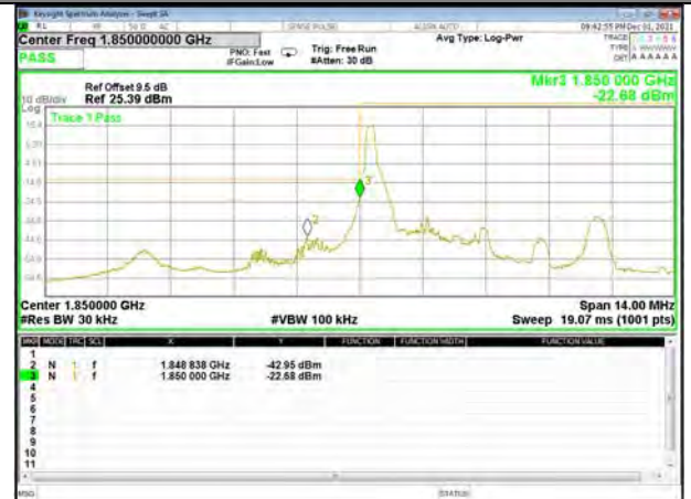
Band 2_3M_QPSK_Low_1-RB
