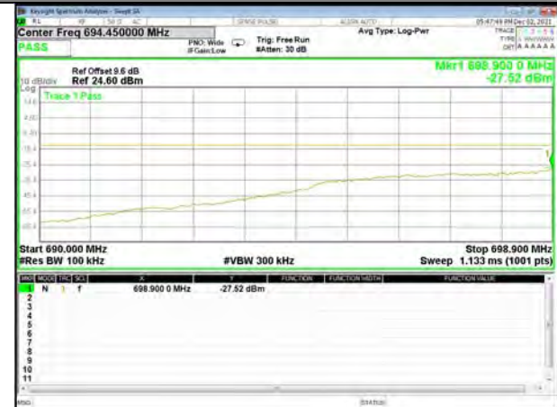
Band 12_5M_QPSK_Low_Full-RB
