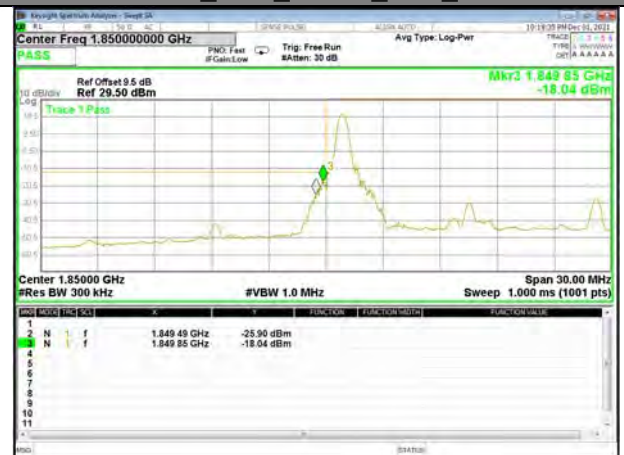
Band 2_15M_QPSK_Low_1-RB
