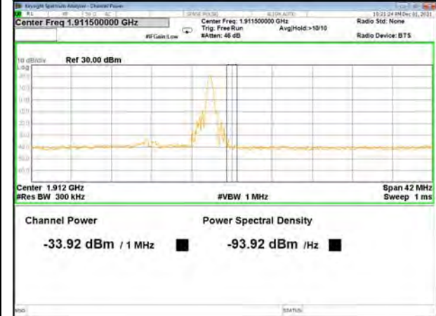
Band 2_15M_QPSK_High_Full-RB
