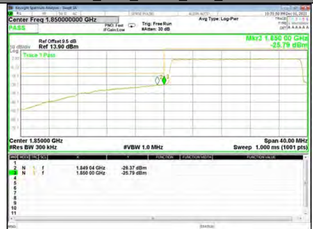
Band 2_20M_QPSK_Low_Full-RB
