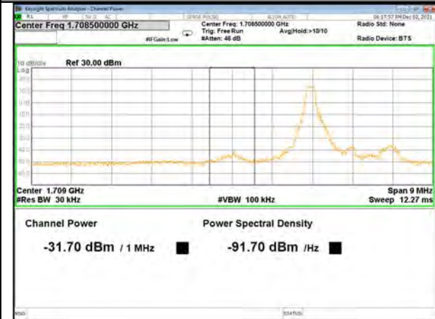
Band 66_1.4M_16QAM_Low_Full-RB
