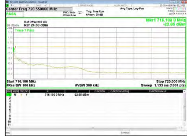
Band 12_1.4M_16QAM_High_Full-RB
