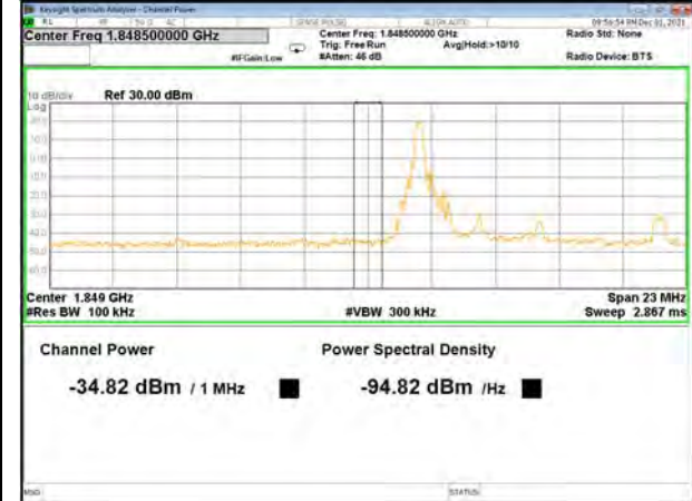
Band 2_5M_QPSK_Low_Full-RB
