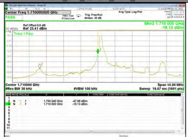
Band 4_3M_QPSK_Low_1-RB
