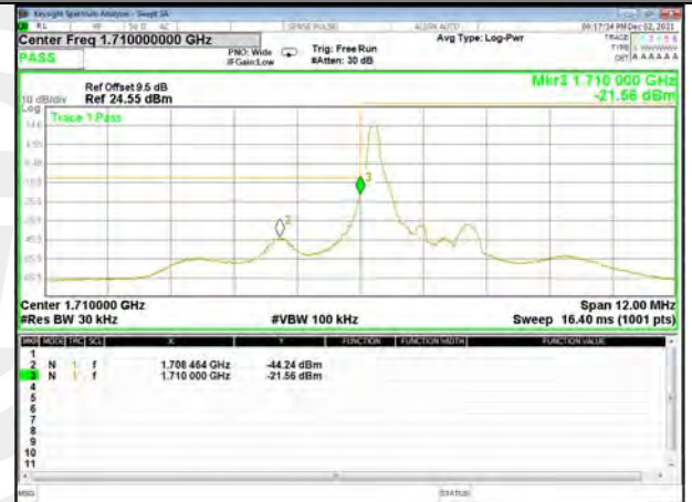
Band 66_1.4M_16QAM_Low_Full-RB
