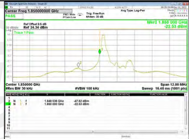
Band 2_1.4M_16QAM_Low_Full-RB
