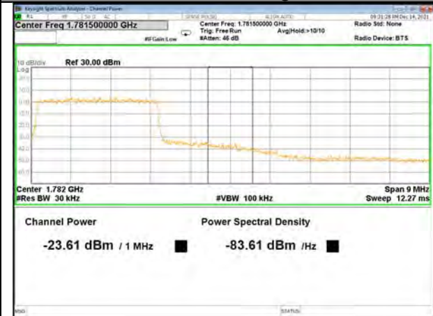
Band 66_3M_QPSK_High_Full-RB
