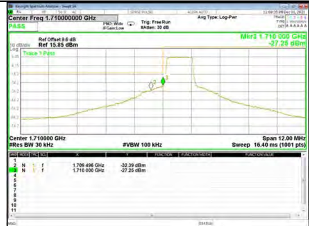
Band 4_1.4M_16QAM_Low_Full-RB
