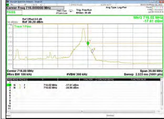
Band 12_10M_16QAM_High_1-RB
