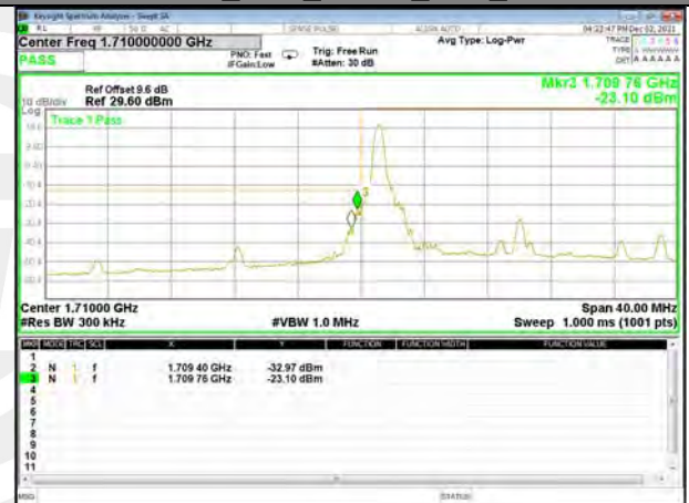
Band 4_20M_QPSK_Low_Full-RB
