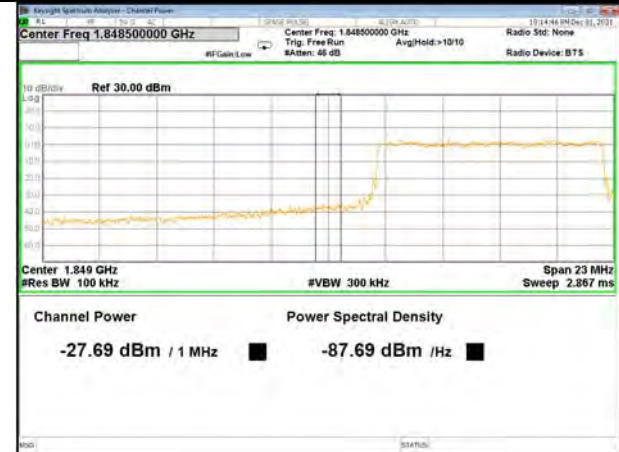
Band 2_10M_16QAM_Low_Full-RB
