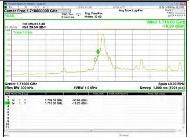
Band 66_20M_16QAM_Low_1-RB
