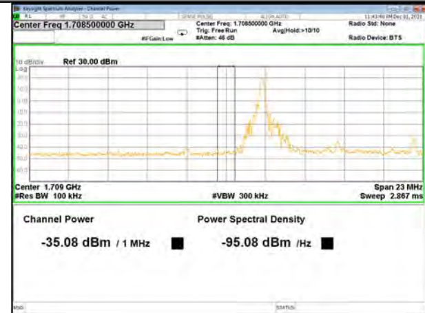
Band 4_10M_16QAM_Low_Full-RB
