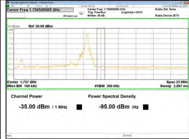
Band 4_5M_QPSK_High_Full-RB
