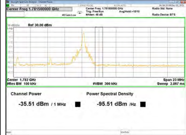
Band 66_10M_16QAM_High_Full-RB
