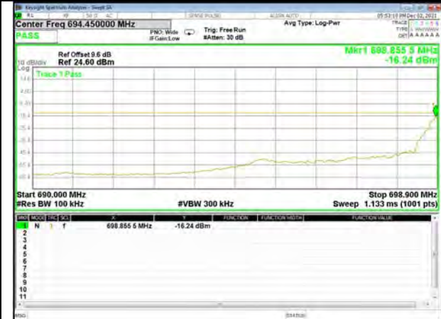
Band 12_5M_16QAM_Low_1-RB
