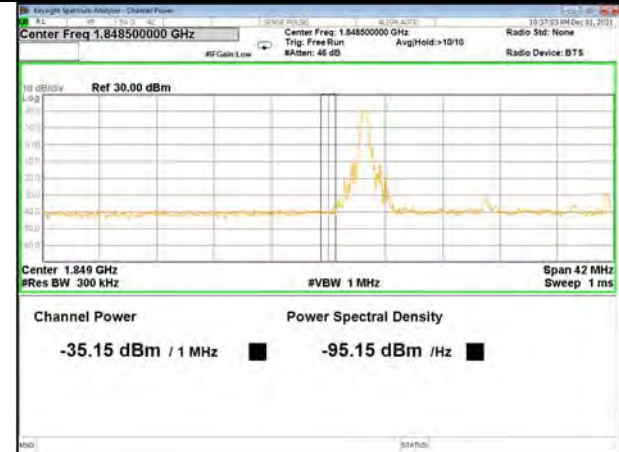
Band 2_20M_16QAM_Low_1-RB
