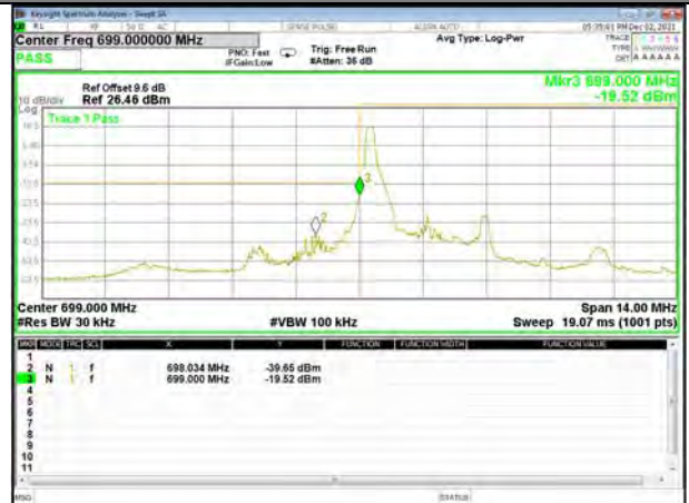
Band 12_3M_QPSK_Low_1-RB
