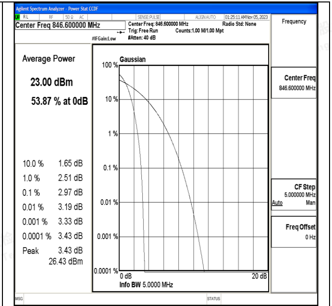
Channel 4233 / 846.6 MHz
