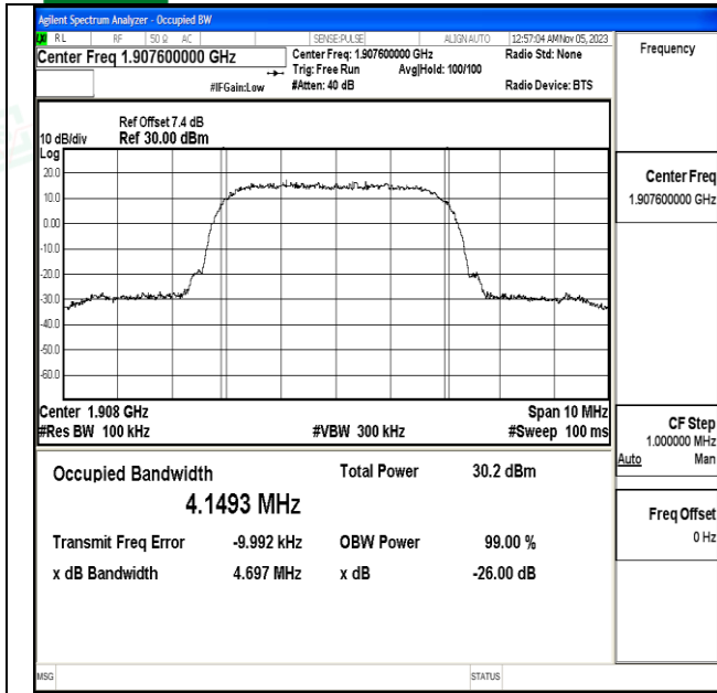
Channel 9538 / 1907.6 MHz
