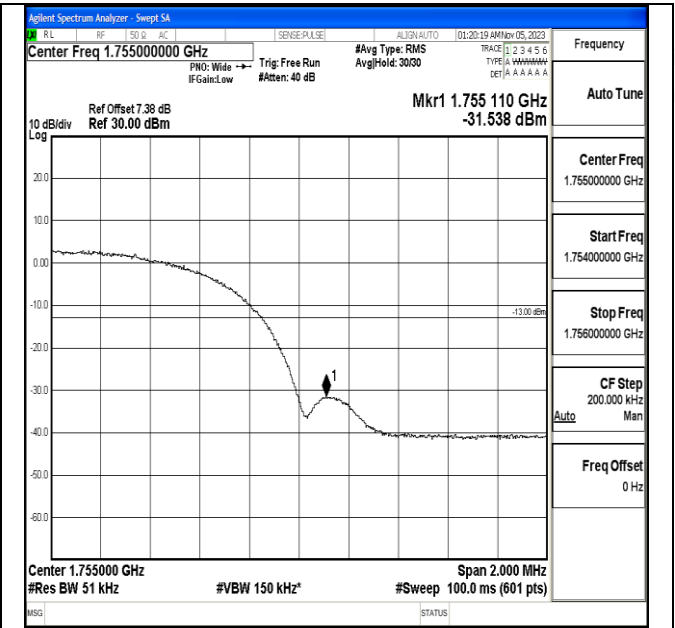
Channel 1513 / 1755.11 MHz
