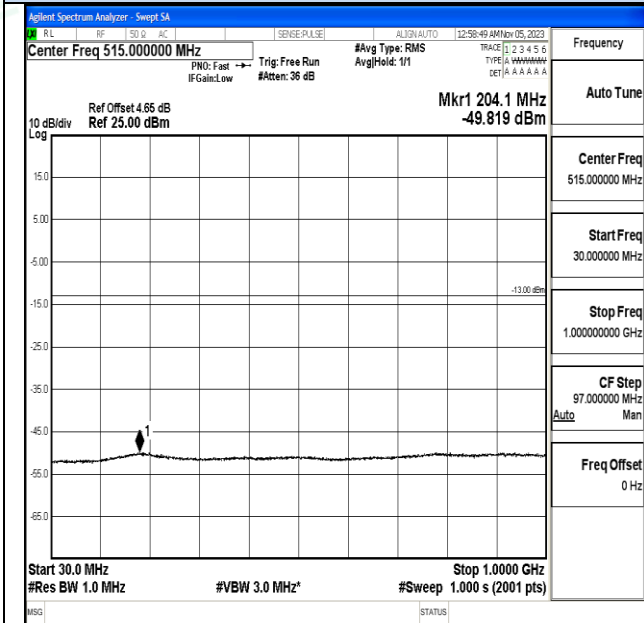
30 MHz – 1000 MHz
