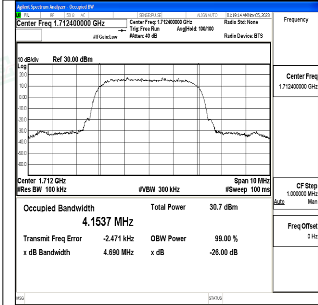
Channel 1312 / 1712.4 MHz
