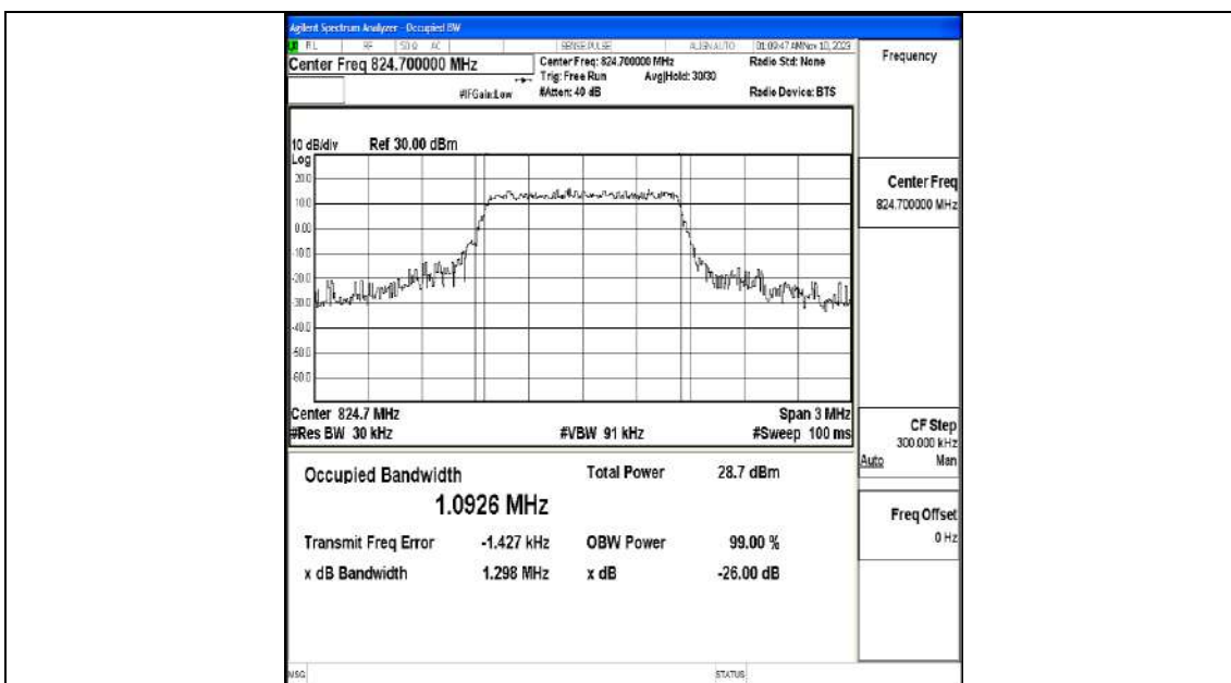
Band5-1.4MHz-QPSK-20407-6RB#0-PASS
