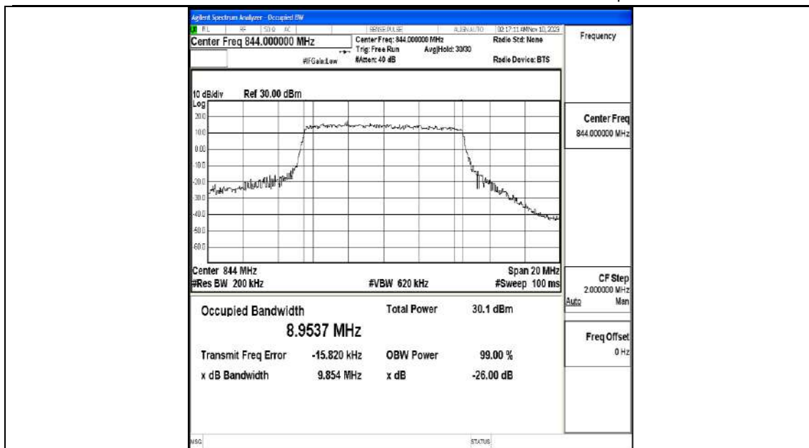
Band5-10MHz-QPSK-20600-50RB#0-PASS
