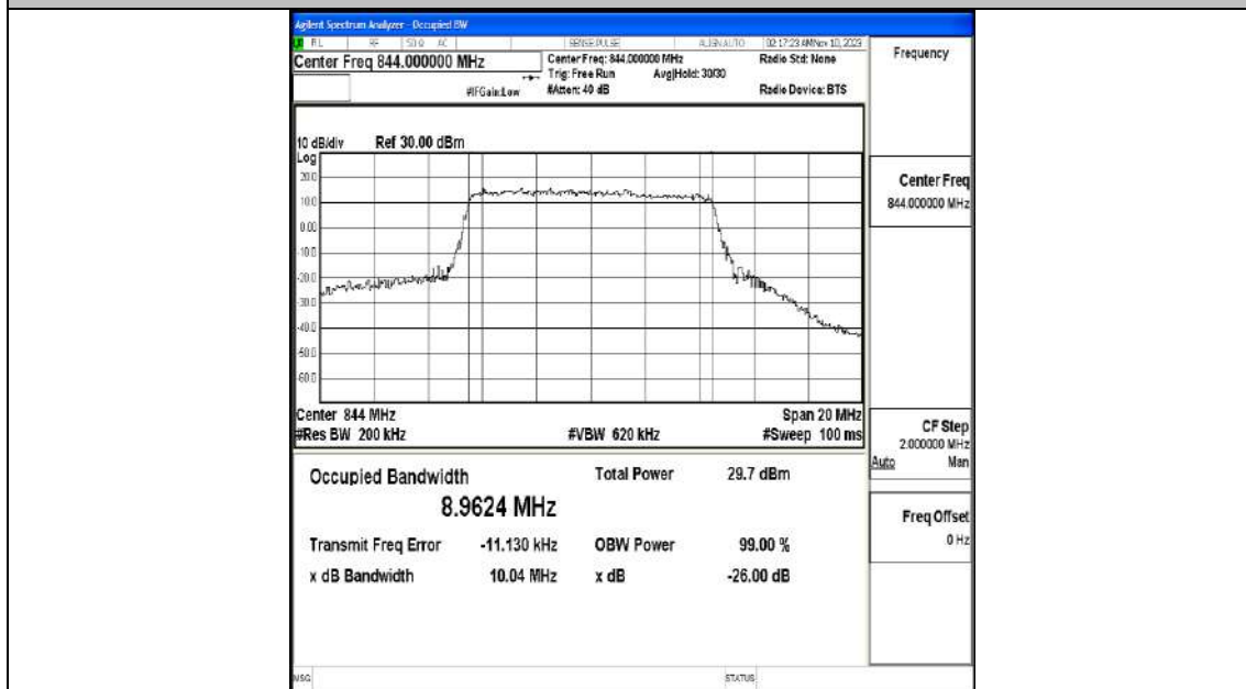
Band5-10MHz-16QAM-20600-50RB#0-PASS
