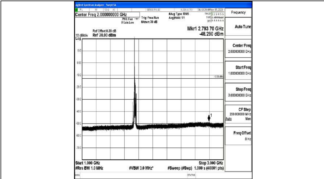
Band4_15MHz_16QAM_20325_1RB#0_1000~3000_1000~3000
