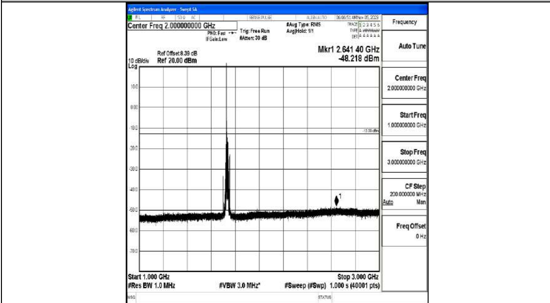
Band4_15MHz_QPSK_20175_1RB#0_1000~3000_1000~3000
