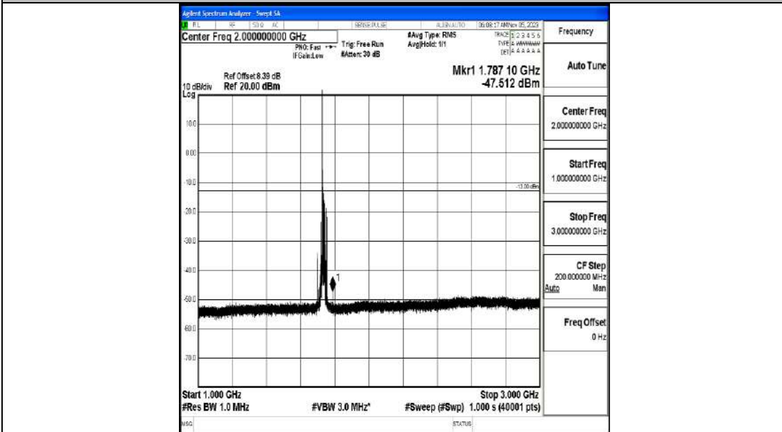
Band4_15MHz_16QAM_20175_1RB#0_1000~3000_1000~3000
