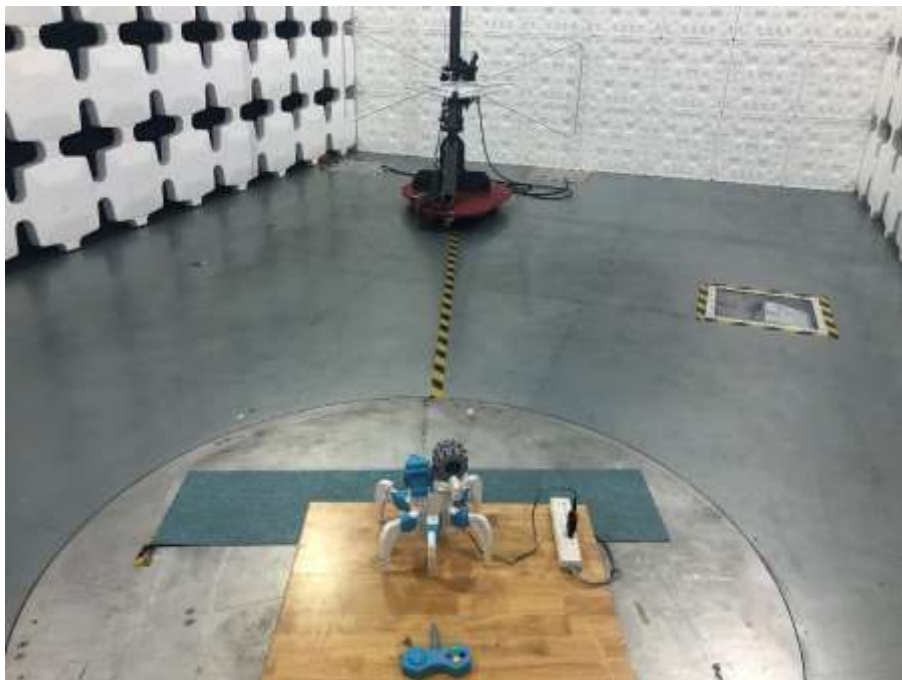
Photograph 4: Set-up for Radiated emission
