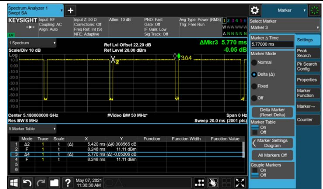
802.11ax-HE80(T=5.420ms)
