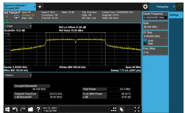
Channel 09 (2452MHz)
