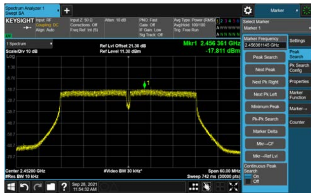
Channel 09 (2452MHz)
