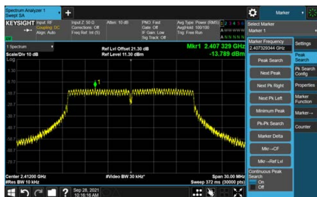
Channel 01 (2412MHz)
