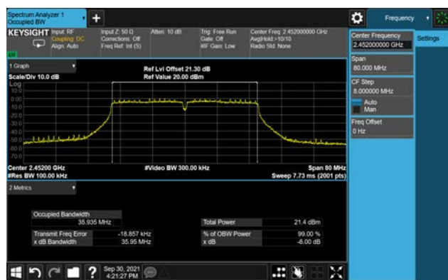
Channel 09 (2452MHz)
