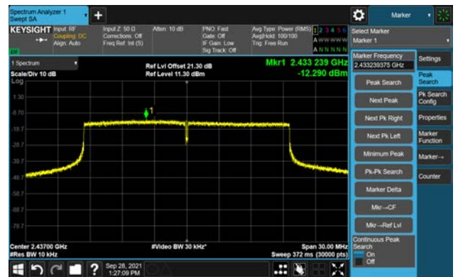
Channel 06 (2437MHz)
