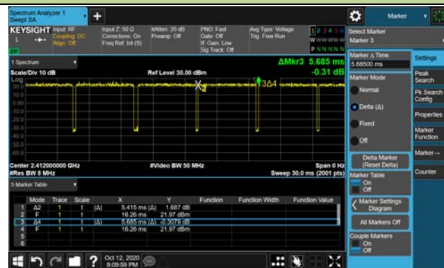
802.11VHT20 (T = 5.415 ms)
