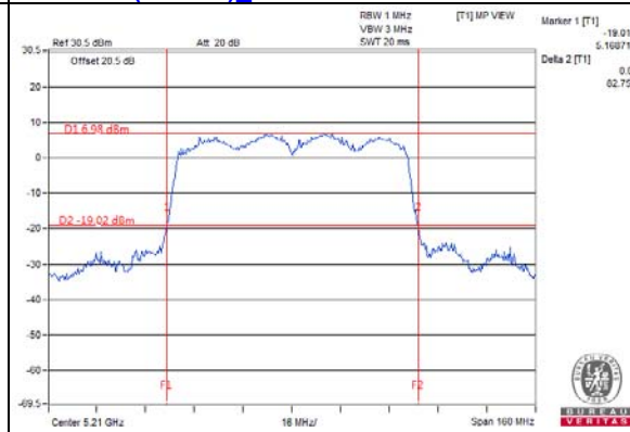
802.11ac (80MHz)_Chain 0 / CH42
