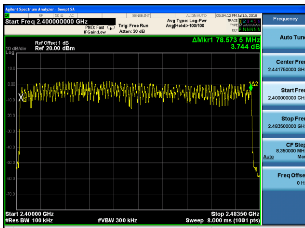
8- DPSK
