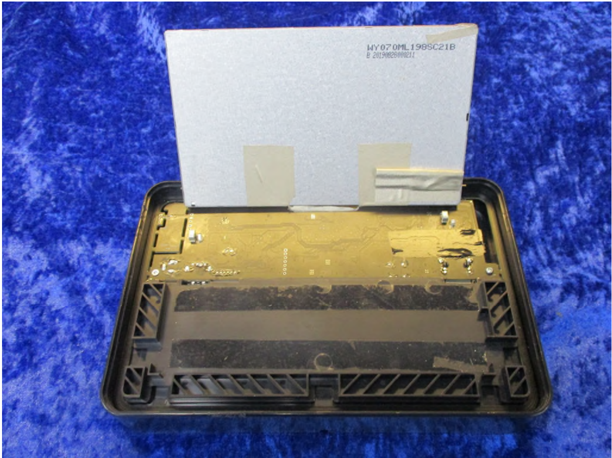
Pcb in chassis – display lifted
