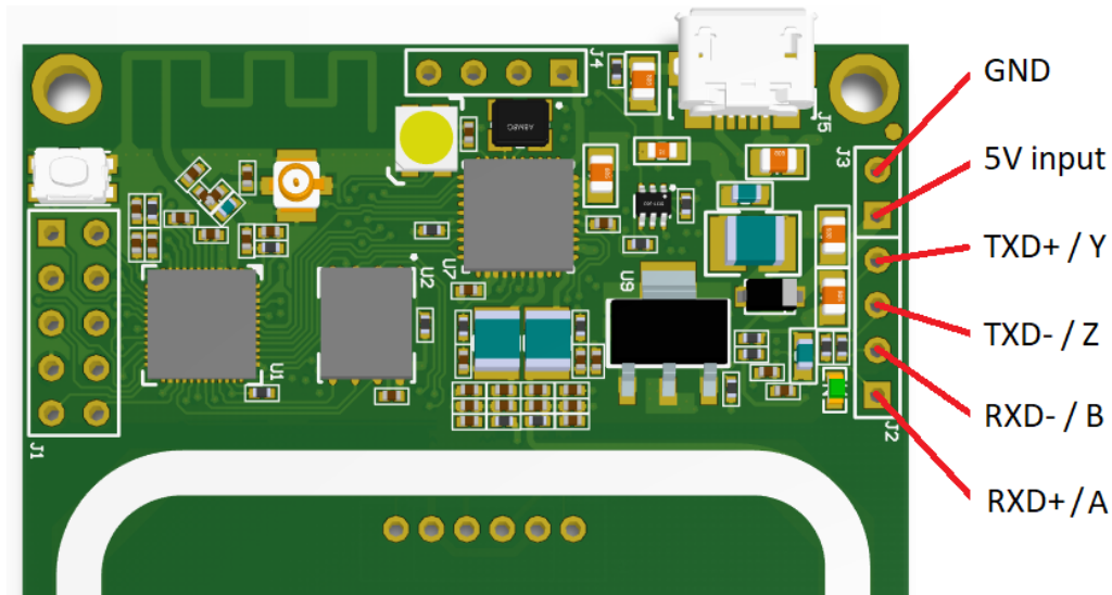
Figure 9 RS-485 pinout
