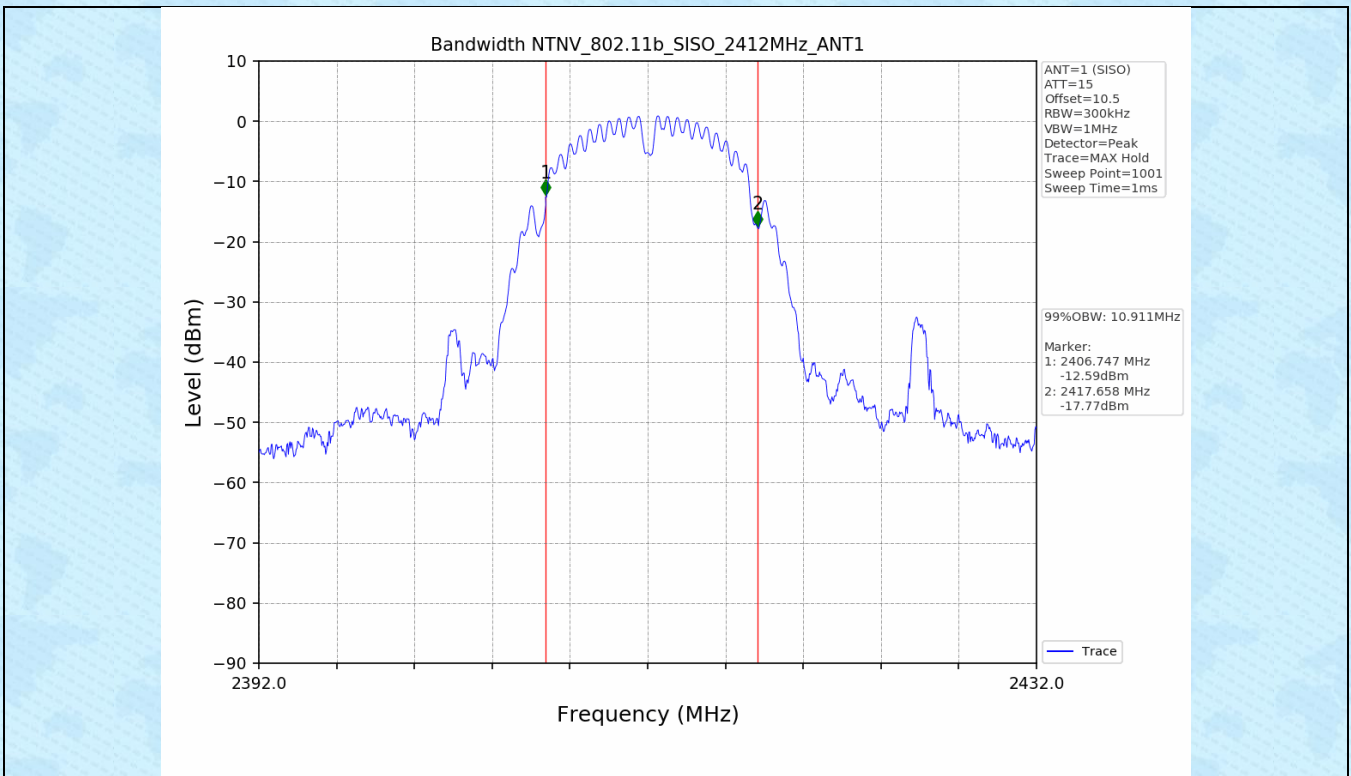
1.3 Test Graph - 99% Occupied Bandwidth
