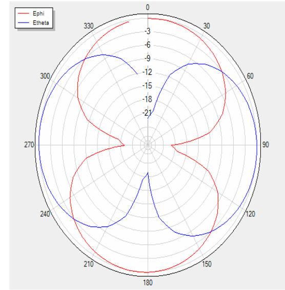
H Theta=0 freq=2430MHz
