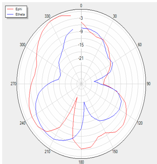
H Theta=90 freq=2470MHz
