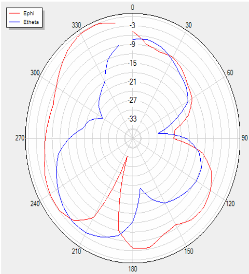
H Theta=90 freq=2440MHz
