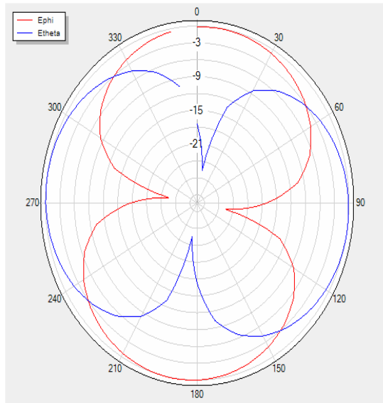
H Theta=0 freq=2420MHz
