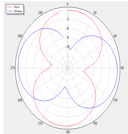
H Theta=0 freq=2450MHz
