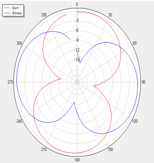
H Theta=0 freq=2440MHz
