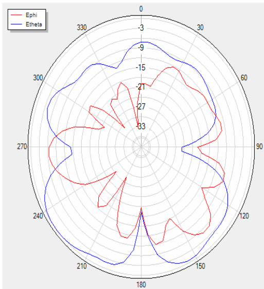
V Phi=90 freq=2490MHz
