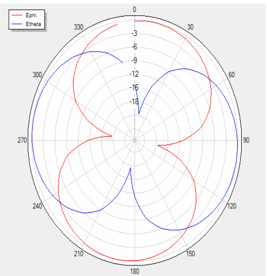
H Theta=0 freq=2430MHz
