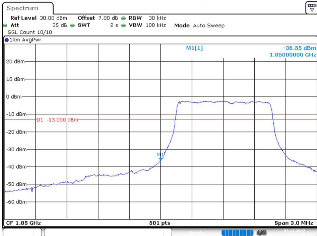
Band 2_1.4 MHz_Low_16QAM
