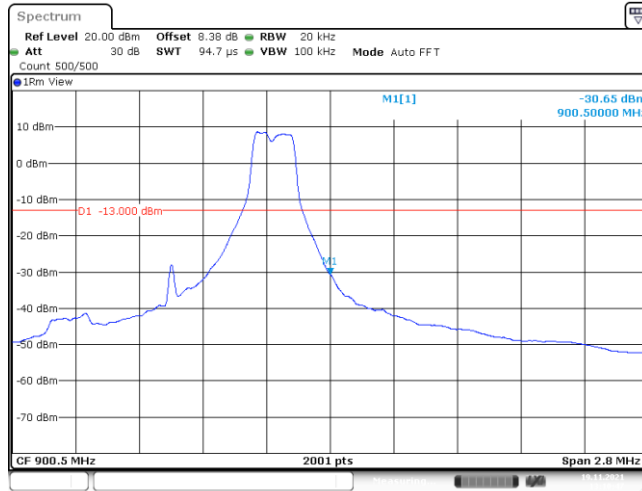
Band8-1.4MHz-QPSK-21648-6-0-Low--37.50-PASS
