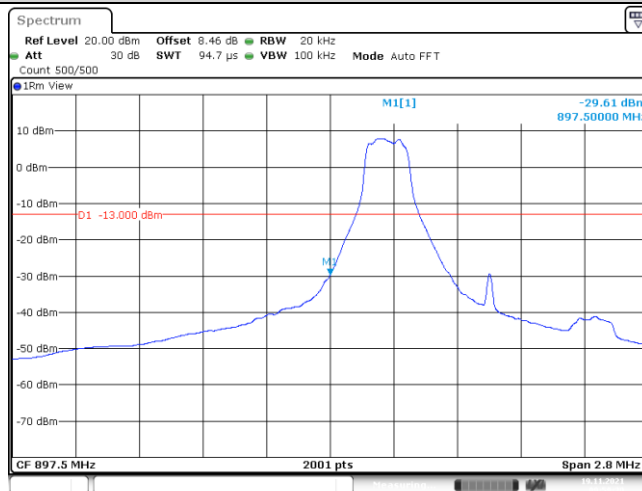
Band8-1.4MHz-16QAM-21632-1-0-Low--29.61-PASS
