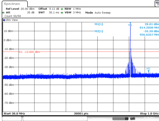
Band26-1.4MHz-QPSK-26697-1-0-Low-30-1000--35.59-PASS
