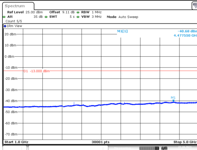
Band26-1.4MHz-QPSK-26697-1-0-Low-1000-5000--40.68-PASS
