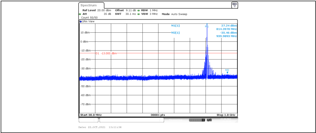
Band26-1.4MHz-16QAM-26697-1-0-Low-1000-5000--40.61-PASS
