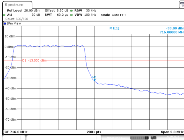
Band12-1.4MHz-QPSK-23173-6-0-Low--33.09-PASS
