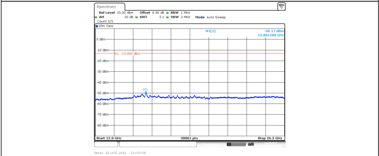
Band12-1.4MHz-16QAM-23095-1-0-Low-30-1000--35.8-PASS
