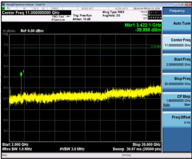
Band66-15MHz-16QAM-132047-1RB#0-Range3:2000~20000MHz
