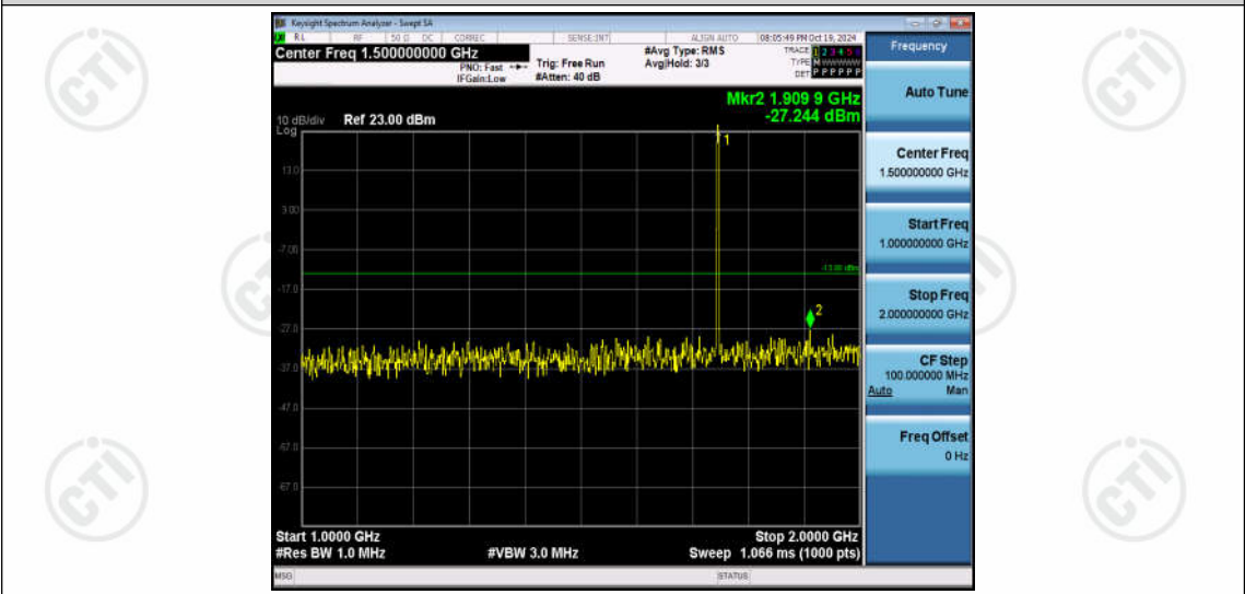
Band66-1.4MHz-16QAM-132322-1RB#0-Range2:1000~2000MHz
