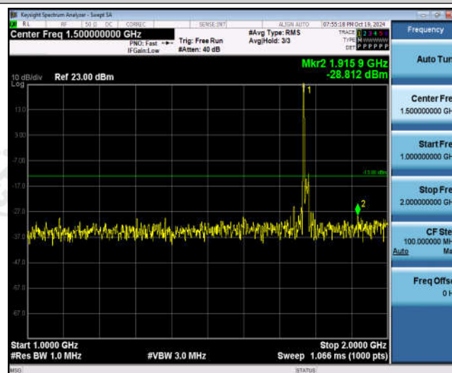
Band66-15MHz-QPSK-132597-1RB#0-Range2:1000~2000MHz
