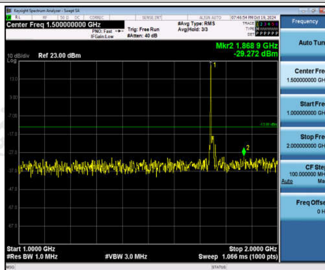
Band66-10MHz-QPSK-132322-1RB#0-Range2:1000~2000MHz
