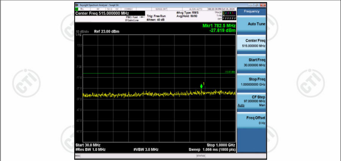
Band66-3MHz-16QAM-132657-1RB#0-Range1:30~1000MHz
