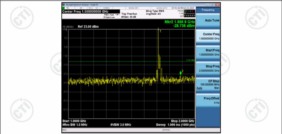
Band66-15MHz-QPSK-132047-1RB#0-Range2:1000~2000MHz
