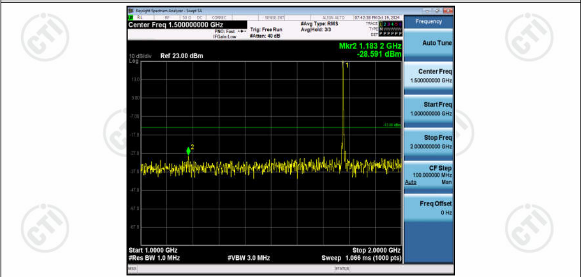
Band66-5MHz-QPSK-132647-1RB#0-Range2:1000~2000MHz
