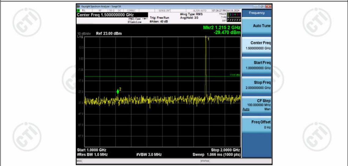
Band66-3MHz-QPSK-132657-1RB#0-Range2:1000~2000MHz
