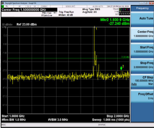
Band66-20MHz-16QAM-132072-1RB#0-Range2:1000~2000MHz
