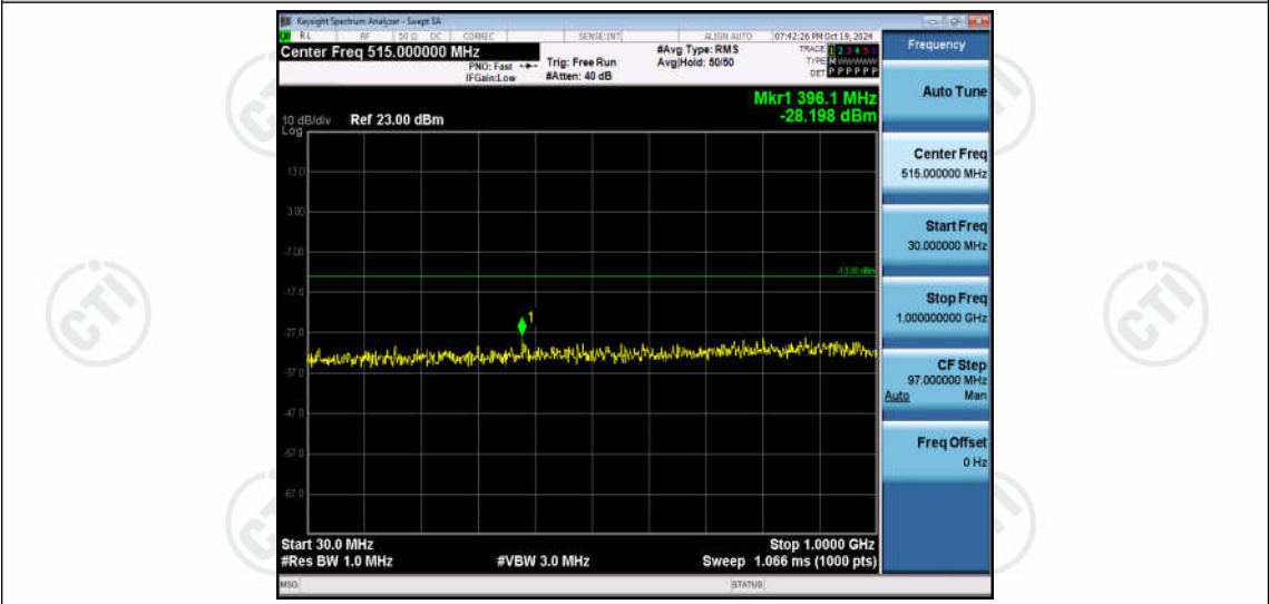
Band66-5MHz-QPSK-132647-1RB#0-Range1:30~1000MHz
