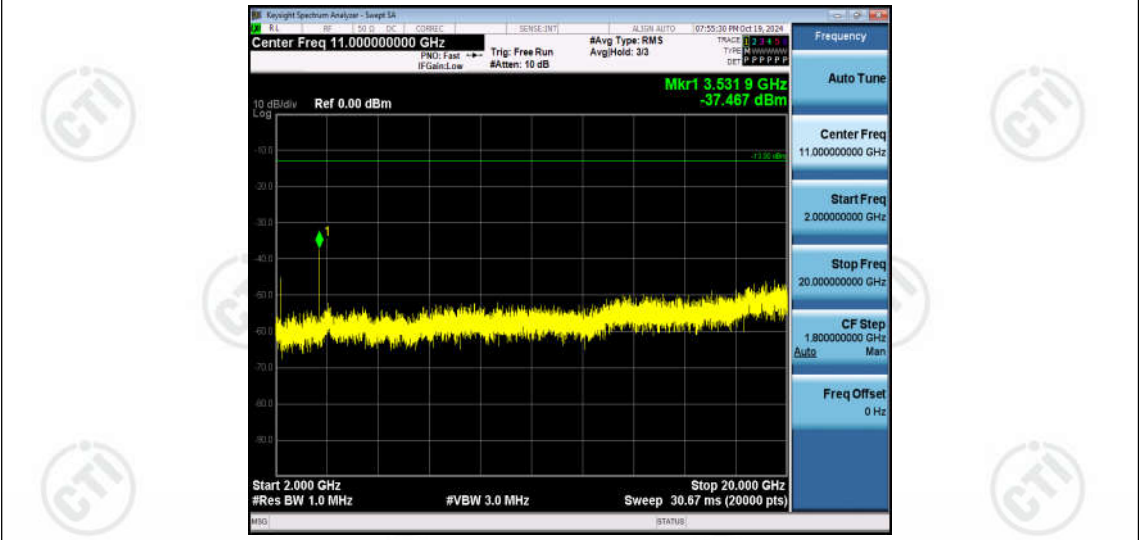
Band66-15MHz-QPSK-132597-1RB#0-Range3:2000~20000MHz
