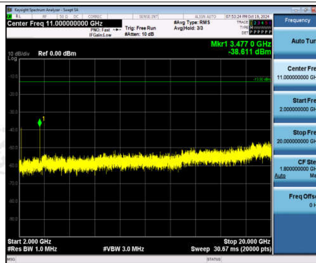
Band66-15MHz-QPSK-132322-1RB#0-Range3:2000~20000MHz
