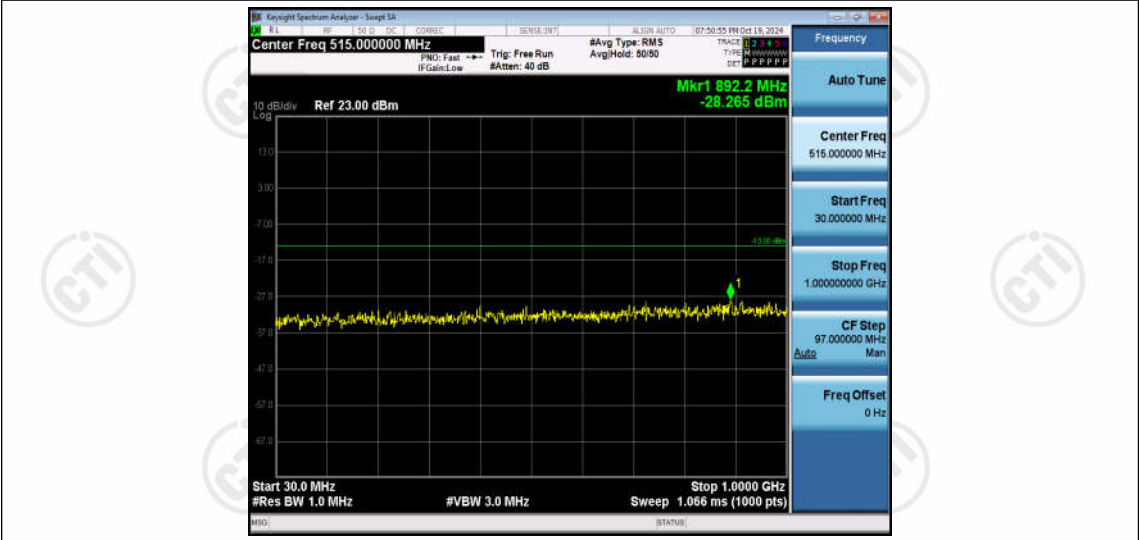
Band66-15MHz-QPSK-132047-1RB#0-Range1:30~1000MHz
