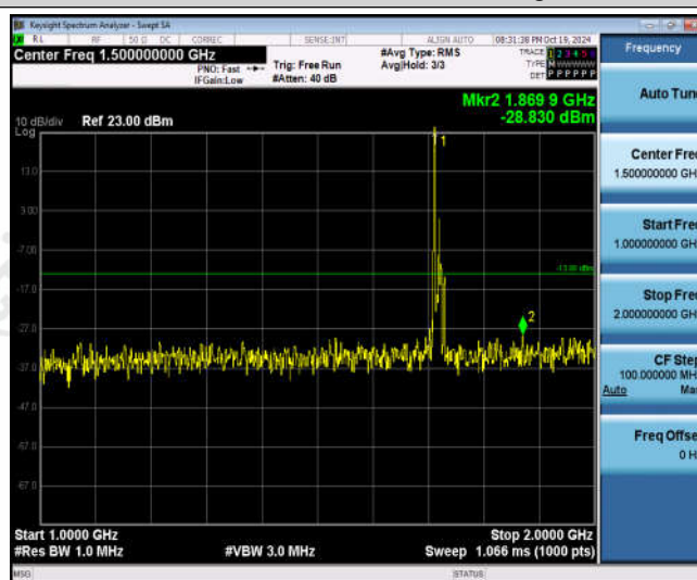
Band66-10MHz-16QAM-132022-1RB#0-Range2:1000~2000MHz
