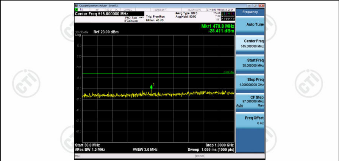
Band66-10MHz-QPSK-132622-1RB#0-Range1:30~1000MHz
