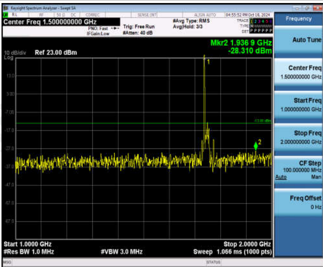
Band66-20MHz-16QAM-132322-1RB#0-Range2:1000~2000MHz
