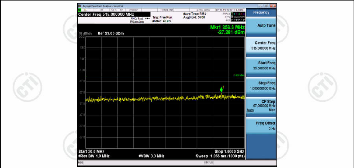
Band66-3MHz-QPSK-132657-1RB#0-Range1:30~1000MHz
