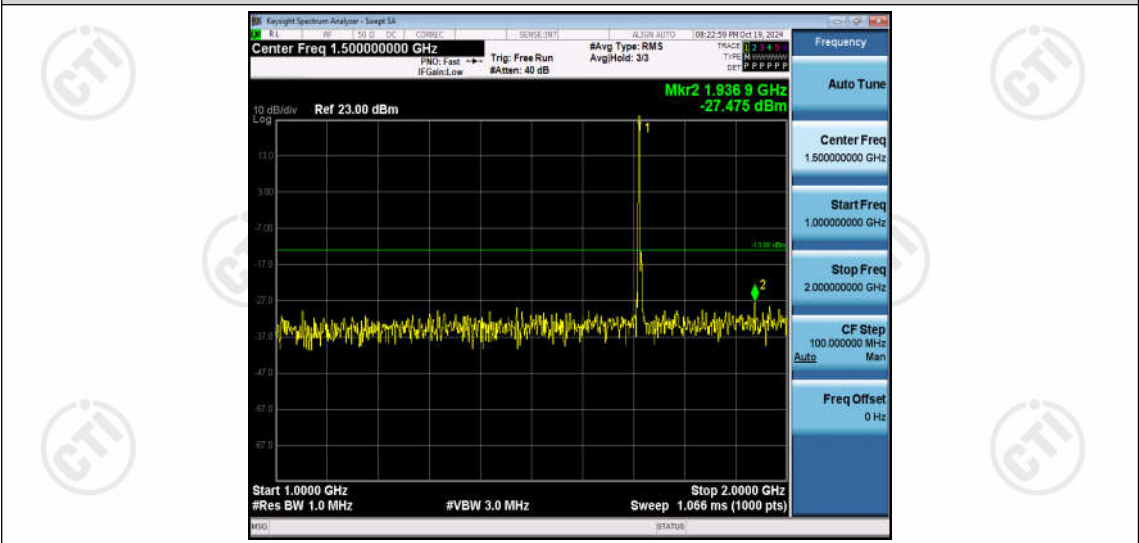
Band66-5MHz-16QAM-131997-1RB#0-Range2:1000~2000MHz
