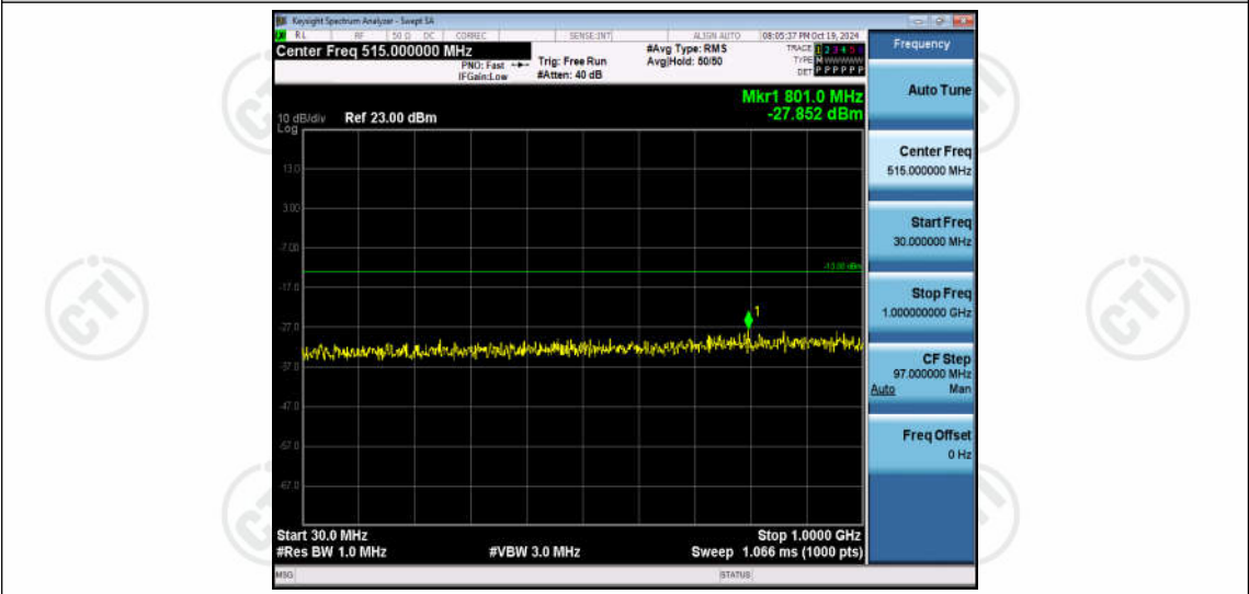
Band66-1.4MHz-16QAM-132322-1RB#0-Range1:30~1000MHz
