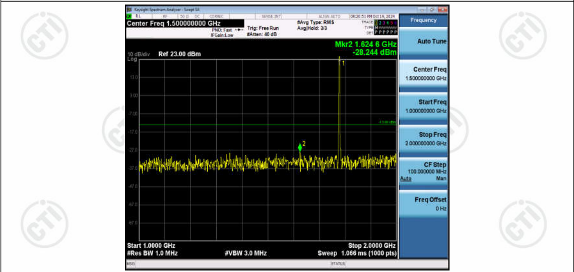
Band66-3MHz-16QAM-132657-1RB#0-Range2:1000~2000MHz
