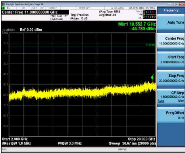
Band66-20MHz-16QAM-132072-1RB#0-Range3:2000~20000MHz
