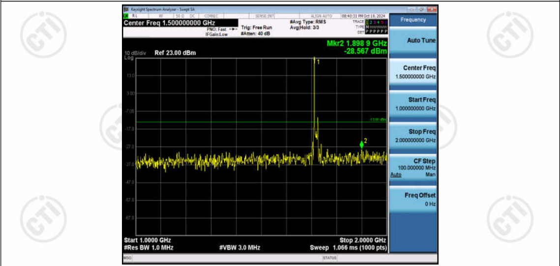
Band66-15MHz-16QAM-132047-1RB#0-Range2:1000~2000MHz
