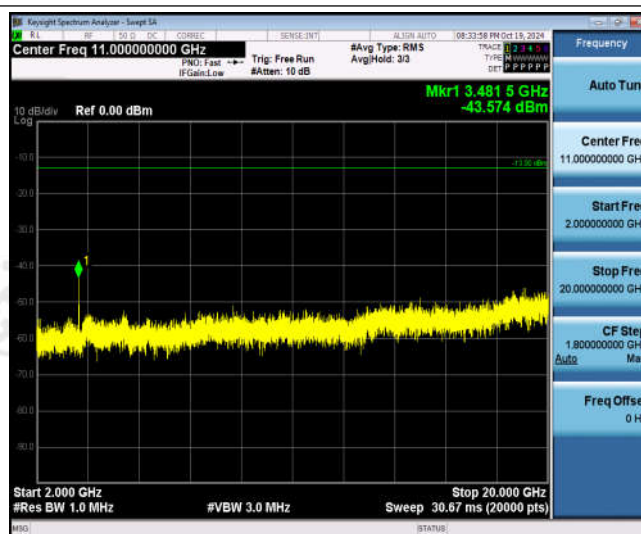
Band66-10MHz-16QAM-132322-1RB#0-Range3:2000~20000MHz
