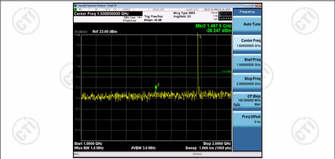
Band66-5MHz-16QAM-132647-1RB#0-Range2:1000~2000MHz
