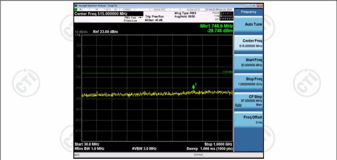
Band66-20MHz-QPSK-132322-1RB#0-Range1:30~1000MHz
