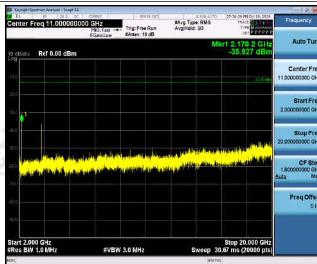
Band66-3MHz-QPSK-132657-1RB#0-Range3:2000~20000MHz
