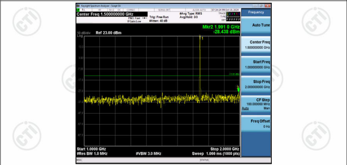
Band66-3MHz-QPSK-132322-1RB#0-Range2:1000~2000MHz
