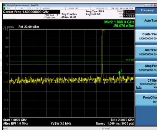
Band66-5MHz-16QAM-132322-1RB#0-Range2:1000~2000MHz
