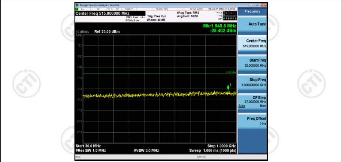
Band66-15MHz-16QAM-132047-1RB#0-Range1:30~1000MHz
