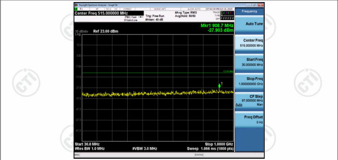
Band66-10MHz-QPSK-132022-1RB#0-Range1:30~1000MHz
