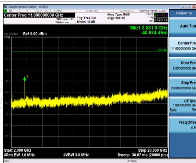
Band66-15MHz-16QAM-132597-1RB#0-Range3:2000~20000MHz
