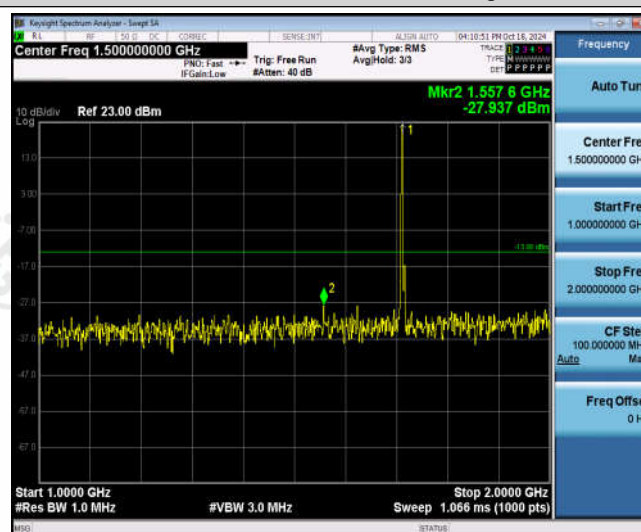
Band66-3MHz-16QAM-131987-1RB#0-Range2:1000~2000MHz
