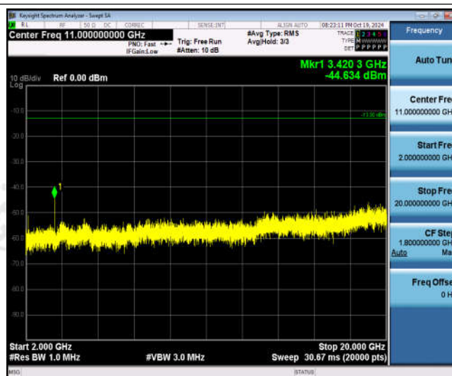
Band66-5MHz-16QAM-131997-1RB#0-Range3:2000~20000MHz
