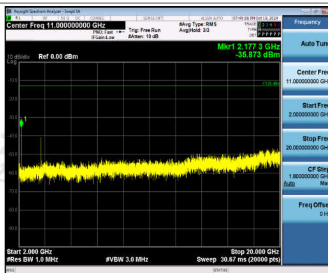
Band66-10MHz-QPSK-132622-1RB#0-Range3:2000~20000MHz
