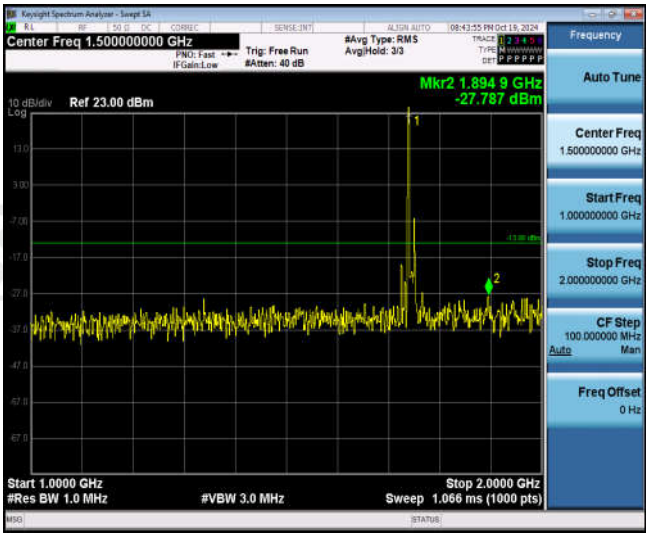
Band66-15MHz-16QAM-132322-1RB#0-Range2:1000~2000MHz
