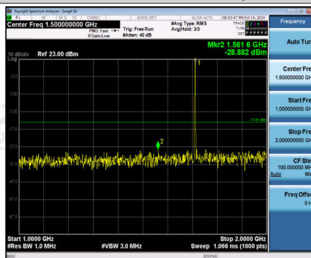
Band66-1.4MHz-16QAM-131979-1RB#0-Range2:1000~2000MHz
