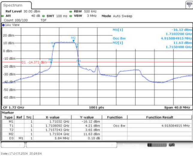
Band66-20MHz-16QAM-132072-25RB#0-4.915
