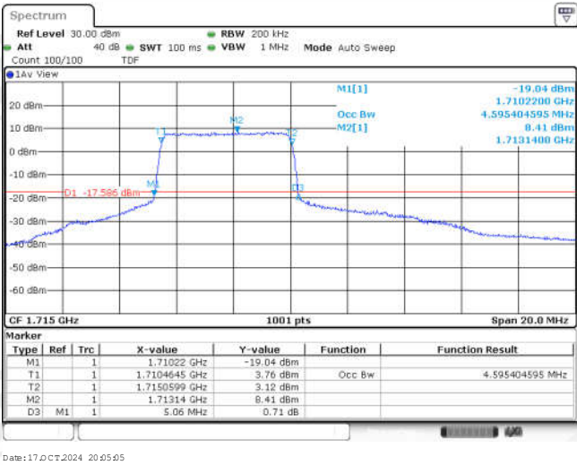
Band66-10MHz-16QAM-132022-25RB#0-4.595
