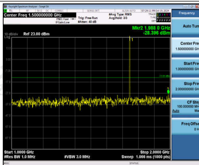
Band66-1.4MHz-QPSK-132322-1RB#0-Range2:1000~2000MHz
