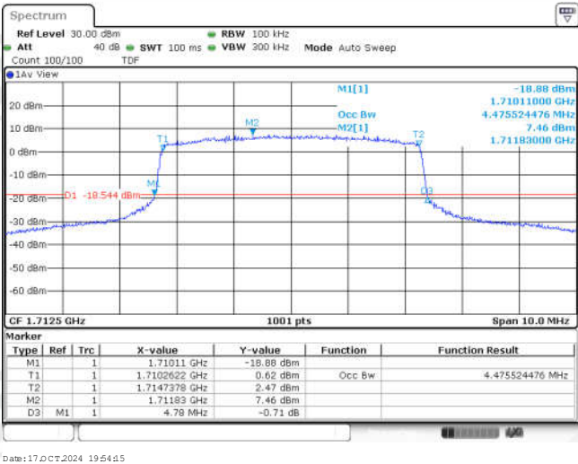
Band66-5MHz-16QAM-131997-25RB#0-4.476
