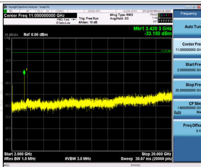
Band66-1.4MHz-QPSK-131979-1RB#0-Range3:2000~20000MHz
