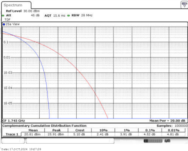
Band66-5MHz-QPSK-132322-25RB#0
