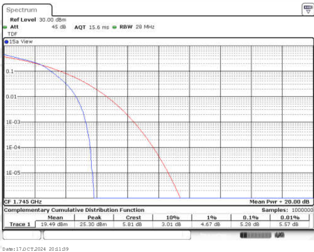
Band66-10MHz-16QAM-132322-25RB#0
