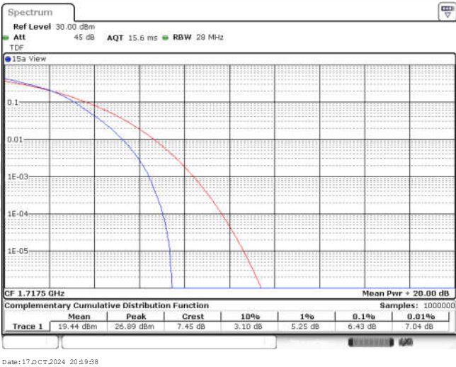
Band66-15MHz-16QAM-132047-25RB#0
