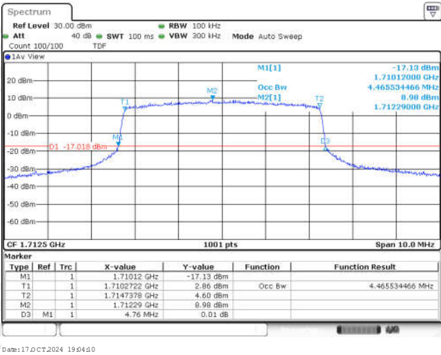
Band66-5MHz-QPSK-131997-25RB#0-4.466
