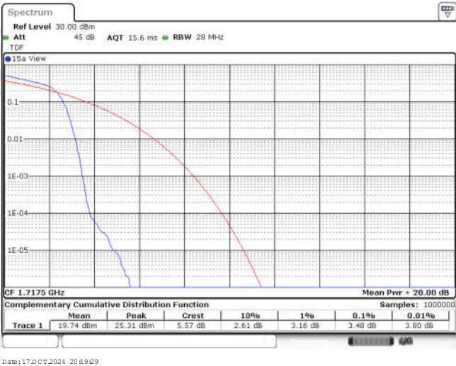
Band66-15MHz-16QAM-132047-1RB#0
