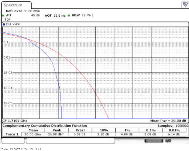
Band66-1.4MHz-16QAM-131979-1RB#0
