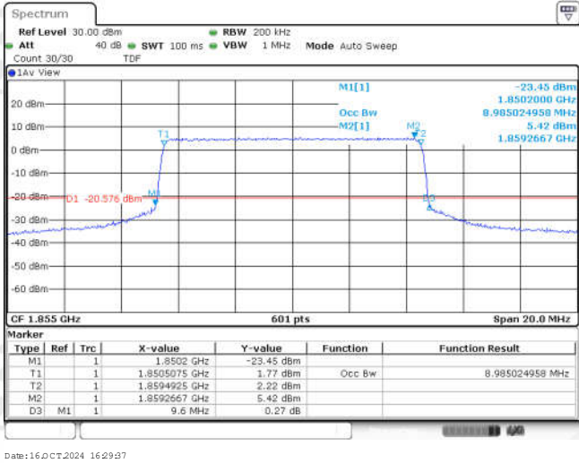
Band25-10MHz-QPSK-26090-50RB#0-8.985
