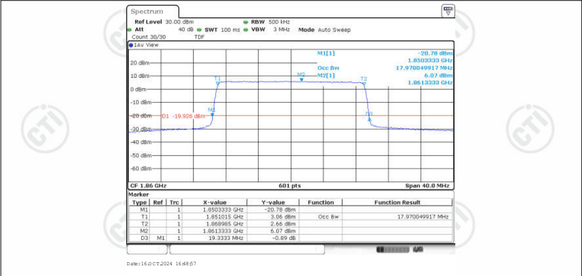
Band25-20MHz-QPSK-26140-100RB#0-17.97
