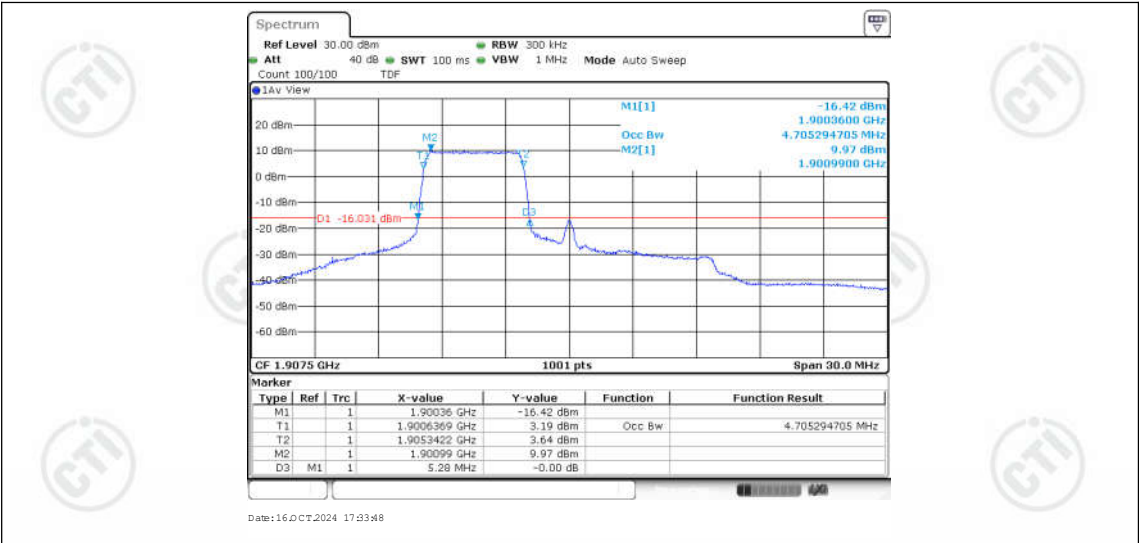
Band25-15MHz-16QAM-26615-25RB#0-4.705
