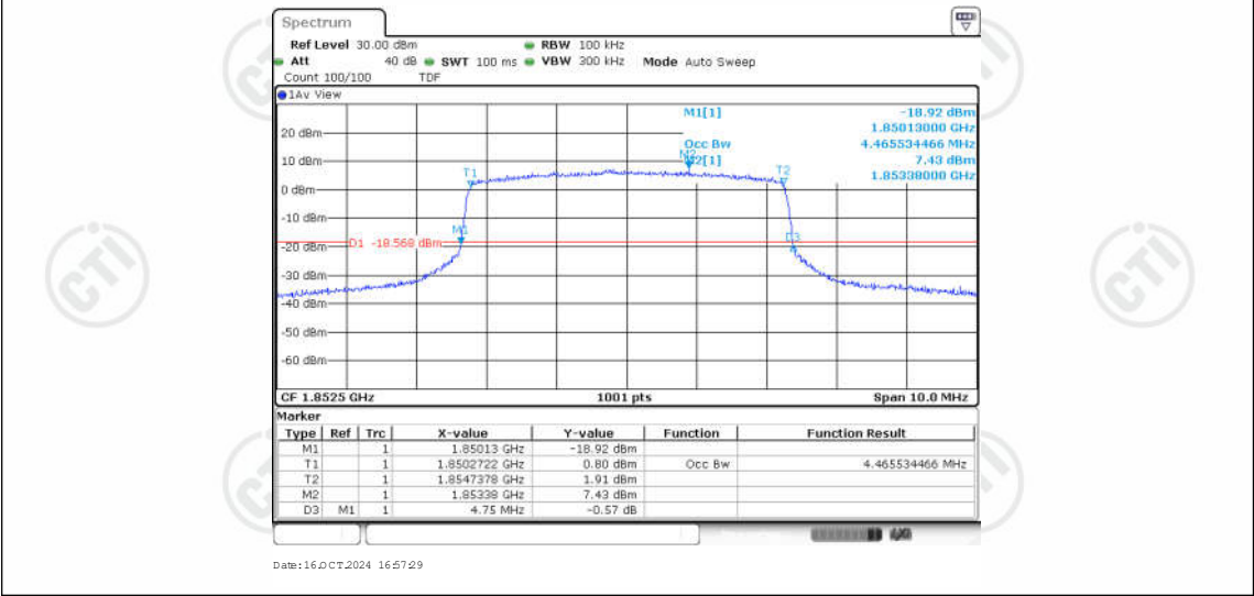
Band25-5MHz-16QAM-26065-25RB#0-4.466
