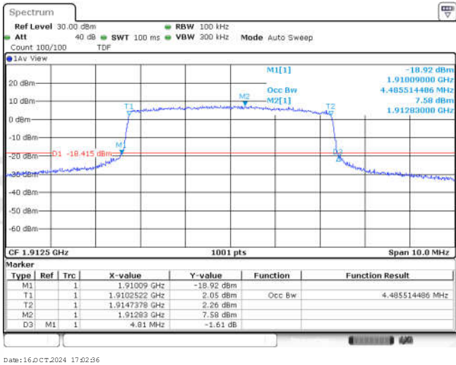
Band25-5MHz-16QAM-26665-25RB#0-4.486
