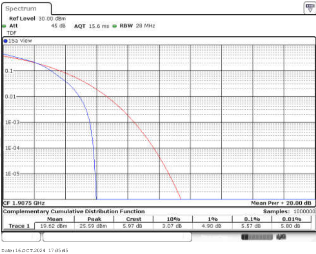
Band25-15MHz-16QAM-26615-25RB#0
