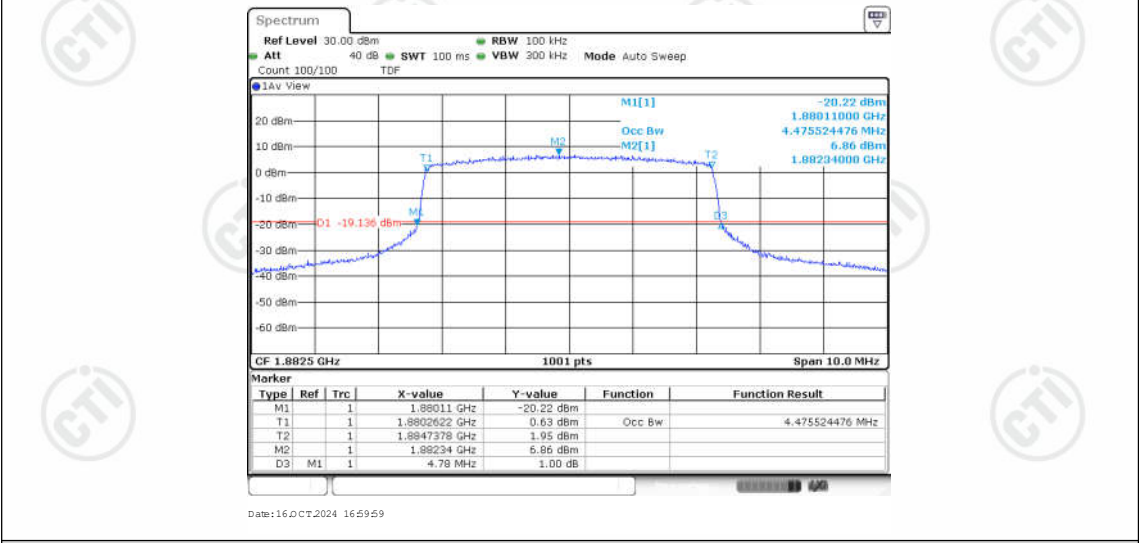
Band25-5MHz-16QAM-26365-25RB#0-4.476
