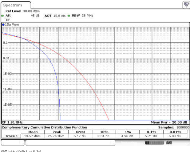
Band25-10MHz-16QAM-26640-25RB#0
