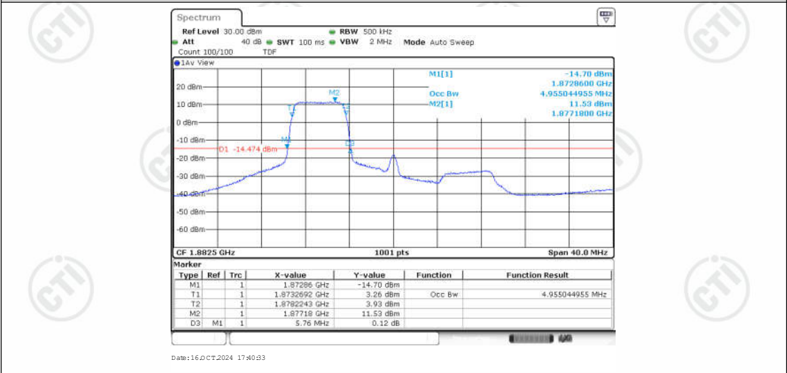
Band25-20MHz-16QAM-26365-25RB#0-4.955
