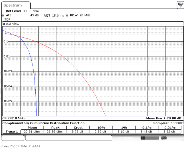
Band13-5MHz-QPSK-23230-1RB#0
