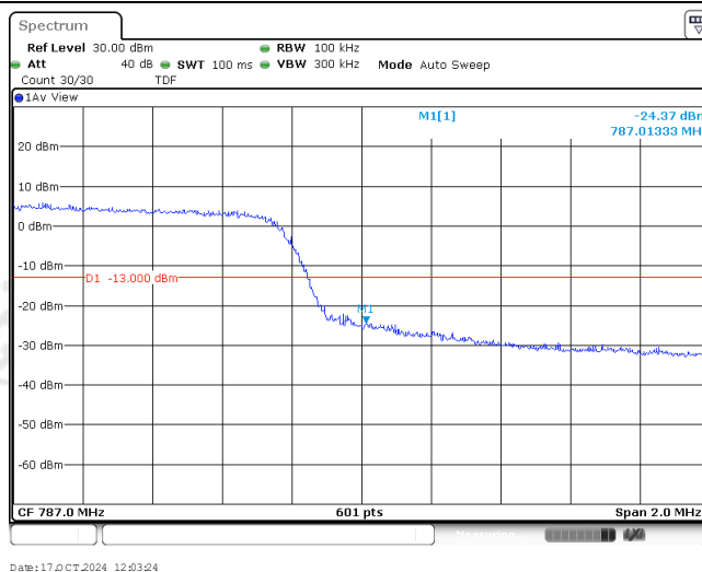
Band13-5MHz-16QAM-23255-25RB#0
