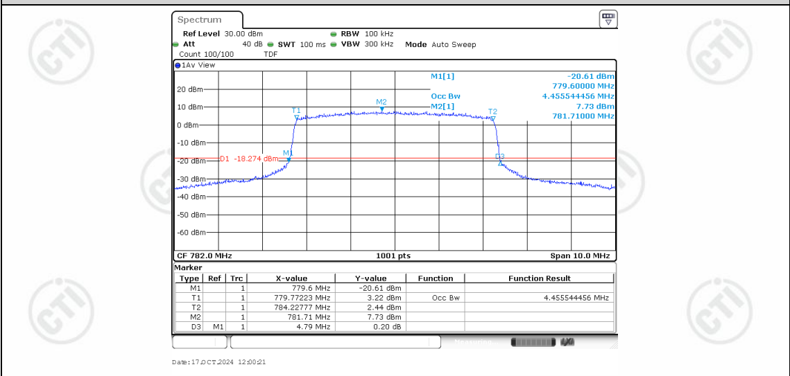
Band13-5MHz-16QAM-23230-25RB#0-4.456
