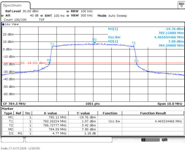
Band13-5MHz-16QAM-23255-25RB#0-4.466
