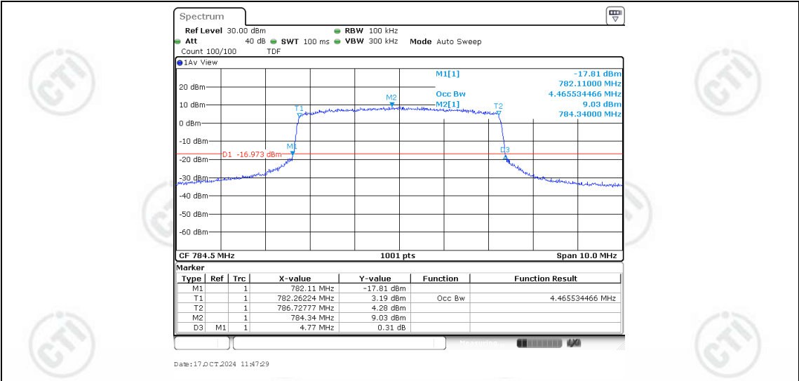
Band13-5MHz-QPSK-23255-25RB#0-4.466
