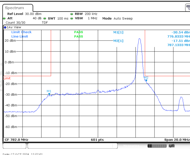
Band13-10MHz-QPSK-23230-1RB#49
