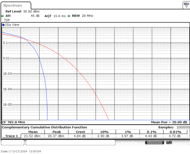
Band13-5MHz-16QAM-23230-1RB#0
