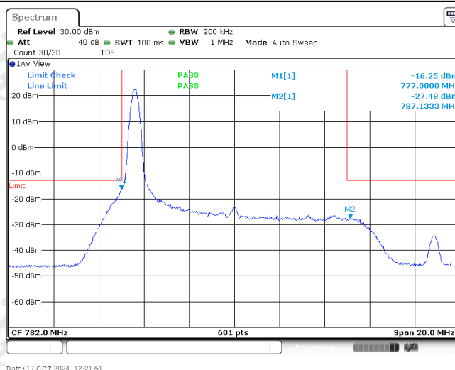
Band13-10MHz-QPSK-23230-1RB#0
