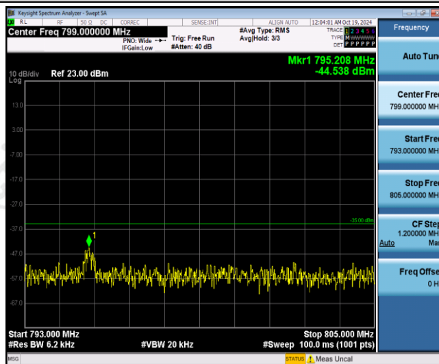
Band13-10MHz-16QAM-23230-1RB#0-Range2:793~805MHz
