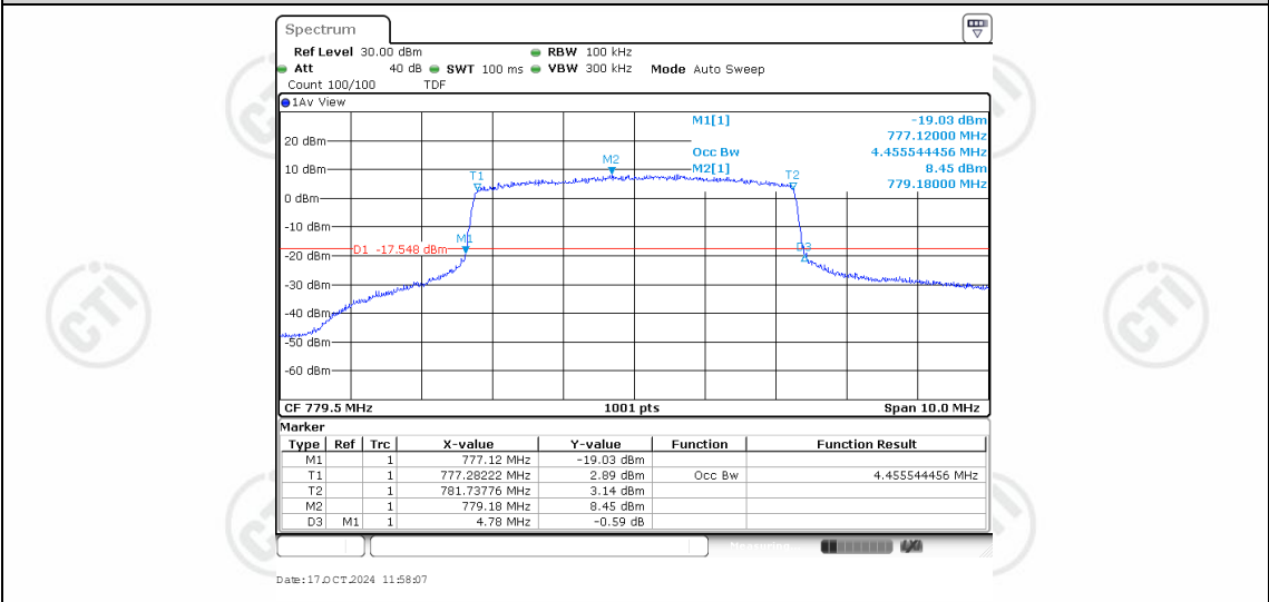
Band13-5MHz-16QAM-23205-25RB#0-4.456
