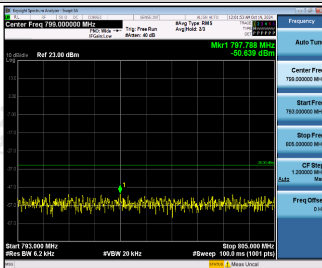
Band13-5MHz-16QAM-23230-1RB#0-Range2:793~805MHz
