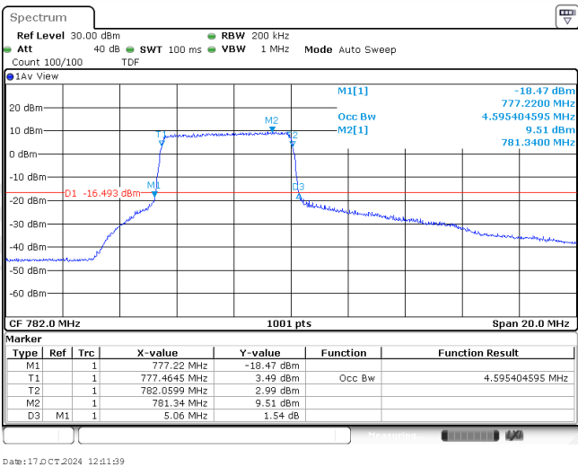
Band13-10MHz-16QAM-23230-25RB#0-4.595
