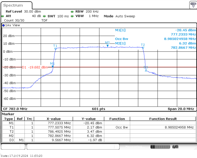
Band13-10MHz-QPSK-23230-50RB#0-8.985
