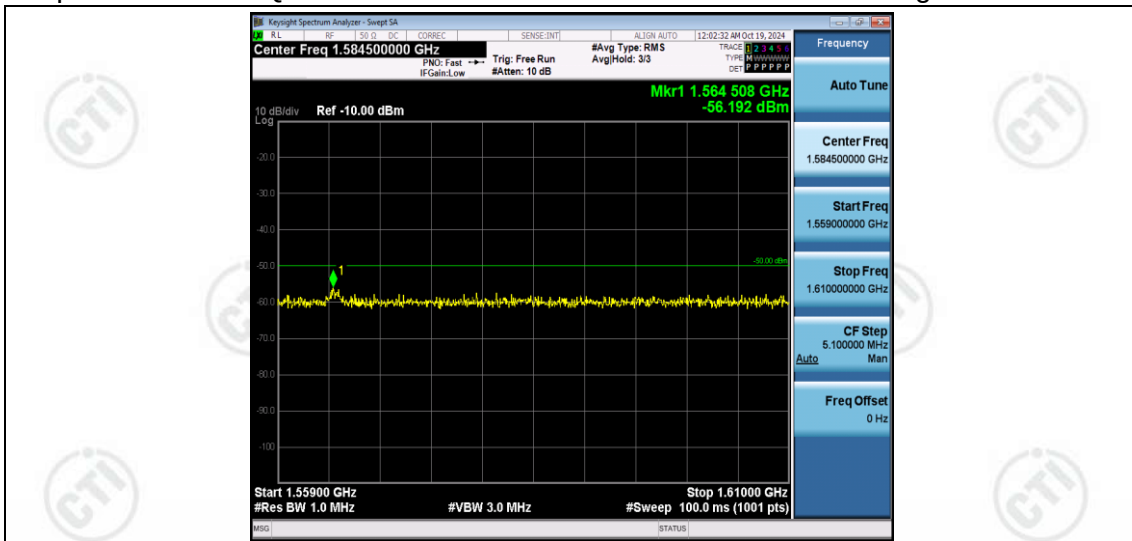
Band13-5MHz-16QAM-23255-1RB#0-Range3:1559~1610MHz
