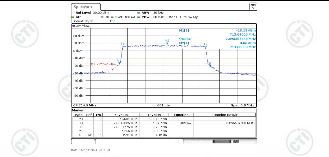
Band12-3MHz-QPSK-23165-15RB#0-2.696
