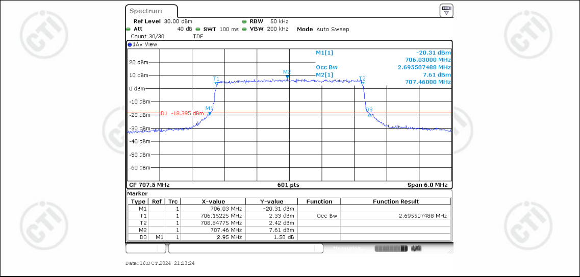
Band12-3MHz-16QAM-23095-15RB#0-2.696
