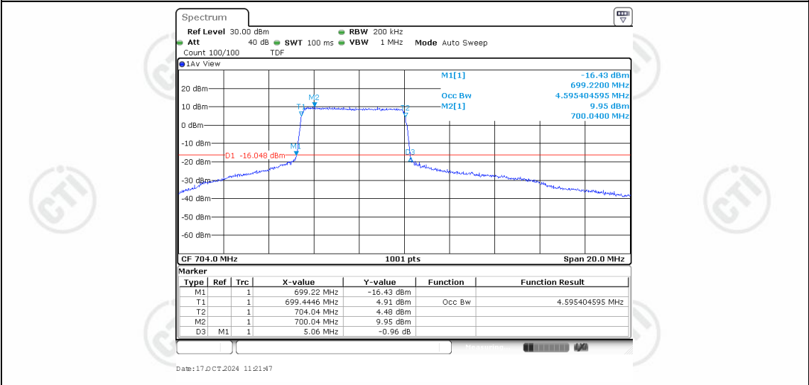
Band12-10MHz-16QAM-23060-25RB#0-4.595
