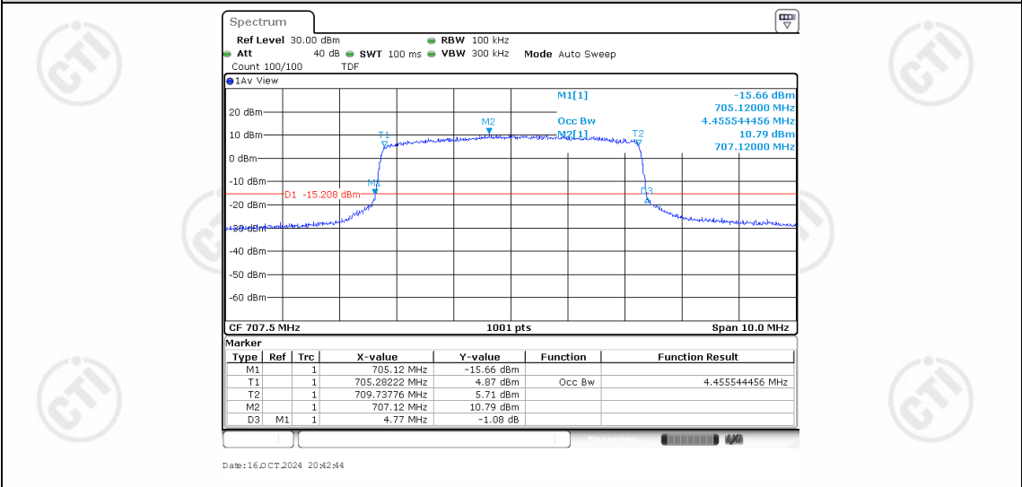
Band12-5MHz-QPSK-23095-25RB#0-4.456
