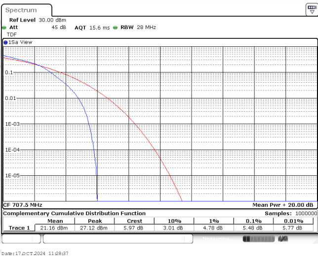
Band12-10MHz-16QAM-23095-25RB#0
