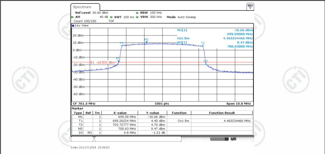
Band12-5MHz-QPSK-23035-25RB#0-4.466
