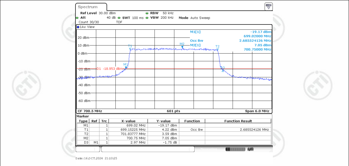
Band12-3MHz-16QAM-23025-15RB#0-2.686
