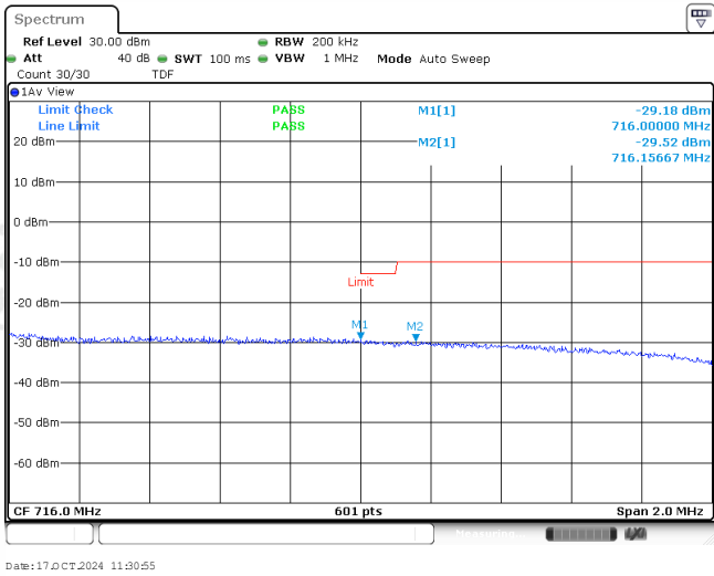
Band12-10MHz-16QAM-23130-1RB#24
