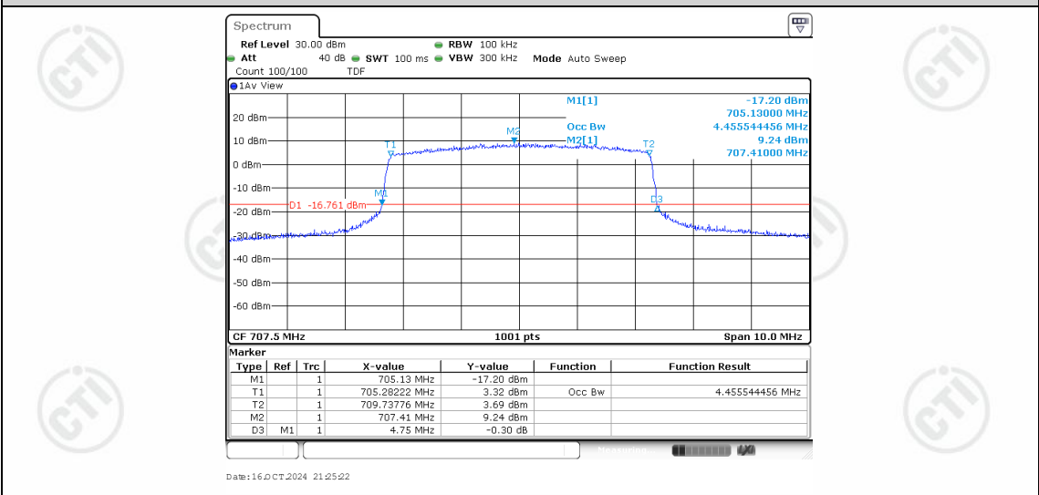
Band12-5MHz-16QAM-23095-25RB#0-4.456
