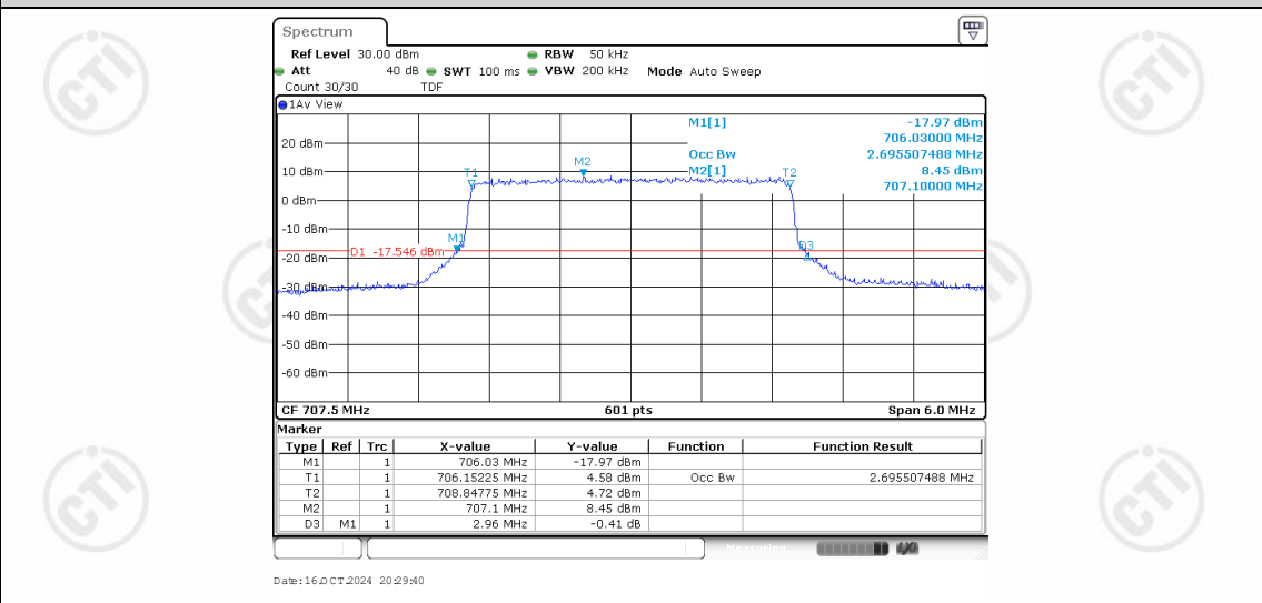
Band12-3MHz-QPSK-23095-15RB#0-2.696
