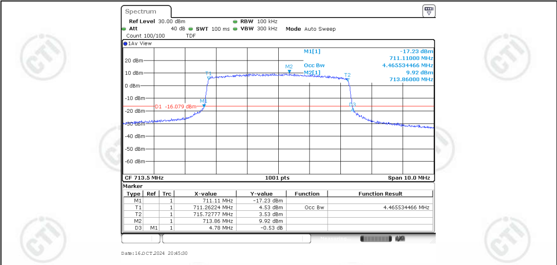
Band12-5MHz-QPSK-23155-25RB#0-4.466
