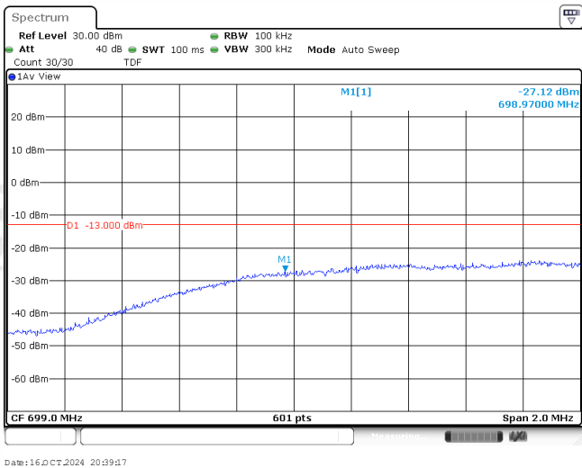
Band12-5MHz-QPSK-23035-1RB#24
