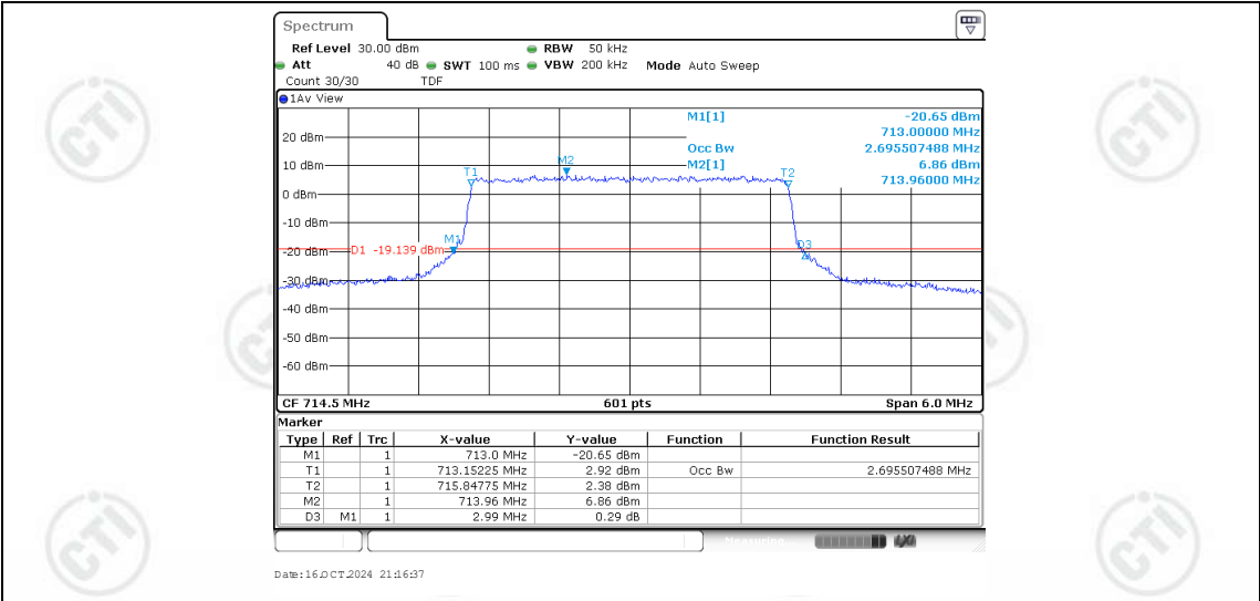
Band12-3MHz-16QAM-23165-15RB#0-2.696
