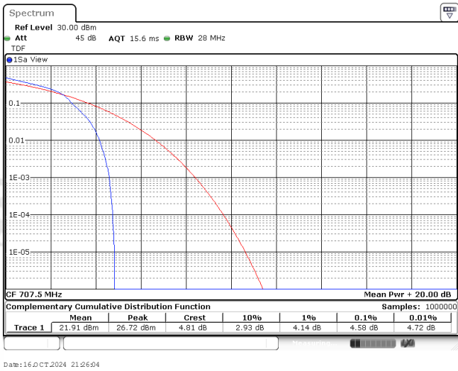
Band12-5MHz-16QAM-23095-1RB#0
