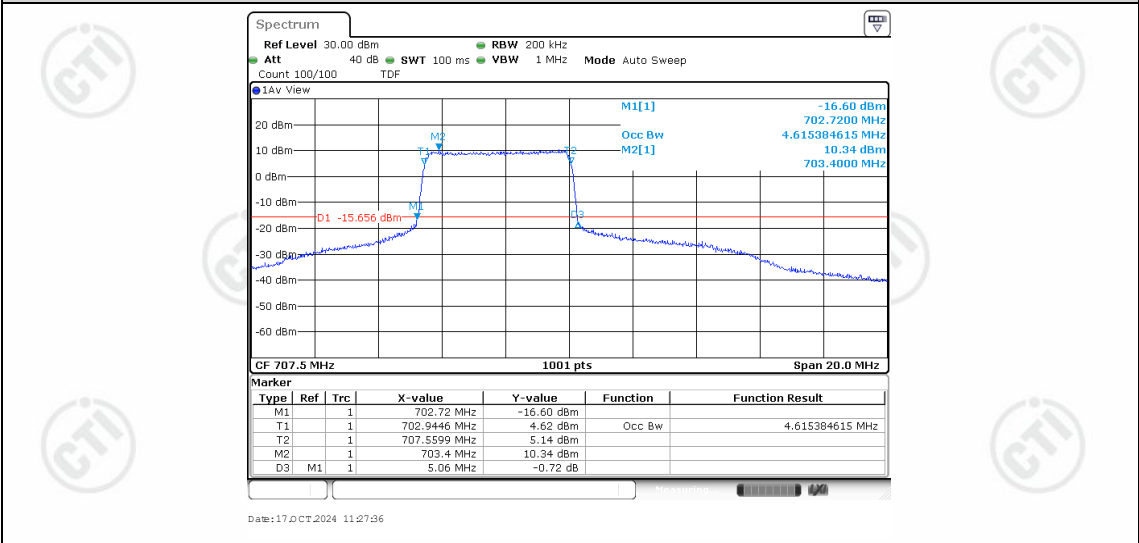
Band12-10MHz-16QAM-23095-25RB#0-4.615
