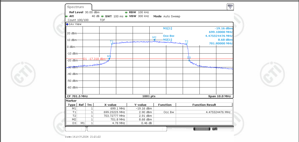
Band12-5MHz-16QAM-23035-25RB#0-4.476
