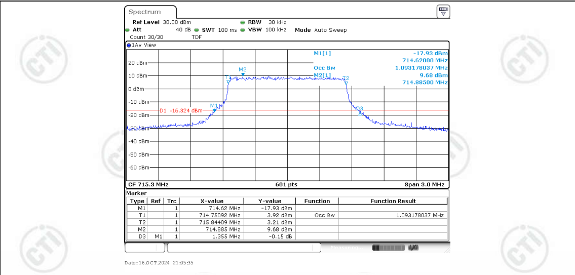
Band12-1.4MHz-16QAM-23173-6RB#0-1.093
