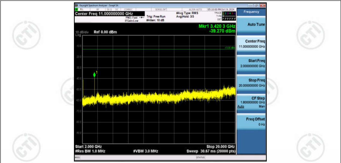
Band4-3MHz-16QAM-19965-1RB#0-Range3:2000~20000MHz
