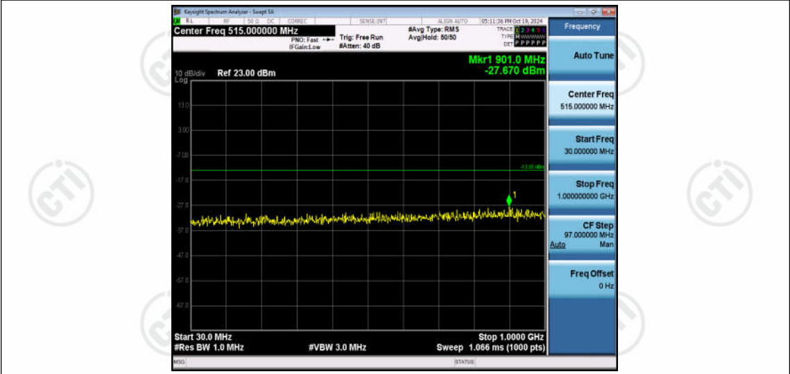
Band4-3MHz-16QAM-20385-1RB#0-Range1:30~1000MHz
