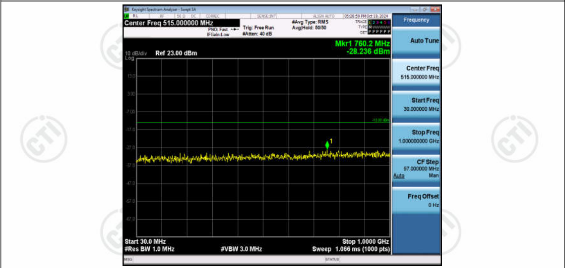
Band4-15MHz-16QAM-20175-1RB#0-Range1:30~1000MHz
