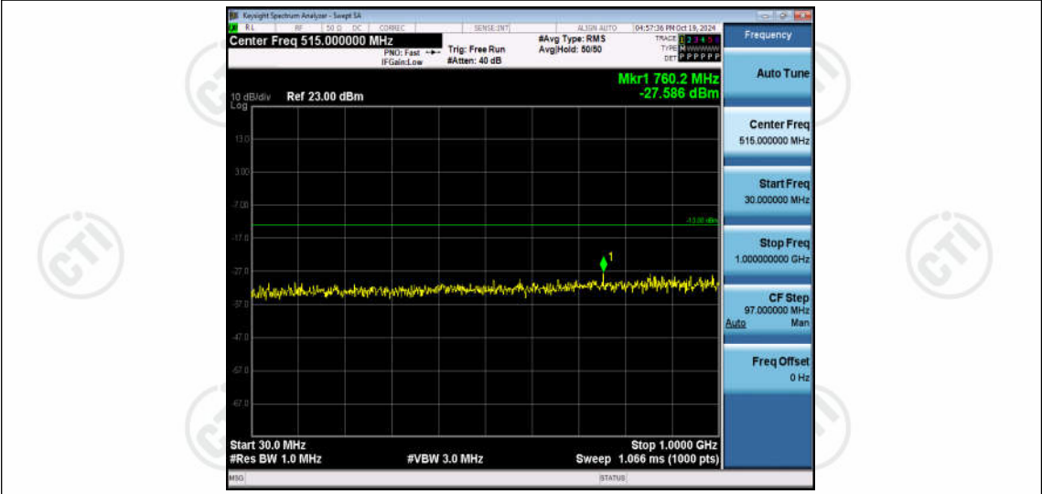
Band4-10MHz-QPSK-20350-1RB#0-Range1:30~1000MHz
