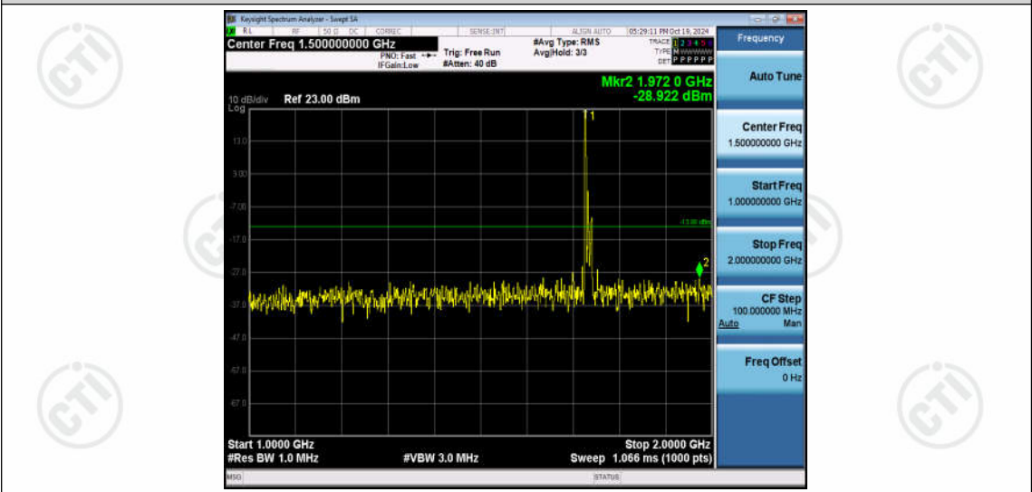
Band4-15MHz-16QAM-20175-1RB#0-Range2:1000~2000MHz
