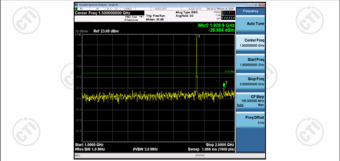
Band4-5MHz-16QAM-20375-1RB#0-Range2:1000~2000MHz
