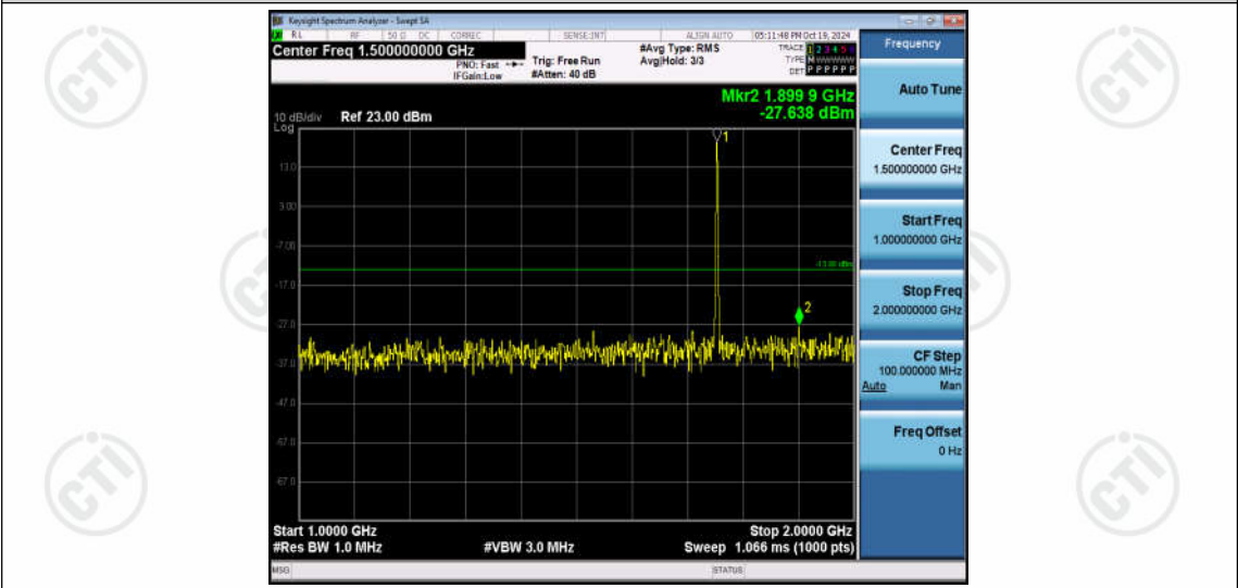
Band4-3MHz-16QAM-20385-1RB#0-Range2:1000~2000MHz
