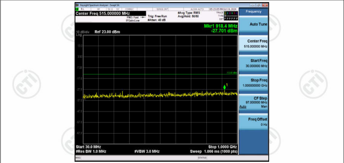
Band4-5MHz-16QAM-20375-1RB#0-Range1:30~1000MHz
