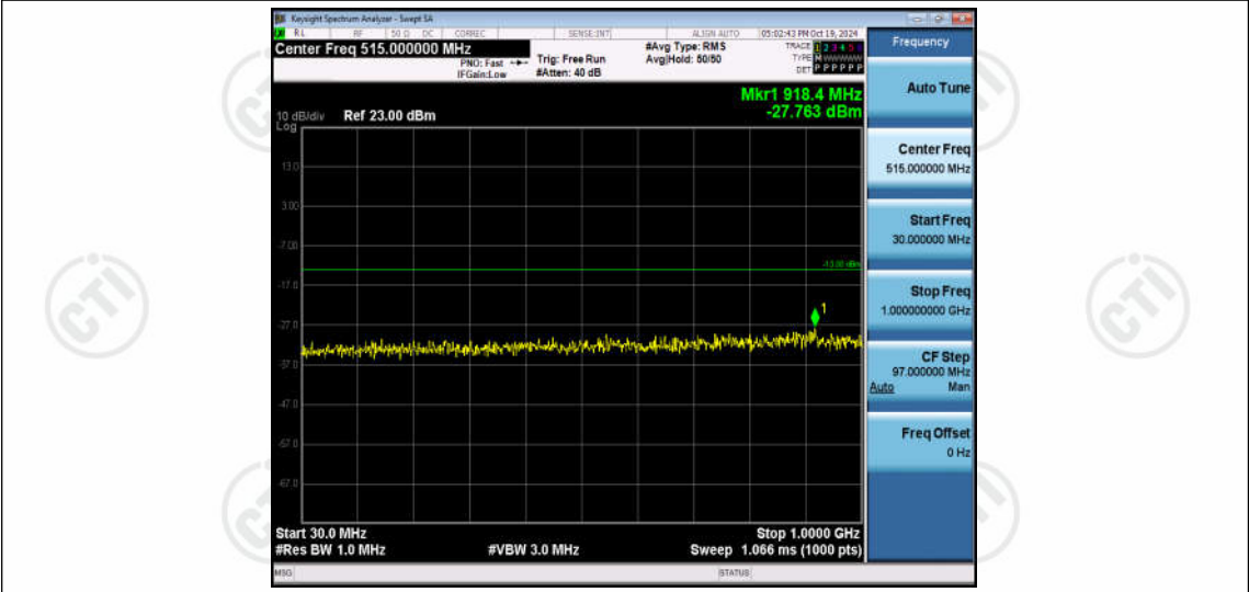
Band4-20MHz-QPSK-20050-1RB#0-Range1:30~1000MHz
