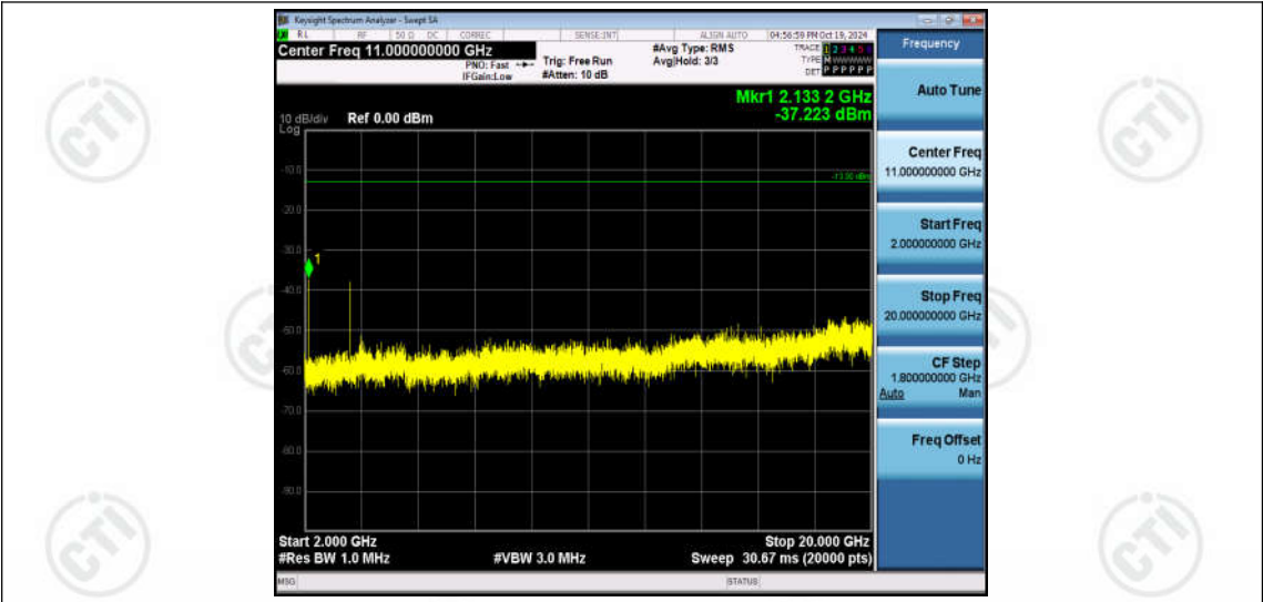
Band4-10MHz-QPSK-20175-1RB#0-Range3:2000~20000MHz
