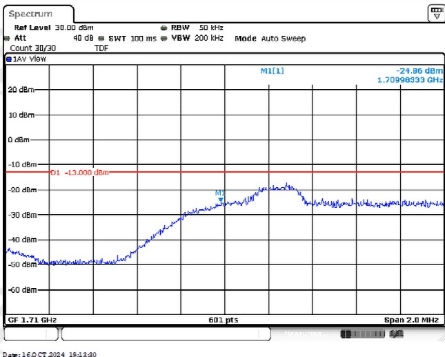
Band4-3MHz-16QAM-19965-1RB#14
