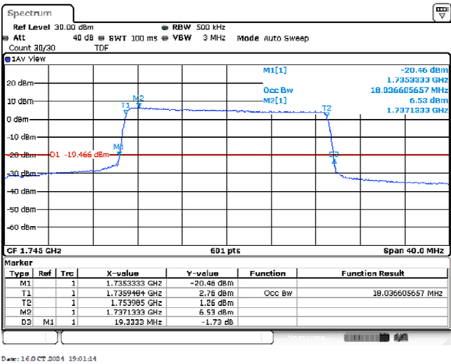
Band4-20MHz-QPSK-20300-100RB#0-18.037
