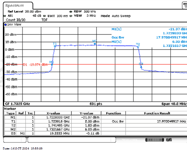
Band4-20MHz-QPSK-20175-100RB#0-17.97
