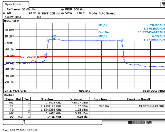
Band4-15MHz-QPSK-20325-75RB#0-13.527
