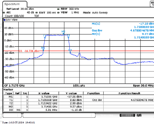
Band4-15MHz-16QAM-20025-25RB#0-4.675
