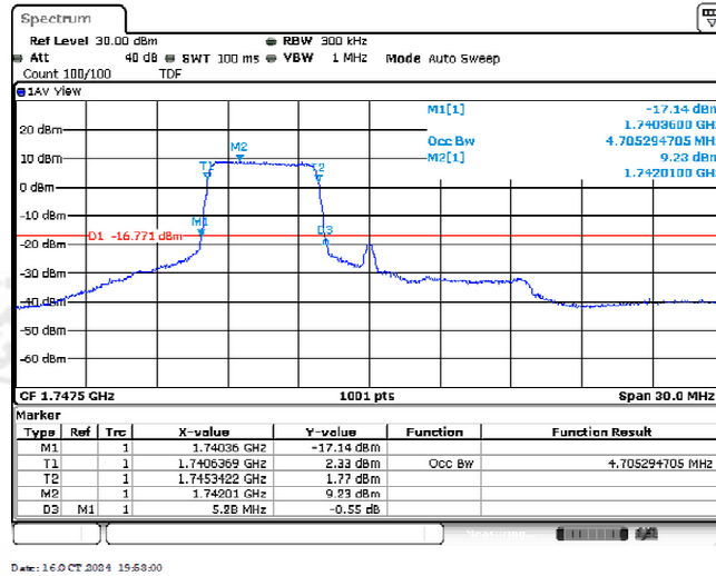
Band4-15MHz-16QAM-20325-25RB#0-4.705
