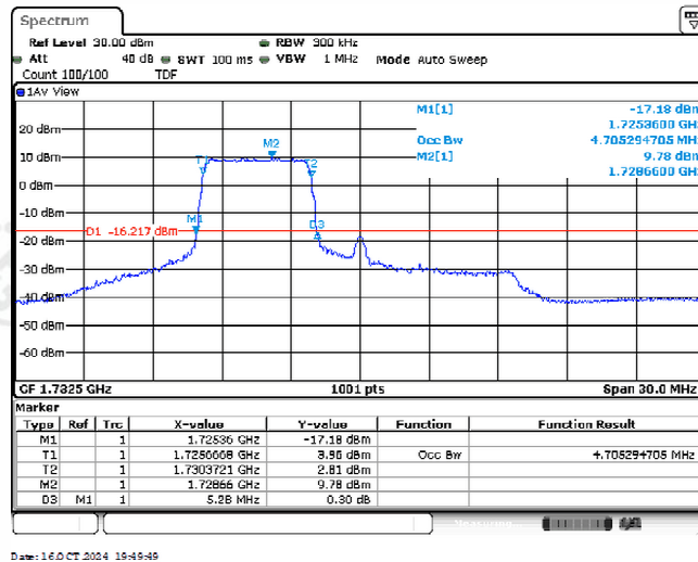
Band4-15MHz-16QAM-20175-25RB#0-4.705
